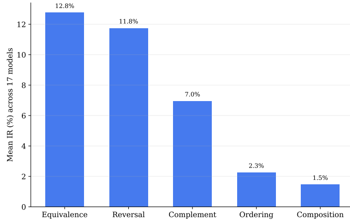
Figure 4: Transformation-family difficulty, averaged over 17 models. Equivalence (paraphrase) and Reversal are hardest; Composition and Ordering are easiest. The ranking generalizes moderately well across models (mean pairwise \rho = 0.57 ), not near-perfectly.
