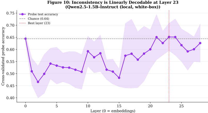
Figure 10: Layer Probe Accuracy in Qwen-2.5-1.5B-Instruct (local, white box)
