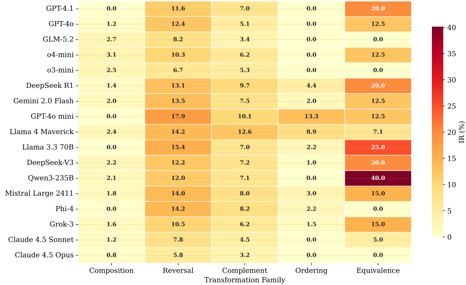
Figure 7: Inconsistency rate (%) by model and transformation family.
