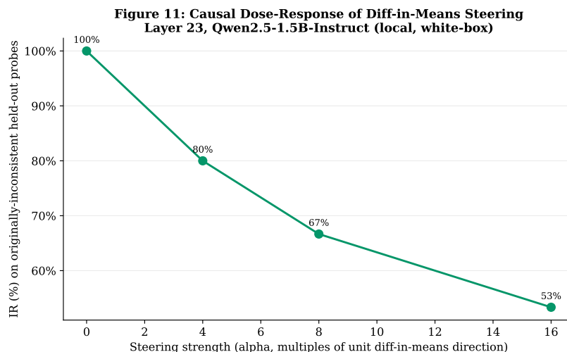
Figure 11: Effect of a causal intervention on internal activations. Inconsistency rate on held-out probes originally answered inconsistently, measured at increasing intervention strength.
