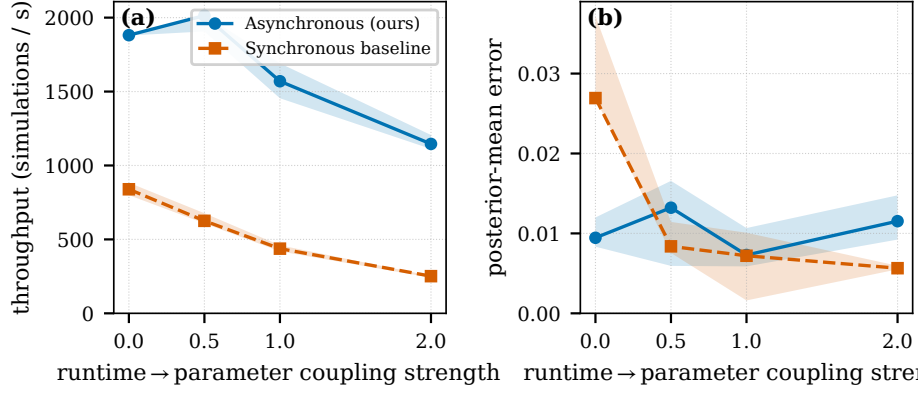
Fig. 4 Parameter-coupled runtime on the Gaussian-mean benchmark (analytic posterior; 48 workers, 60s budget, five replicates; bands are inter-quartile ranges). The post-evaluation delay grows with the inferred mean, so one region of parameter space is sampled far more often than its mirror image. (a) Aggregate throughput falls as the coupling steepens (more steeply for the barrier-bound baseline), confirming that the fast region dominates the raw sample counts. (b) Posterior-mean error to the analytic posterior nonetheless does not increase with coupling and stays comparable between the asynchronous method and the discard-latecomers synchronous baseline, so the over-representation does not measurably distort the reported posterior at these coupling levels.
