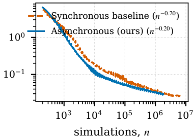
(b) g-and-k, 4-D, 2 ms
