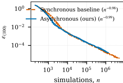
(a) Gaussian mean, 1-D, 0.1 ms
