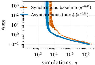
(c) Lotka-Volterra, 4-D, 4 ms
