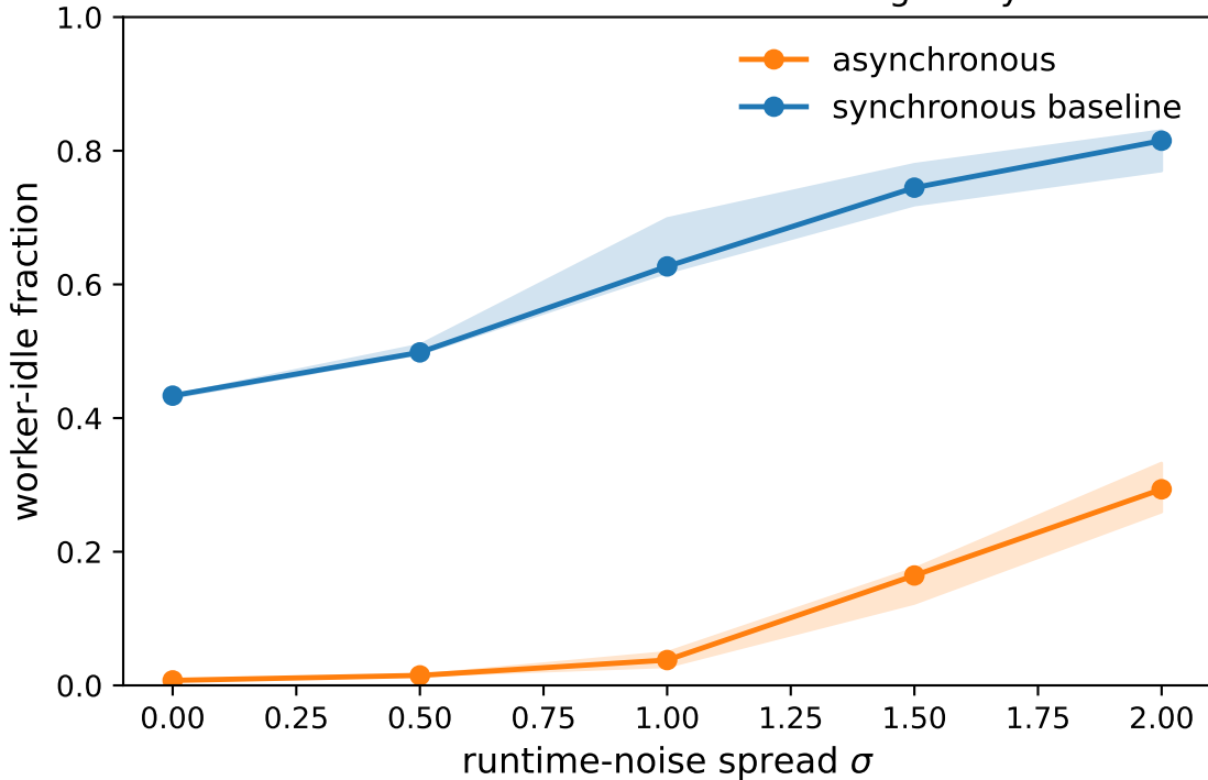
Worker utilization loss vs. heterogeneity
