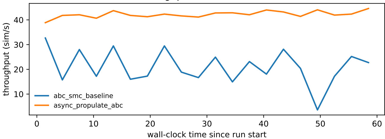
Throughput over time: \sigma=1
