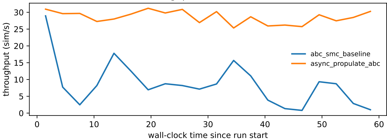
Throughput over time: \sigma=1.5
