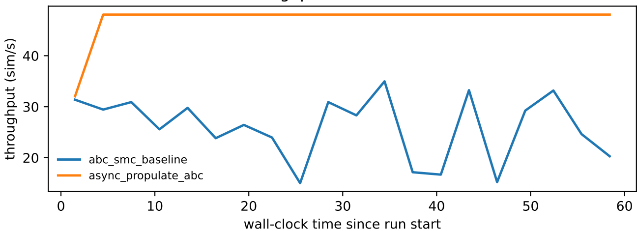
Throughput over time: \sigma=0.5
