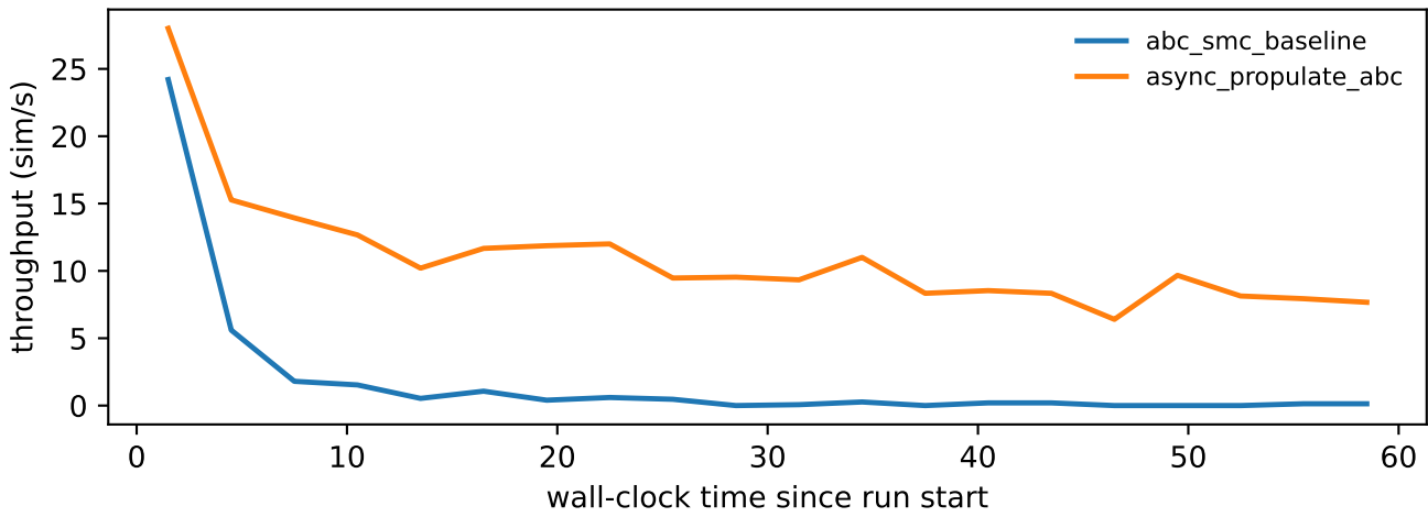
Throughput over time: \sigma=2
