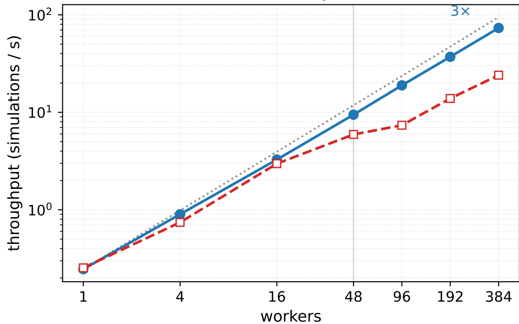
Cellular Potts (costly simulator)
