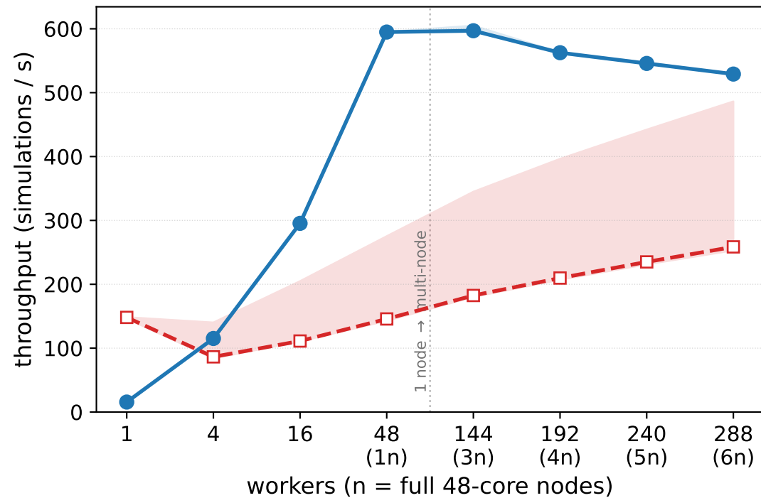
Lotka--Volterra (near-instant simulator)
