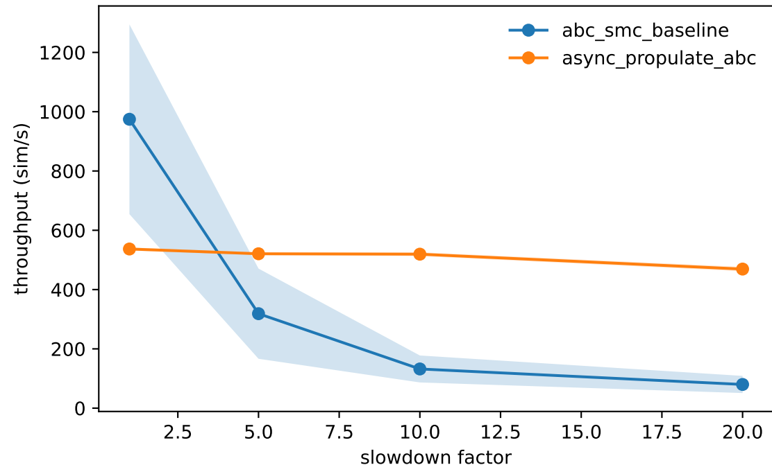
Throughput vs. straggler slowdown by method
