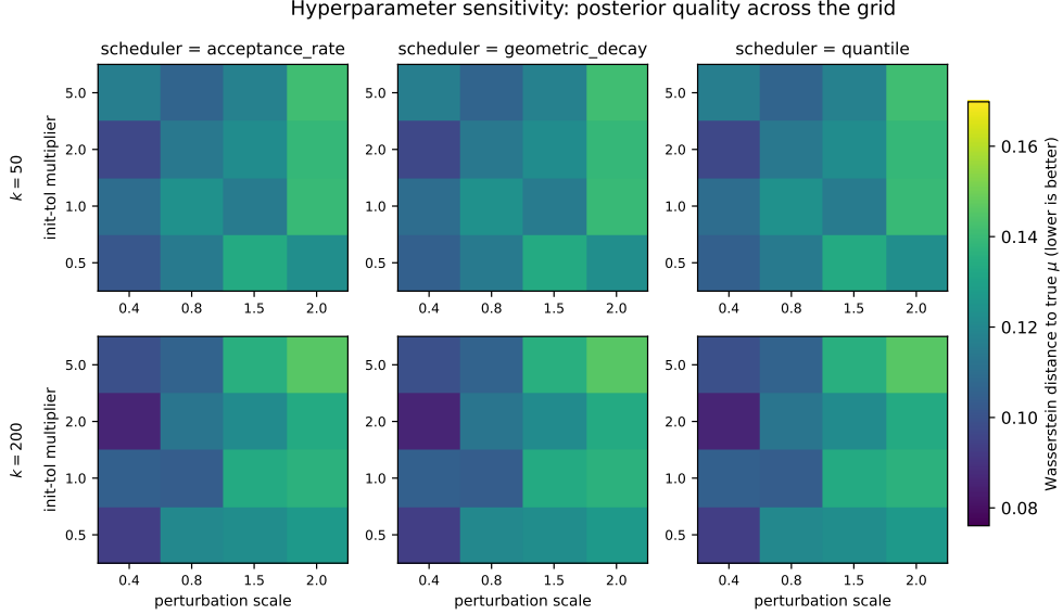
Fig. 14 Hyperparameter sensitivity of the asynchronous method, measured by posterior quality (Wasserstein distance to the true \mu , lower is better; averaged over replicates and smoothing kernel). Each panel sweeps perturbation scale ( x ) against the initial-tolerance multiplier ( y ); panels are faceted by archive size k (rows) and tolerance scheduler (columns). Quality is stable across the grid (Wasserstein \approx 0.08 – 0.17 ) with no failure region; the scheduler has no discernible effect, while larger perturbation scales degrade quality only mildly.
