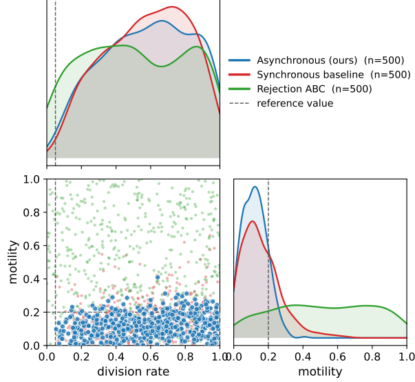
Fig. 12 Cellular Potts posterior (division rate, motility) on the real cellsInSilico simulator: asynchronous (blue), synchronous baseline (red), and rejection ABC (green), with dashed lines at the reference values. The asynchronous posterior is drawn from its AMIS estimator (500 resampled draws); the synchronous baseline and rejection ABC show their final populations (500 each). The asynchronous method and the synchronous baseline both place their motility mass at low values while the division rate is only weakly identified by the summaries for all methods, and both concentrate more tightly than rejection ABC.
