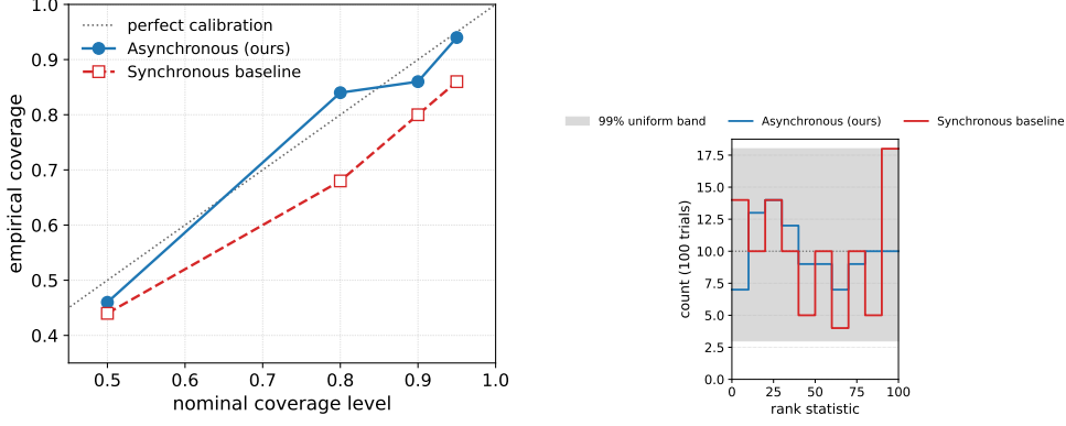
Fig. 7 Simulation-based calibration on Gaussian-mean inference: empirical coverage versus nominal level (left) and rank histogram (right). The asynchronous estimator is close to calibrated.
