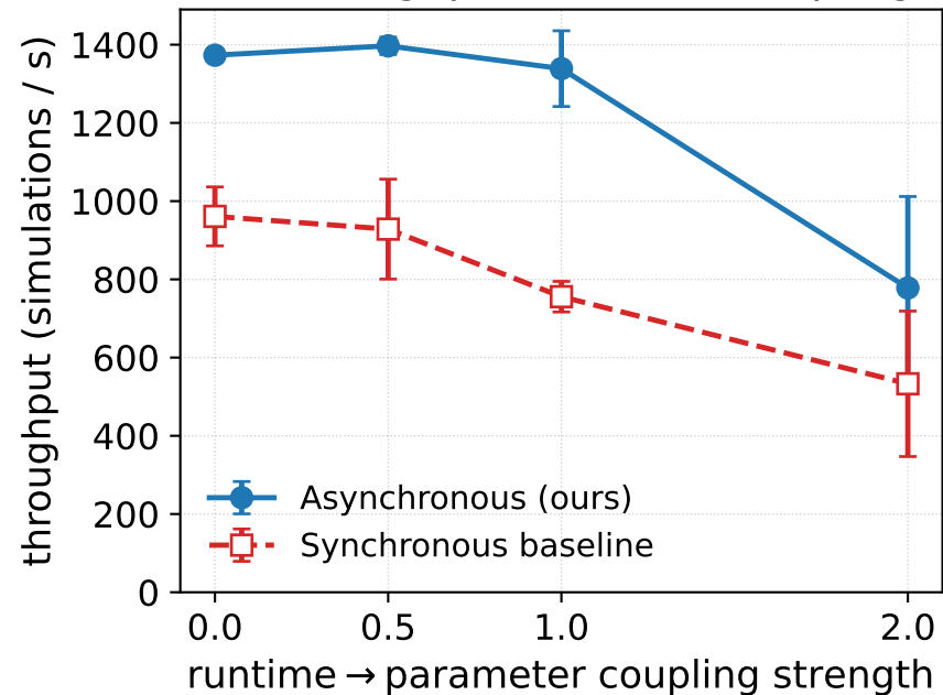
(a) throughput falls with coupling
