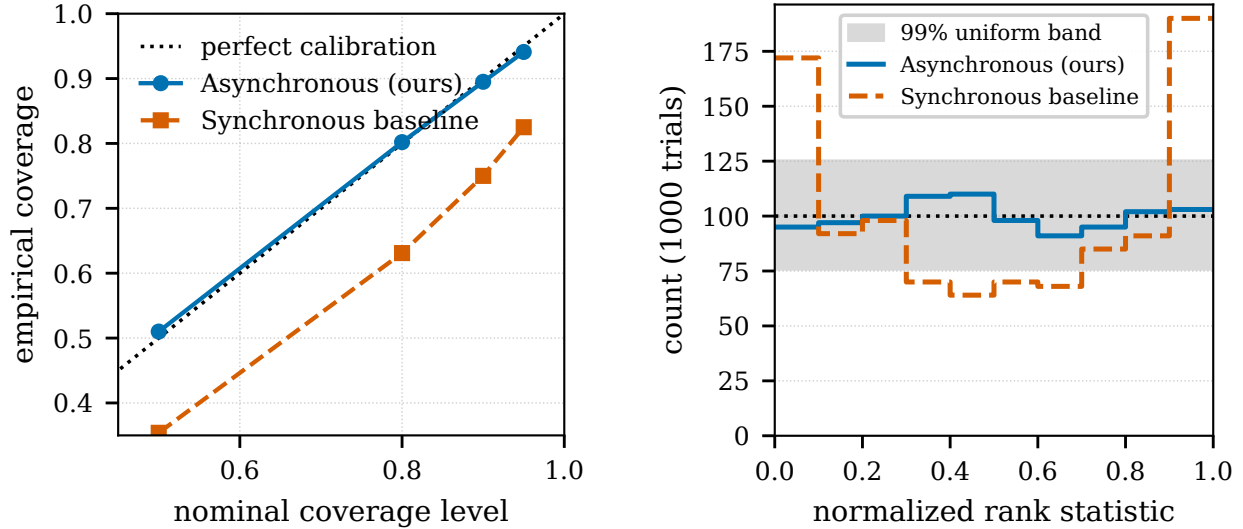
Figure 12: Simulation-based calibration on Gaussian-mean inference (1000 trials; the reported full-history AMIS posterior): empirical coverage versus nominal level (left) and rank histogram (right). The asynchronous estimator is close to calibrated.
