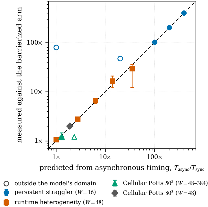
Figure 1: Barrier cost predicted from the asynchronous arm’s timing (§5.3) against the cost measured with the barrierized twin, for the straggler (16 workers), heterogeneity (48) and Cellular Potts campaigns ( 50^3 at 48–384 workers, utilization ratio, earlier configuration; 80^3 at 48, against pyABC). Medians with replicate ranges; the dashed line is equality; open markers are the three configurations outside the model’s domain.
