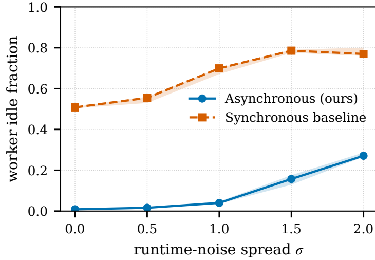
Figure 7: Worker utilization loss under runtime heterogeneity: the fraction of worker wall-clock spent idle versus the runtime-noise spread \sigma (five replicates; bands are inter-quartile ranges). The synchronous baseline idles at generation barriers (its idle fraction rises from \approx 0.51 to \approx 0.79 as heterogeneity grows) while the asynchronous method stays near-fully utilized (idle fraction \approx 0.01 rising to \approx 0.27 ).
