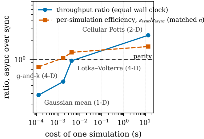
Figure 3: Throughput ratio and per-simulation efficiency of the asynchronous method over the matched synchronous baseline, against the cost of one simulation, one point per benchmark (Table 3). Both rise with the cost; throughput parity is reached at about 4ms per simulation at these budgets and this placement (§6.3).
