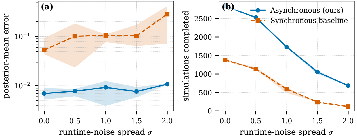
Figure 8: Inference per unit wall clock under runtime heterogeneity (Gaussian mean, analytic posterior, 48 workers, 60s budget, five replicates; bands are inter-quartile ranges). Left: error of the archive mean (the unweighted top- k archive, not the reported estimator; §6.4) to the analytic posterior mean, against the runtime spread \sigma . Right: simulations completed within the budget. The barrier starves the synchronous baseline as \sigma grows; the asynchronous method’s error stays flat.
