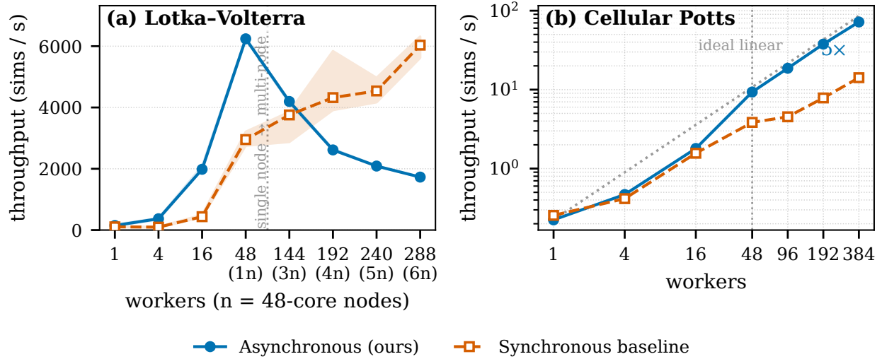
Figure 2: Strong scaling at a fixed wall-clock budget against a synchronous baseline with population \max(100, W) . Left: Lotka–Volterra (4ms; 180s; medians and inter-quartile ranges over five replicates). Right: Cellular Potts 50^3 , earlier configuration (5.1s; 1800s; log-log), with linear scaling dotted; the asynchronous method reaches 97% parallel efficiency from one node to eight (84% from one worker).
