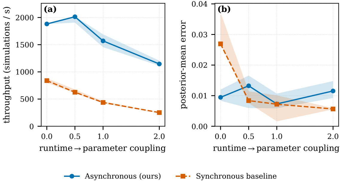
Figure 10: Parameter-coupled runtime on the Gaussian-mean benchmark (analytic posterior; 48 workers, 60s budget, five replicates; bands are inter-quartile ranges). The post-evaluation delay grows with the inferred mean, so one region of parameter space is sampled far more often than its mirror image. (a) Aggregate throughput falls as the coupling steepens (monotonically for the barrier-bound baseline, and from a peak at c = 0.5 for the asynchronous method), consistent with the fast region dominating the raw sample counts. (b) Posterior-mean error to the analytic posterior nonetheless does not increase with coupling and stays comparable between the asynchronous method and the discard-latecomers synchronous baseline, so the over-representation does not measurably distort the reported posterior at these coupling levels.
