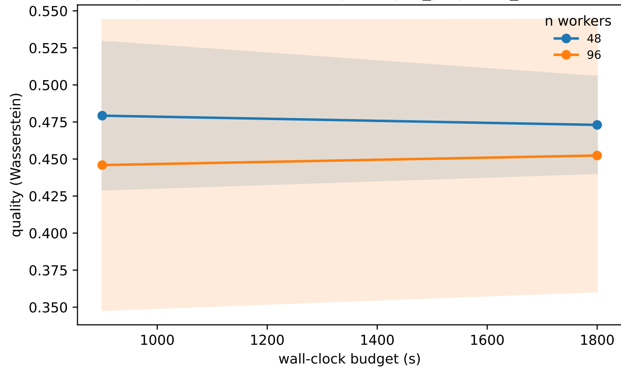
Quality vs fixed wall-clock budget: async_propulate_abc, k=100
