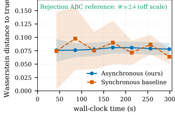
Fig. 10 Gaussian-mean posterior recovery: Wasserstein distance to the analytic posterior versus wall-clock time, with replicate confidence bands. The asynchronous method (archive) tracks the matched synchronous baseline (generation) throughout the budget; the inset shows both far below the rejection-ABC reference ( W \approx 2.4 ).
