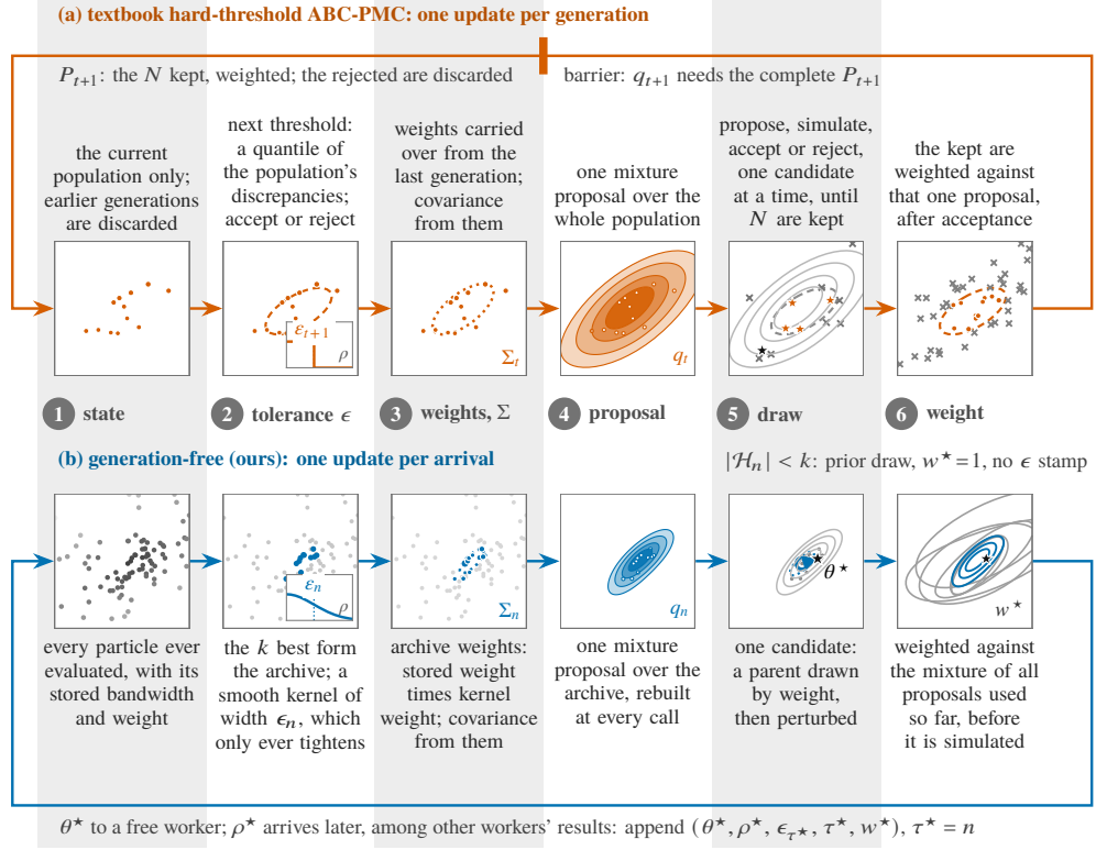
Fig. 1 One generation of ABC-PMC (a) against one single-arrival update of Algorithm 1 (b), step by step on a two-dimensional toy ( k = N = 12 ). Row (a) is textbook PMC with a quantile schedule and a hard threshold, \omega_i^{(t+1)} \propto \pi(\theta_i)/q_t(\theta_i) normalized over the N kept; it is not the matched-kernel pyABC baseline of §5.2. In row (b), \epsilon_n = \min(\epsilon_{\text{hist}}, \epsilon_{\text{sched}}) , \Sigma_n = L_n L_n^\top , and w^* = \pi(\theta^*)/\bar{q}_n^{\text{on}}(\theta^*) with the denominator of (4) over the stored proposals. w^* is assigned before the simulation, stored with the particle and never reported: the reported posterior reweights every particle of \mathcal{H}_n by (7). Bootstrap draws ( |\mathcal{H}_n| < k ) are prior draws with w^* = 1 and no bandwidth stamp. Point sizes vary where weights do (a1–a3 by \omega^{(t)} , a6 by \omega^{(t+1)} , b3 by \bar{W}_j ); shading in b1 is \rho_i (light: far); dotted ellipses are \Sigma_t and \Sigma_n ; gray contours are the current proposal in a5 and b5 and the stored proposals q_s in b6; the dashed ellipse in row (a) is the hard acceptance region; the inset in column 2 is the kernel over \rho , the Gaussian K_{\epsilon_n} in (b) against the indicator in (a).
