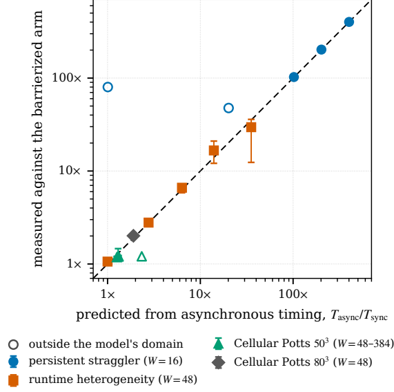
Fig. 2 Barrier cost predicted from the asynchronous arm’s timing (§5.3) against the cost measured with the barrierized twin, for the straggler (16 workers), heterogeneity (48) and Cellular Potts campaigns ( 50^3 at 48–384 workers, utilization ratio, earlier configuration; 80^3 at 48, against pyABC). Medians with replicate ranges; the dashed line is equality; open markers are the three configurations outside the model’s domain.
