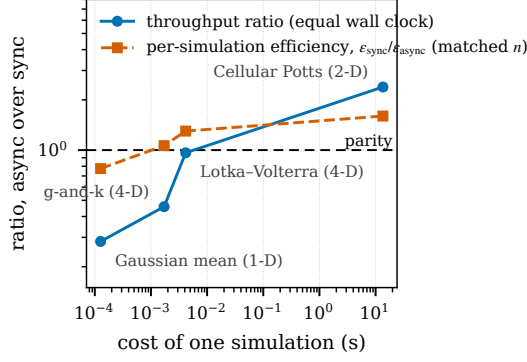
Fig. 4 Throughput ratio and per-simulation efficiency of the asynchronous method over the matched synchronous baseline, against the cost of one simulation, one point per benchmark (Table 3). Both rise with the cost; throughput parity is reached at about 4 ms per simulation at these budgets and this placement (§6.3).
