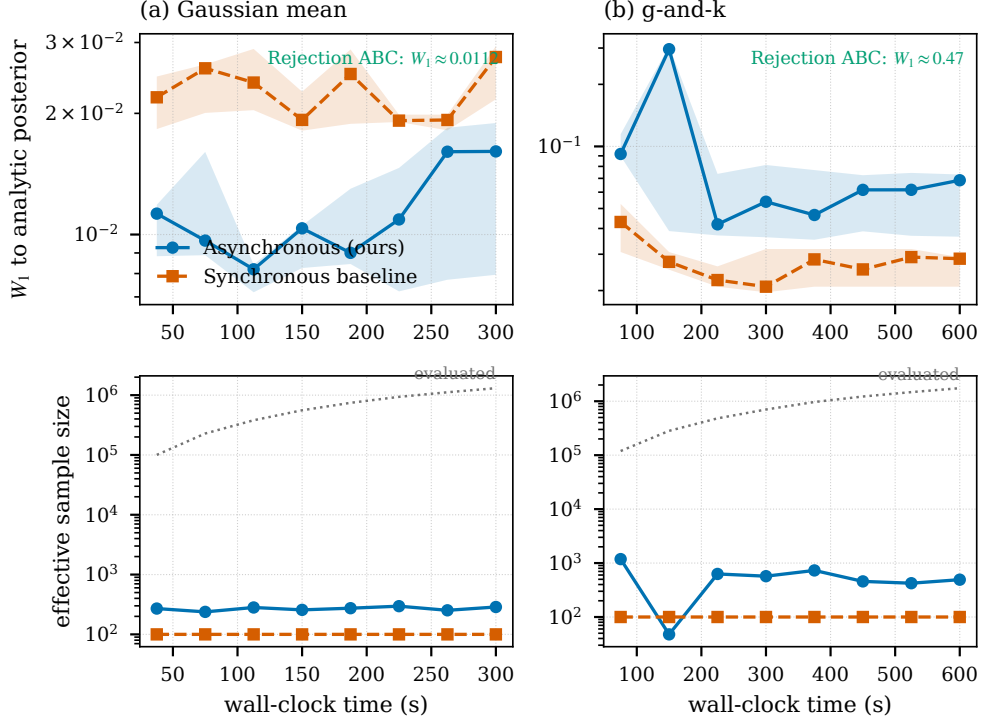
Fig. 5 What the reported estimator recovers, and with how many effective particles. Each method is scored on the posterior it reports (§5.3) against the analytic posterior (a) and the g-and-k reference posterior (b). Top: W_1 , median and inter-quartile range over five replicates. Bottom: the effective sample size of the reported posterior, with the evaluated-particle count dotted; the history grows by more than an order of magnitude and the effective sample does not follow it.
