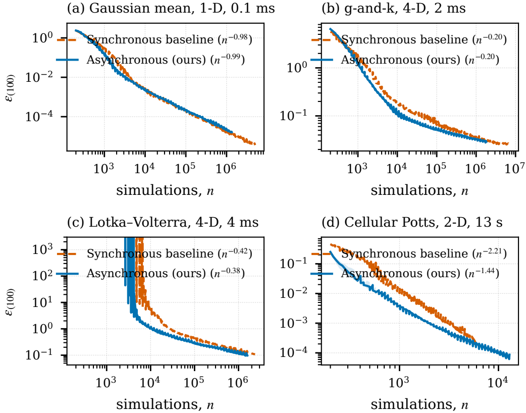
Figure 10: Tolerance against simulations spent, \epsilon_{(100)}(n) , asynchronous against the matched synchronous baseline on every benchmark (medians and replicate range over five replicates; the slope over the last decade of n in the legend). The vertical gap at equal n is the per-simulation efficiency, the horizontal extent is what the wall clock bought. On Lotka–Volterra 98% of simulations return the extinction fallback, so \epsilon_{(100)} sits on that plateau until about 5000 draws have produced 100 survivors; the plateau is cut off.
