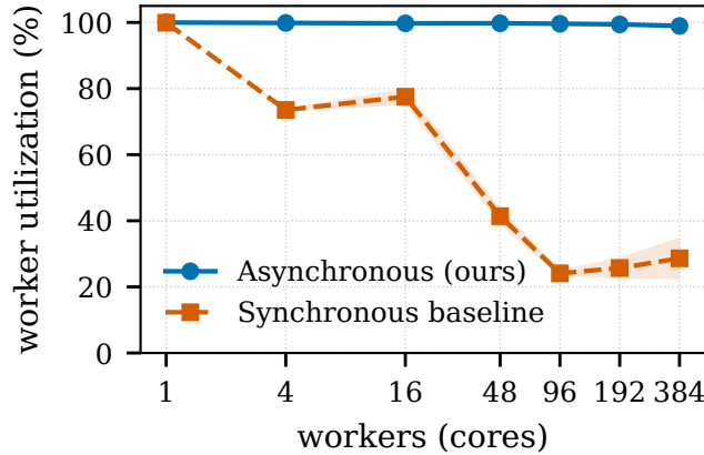
Figure 14: Cellular Potts 50^3 worker utilization in the benchmark’s earlier single-simulation configuration (fraction of worker wall-clock spent inside the simulator) versus worker count (1800s budget; error bars are \pm 1 s.d.); the synchronous baseline uses a population equal to the worker count (Fig. 3, right). The asynchronous method stays \approx 98.9 – 99.8\% utilized at every scale. The synchronous baseline fills every core within a generation but then idles at the barrier waiting for the slowest simulation, so its utilization falls to \approx 24 – 29\% ( 41\% \rightarrow 24\% \rightarrow 26\% \rightarrow 29\% at 48/96/192/384 workers, i.e. \approx 70 – 76\% idle at every multi-node scale). The figure is the measured utilization behind the synchronous method’s sub-linear scaling in Fig. 3 (right).
