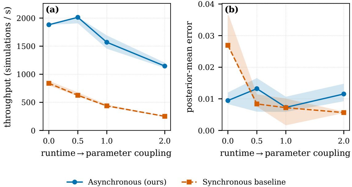
Figure 11: Parameter-coupled runtime on the Gaussian-mean benchmark (analytic posterior; 48 workers, 60s budget, five replicates; bands are inter-quartile ranges). The post-evaluation delay grows with the inferred mean, so one region of parameter space is sampled far more often than its mirror image. (a) Aggregate throughput falls as the coupling steepens (monotonically for the barrier-bound baseline, and from a peak at c = 0.5 for the asynchronous method), consistent with the fast region dominating the raw sample counts. (b) Posterior-mean error to the analytic posterior nonetheless does not increase with coupling and stays comparable between the asynchronous method and the discard-latecomers synchronous baseline, so the over-representation does not measurably distort the reported posterior at these coupling levels.
