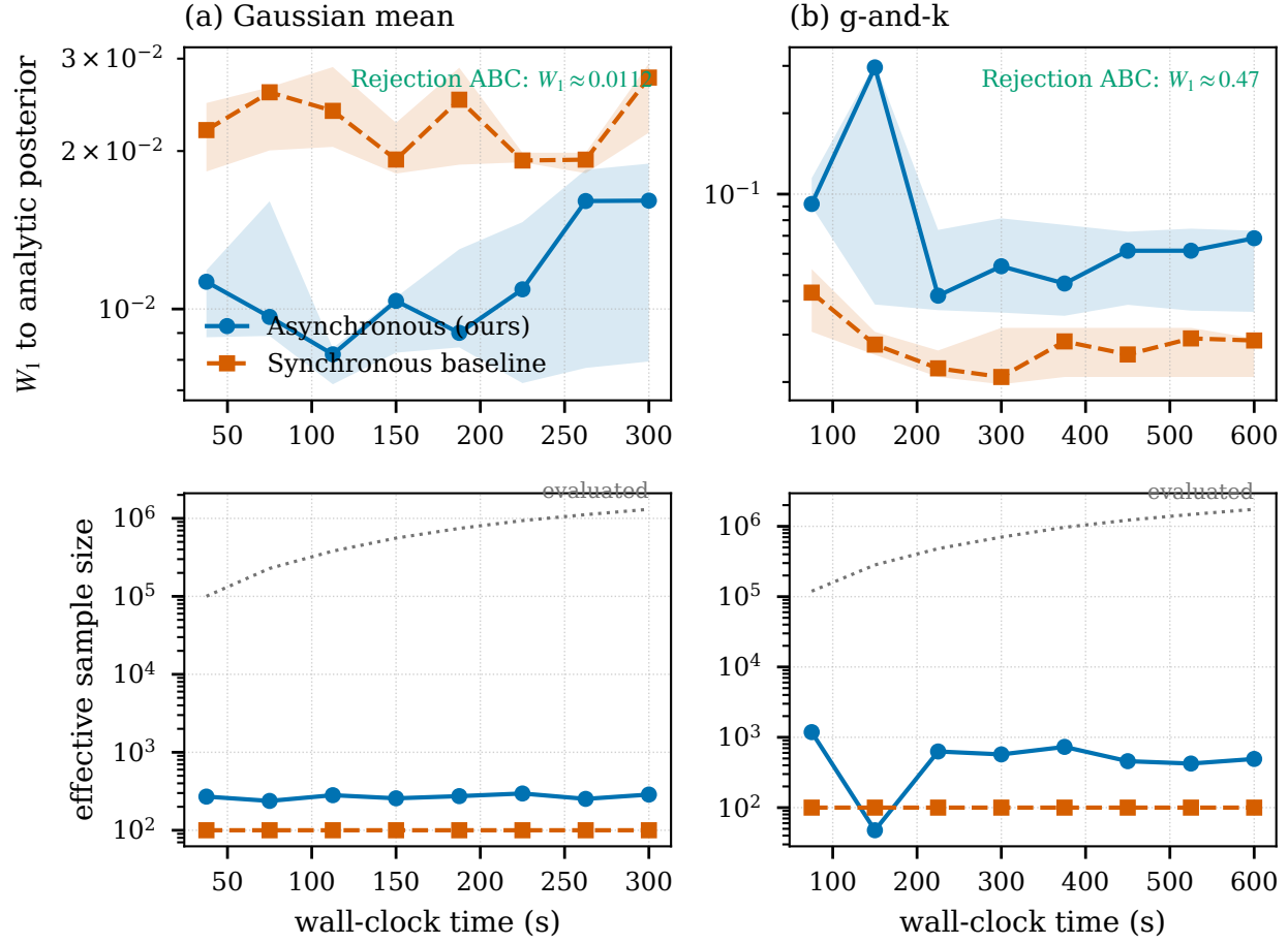
Figure 5: What the reported estimator recovers, and with how many effective particles. Each method is scored on the posterior it reports (§5.3) against the analytic posterior (a) and the g-and-k reference posterior (b). Top: W_1 , median and inter-quartile range over five replicates. Bottom: the effective sample size of the reported posterior, with the evaluated-particle count dotted; the history grows by more than an order of magnitude and the effective sample does not follow it.
