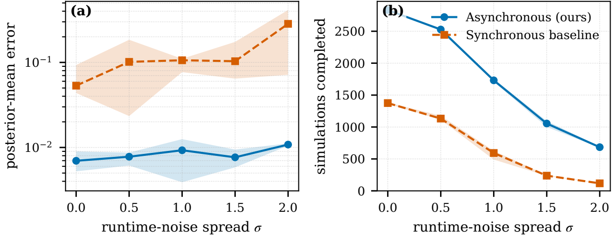
Figure 9: Inference per unit wall clock under runtime heterogeneity (Gaussian mean, analytic posterior, 48 workers, 60s budget, five replicates; bands are inter-quartile ranges). Left: error of the archive mean (the unweighted top- k archive, not the reported estimator; §6.4) to the analytic posterior mean, against the runtime spread \sigma . Right: simulations completed within the budget. The barrier starves the synchronous baseline as \sigma grows; the asynchronous method’s error stays flat.
