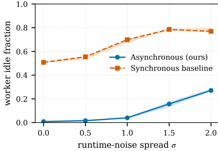
Figure 8: Worker utilization loss under runtime heterogeneity: the fraction of worker wall-clock spent idle versus the runtime-noise spread \sigma (five replicates; bands are inter-quartile ranges). The synchronous baseline idles at generation barriers (its idle fraction rises from \approx 0.51 to \approx 0.79 as heterogeneity grows) while the asynchronous method stays near-fully utilized (idle fraction \approx 0.01 rising to \approx 0.27 ).
