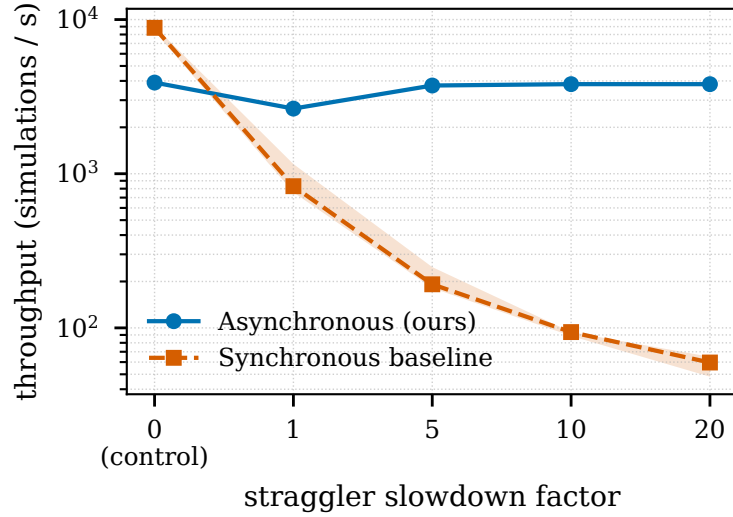
Figure 7: Throughput (median and inter-quartile range over five replicates) against straggler slowdown on the Gaussian-mean benchmark, 300s wall-limited campaign; one of 16 workers carries a permanent post-evaluation delay of 0.1s scaled by the factor. The synchronous baseline falls from \approx 8800 to \approx 60 simulations per second because every generation waits for it; the asynchronous method holds \approx 2600 – 3900 , and the twin campaign’s asynchronous arm (Table 2) agrees within 15% except at 1\times . Logarithmic throughput axis.
