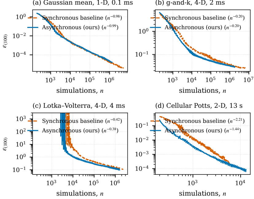
Fig. F2 Tolerance against simulations spent, \epsilon_{(100)}(n) , asynchronous against the matched synchronous baseline on every benchmark (medians and replicate range over five replicates; the slope over the last decade of n in the legend). The vertical gap at equal n is the per-simulation efficiency, the horizontal extent is what the wall clock bought. On Lotka–Volterra 98% of simulations return the extinction fallback, so \epsilon_{(100)} sits on that plateau until about 5000 draws have produced 100 survivors; the plateau is cut off.
