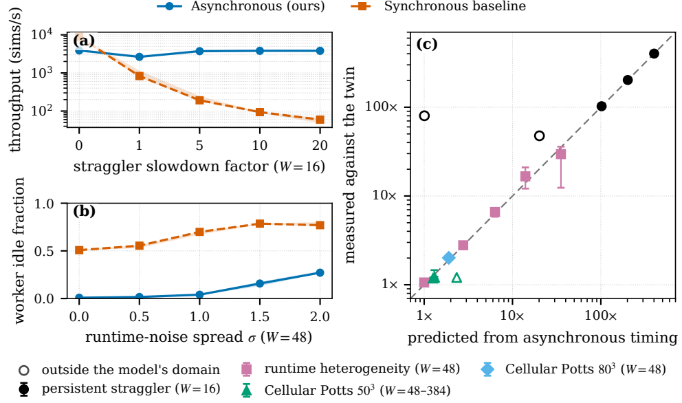
Fig. 2 The barrier against pyABC and against our own twin. (a) Throughput under a persistent straggler: one of 16 workers carries a permanent post-evaluation delay of 0.1 s scaled by the factor (Gaussian mean, 300 s; medians and inter-quartile ranges over five replicates; logarithmic axis). The synchronous pyABC baseline falls from \approx 8800 to \approx 60 simulations per second because every generation waits for the slow worker; the asynchronous method holds \approx 2600 – 3900 . The twin campaign’s asynchronous arm (Table 2) agrees within 15% except at 1\times . (b) Fraction of worker time spent idle under lognormal runtime heterogeneity of spread \sigma (48 workers, 60 s): pyABC idles at its barriers ( \approx 0.51 to \approx 0.79 ) while the asynchronous method stays near-fully utilized ( \approx 0.01 to \approx 0.27 ). (c) Barrier cost predicted from the asynchronous arm’s timing (§5.3) against the cost measured with the barrierized twin, for the straggler (16 workers), heterogeneity (48) and Cellular Potts campaigns ( 50^3 at 48–384 workers, utilization ratio, earlier configuration; 80^3 at 48, against pyABC). Medians with replicate ranges; the dashed line is equality; open markers are the three configurations outside the model’s domain.
