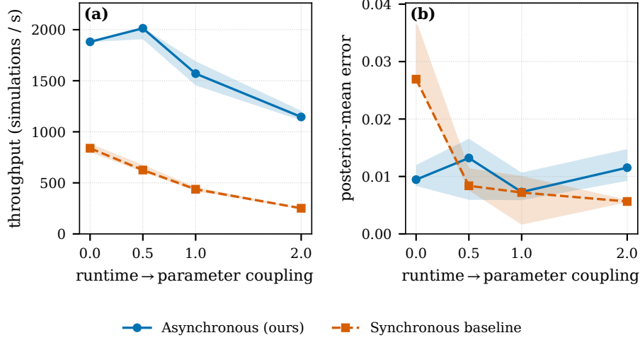
Fig. F3 Parameter-coupled runtime on the Gaussian-mean benchmark (analytic posterior; 48 workers, 60s budget, five replicates; bands are inter-quartile ranges). The post-evaluation delay grows with the inferred mean, so one region of parameter space is sampled far more often than its mirror image. (a) Aggregate throughput falls as the coupling steepens (monotonically for the barrier-bound baseline, and from a peak at c = 0.5 for the asynchronous method), consistent with the fast region dominating the raw sample counts. (b) Posterior-mean error to the analytic posterior nonetheless does not increase with coupling and stays comparable between the asynchronous method and the discard-latecomers synchronous baseline, so the over-representation does not measurably distort the posterior estimate at these coupling levels.
