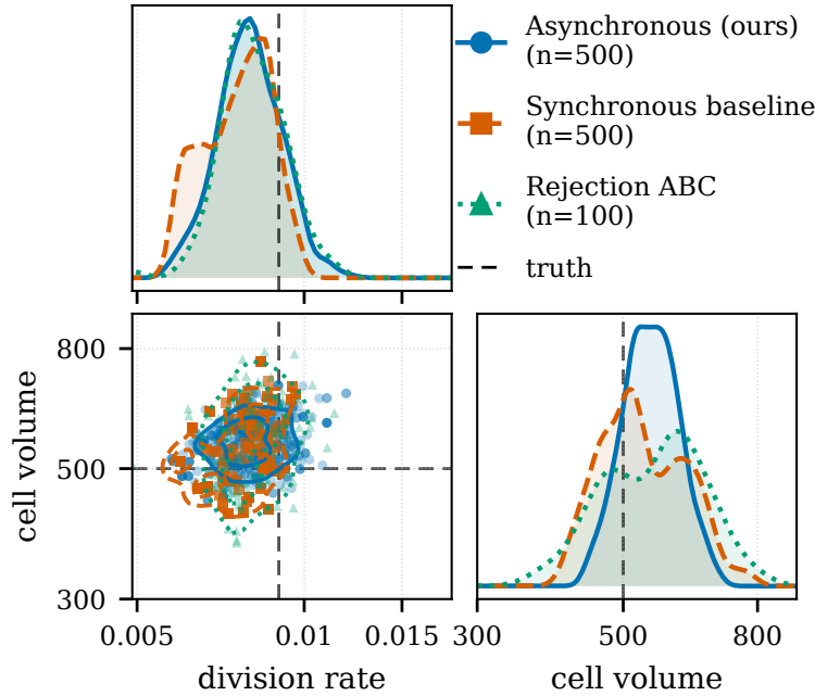
Figure 6: Cellular Potts posterior (division rate, cell volume) on the fixed production run, replicate 0: the asynchronous AMIS estimator (500 resampled draws), the synchronous baseline’s last completed generation with pyABC’s weights (500 resampled draws), and the 100 best rejection draws (Table 5). Axes are the log-uniform prior coordinates ticked in physical units; dashed lines mark the truth. Every method recovers the division rate; the asynchronous estimator is the tightest on the cell volume.
