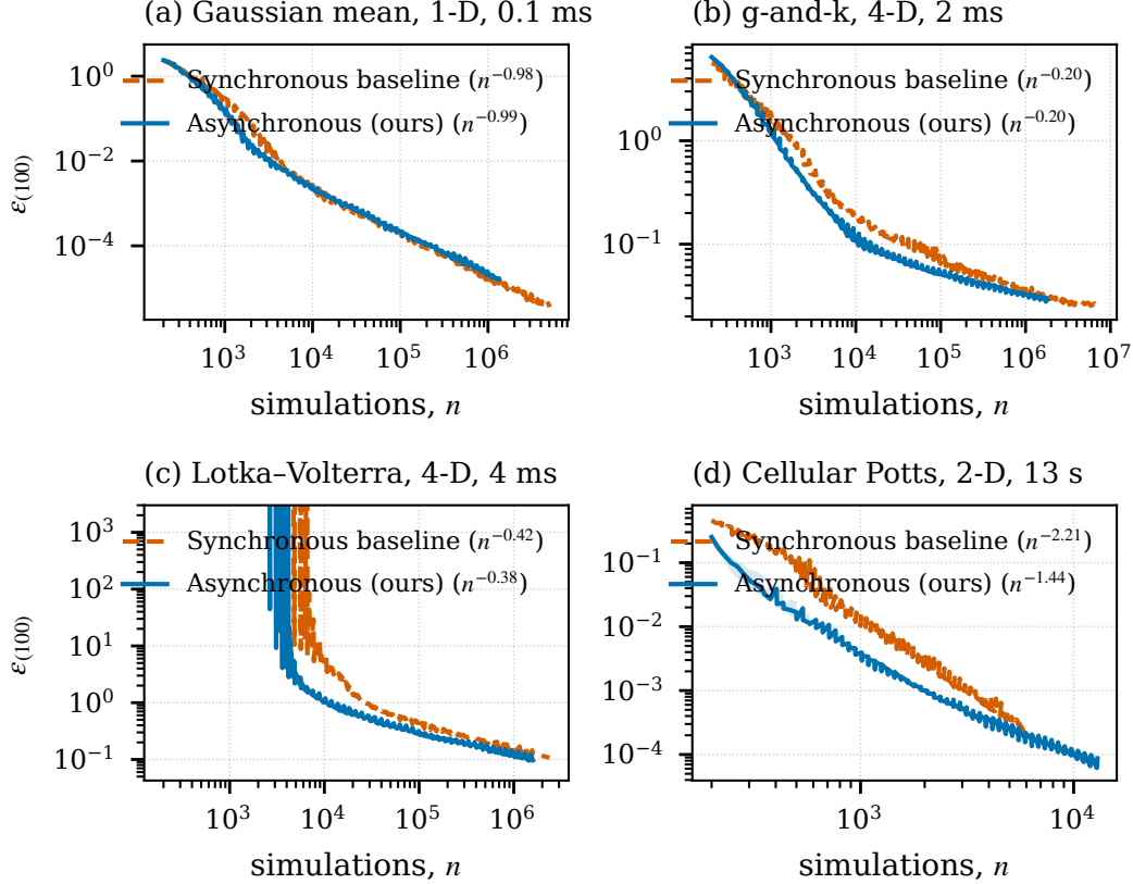
Figure 8: Tolerance against simulations spent, \epsilon_{(100)}(n) , asynchronous against the matched synchronous baseline on every benchmark (medians and replicate range over five replicates; the slope over the last decade of n in the legend). The vertical gap at equal n is the per-simulation efficiency, the horizontal extent is what the wall clock bought. On Lotka–Volterra 98% of simulations return the extinction fallback, so \epsilon_{(100)} sits on that plateau until about 5000 draws have produced 100 survivors; the plateau is cut off.
