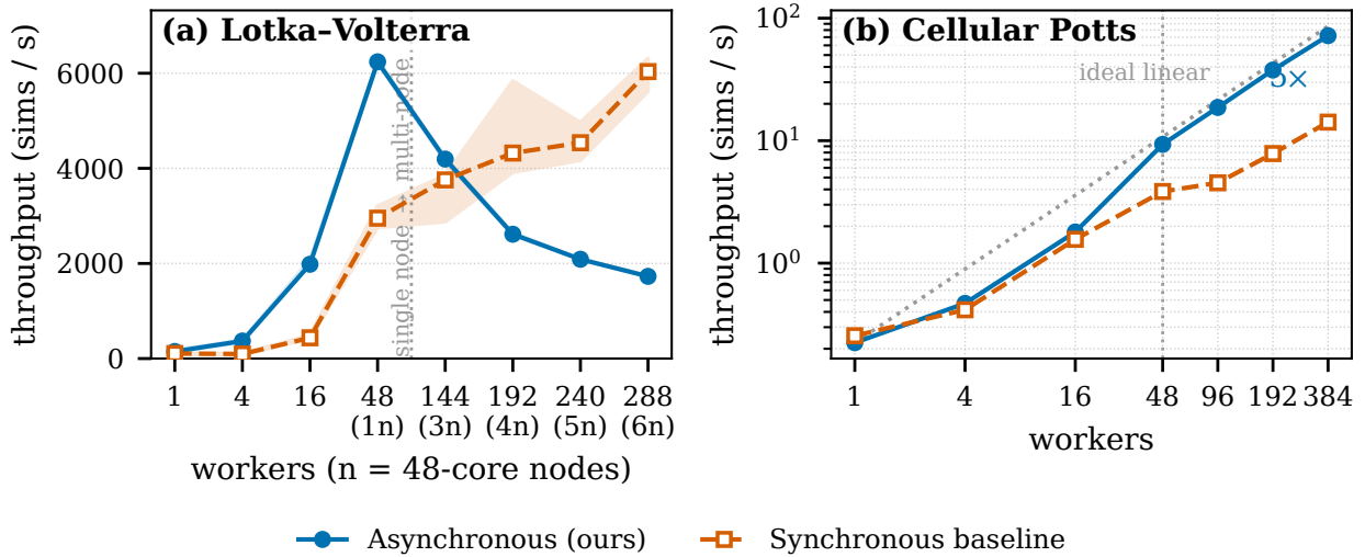
Figure 3: Strong scaling at a fixed wall-clock budget against a synchronous baseline with population \max(100, W) . Left: Lotka–Volterra (4ms; 180s; medians and inter-quartile ranges over five replicates). Right: Cellular Potts 50^3 , earlier configuration (5.1s; 1800s; log-log), with linear scaling dotted; the asynchronous method reaches 97% parallel efficiency from one node to eight (84% from one worker).
