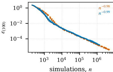
(a) Gaussian mean, 1-D, 0.1 ms
