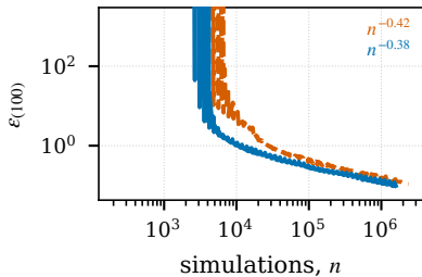
(c) Lotka-Volterra, 4-D, 4 ms
