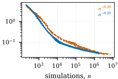
(b) g-and-k, 4-D, 2 ms
