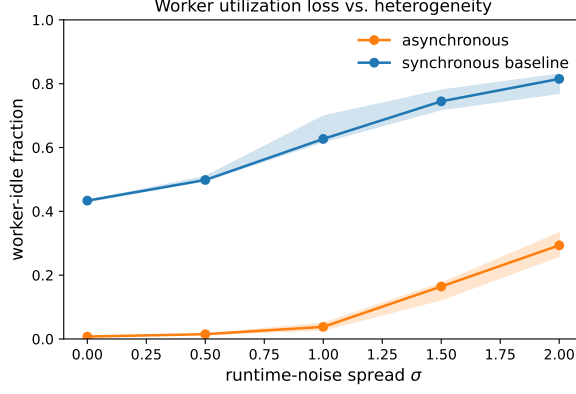
Fig. 2 Worker utilization loss under runtime heterogeneity: the fraction of worker wall-clock spent idle versus the runtime-noise spread \sigma (five replicates; bands are inter-quartile ranges). The synchronous baseline idles at generation barriers — its idle fraction rises from 0.43 to 0.82 as heterogeneity grows — while the asynchronous method stays near-fully utilized.
