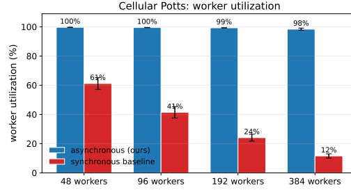
Fig. 12 Cellular Potts worker utilization (fraction of worker wall-clock spent inside the simulator) from 48 to 384 workers ( k = 100 , 1800s budget; error bars are \pm 1 s.d.), from the same run as Fig. 11. The asynchronous method stays \approx 98\text{--}99.7\% utilized at every scale, while the synchronous baseline idles at the generation barrier — and its idle fraction grows monotonically with scale (39% \rightarrow 59% \rightarrow 76% \rightarrow 88% at 48/96/192/384 workers), as more workers wait on the slowest simulation per generation. This growing barrier idle is the measured mechanism behind the synchronous plateau in Fig. 11.
