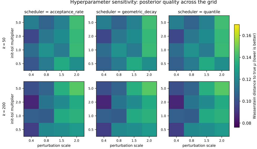
Fig. 15 Hyperparameter sensitivity of the asynchronous method, measured by posterior quality (Wasserstein distance to the true \mu , lower is better; averaged over replicates and smoothing kernel). Each panel sweeps perturbation scale ( x ) against the initial-tolerance multiplier ( y ); panels are faceted by archive size k (rows) and tolerance scheduler (columns). Quality is stable across the grid (Wasserstein \approx 0.08 – 0.17 ) with no failure region; the scheduler has no discernible effect, while larger perturbation scales degrade quality only mildly.
