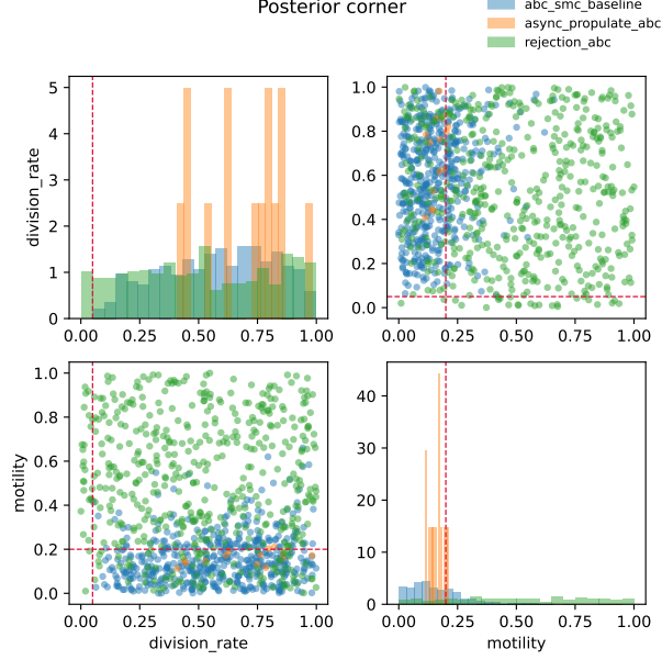
Fig. 13 Cellular Potts posterior (division rate, motility) on the real cellsInSilico simulator: the asynchronous method (orange) tracks the synchronous baseline (blue), with motility concentrating near its reference value (dashed) while the division rate is only weakly identified by the summaries for all methods. Both improve on rejection ABC (green).
