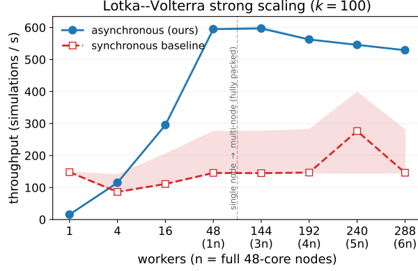
Fig. 5 Strong scaling on Lotka–Volterra: median simulation throughput versus worker count at a fixed 900 s budget ( k = 100 ; bands are inter-quartile ranges over five replicates; x -axis is categorical). Multi-node points use fully packed nodes (worker counts that are exact multiples of 48; node count n in labels). Asynchronous throughput rises almost linearly within a single node, peaks around 1–3 nodes, and then declines only gently across fully-packed nodes as per-arrival coordination begins to pay inter-node latency — a modest decline that persists even with no idle cores, confirming it is an inter-node coordination effect rather than a packing artifact. The synchronous baseline stays low and high-variance — its wide band reflects coarse quantization by the generation barrier at a fixed budget rather than a stable trend.
