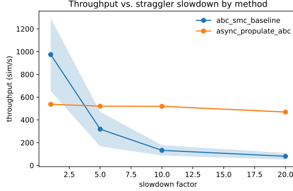
Fig. 1 Throughput versus straggler slowdown factor. The synchronous baseline degrades sharply at the generation barrier; the asynchronous method is robust.
