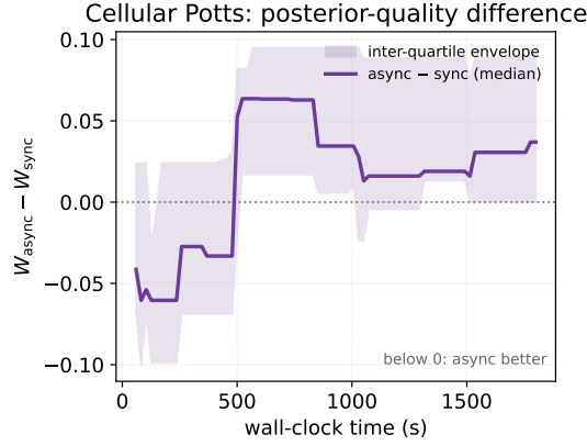
Fig. 9 Cellular Potts posterior-quality difference (asynchronous minus synchronous Wasserstein to the reference) versus wall-clock time, with a zero reference line and an inter-quartile envelope over five replicates (the per-method Cellular Potts curves of Fig. 8, differenced). The difference stays within \approx 0.06 against an absolute Wasserstein of \approx 0.4 and its envelope straddles zero for most of the budget, so the two methods are comparable on this expensive simulator; the asynchronous method ends only marginally behind, consistent with the weakly identified, near-rejection-floor regime (§7.3).
