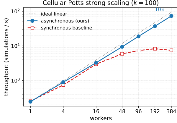
Fig. 11 Cellular Potts strong scaling: median simulation throughput versus worker count ( k = 100 , log-log; medians over the available replicates). On the cost-bearing cellsInSilico simulator the asynchronous method tracks ideal-linear scaling (dotted line) across the single-node→multi-node boundary all the way to eight nodes (384 workers, \approx 97\% parallel efficiency relative to the single-node rate), whereas the synchronous baseline plateaus at \approx 6\text{--}8 sims/s — a nearly 10\times gap at 384 workers. Contrast the near-instantaneous Lotka–Volterra case (Table 3), where per-arrival coordination caps throughput beyond one node.
