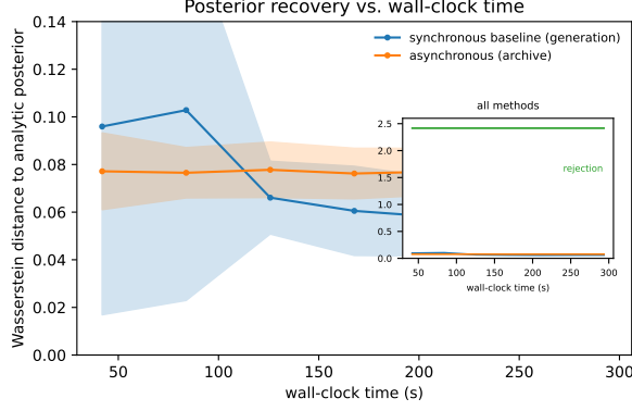
Fig. 10 Gaussian-mean posterior recovery: Wasserstein distance to the analytic posterior versus wall-clock time, with replicate confidence bands. The asynchronous method (archive) tracks the matched synchronous baseline (generation) throughout the budget; the inset shows both far below the rejection-ABC reference ( W \approx 2.4 ).
