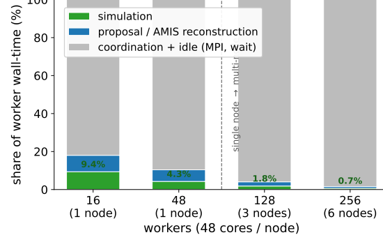
Fig. 6 Measured decomposition of asynchronous worker wall-time on Lotka–Volterra ( k = 100 ), from a dedicated instrumented run (300s, three replicates) that logs per-attempt simulation spans and per-arrival proposal/AMIS reconstruction time; the residual is coordination and idle (MPI exchange, serialization, waiting). The productive simulation fraction (green, annotated) collapses from 9.4% at 16 workers to 0.7% at 256, and the coordination/idle residual crosses 95% exactly as the job spreads beyond one node (16/48 = 1 node; 128 = 3 nodes; 256 = 6 nodes). The strong-scaling knee of Fig. 5 is therefore a measured property of coordinating a near-instantaneous simulator, not an inferred one.
