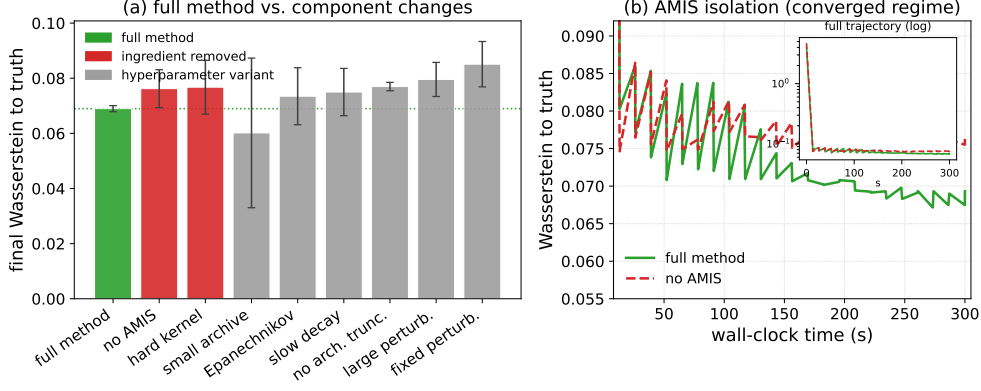
Fig. 14 Ablation on the Gaussian-mean benchmark (analytic posterior; 48 workers, 300 s budget, k = 100 , five replicates, asynchronous method). (a) Final Wasserstein-to-truth for the full method (green), the two ingredient removals named in the claim (red: no AMIS, hard kernel), and hyperparameter variants (grey); error bars are 95% CIs and the dotted line marks the full-method mean. (b) AMIS isolation: full method vs. no-AMIS on a shared wall-clock grid (bands are \pm 1 s.d. over replicates), zoomed to the converged regime so the persistent full-method < no-AMIS gap is visible; the inset shows the full prior-to-posterior transient on a log axis.
