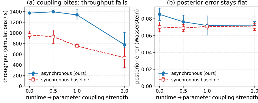
Fig. 4 Parameter-coupled runtime on the Gaussian-mean benchmark (analytic posterior; 48 workers, 60 s budget, five replicates; error bars are \pm 1 s.d.). The post-evaluation delay grows with the inferred mean, so one region of parameter space is sampled far more often than its mirror image. (a) Aggregate throughput falls by \approx 40\% as the coupling steepens — the bias bites. (b) Posterior error (Wasserstein to the analytic posterior) nonetheless stays flat and comparable between the asynchronous method and the discard-latecomers synchronous baseline: the AMIS importance weights compensate for the raw over-representation.
