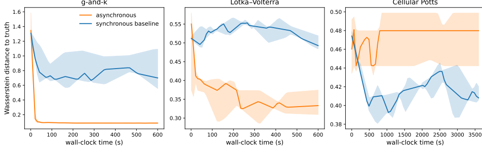
Fig. 8 Posterior quality (Wasserstein distance to the truth/reference, lower is better) versus wall-clock time on g-and-k (left), Lotka–Volterra (middle), and Cellular Potts (right), asynchronous vs. synchronous; shaded bands are inter-quartile ranges over five replicates. On the two fast simulators the asynchronous method reaches a markedly lower Wasserstein distance within the budget; on the expensive Cellular Potts simulator the two are comparable.
