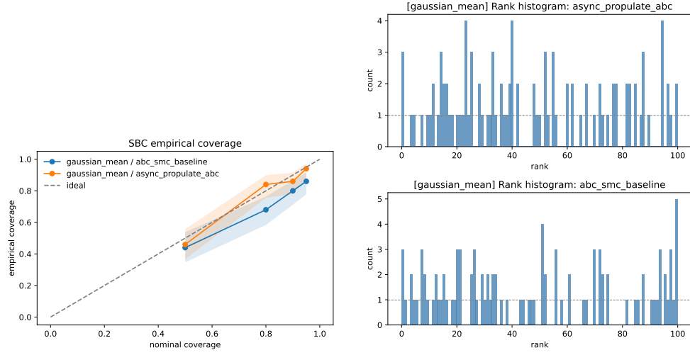
Fig. 7 Simulation-based calibration on Gaussian-mean inference: empirical coverage versus nominal level (left) and rank histogram (right). The asynchronous estimator is close to calibrated.
