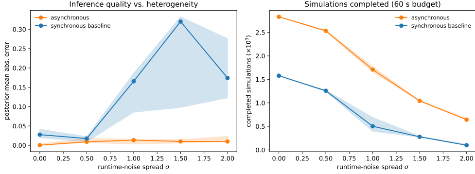
Fig. 3 Inferential efficiency under runtime heterogeneity (Gaussian-mean benchmark, analytic posterior, fixed 60 s budget, five replicates; bands are inter-quartile ranges). Left: posterior-mean error to the analytic posterior versus runtime-noise spread \sigma — the synchronous baseline degrades sharply while the asynchronous method stays flat. Right: simulations completed within the budget — the synchronous baseline is starved by barrier idling as \sigma grows, whereas the asynchronous method sustains several-fold higher completion.
