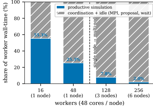
Fig. F6 Measured decomposition of asynchronous worker wall-time on Lotka-Volterra ( k = 100 ; 180 s budget) from a dedicated instrumented run. The productive simulation fraction (blue, annotated), the share of worker wall-clock spent inside the simulator, collapses from 55% at 16 workers to 2% at 256, while coordination and idle (MPI exchange, per-arrival proposal reconstruction, serialization, waiting) dominate as the job spreads beyond one node (16/48 = 1 node; 128 = 3 nodes; 256 = 6 nodes). The strong-scaling decline of Fig. 2 is therefore a measured property of coordinating a near-instantaneous simulator.
