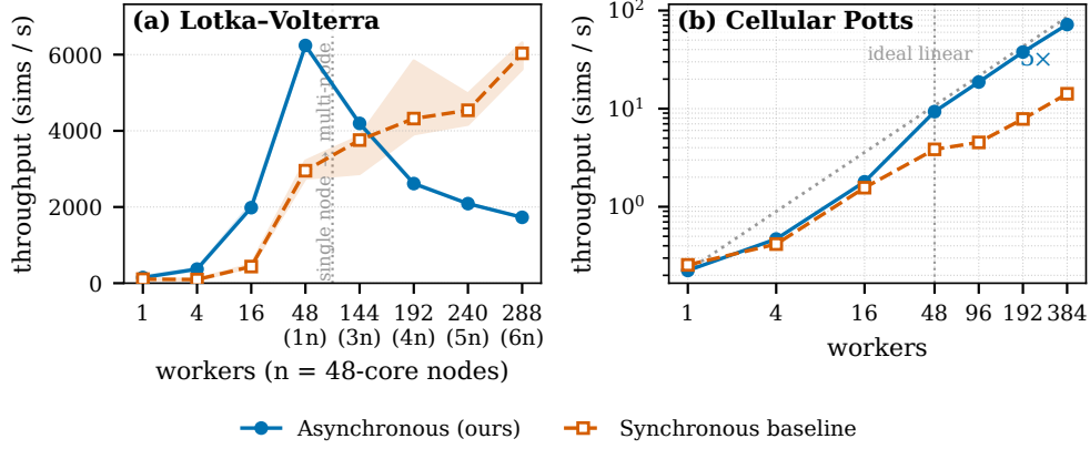
Fig. 2 Strong scaling at a fixed wall-clock budget against a synchronous baseline with population \max(100, W) . Left: Lotka–Volterra (4 ms; 180 s; medians and inter-quartile ranges over five replicates). Right: Cellular Potts 50^3 , earlier configuration (5.1 s; 1800 s; log–log), with linear scaling dotted; the asynchronous method reaches 97% parallel efficiency from one node to eight (84% from one worker).
