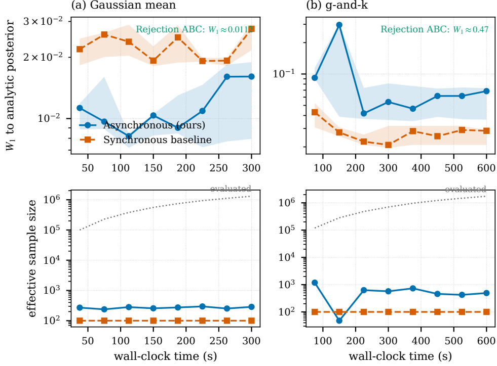
Fig. 4 What the reported estimator recovers, and with how many effective particles. Each method is scored on the posterior it reports (§5.3) against the analytic posterior (a) and the g-and-k reference posterior (b). Top: W_1 , median and inter-quartile range over five replicates. Bottom: the effective sample size of the reported posterior, with the evaluated-particle count dotted; the history grows by more than an order of magnitude and the effective sample does not follow it.
