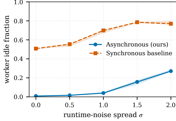
Fig. F2 Worker utilization loss under runtime heterogeneity: the fraction of worker wall-clock spent idle versus the runtime-noise spread \sigma (five replicates; bands are inter-quartile ranges). The synchronous baseline idles at generation barriers (its idle fraction rises from \approx 0.51 to \approx 0.79 as heterogeneity grows) while the asynchronous method stays near-fully utilized (idle fraction \approx 0.01 rising to \approx 0.27 ).
