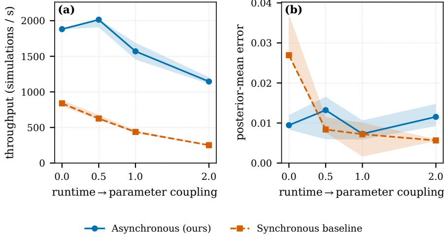
Fig. F5 Parameter-coupled runtime on the Gaussian-mean benchmark (analytic posterior; 48 workers, 60 s budget, five replicates; bands are inter-quartile ranges). The post-evaluation delay grows with the inferred mean, so one region of parameter space is sampled far more often than its mirror image. (a) Aggregate throughput falls as the coupling steepens (monotonically for the barrier-bound baseline, and from a peak at c = 0.5 for the asynchronous method), consistent with the fast region dominating the raw sample counts. (b) Posterior-mean error to the analytic posterior nonetheless does not increase with coupling and stays comparable between the asynchronous method and the discard-latecomers synchronous baseline, so the over-representation does not measurably distort the reported posterior at these coupling levels.
