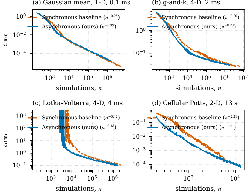
Fig. F4 Tolerance against simulations spent, \epsilon_{(100)}(n) , asynchronous against the matched synchronous baseline on every benchmark (medians and replicate range over five replicates; the slope over the last decade of n in the legend). The vertical gap at equal n is the per-simulation efficiency, the horizontal extent is what the wall clock bought. On Lotka–Volterra 98% of simulations return the extinction fallback, so \epsilon_{(100)} sits on that plateau until about 5000 draws have produced 100 survivors; the plateau is cut off.
