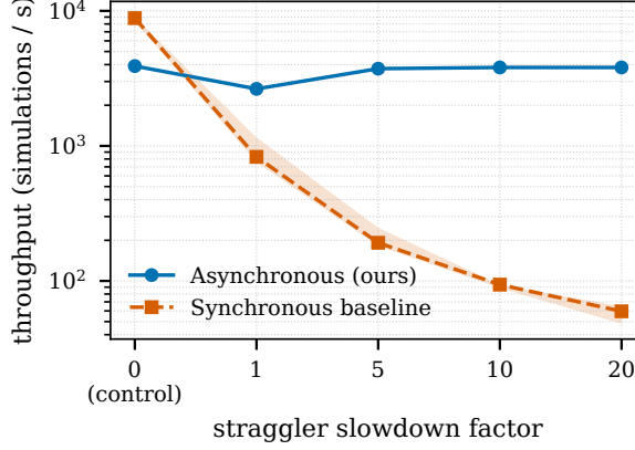
Fig. F1 Throughput (median and inter-quartile range over five replicates) against straggler slowdown on the Gaussian-mean benchmark, 300 s wall-limited campaign; one of 16 workers carries a permanent post-evaluation delay of 0.1 s scaled by the factor. The synchronous baseline falls from \approx 8800 to \approx 60 simulations per second because every generation waits for it; the asynchronous method holds \approx 2600 – 3900 , and the twin campaign’s asynchronous arm (Table 2) agrees within 15% except at 1\times . Logarithmic throughput axis.
