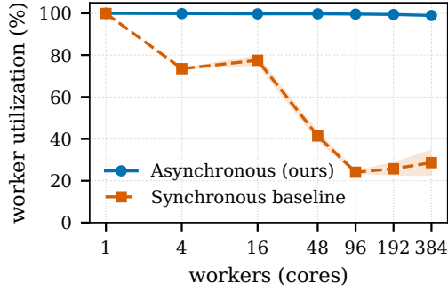
Fig. F8 Cellular Potts 50^3 worker utilization in the benchmark’s earlier single-simulation configuration (fraction of worker wall-clock spent inside the simulator) versus worker count (1800 s budget; error bars are \pm 1 s.d.); the synchronous baseline uses a population equal to the worker count (Fig. 2, right). The asynchronous method stays \approx 98.9 – 99.8\% utilized at every scale. The synchronous baseline fills every core within a generation but then idles at the barrier waiting for the slowest simulation, so its utilization falls to \approx 24 – 29\% ( 41\% \rightarrow 24\% \rightarrow 26\% \rightarrow 29\% at 48/96/192/384 workers, i.e. \approx 70 – 76\% idle at every multi-node scale). The figure is the measured utilization behind the synchronous method’s sub-linear scaling in Fig. 2 (right).
