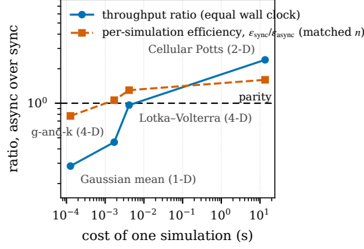
Fig. 3 Throughput ratio and per-simulation efficiency of the asynchronous method over the matched synchronous baseline, against the cost of one simulation, one point per benchmark (Table 3). Both rise with the cost; throughput parity is reached at about 4 ms per simulation at these budgets and this placement (§6.3).
