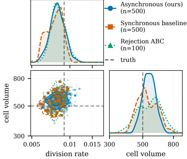
Fig. 5 Cellular Potts posterior (division rate, cell volume) on the fixed production run, replicate 0: the asynchronous AMIS estimator (500 resampled draws), the synchronous baseline’s last completed generation with pyABC’s weights (500 resampled draws), and the 100 best rejection draws (Table 5). Axes are the log-uniform prior coordinates ticked in physical units; dashed lines mark the truth. Every method recovers the division rate; the asynchronous estimator is the tightest on the cell volume.
