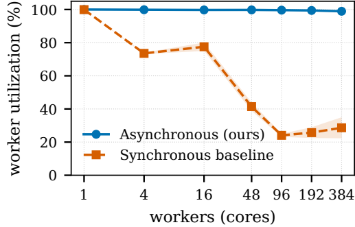
Fig. 11 Cellular Potts worker utilization (fraction of worker wall-clock spent inside the simulator) versus worker count (1800s budget; error bars are \pm 1 s.d.); the synchronous baseline uses a population equal to the worker count (Fig. 5, right). The asynchronous method stays \approx 98.9 – 99.8\% utilized at every scale, while the synchronous baseline, even filling every core within a generation, then idles at the barrier waiting for the slowest simulation, so its utilization falls to \approx 24 – 29\% ( 41\% \rightarrow 24\% \rightarrow 26\% \rightarrow 29\% at 48/96/192/384 workers, i.e. \approx 70 – 76\% idle at every multi-node scale). This barrier idle is the measured mechanism behind the synchronous method’s sub-linear scaling in Fig. 5 (right).
