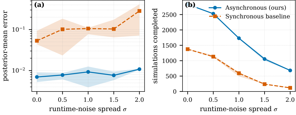
Fig. 5 Inference per unit wall clock under runtime heterogeneity (Gaussian mean, analytic posterior, 48 workers, 60s budget, five replicates; bands are inter-quartile ranges). Left: error of the archive mean (the unweighted top- k archive, not the reported estimator; §7.1) to the analytic posterior mean, against the runtime spread \sigma . Right: simulations completed within the budget. The barrier starves the synchronous baseline as \sigma grows; the asynchronous method’s error stays flat.
