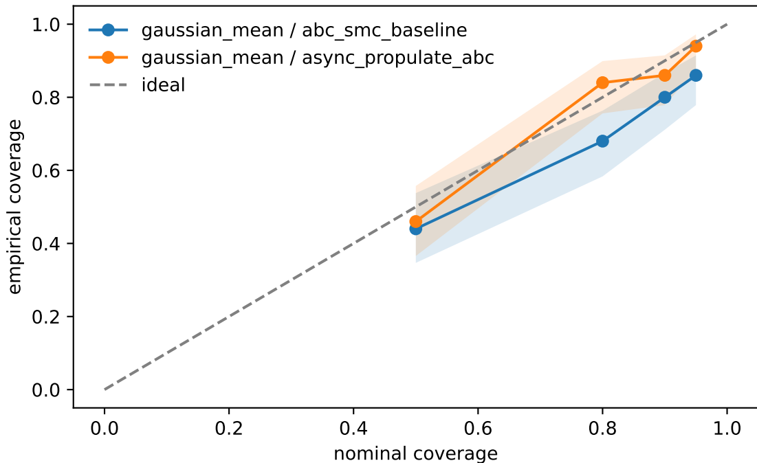
SBC empirical coverage
