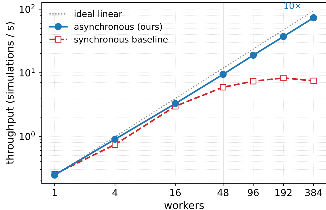
Realistic workload strong scaling ( k = 100 )
