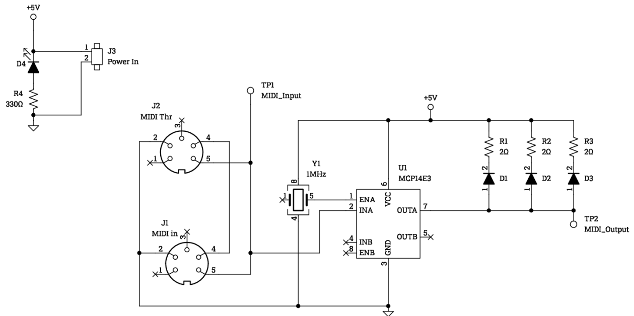
Figure One – MIDI IR Tx Rev B
