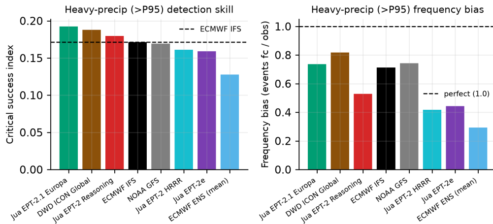
Figure S7: Detection of heavy precipitation ( y \geq P95 ) on Track A over 1–48 h. Left: critical success index, with ECMWF IFS shown by the dashed line. Right: frequency bias, with unity denoting the correct event frequency. All models underpredict the frequency of heavy precipitation.
