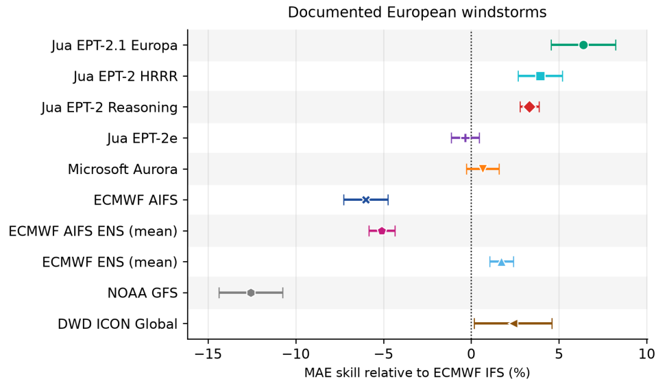
Figure S17: As Figure S16, for the seven externally documented European windstorms. Every model is evaluated on the same eight leads and 123,847 station/valid-time/lead samples.
