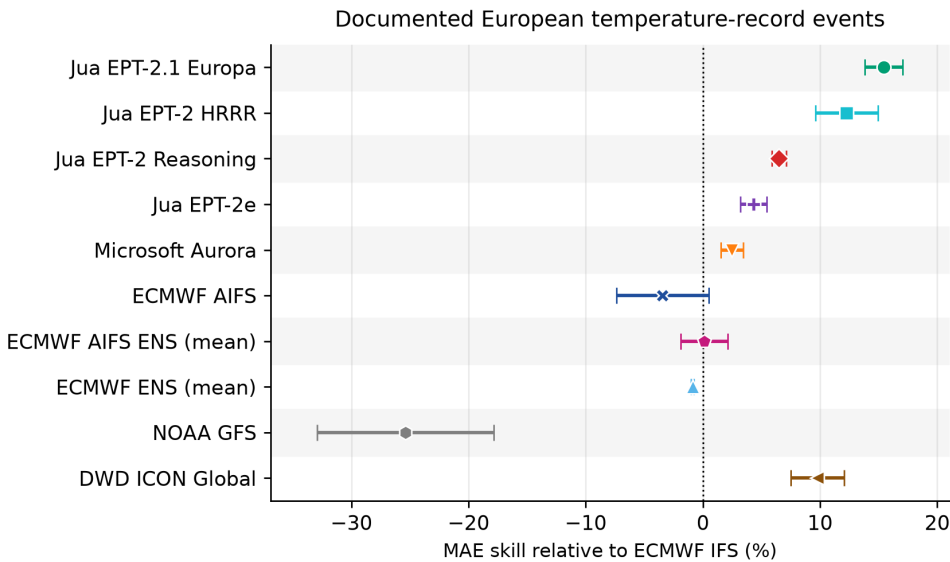
Figure S16: MAE skill relative to ECMWF IFS over the source-defined record-temperature event footprints, aggregated over 6–48 h after bias correction. Every model is evaluated on the same five events, eight leads, and 231,065 station/valid-time/lead samples. Error bars show one leave-one-event-out jackknife SE.
