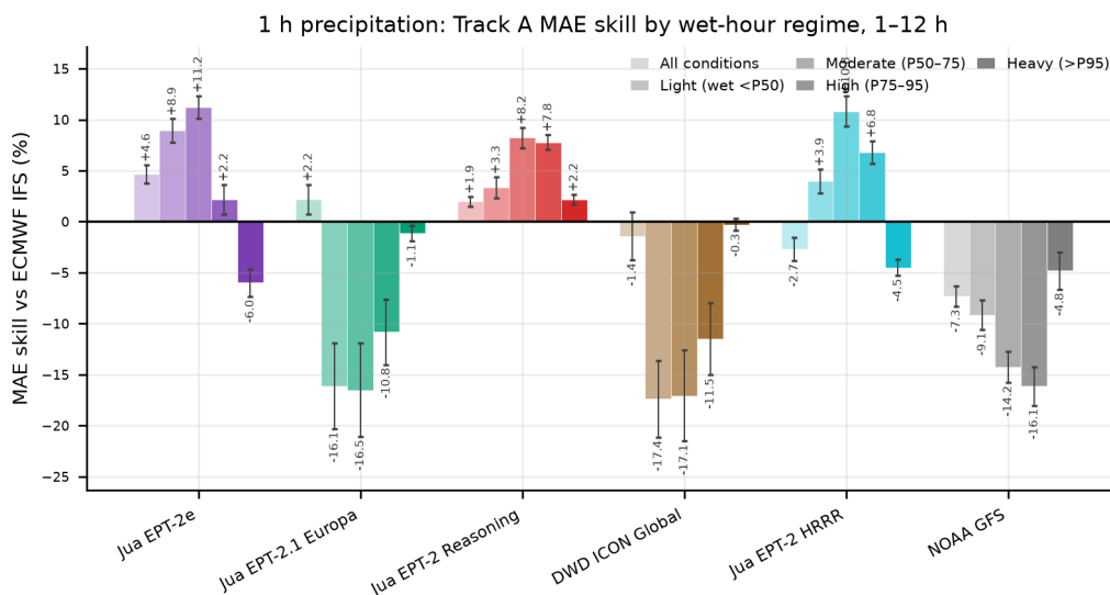
Figure S6: Track A MAE skill relative to ECMWF IFS for precipitation by observed-value regime over 1–12 h, with \pm 1 jackknife SE
