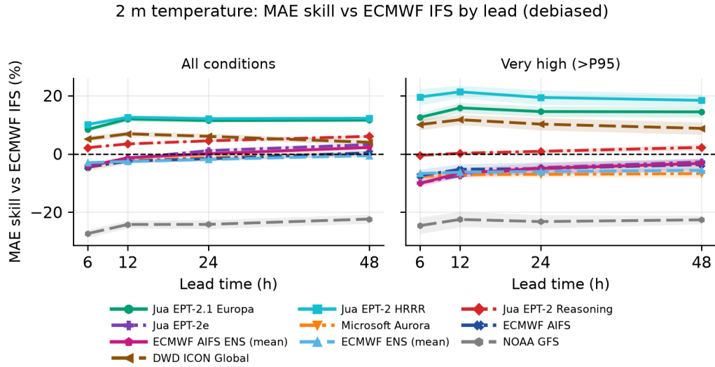
Figure S2: Track A MAE skill relative to ECMWF IFS by lead time for 2 m temperature. The left panel shows all conditions; the right panel shows the heat regime, y \geq P95 . Shading denotes \pm 1 jackknife SE.
