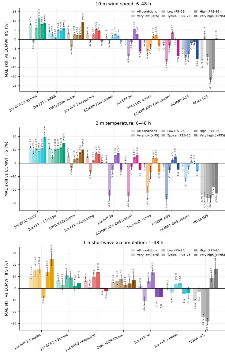
Figure 1: Track A MAE skill relative to ECMWF IFS by observed-value regime, with ±1 jackknife SE. Wind and temperature use 6–48 h leads; solar radiation uses 1–48 h.
