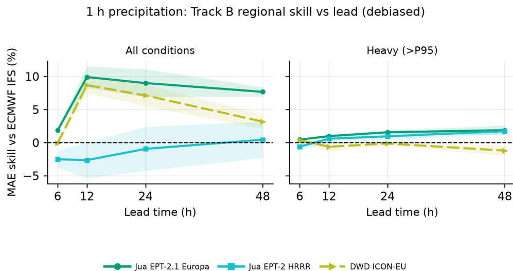
Figure S13: Track B precipitation skill relative to ECMWF IFS by lead time. The left panel shows all conditions; the right panel shows the heavy regime, y \geq P95 . Shading denotes \pm 1 jackknife SE.
