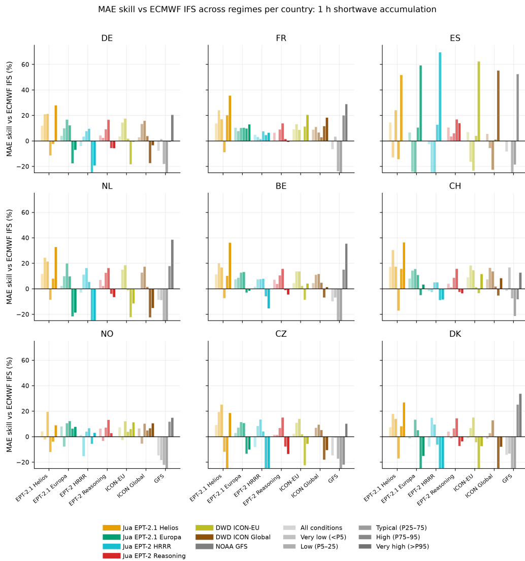
Figure S16: As Figure S14, for 1 h shortwave, with EPT-2.1 Helios added. GB, IT and PL have no solar station observations (Section 2.2).
