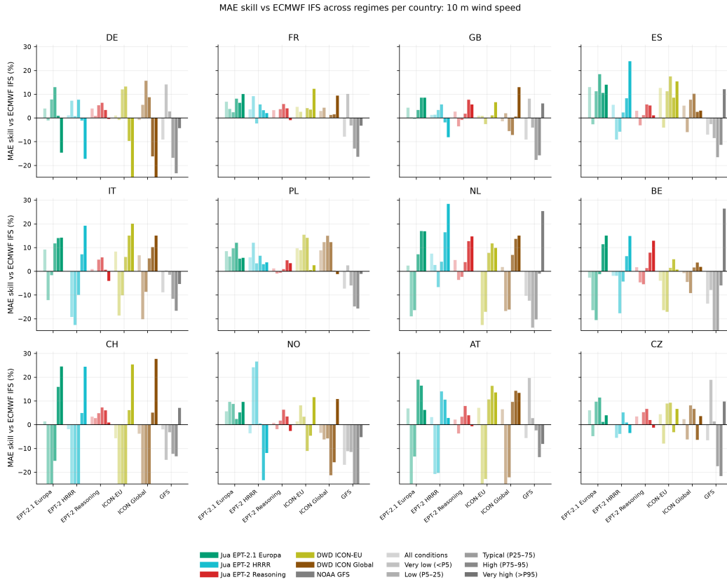
Figure S14: Per-country MAE skill by ERA5 1991–2020 climatological regime, 10 m wind, March–June 2026, pooled 1 to 48 h (hourly). Mixed regional/global model set.
