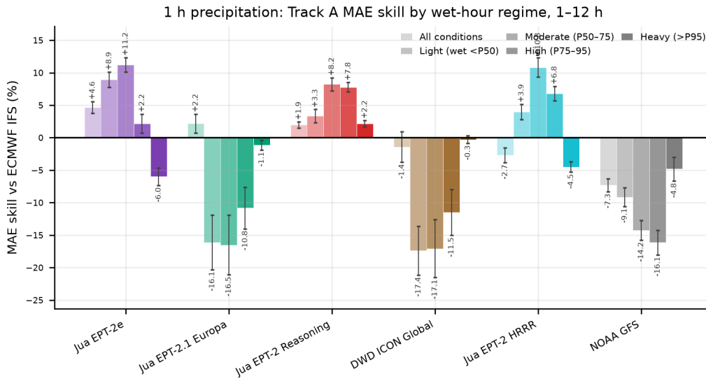
Figure S7: As Figure S6, restricted to the 1–12 h forecast range.
