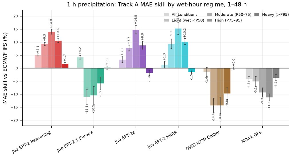
Figure S6: Track A MAE skill relative to ECMWF IFS for hourly precipitation by observed-value regime over 1–48 h, with \pm 1 jackknife SE.
