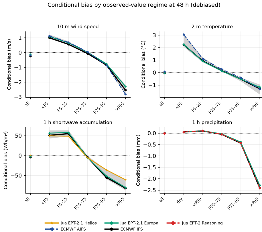
Figure 2: Mean forecast-minus-observation error at 48 h, conditioned on the observed-value regime after bias correction. The grey envelope spans all models; selected models are highlighted.
