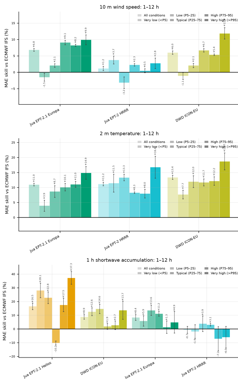
Figure S10: As Figure S9, restricted to the 1–12 h forecast range.
