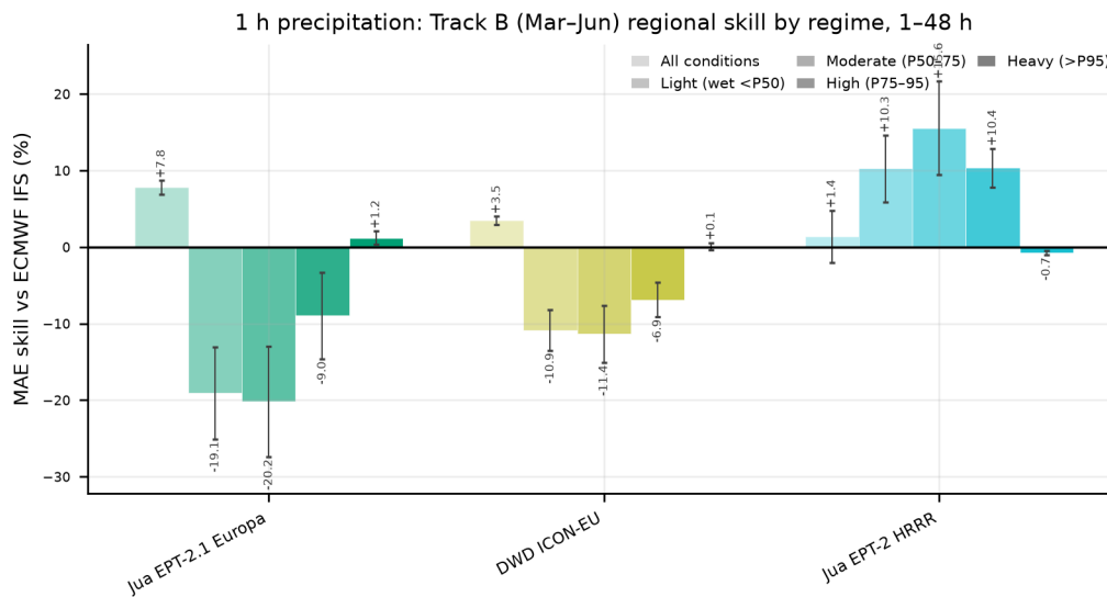
Figure S12: Track B MAE skill relative to ECMWF IFS for hourly precipitation by observed-value regime, aggregated over 1–48 h from March to June 2026, with \pm 1 jackknife SE.
