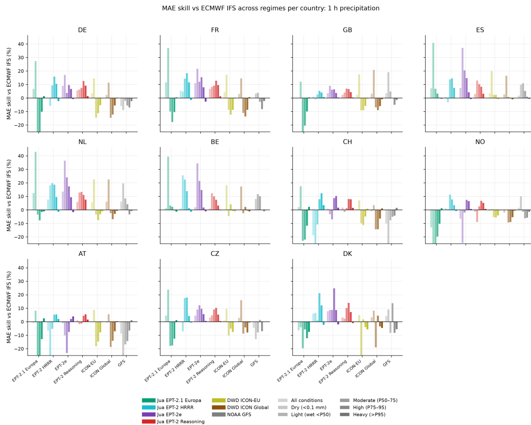
Figure S17: Per-country MAE skill by precipitation regime for the mixed regional/global model set. IT and PL have no gauges in the precipitation panel.
