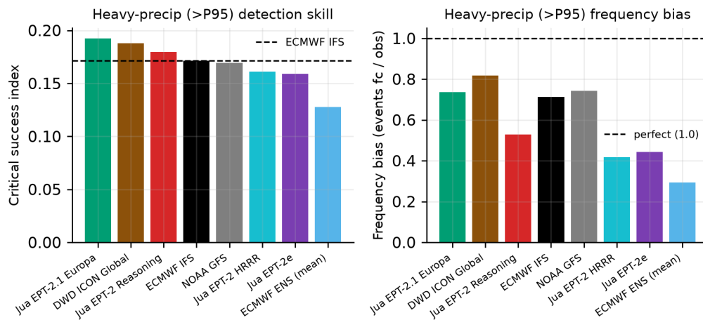
Figure S8: Detection of heavy precipitation ( y \geq P95 ) on Track A over 1–48 h. Left: critical success index, with ECMWF IFS shown by the dashed line. Right: frequency bias, with unity denoting the correct event frequency. All models underpredict the frequency of heavy precipitation.
