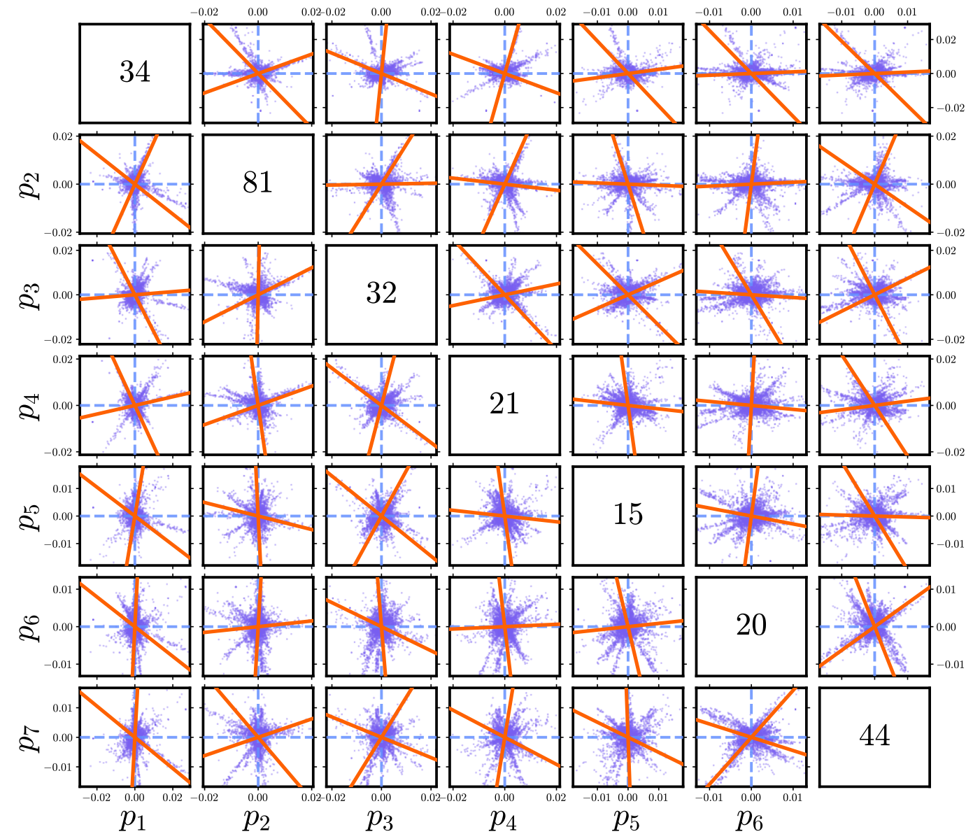
NYTimes PCA Factors: Global GFA Rotation
