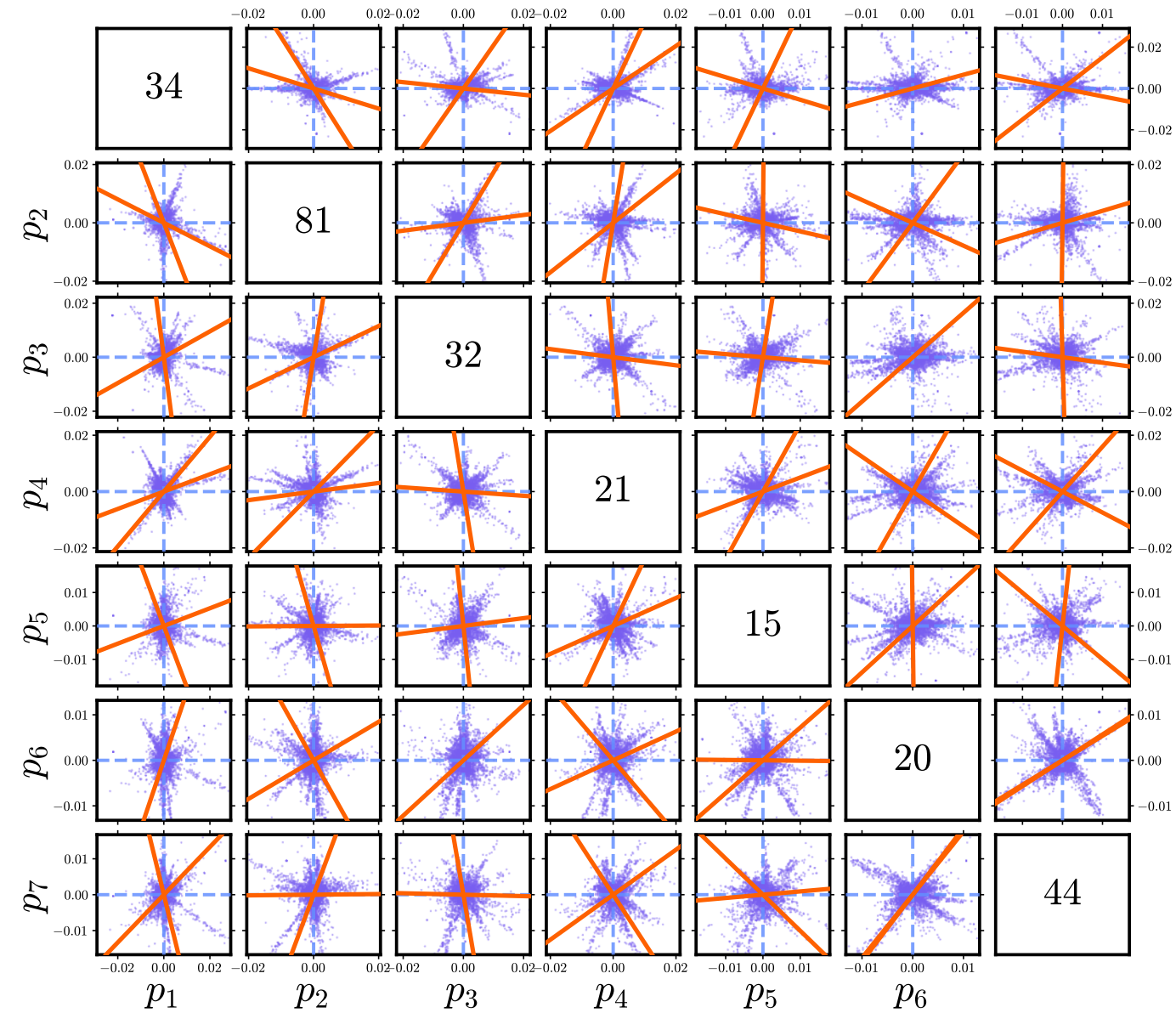
NYTimes PCA Factors: Global Varimax Rotation
