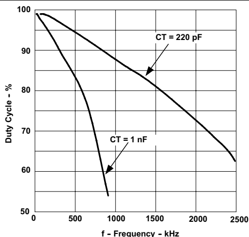
Figure 6-15. Maximum Duty Cycle vs Oscillator Frequency
