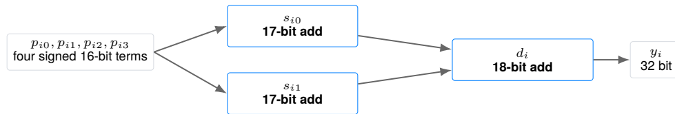
Optimized RTL · explicit balanced tree
