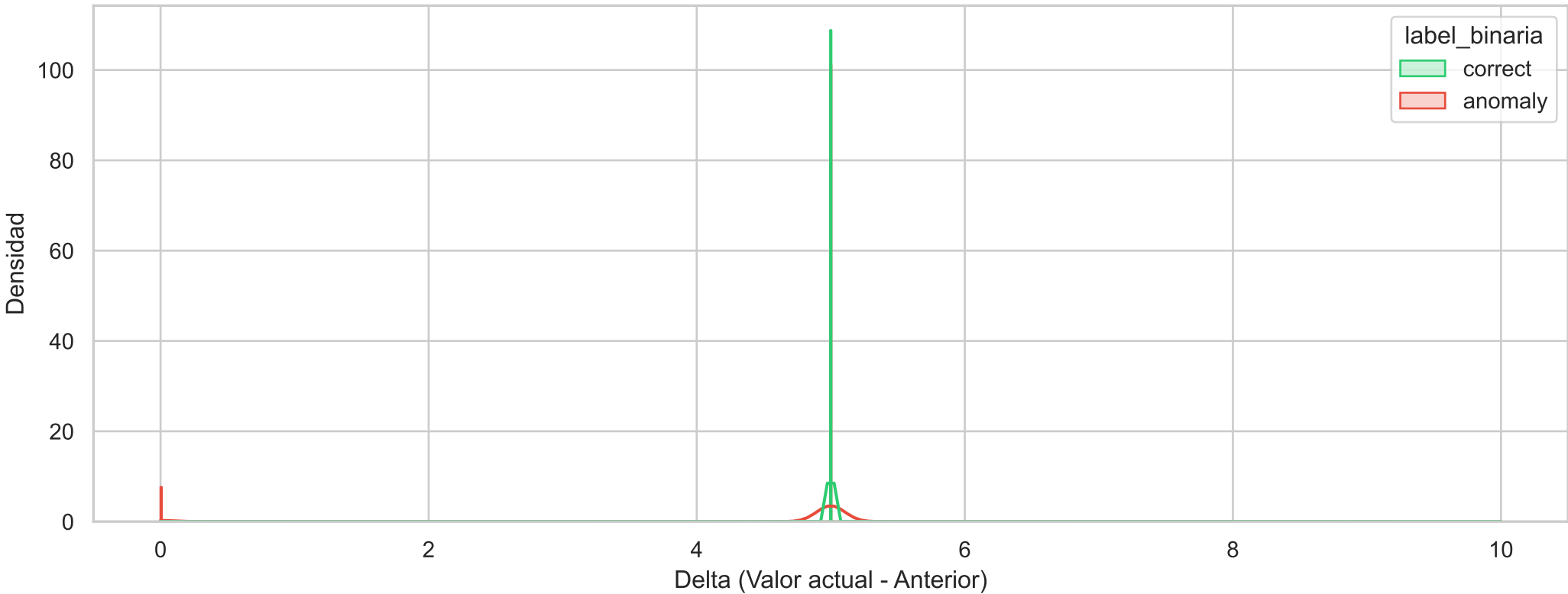
Histograma de Densidad Binario (prometheus_remote_storage_highest_timestamp_in_seconds_diff)
