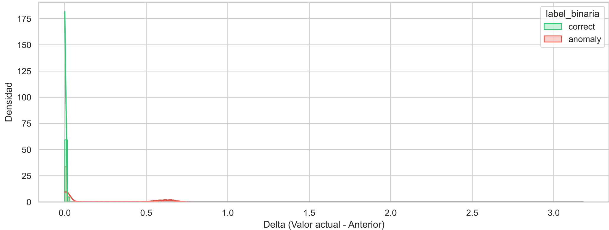
Histograma de Densidad Binario (process_cpu_seconds_total_diff)
