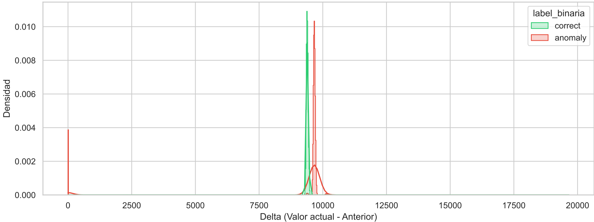
Histograma de Densidad Binario (prometheus_tsdb_wal_storage_size_bytes_diff)
