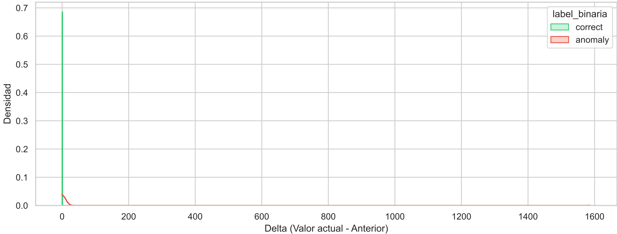
Histograma de Densidad Binario (prometheus_tsdb_mmap_chunks_total_diff)
