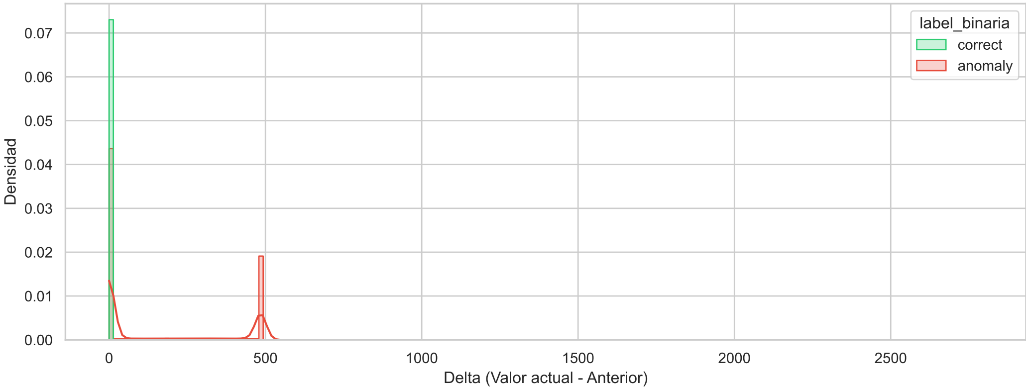
Histograma de Densidad Binario (prometheus_engine_query_duration_seconds_count_diff)
