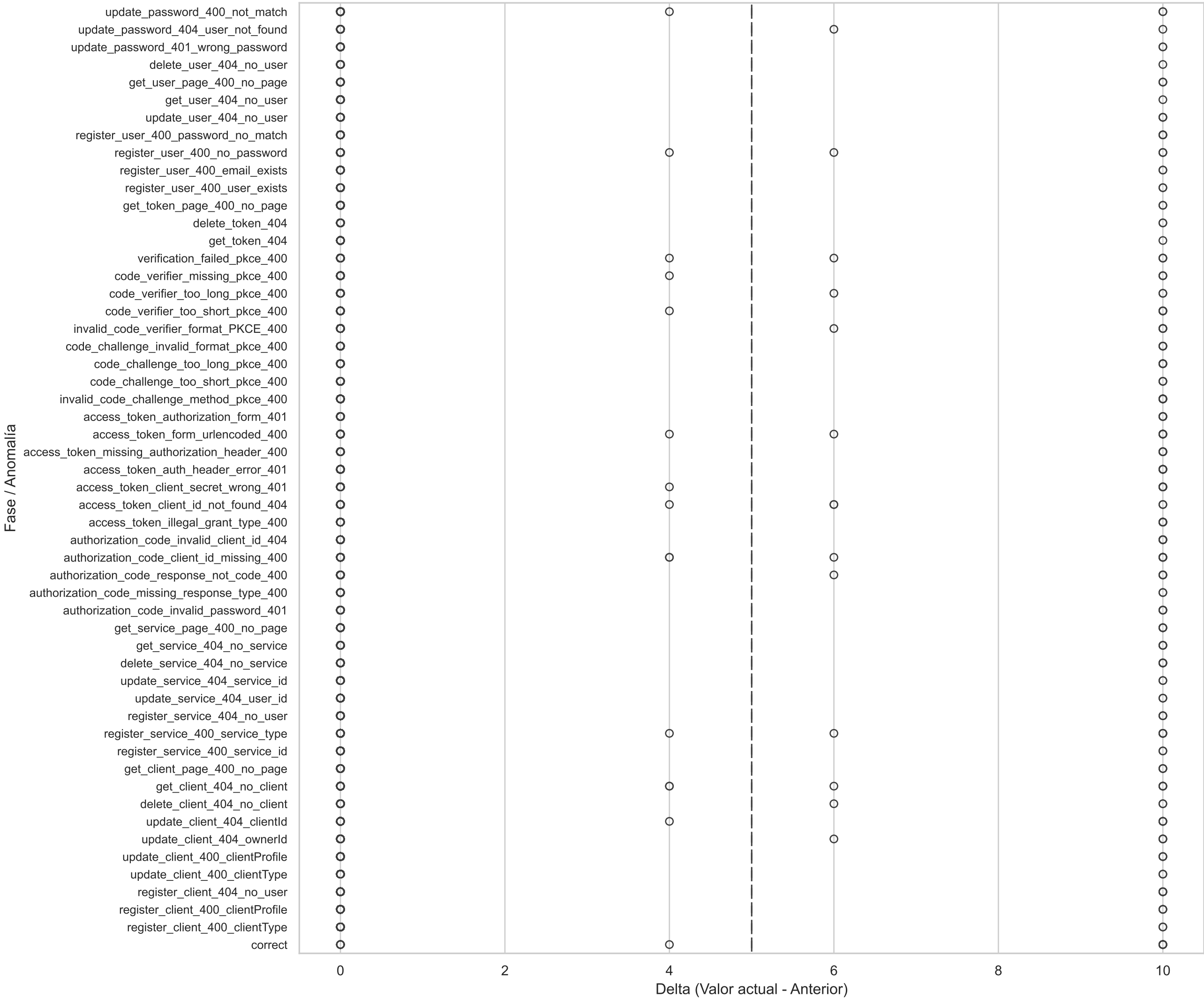
Boxplot Horizontal(prometheus_remote_storage_highest_timestamp_in_seconds_diff)
