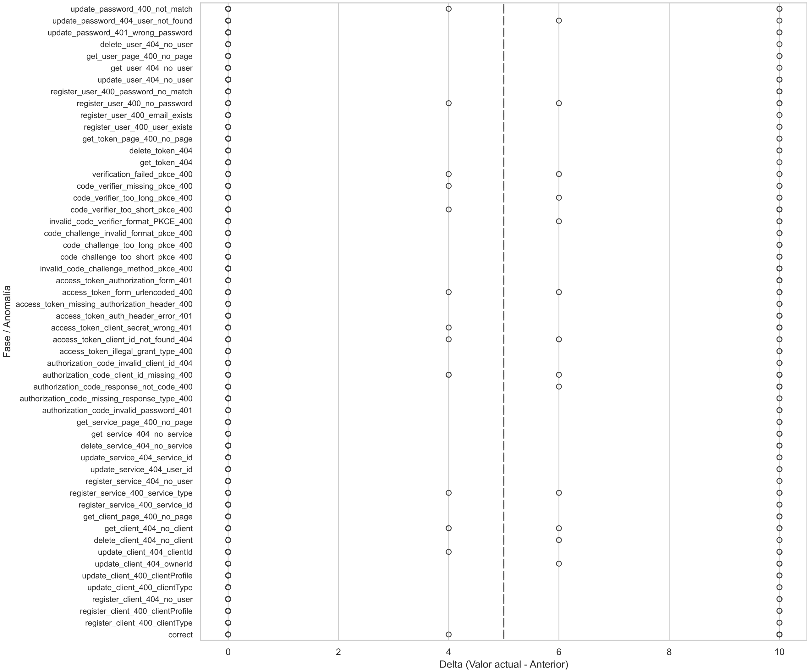
Boxplot Horizontal(prometheus_tsdb_head_max_time_seconds_diff)
