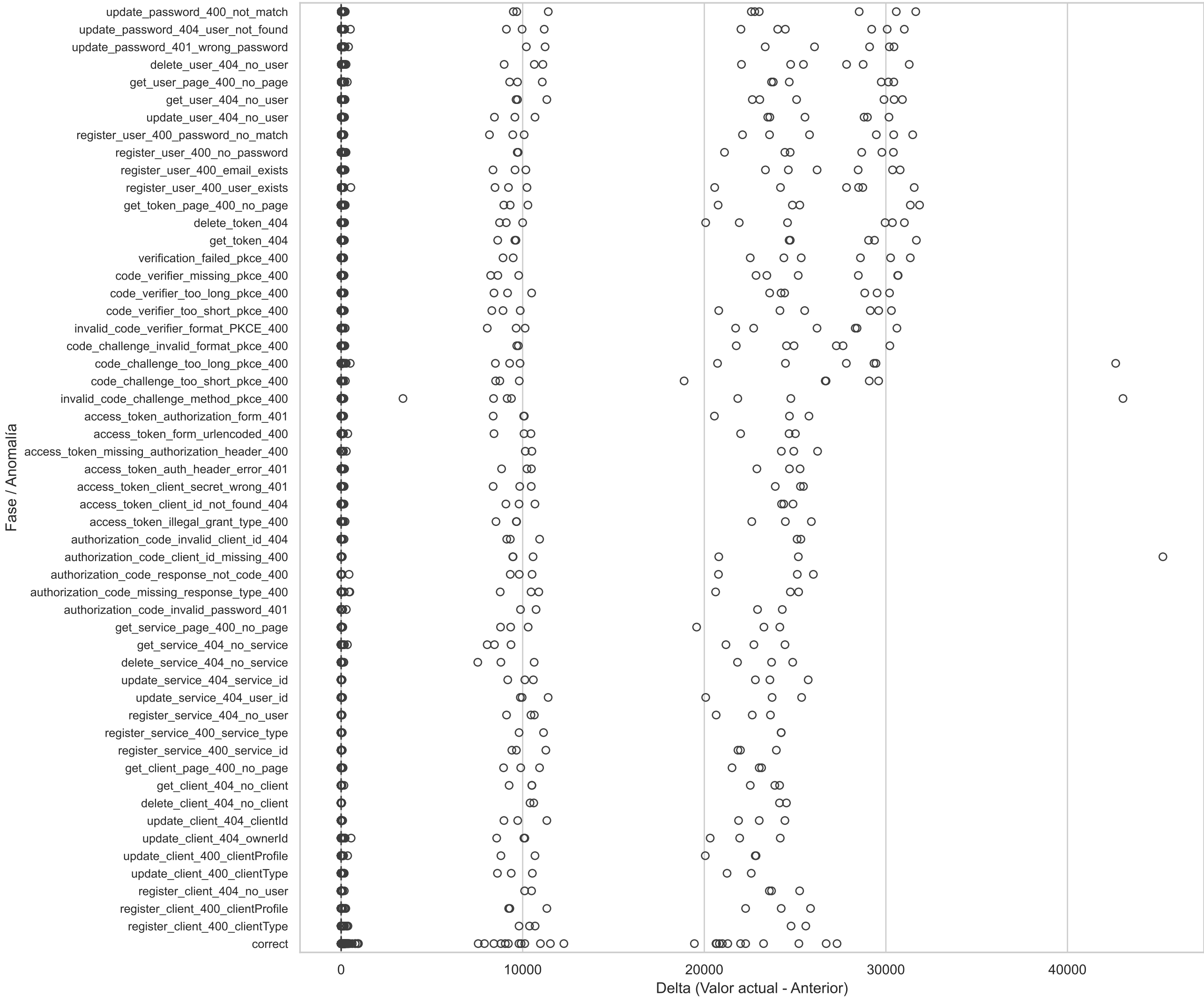
Boxplot Horizontal(node_vmstat_pgmajfault_diff)
