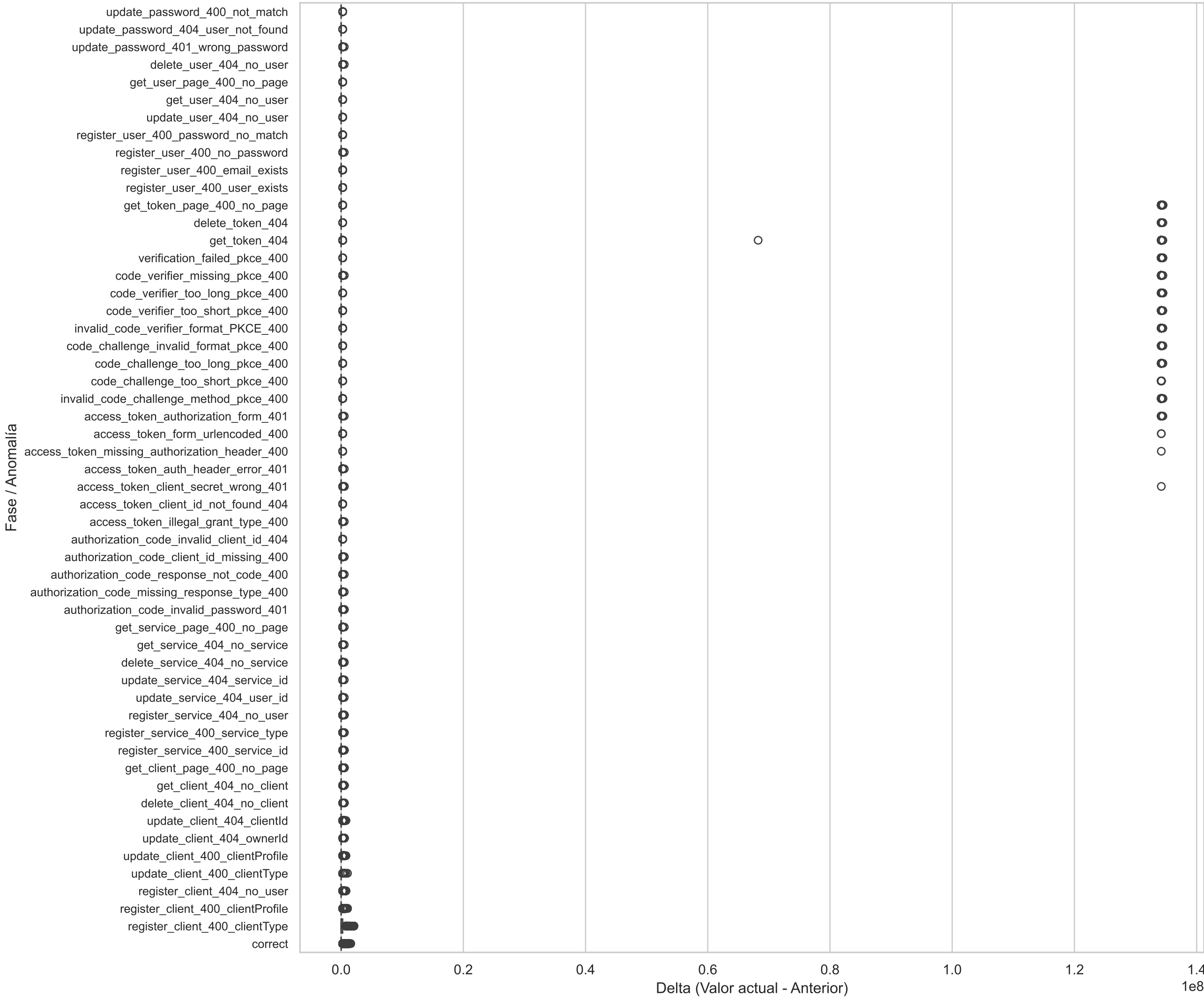
Boxplot Horizontal(process_virtual_memory_bytes_diff)
