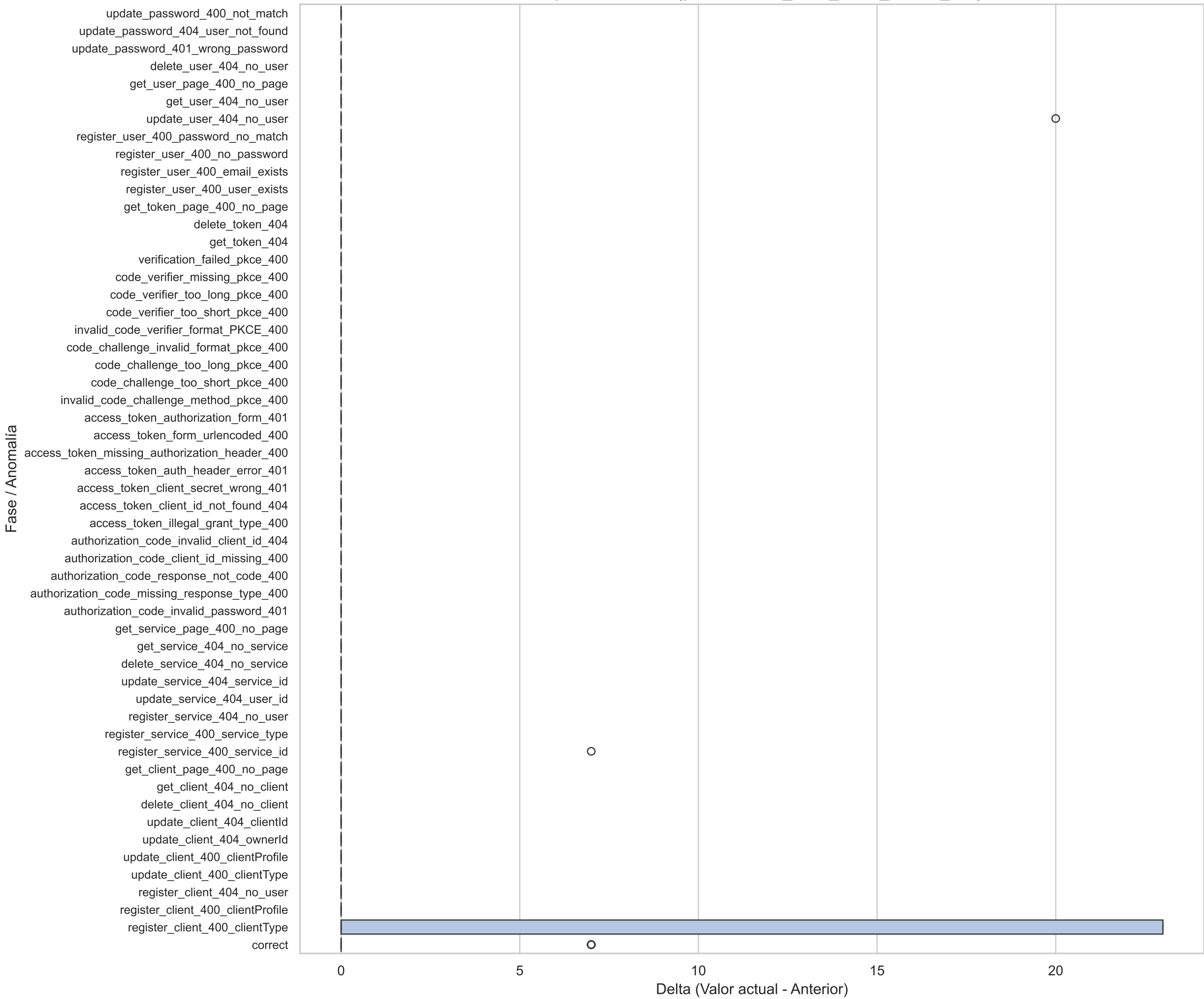
Boxplot Horizontal(prometheus_tsdb_head_series_diff)
