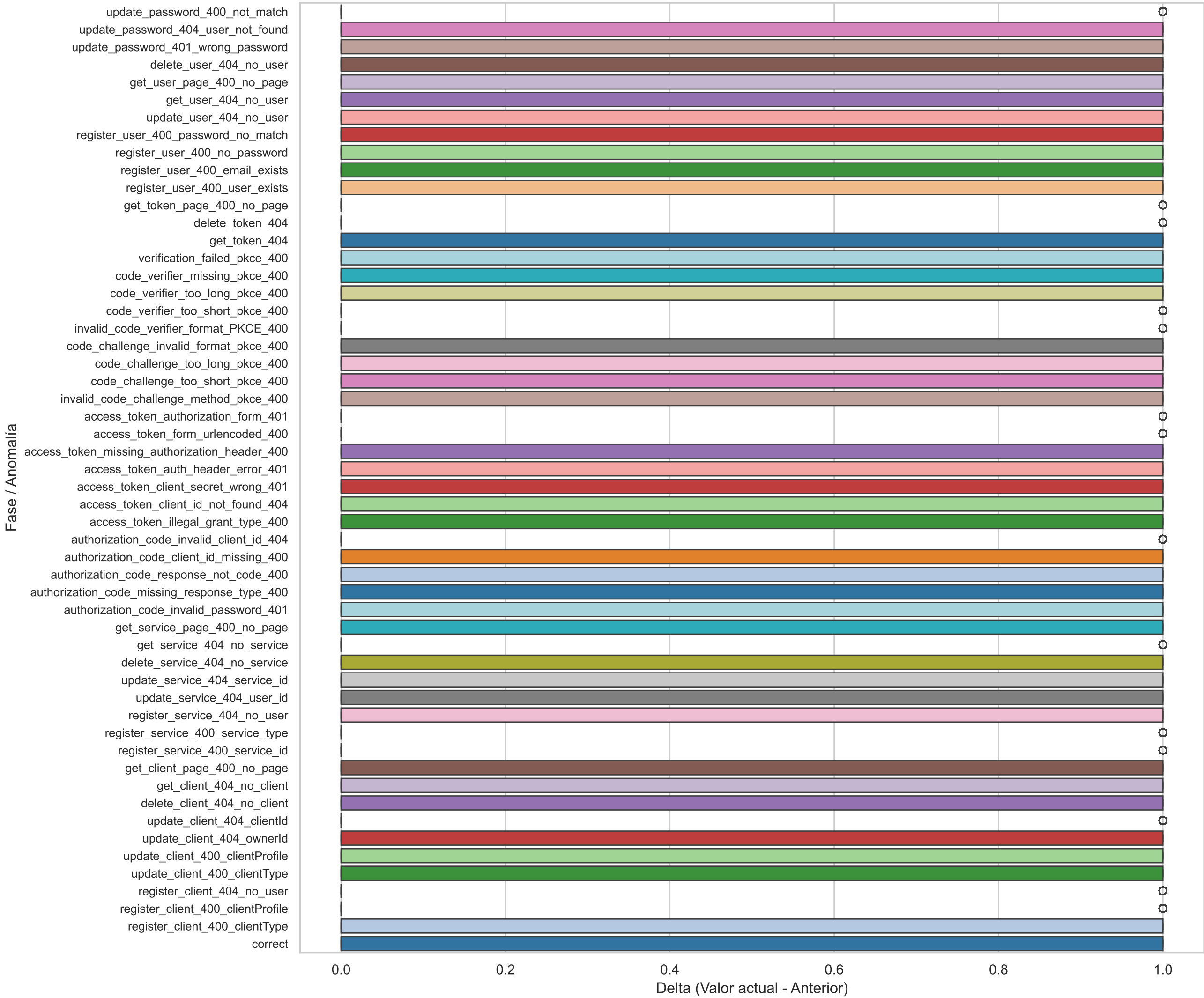
Boxplot Horizontal(prometheus_tsdb_wal_completed_pages_total_diff)
