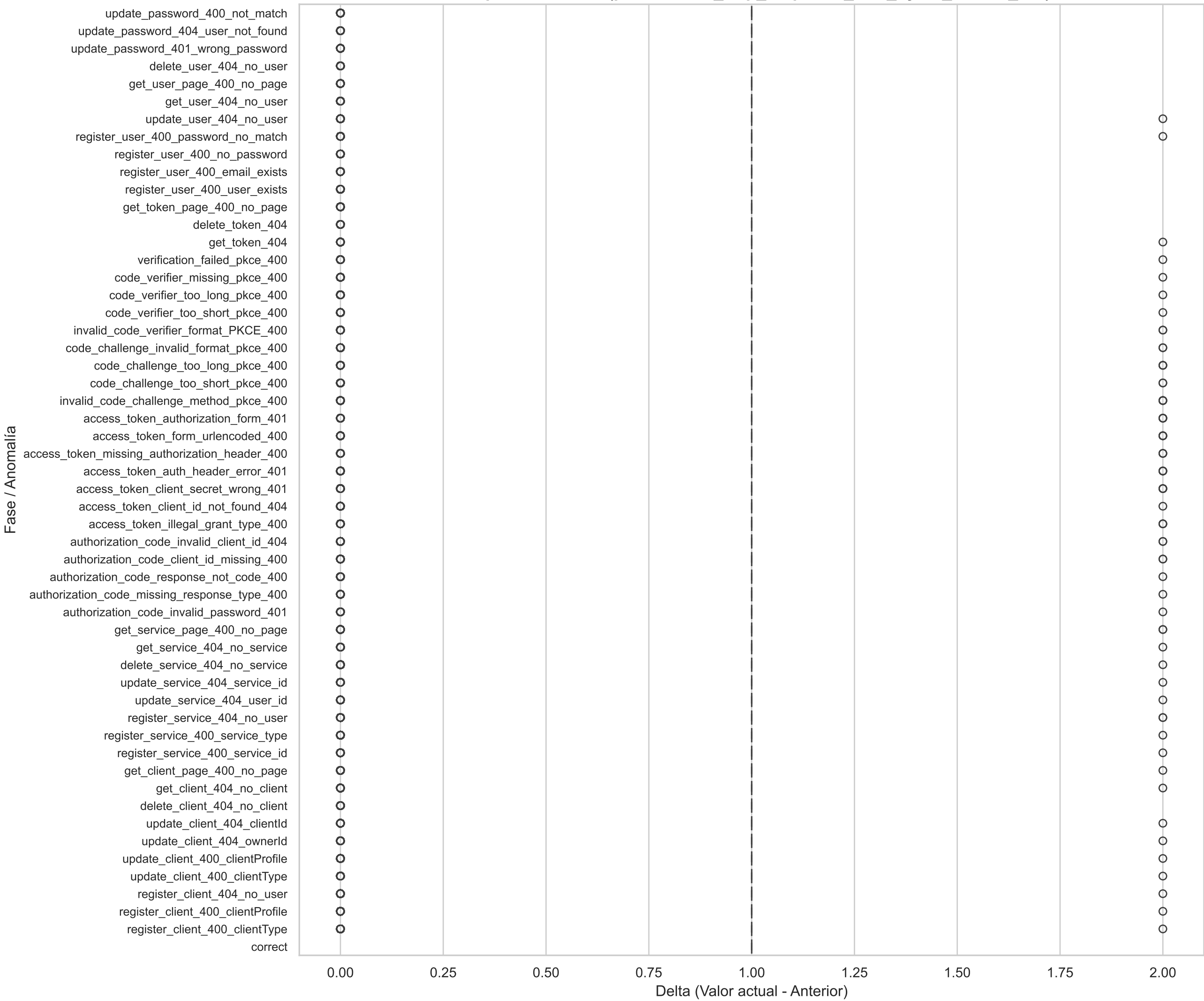
Boxplot Horizontal(prometheus_http_response_size_bytes_bucket_diff)
