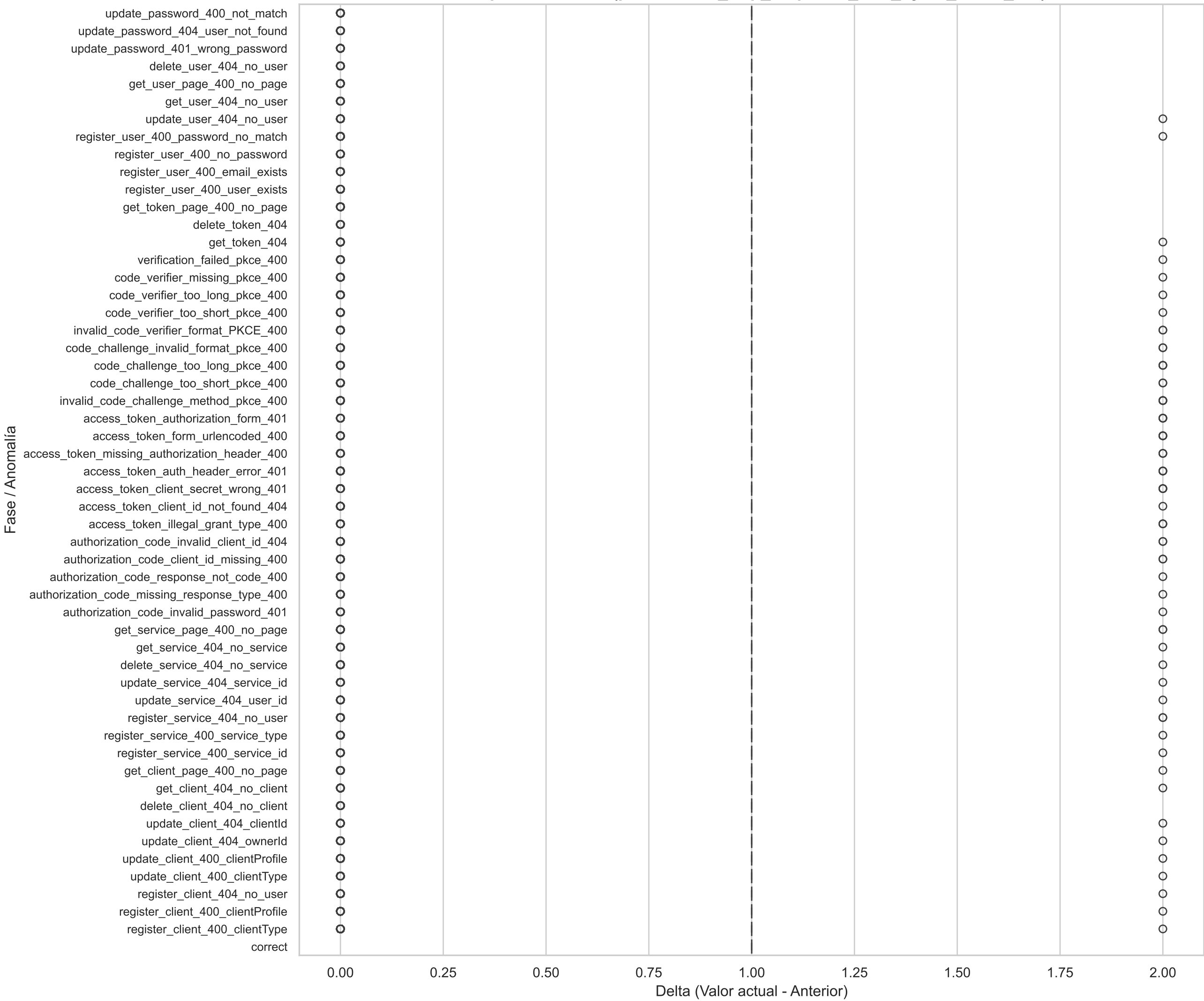
Boxplot Horizontal(prometheus_http_response_size_bytes_count_diff)
