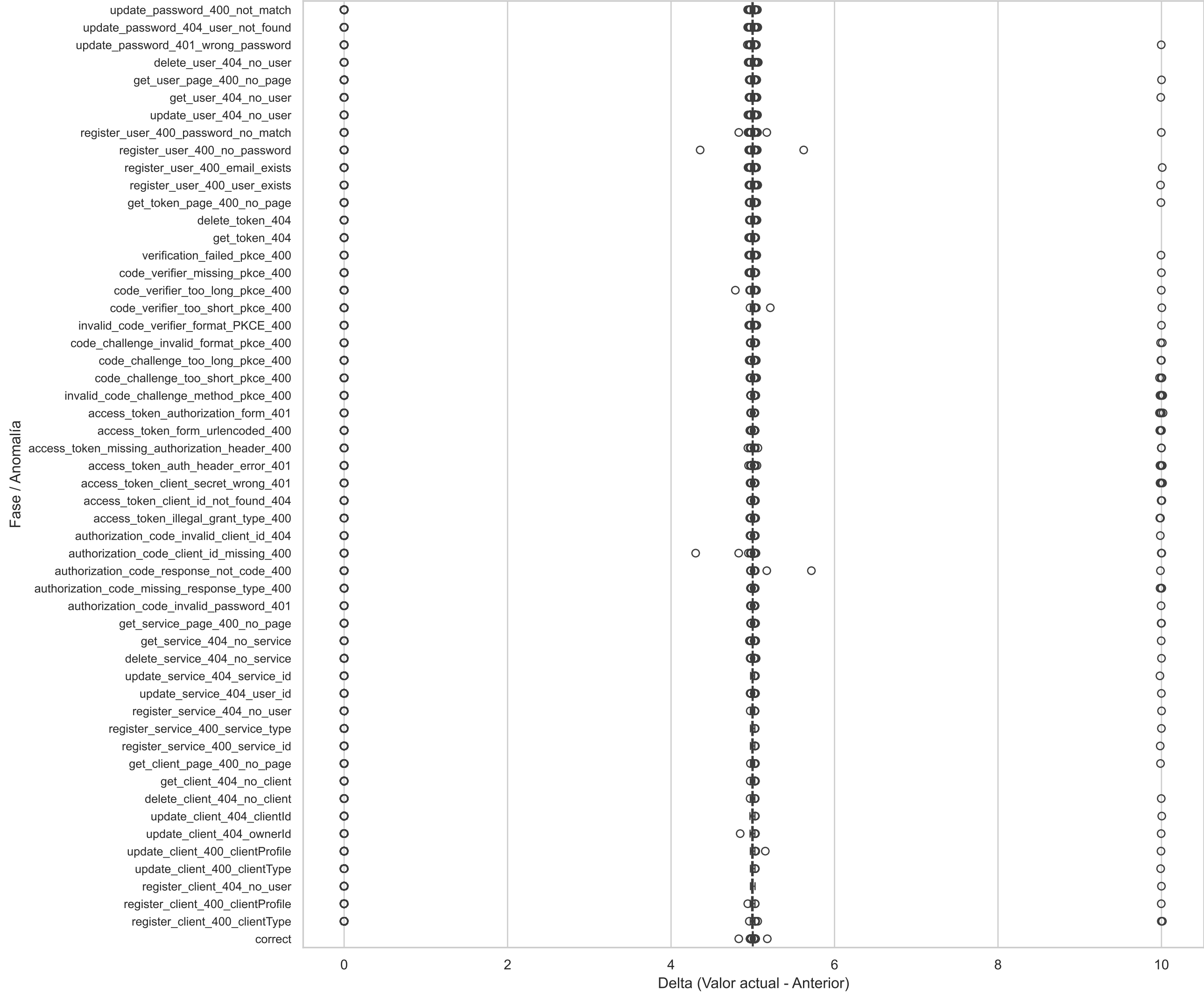
Boxplot Horizontal(node_time_seconds_diff)
