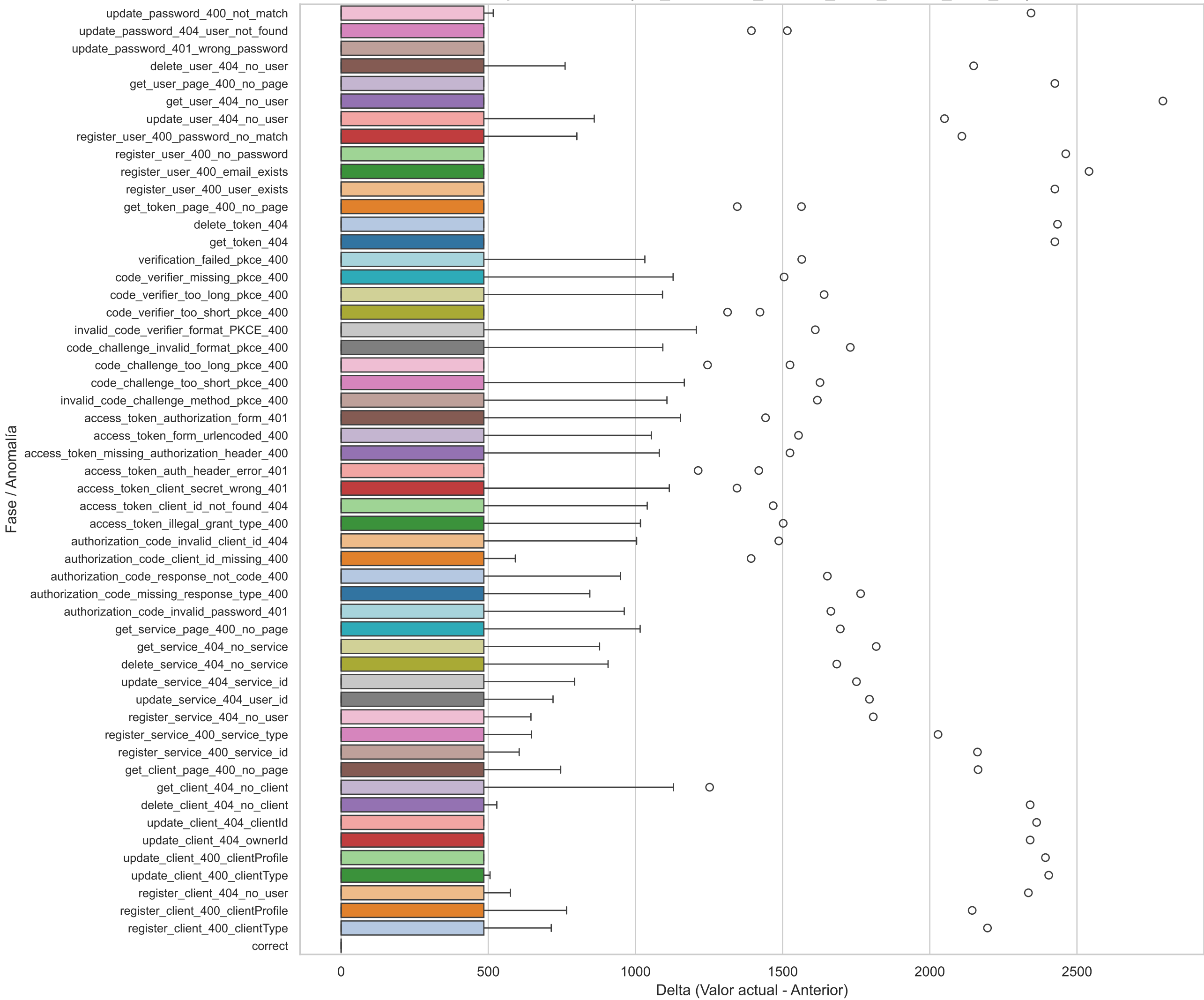
Boxplot Horizontal(net_contrack_listener_conn_closed_total_diff)
