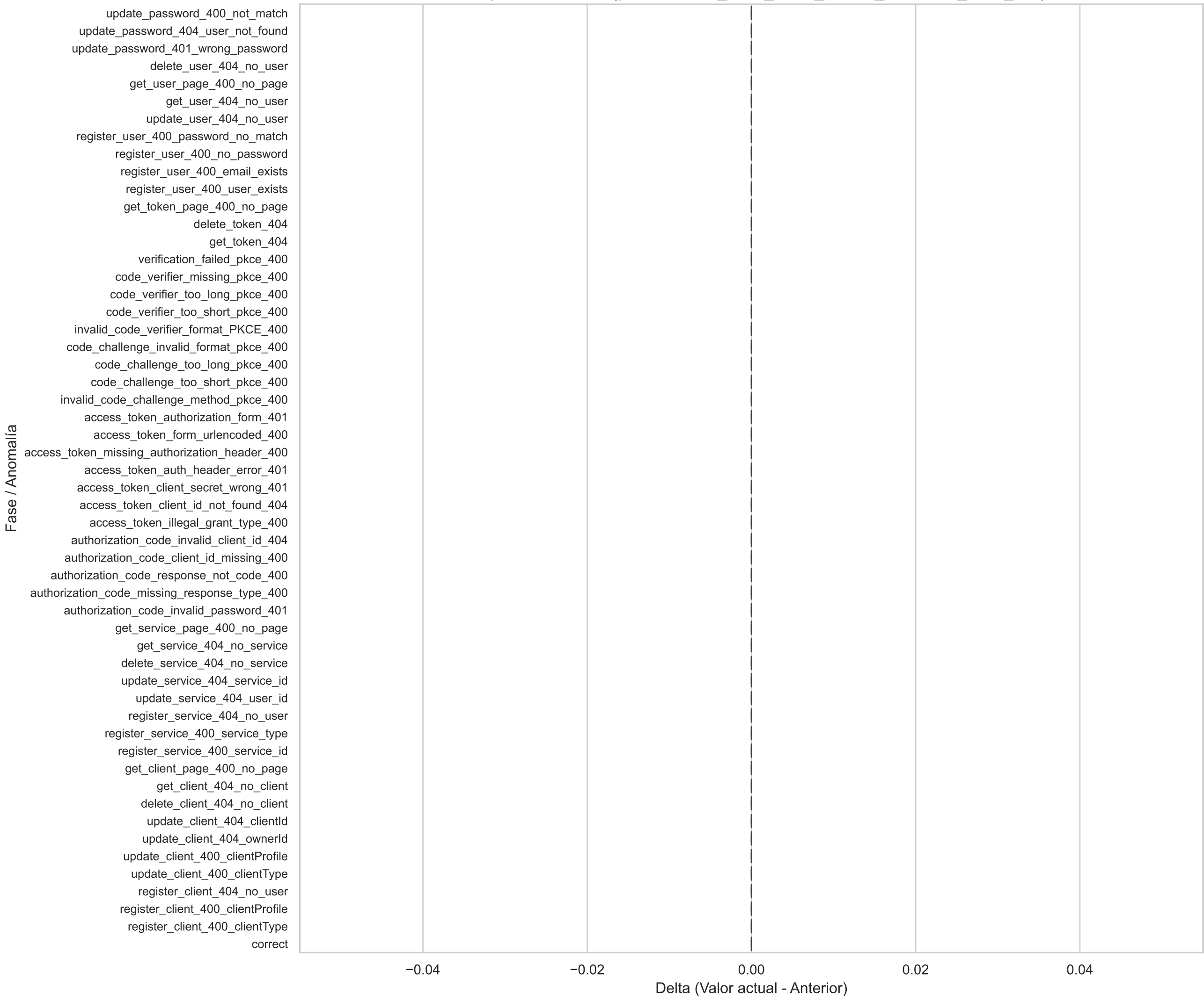
Boxplot Horizontal(prometheus_tsdb_head_series_removed_total_diff)
