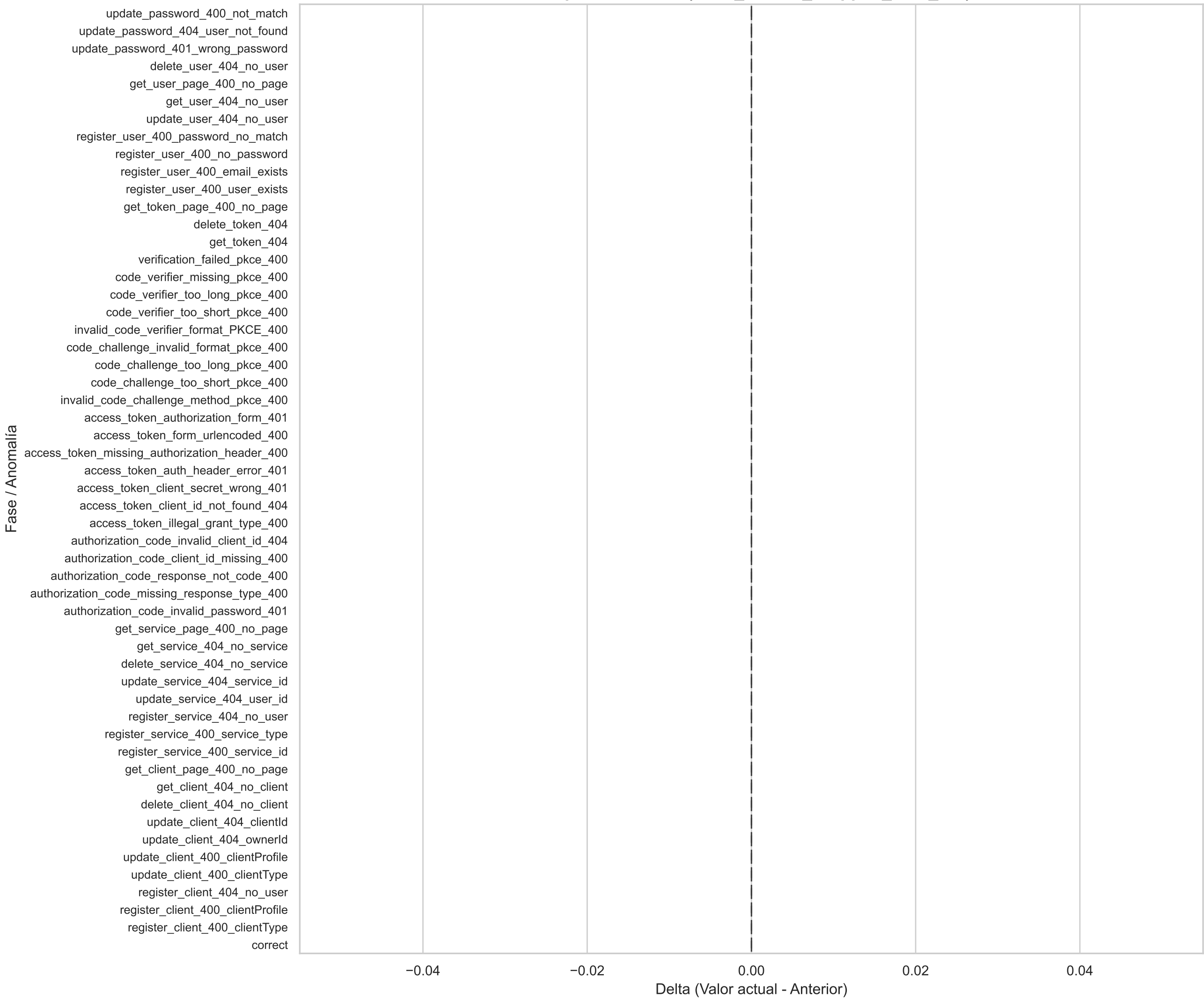
Boxplot Horizontal(node_softnet_dropped_total_diff)
