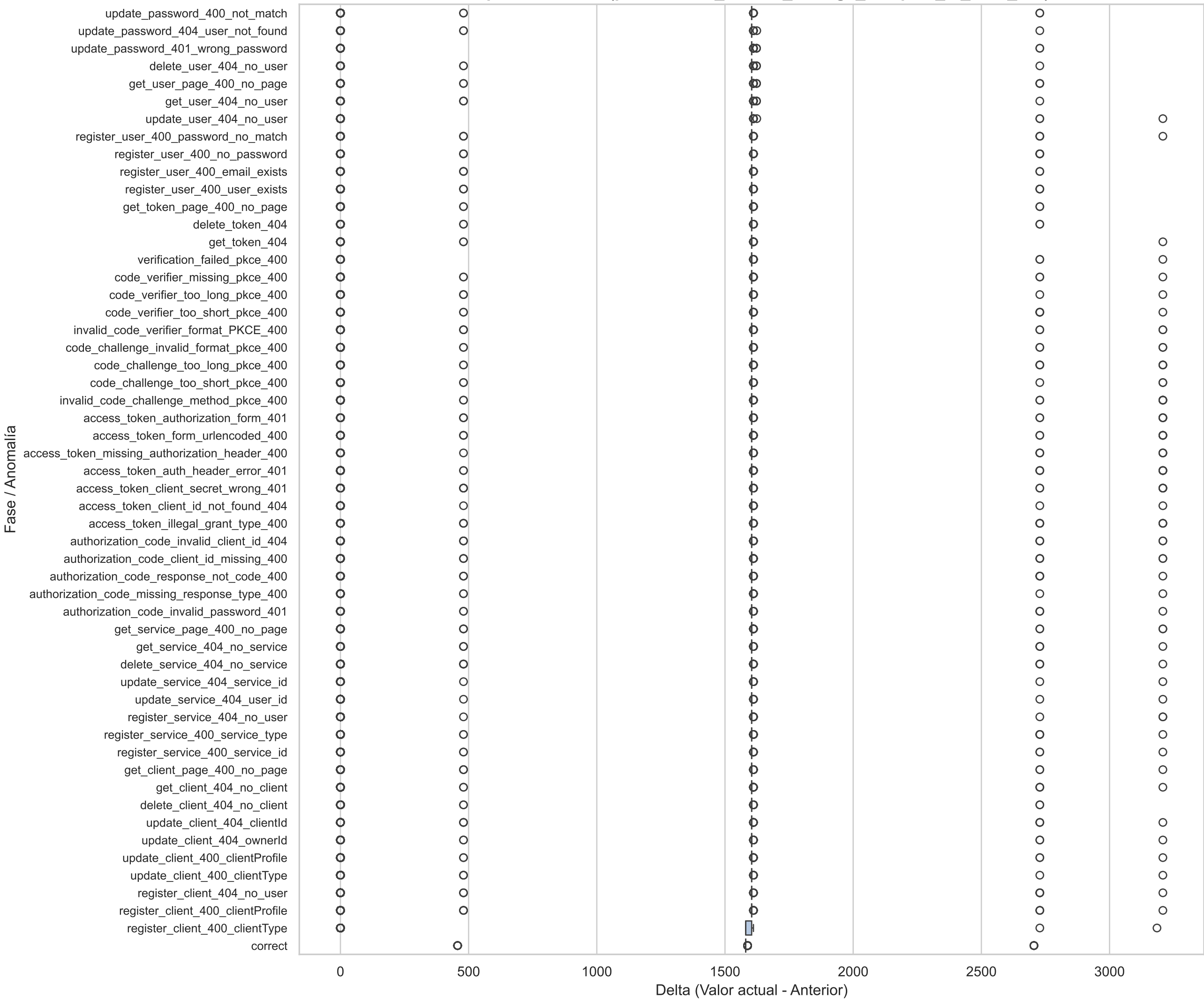
Boxplot Horizontal(prometheus_remote_storage_samples_in_total_diff)
