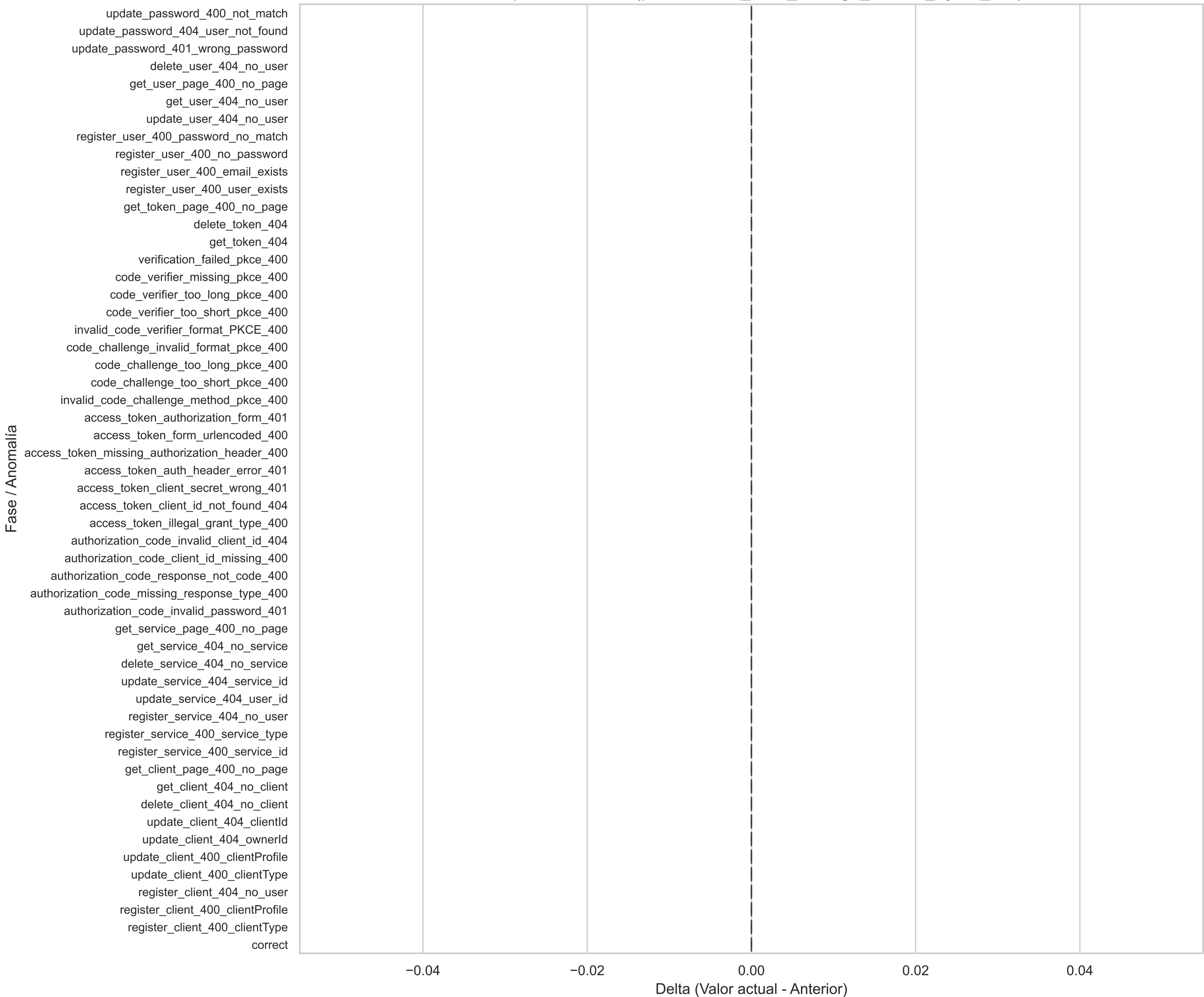
Boxplot Horizontal(prometheus_tsdb_storage_blocks_bytes_diff)
