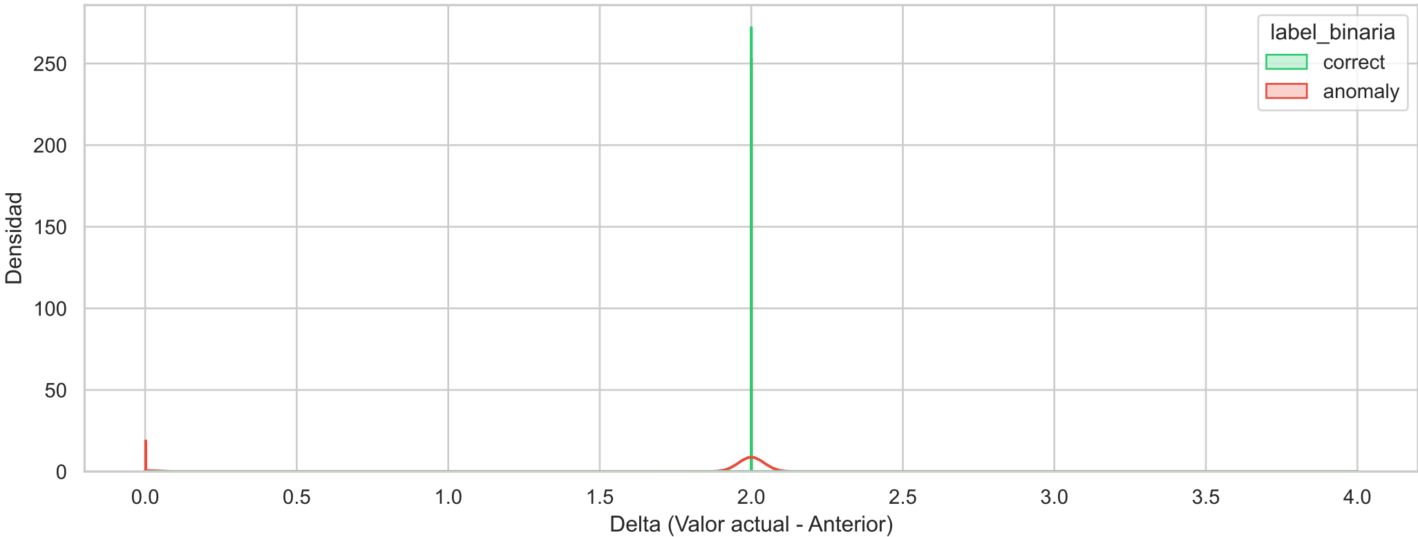
Histograma de Densidad Binario (prometheus_tsdb_isolation_high_watermark_diff)
