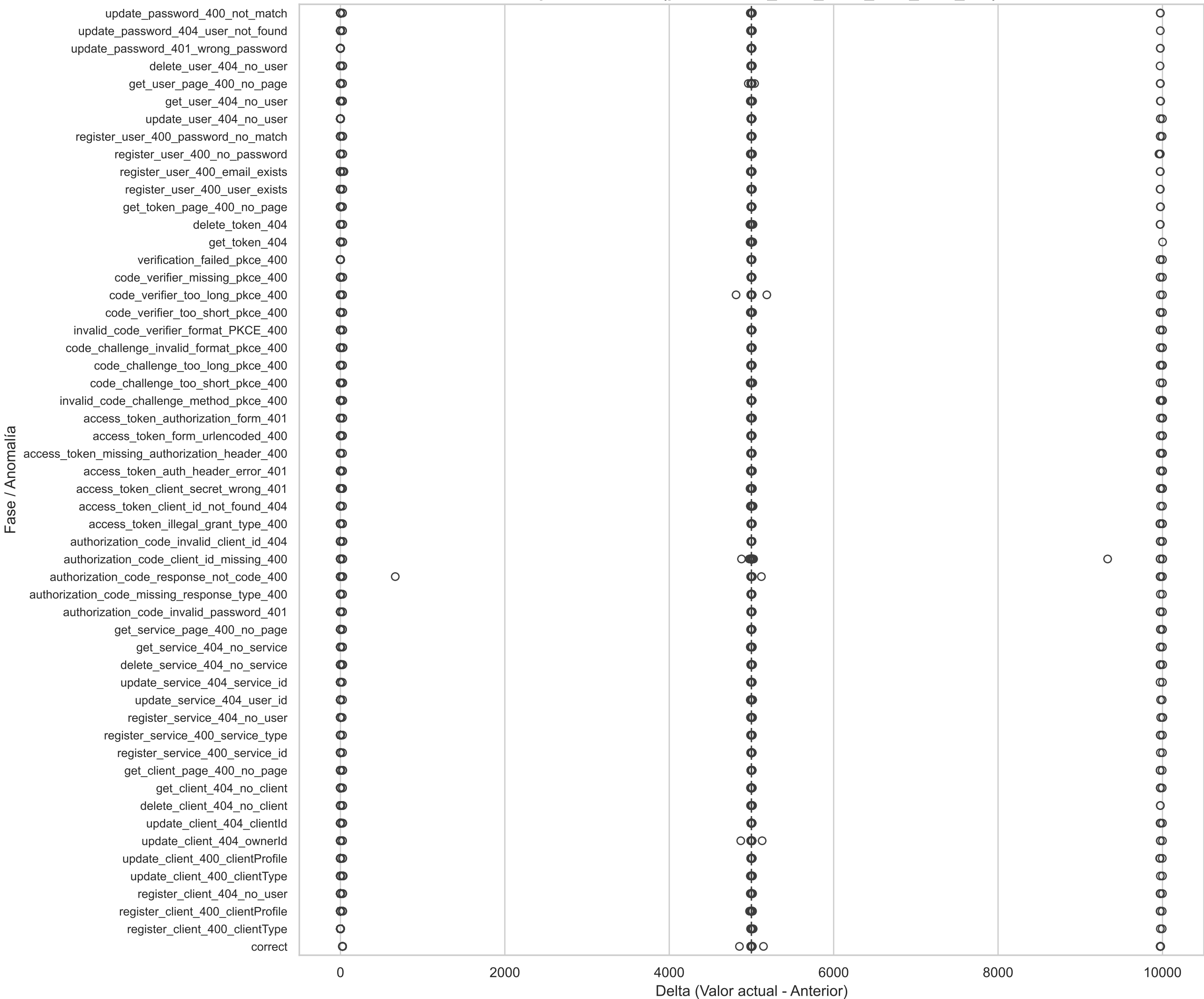
Boxplot Horizontal(prometheus_tsdb_head_max_time_diff)
