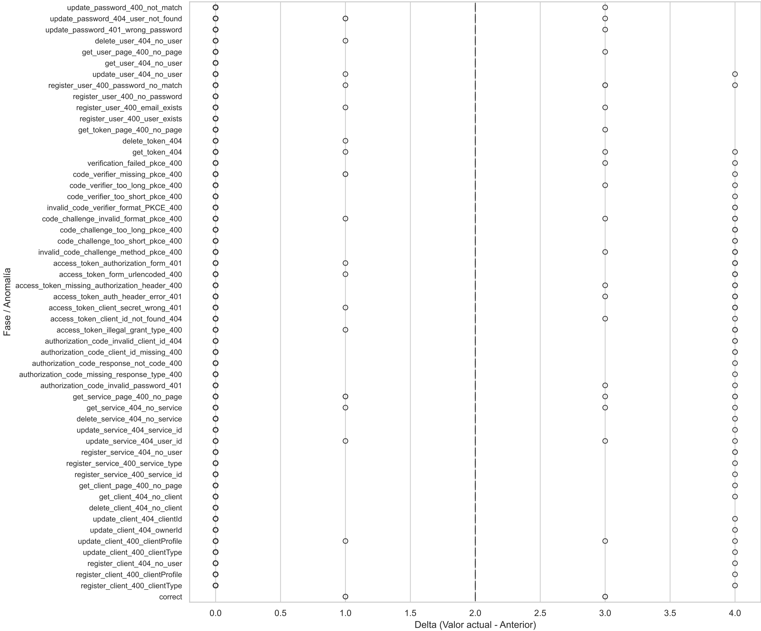
Boxplot Horizontal(prometheus_target_interval_length_seconds_count_diff)
