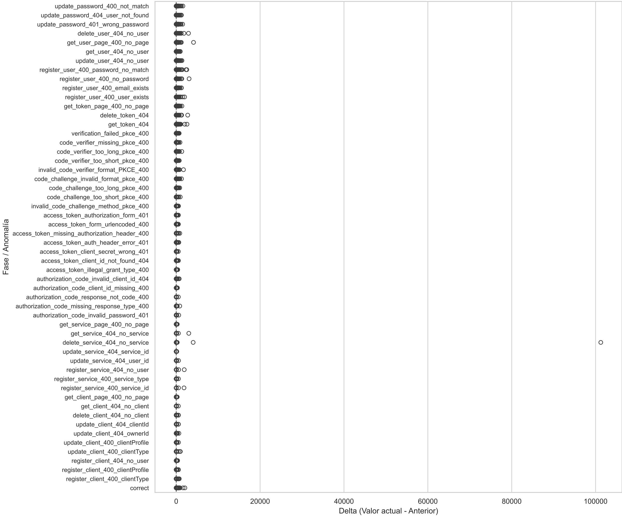
Boxplot Horizontal(node_vmstat_pswpout_diff)
