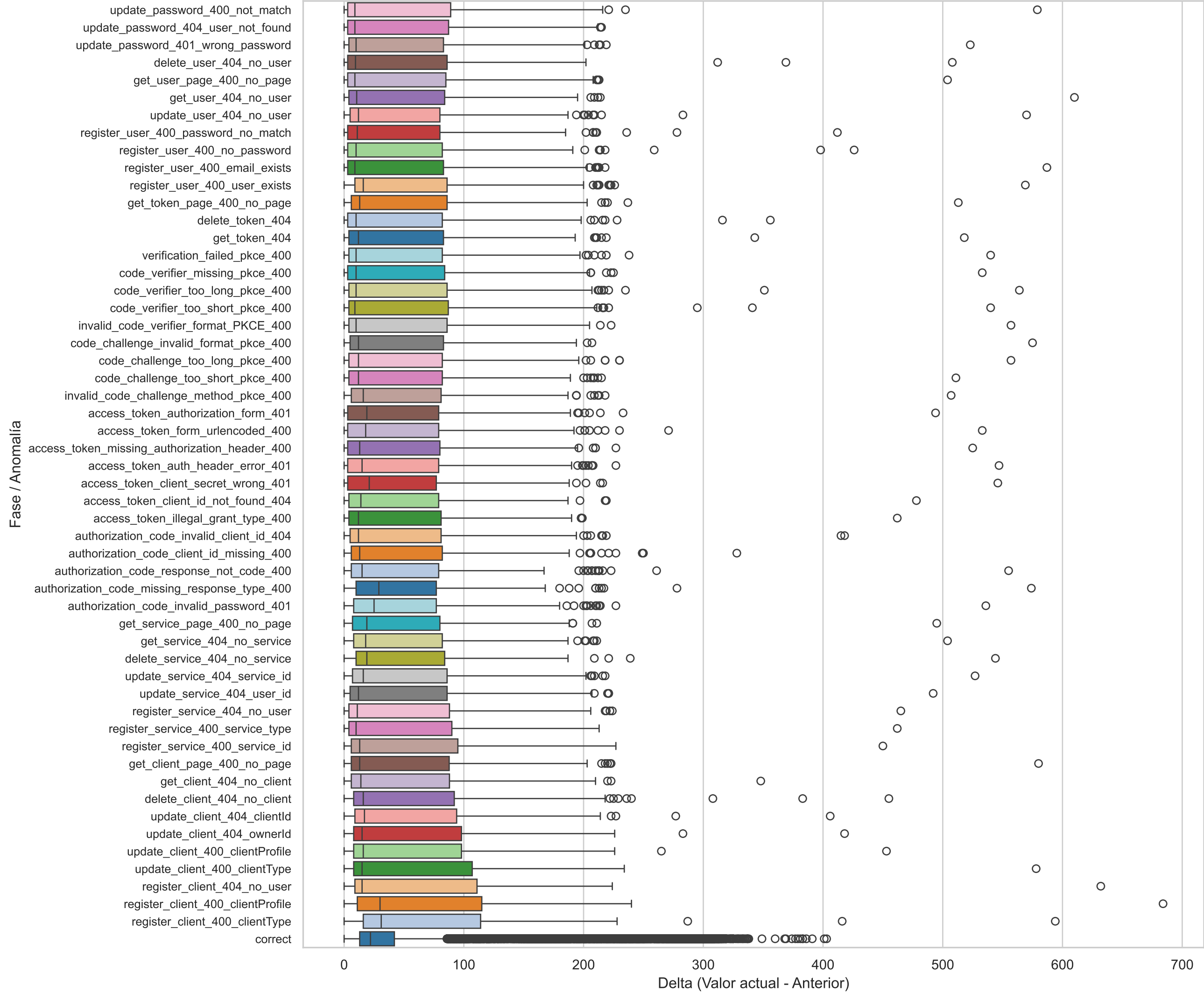
Boxplot Horizontal(node_forks_total_diff)
