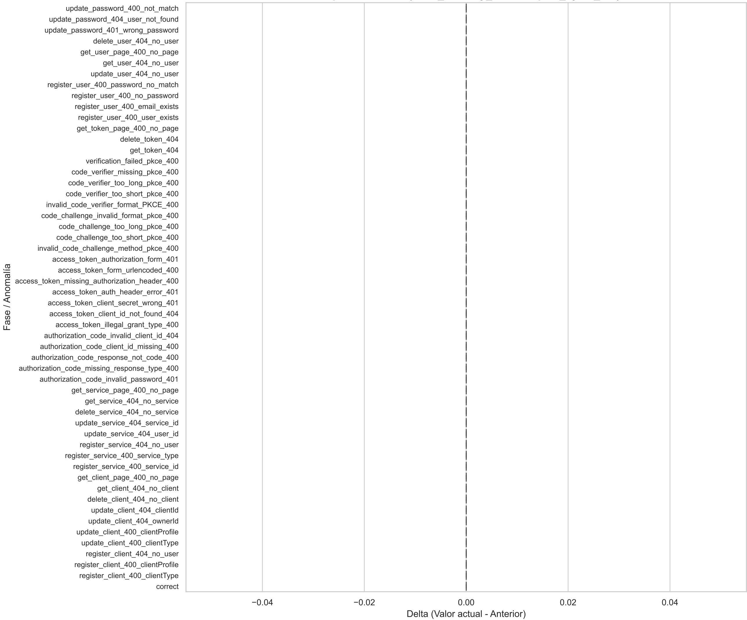
Boxplot Horizontal(node_memory_DirectMap2M_bytes_diff)
