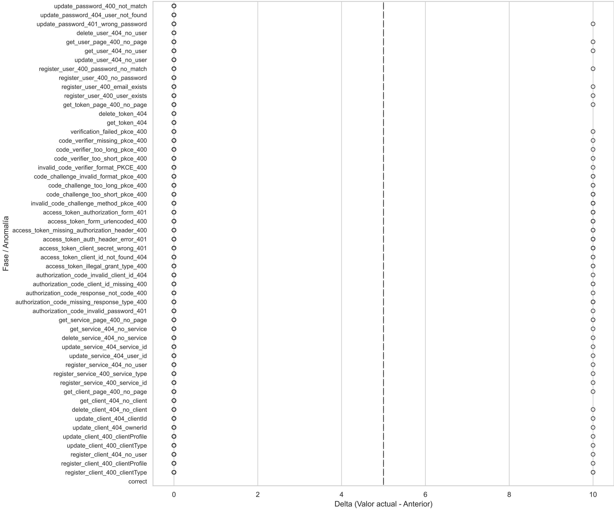
Boxplot Horizontal(node_netstat_Tcp_InSegs_diff)
