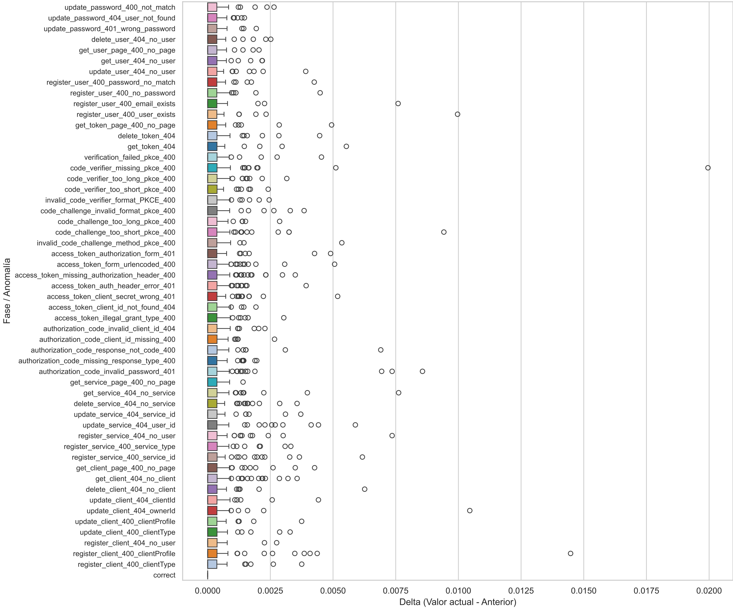
Boxplot Horizontal(prometheus_engine_query_duration_seconds_sum_diff)
