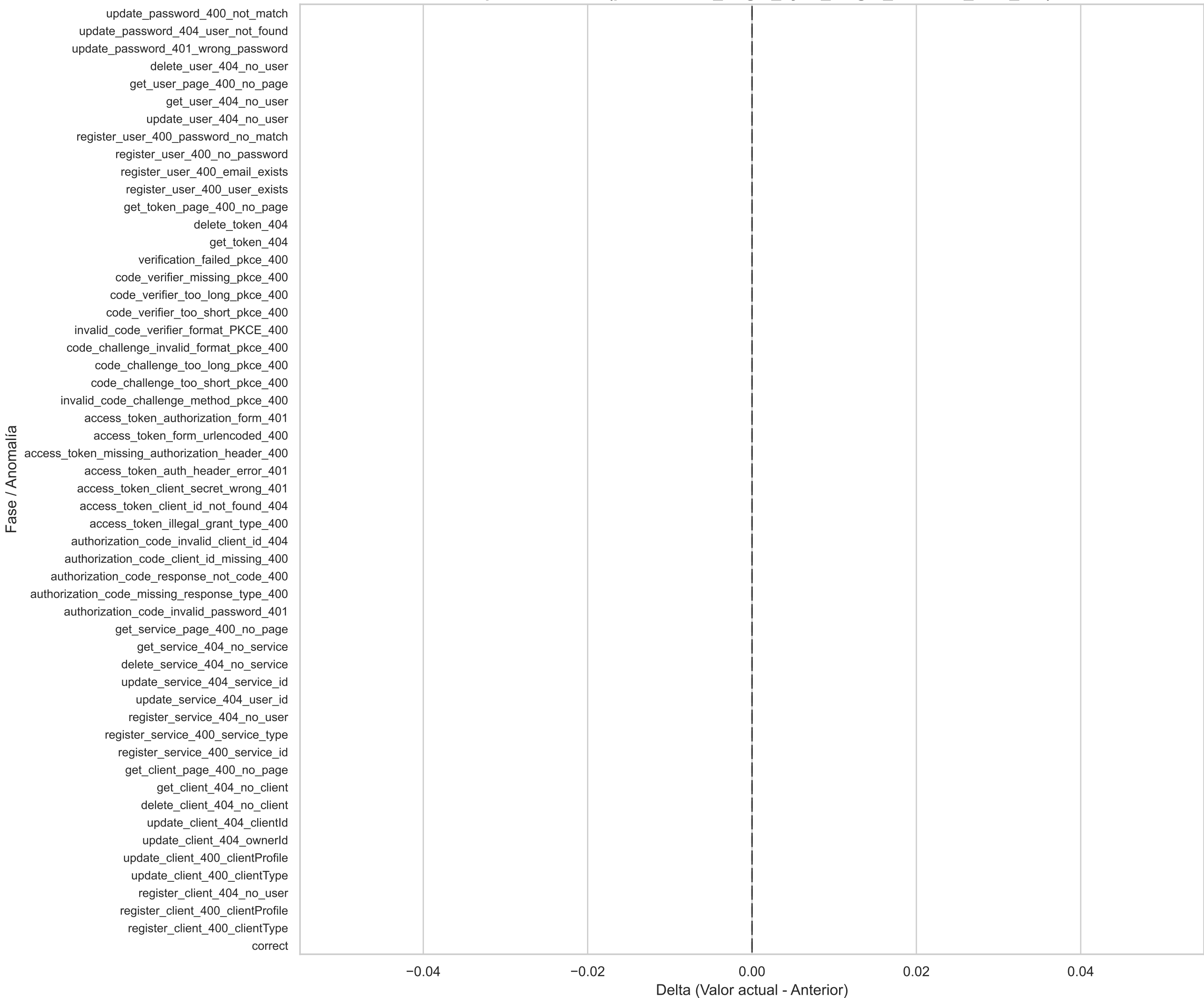
Boxplot Horizontal(prometheus_target_sync_length_seconds_sum_diff)
