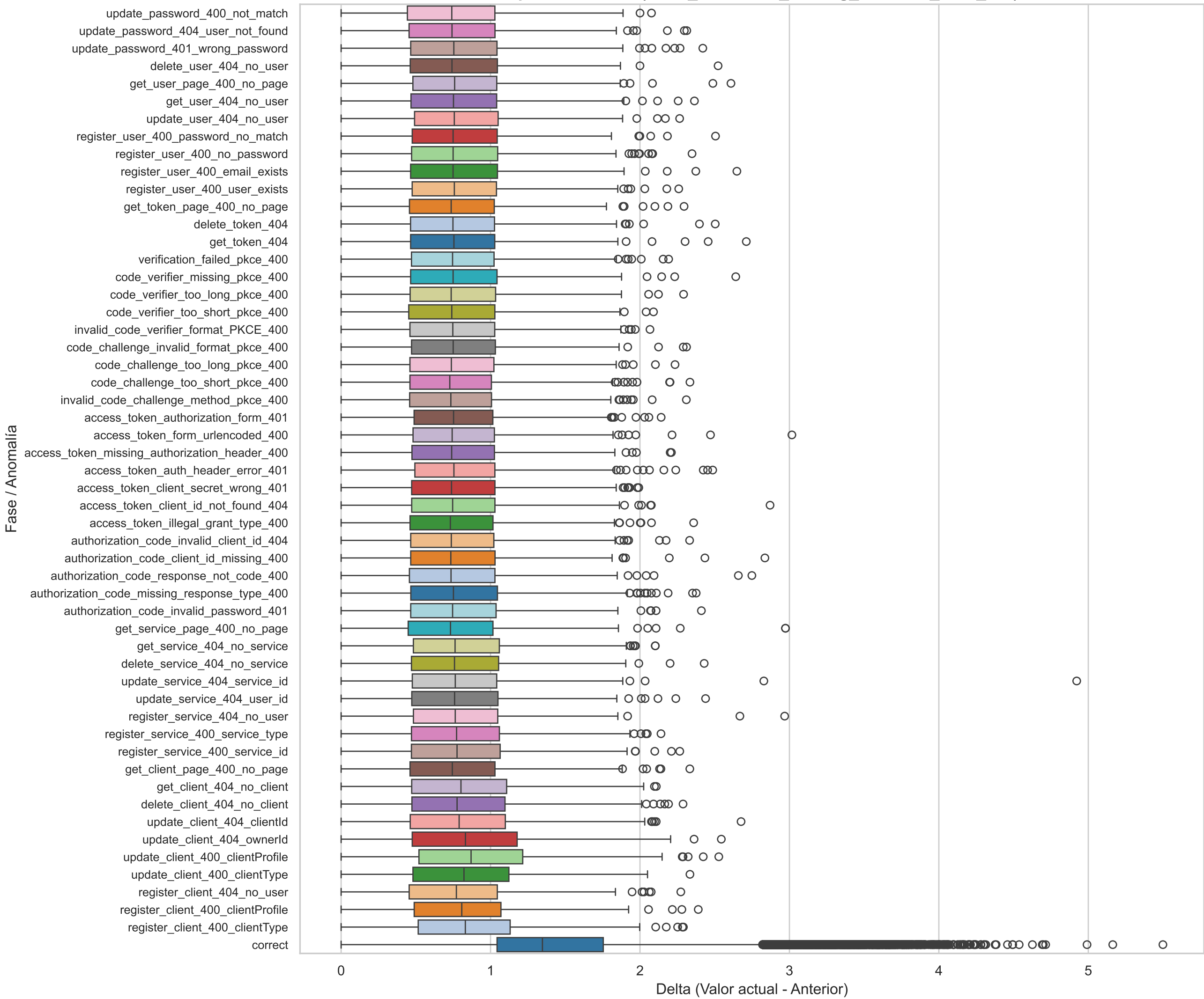
Boxplot Horizontal(node_schedstat_waiting_seconds_total_diff)
