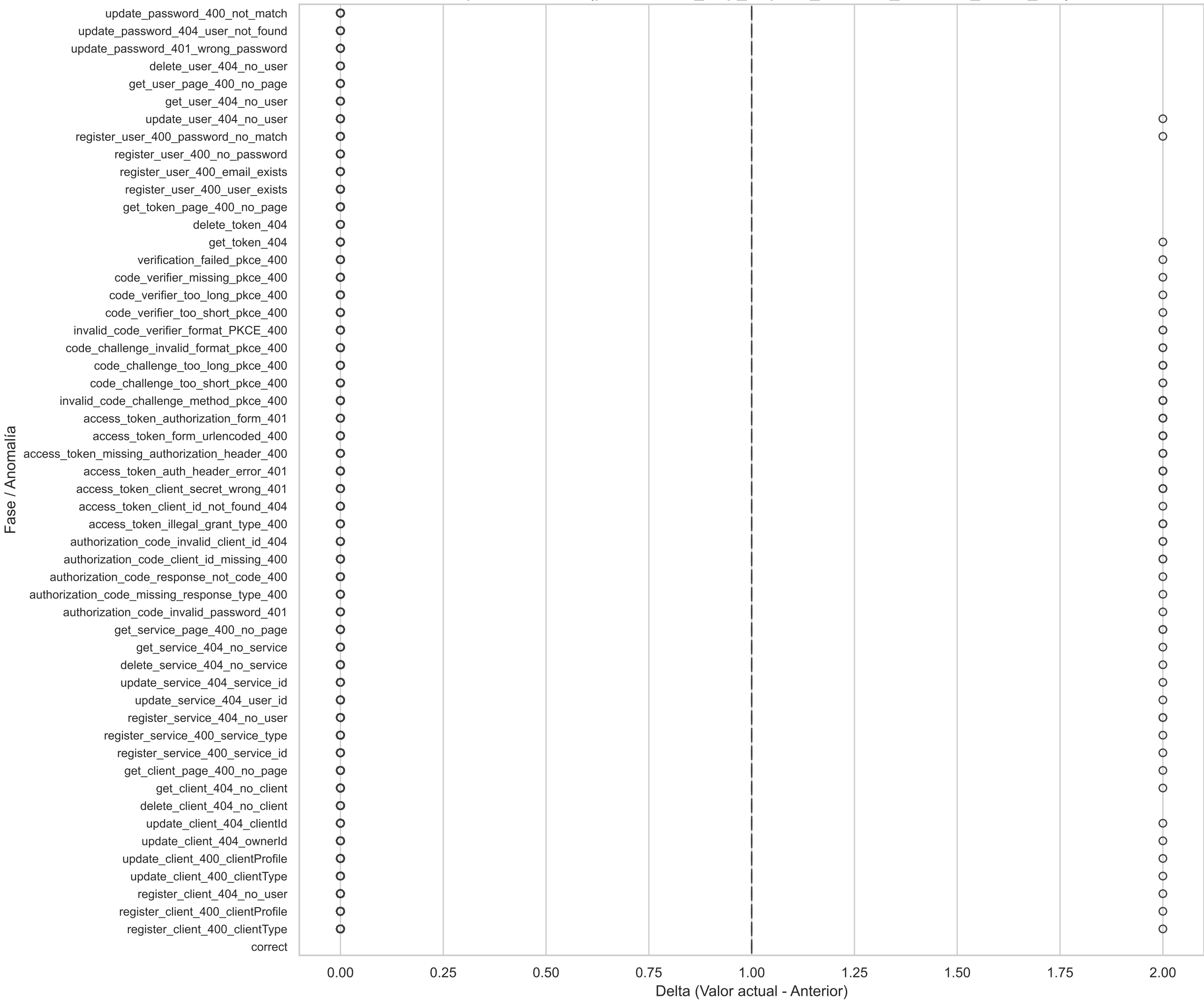
Boxplot Horizontal(prometheus_http_request_duration_seconds_count_diff)
