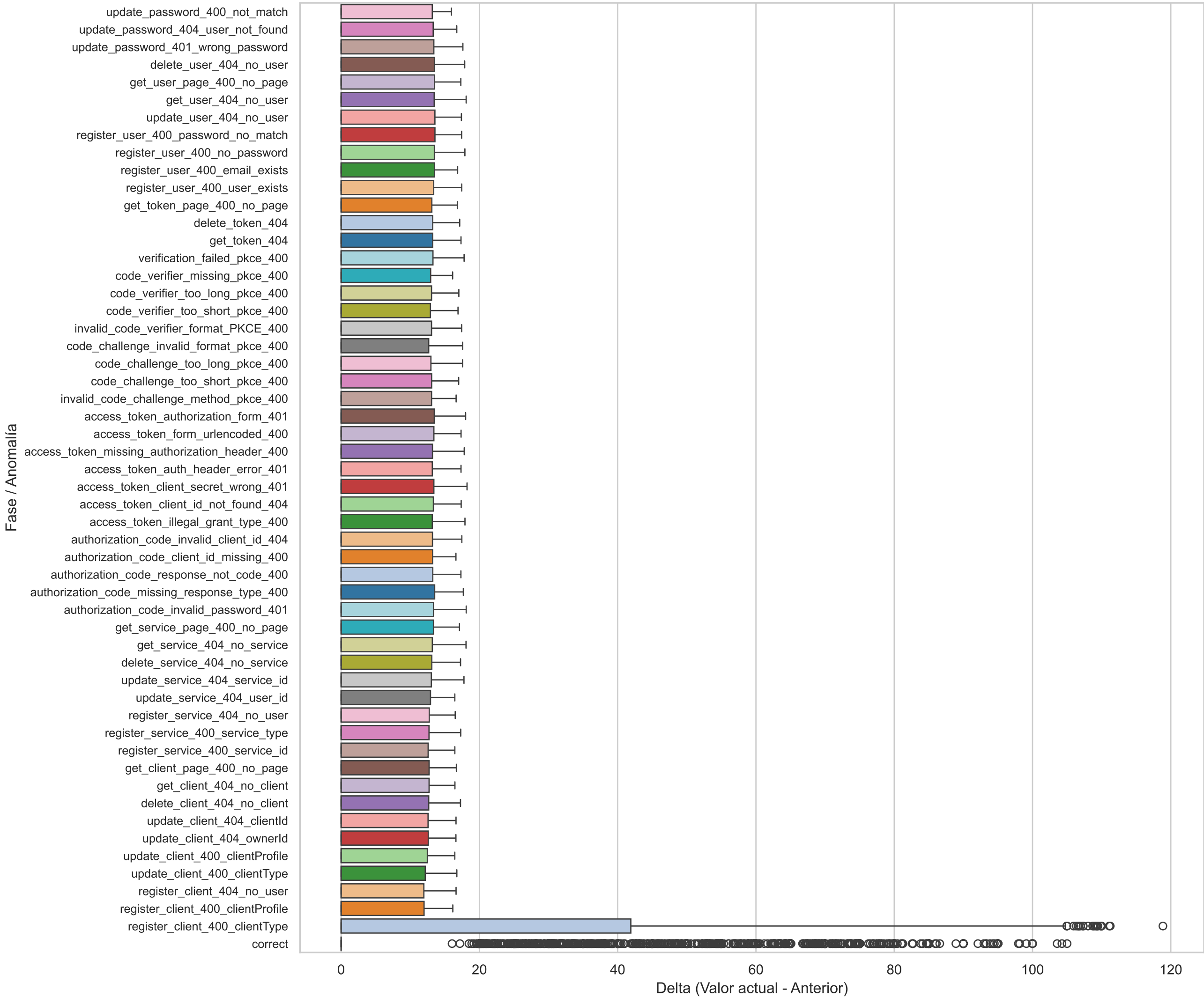
Boxplot Horizontal(go_memstats_last_gc_time_seconds_diff)
