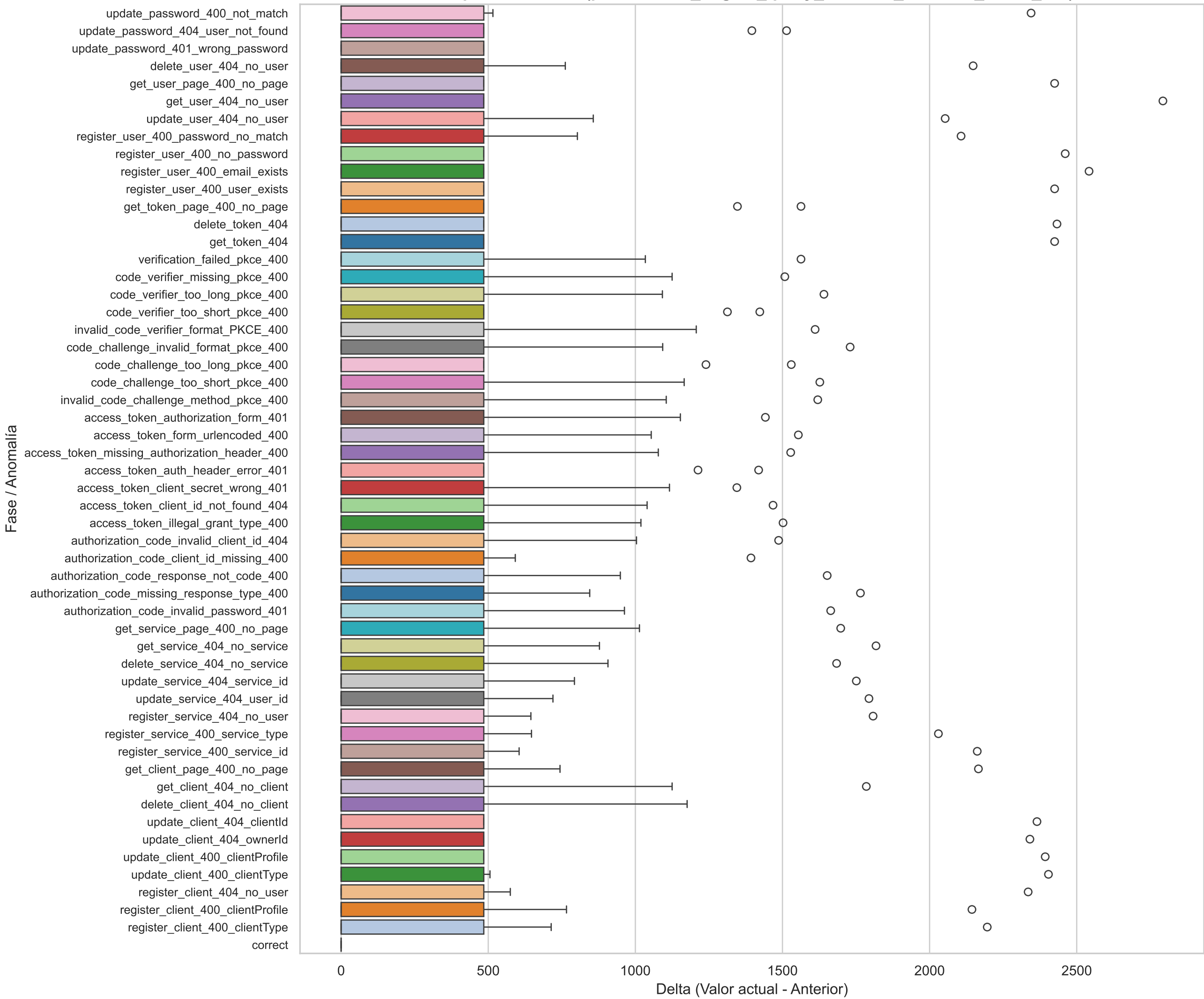
Boxplot Horizontal(prometheus_engine_query_duration_seconds_count_diff)
