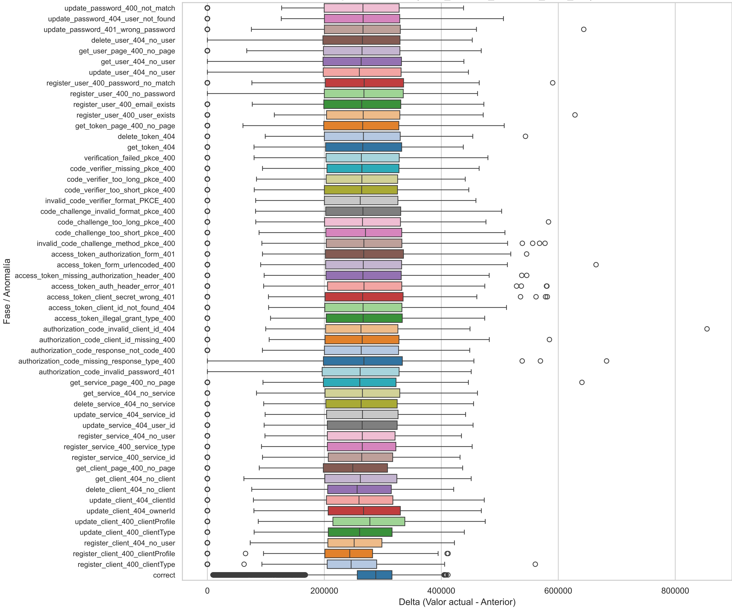
Boxplot Horizontal(node_context_switches_total_diff)
