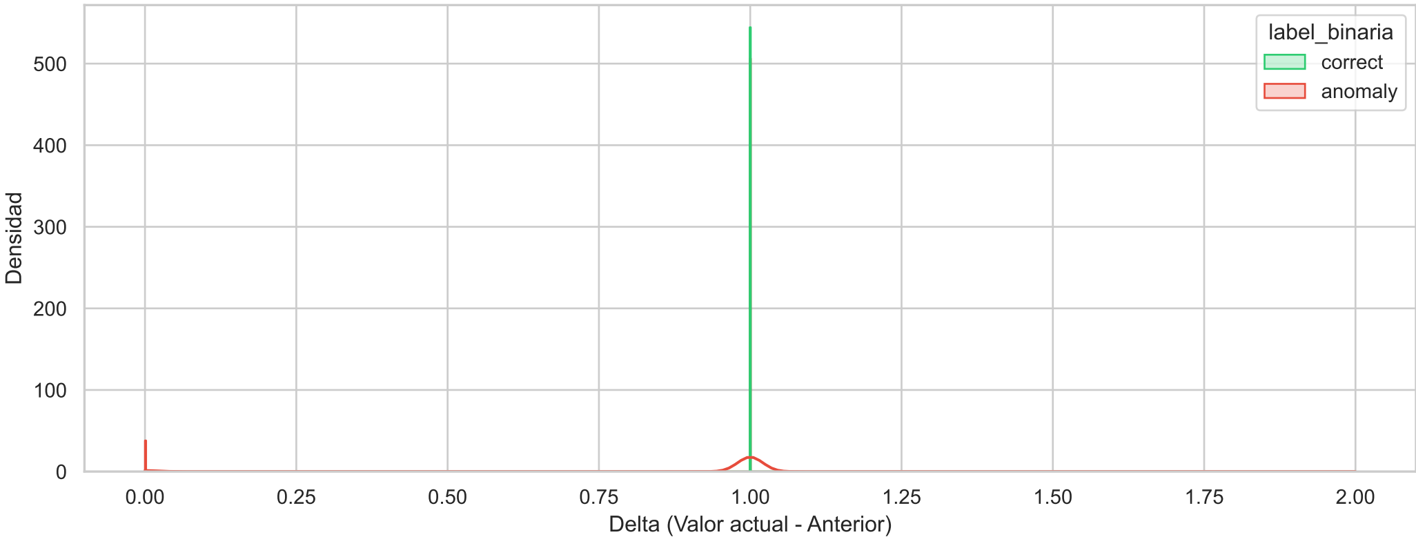
Histograma de Densidad Binario (prometheus_http_request_duration_seconds_count_diff)
