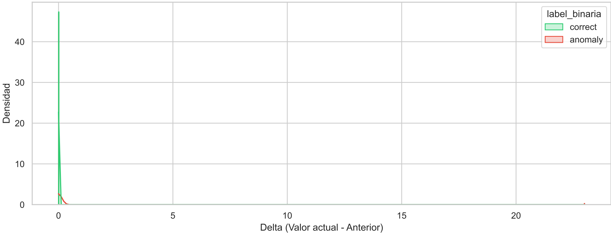
Histograma de Densidad Binario (prometheus_tsdb_head_series_created_total_diff)
