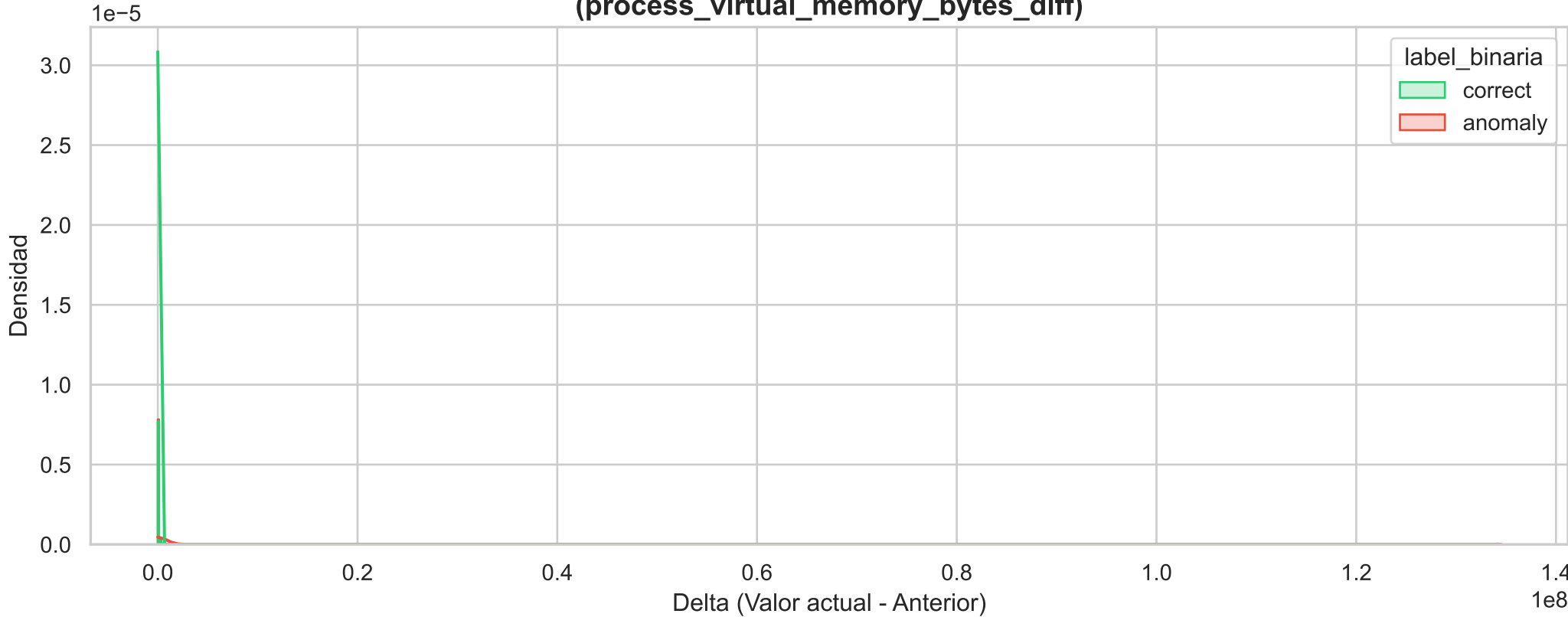
Histograma de Densidad Binario (process_virtual_memory_bytes_diff)
