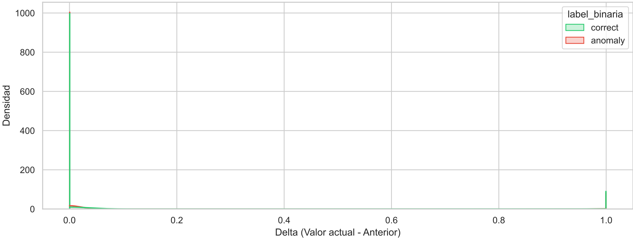
Histograma de Densidad Binario (prometheus_tsdb_compactions_triggered_total_diff)
