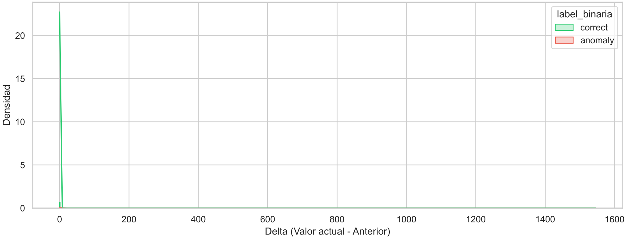
Histograma de Densidad Binario (prometheus_tsdb_head_chunks_created_total_diff)
