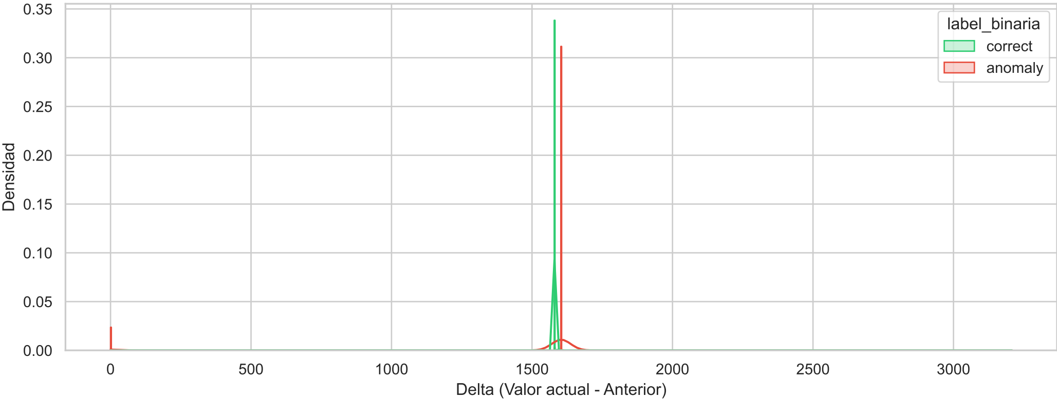
Histograma de Densidad Binario (prometheus_remote_storage_samples_in_total_diff)
