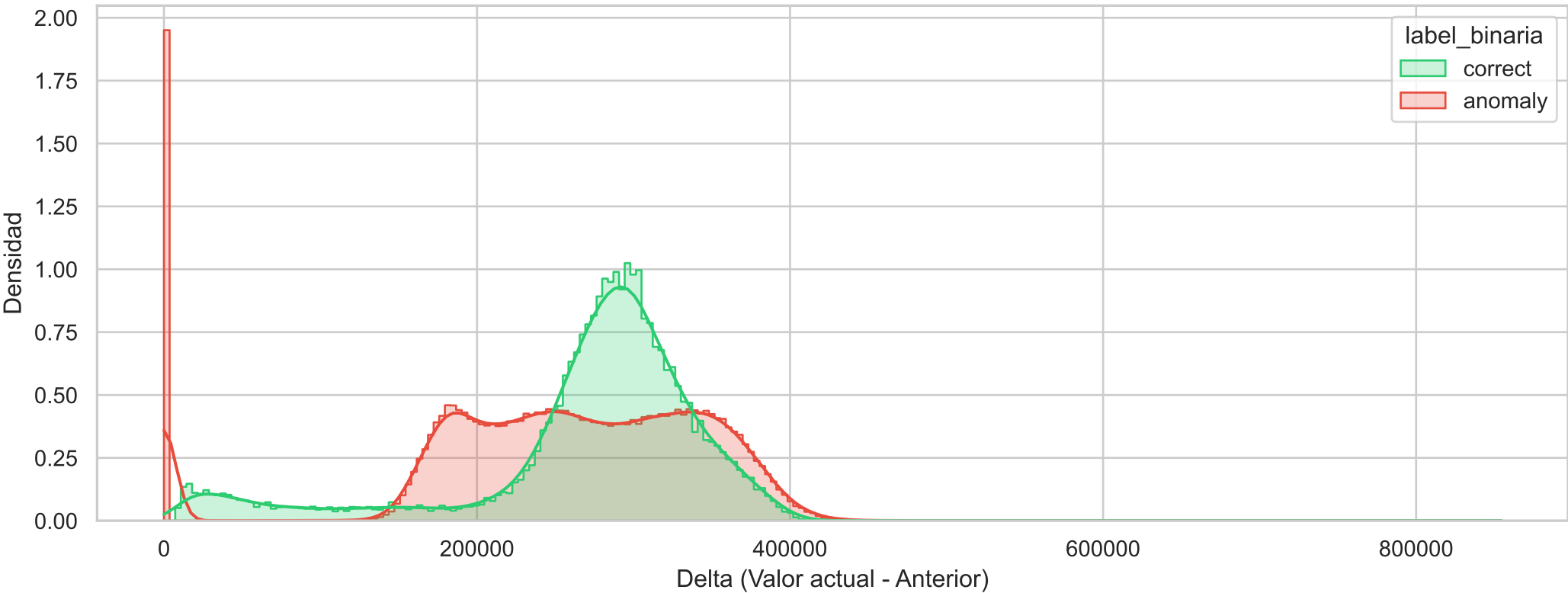
Histograma de Densidad Binario (node_context_switches_total_diff)
