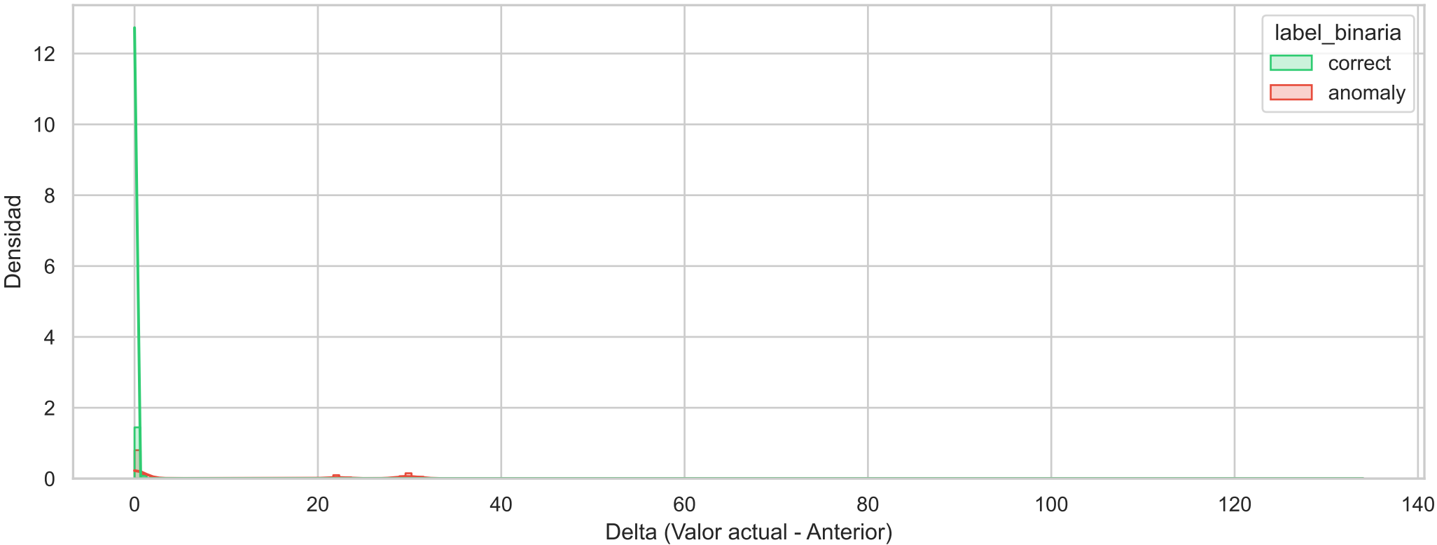
Histograma de Densidad Binario (go_gc_duration_seconds_count_diff)
