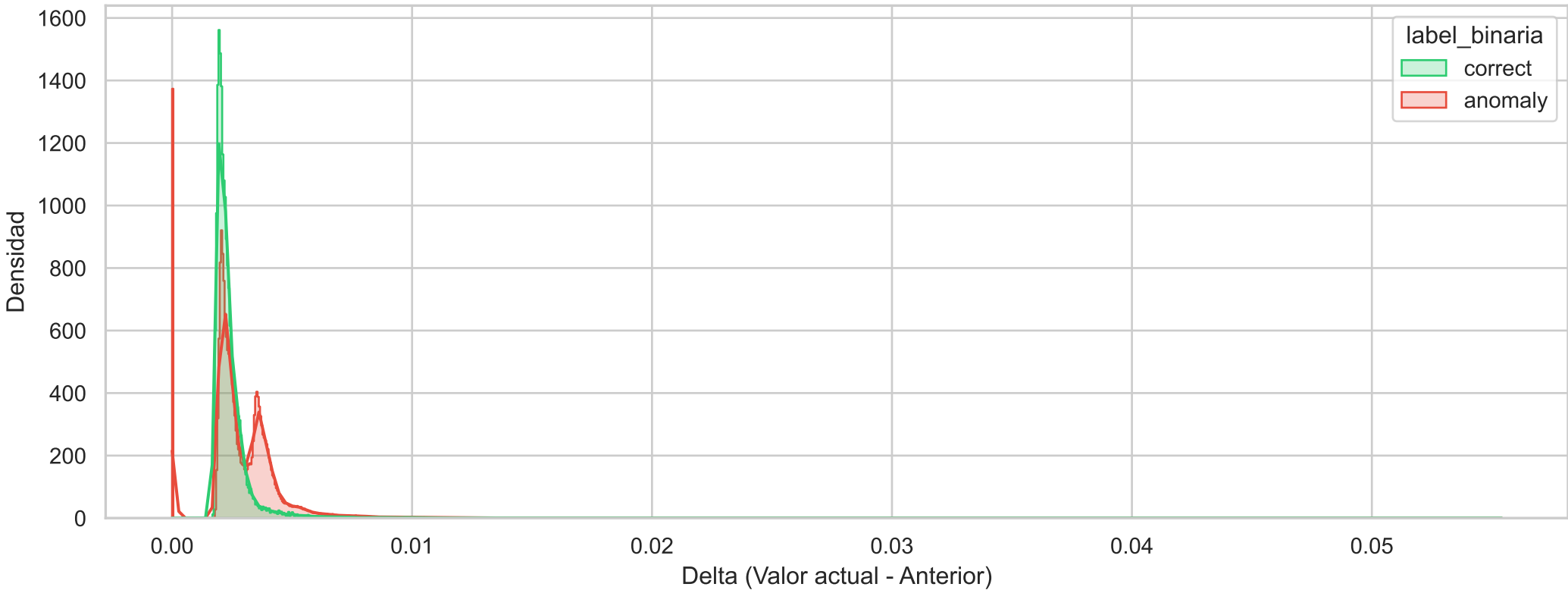
Histograma de Densidad Binario (prometheus_http_request_duration_seconds_sum_diff)
