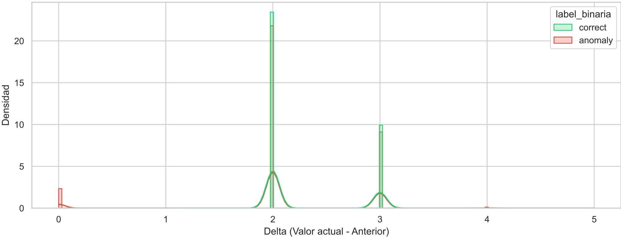
Histograma de Densidad Binario (prometheus_tsdb_wal_page_flushes_total_diff)
