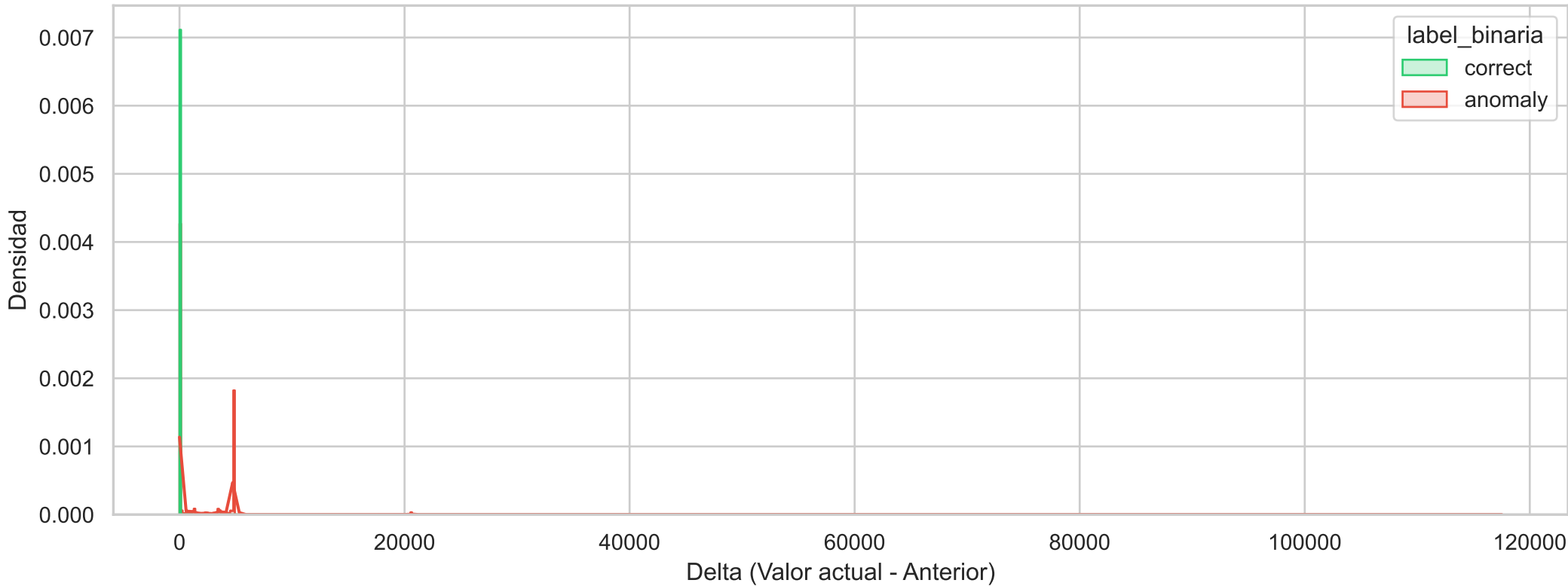
Histograma de Densidad Binario (prometheus_engine_query_samples_total_diff)
