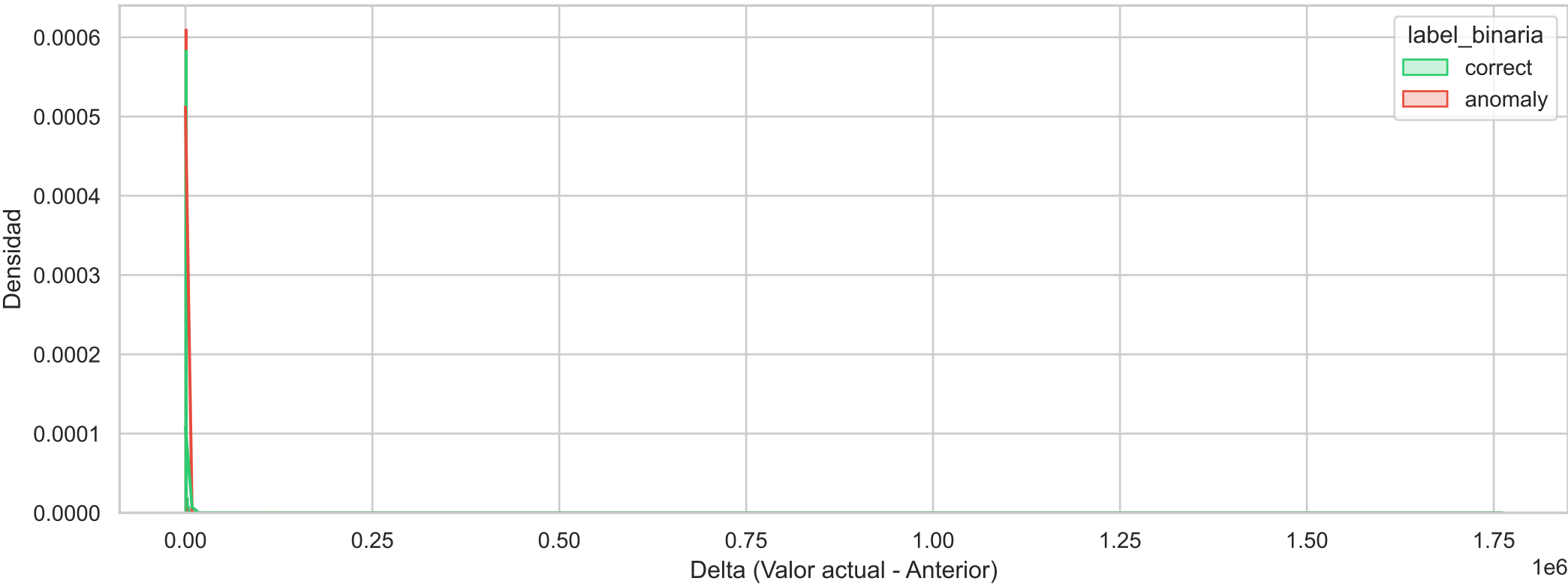
Histograma de Densidad Binario (node_vmstat_pgpgin_diff)
