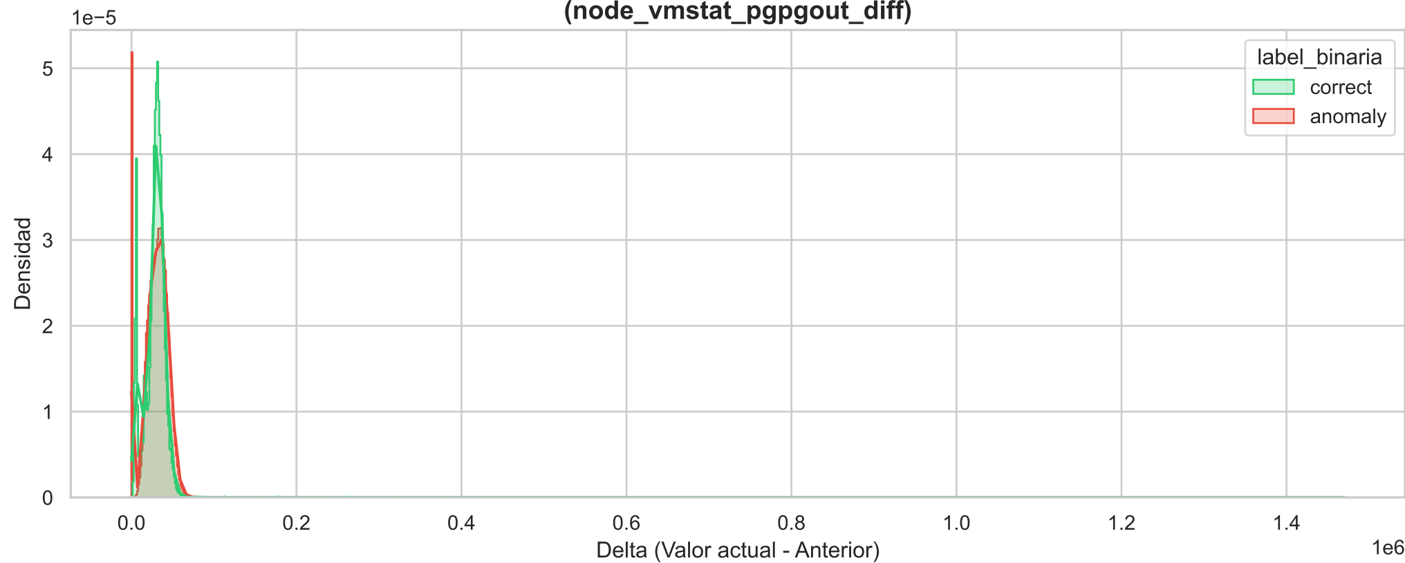
Histograma de Densidad Binario (node_vmstat_pgpgout_diff)
