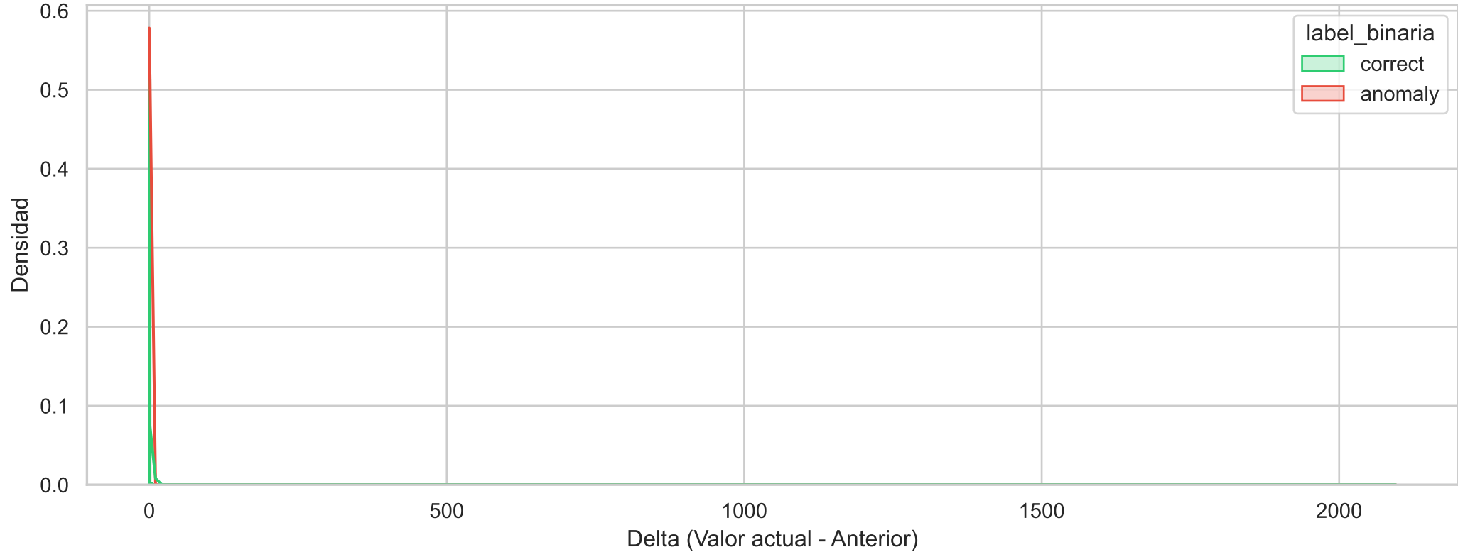
Histograma de Densidad Binario (node_vmstat_pswpin_diff)
