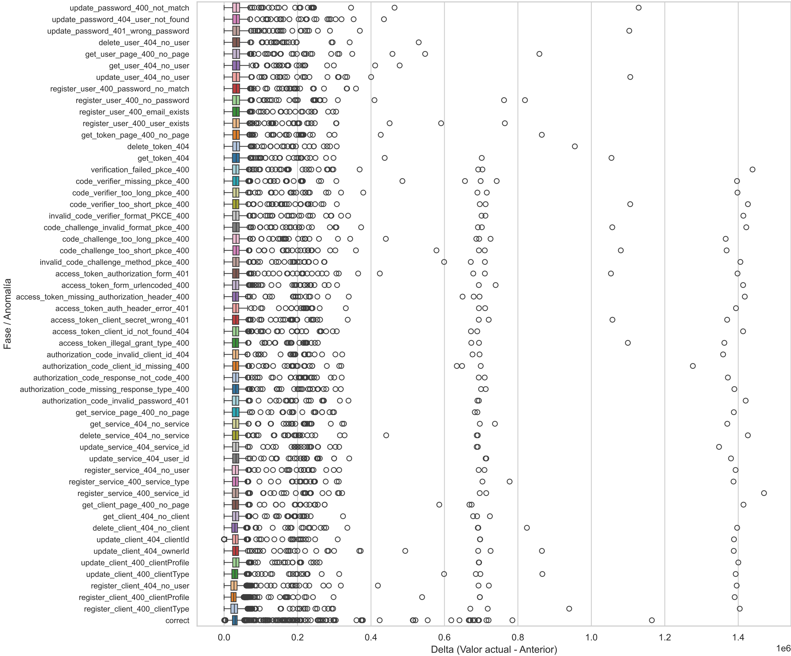
Boxplot Horizontal(node_vmstat_pgpgout_diff)
