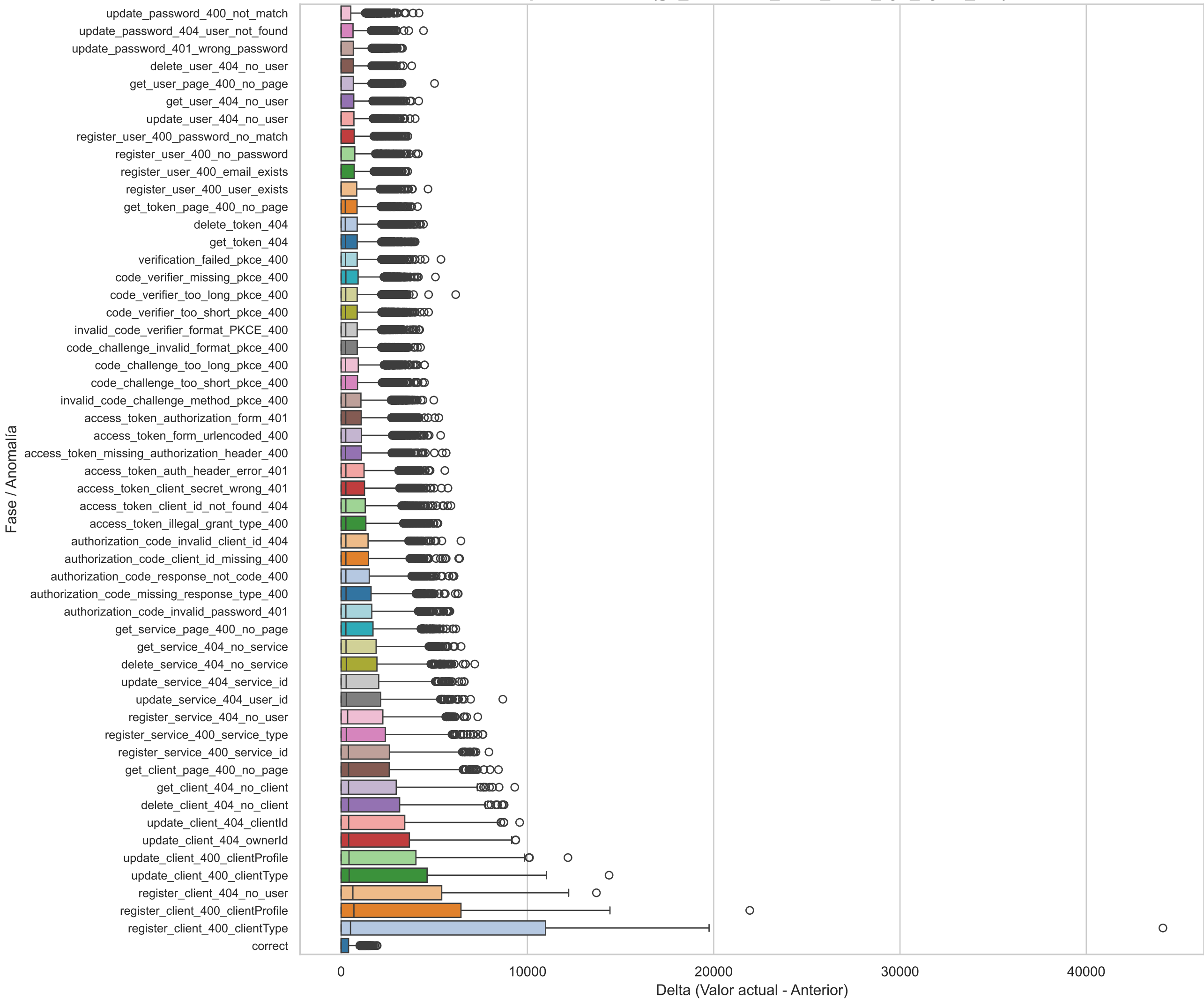
Boxplot Horizontal(go_memstats_buck_hash_sys_bytes_diff)
