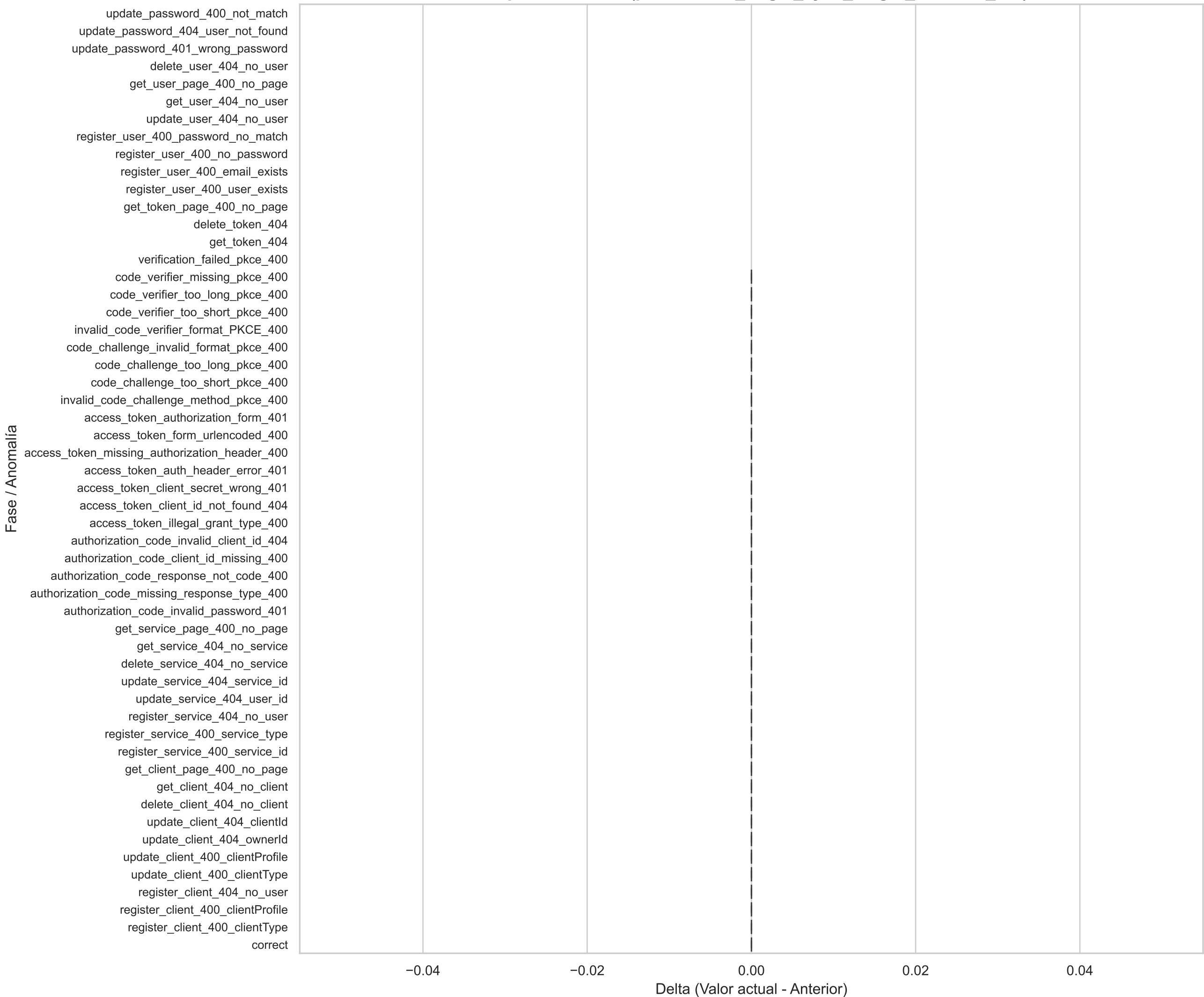
Boxplot Horizontal(prometheus_target_sync_length_seconds_diff)
