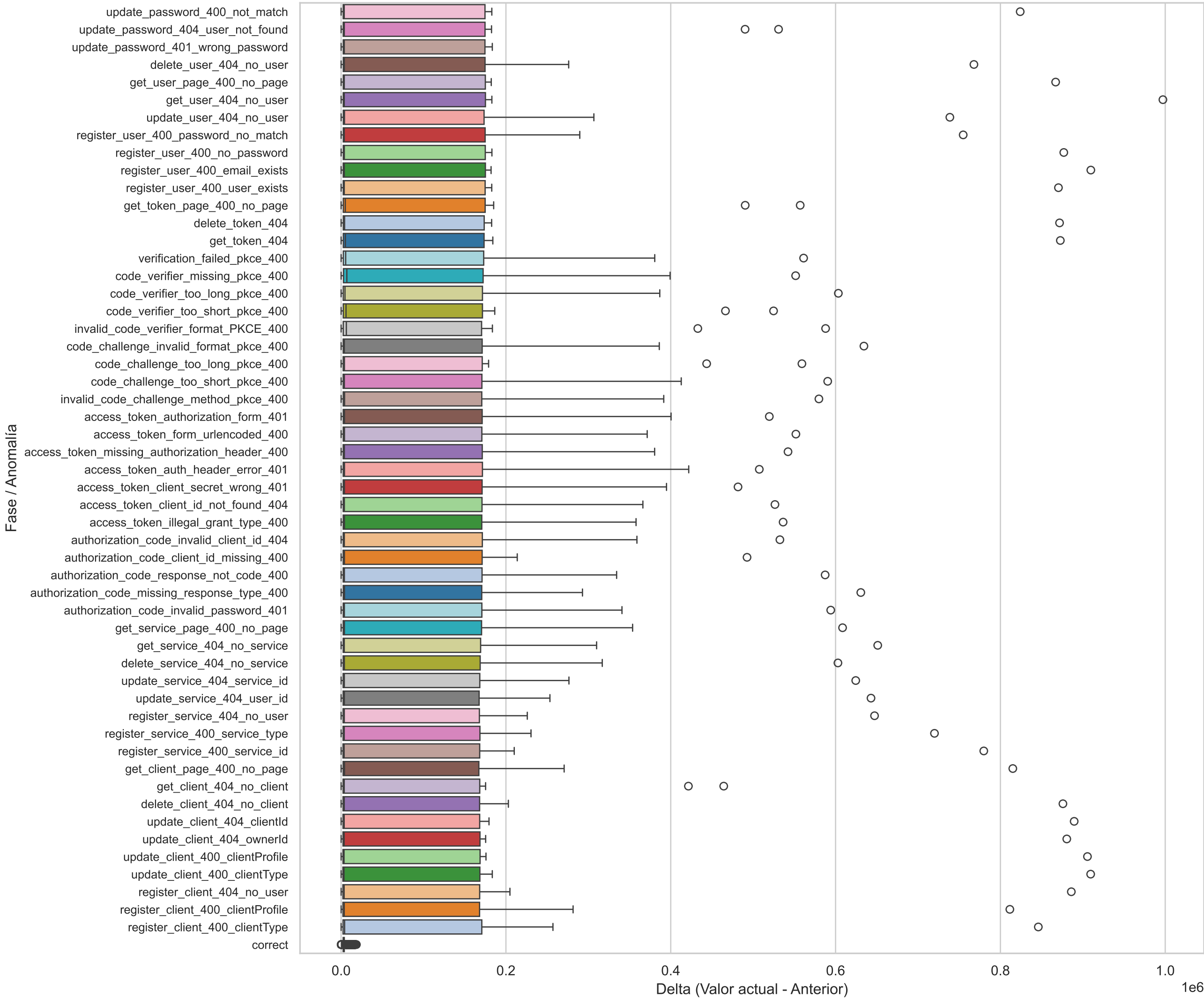
Boxplot Horizontal(go_memstats_mallocs_total_diff)
