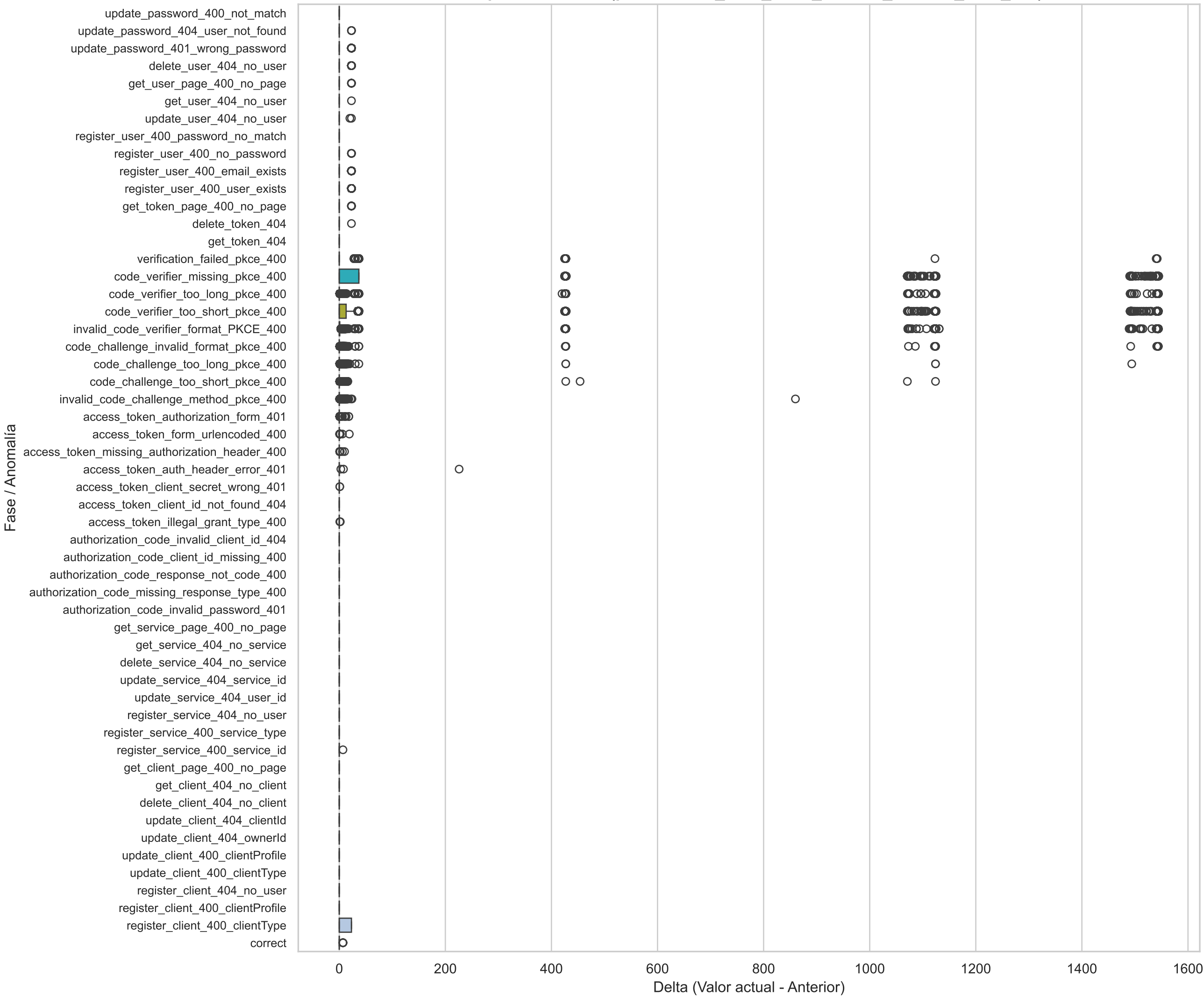
Boxplot Horizontal(prometheus_tsdb_head_chunks_created_total_diff)
