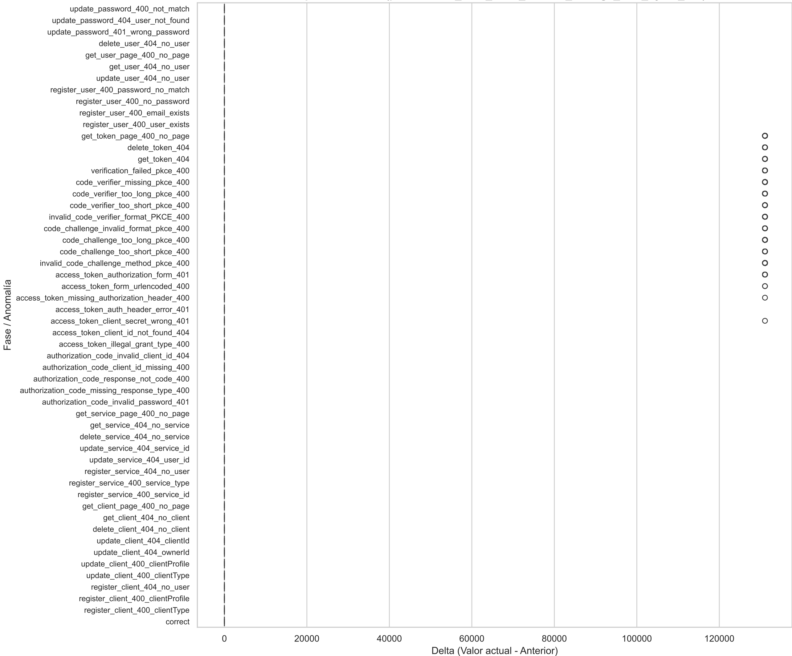
Boxplot Horizontal(prometheus_tsdb_head_chunks_storage_size_bytes_diff)
