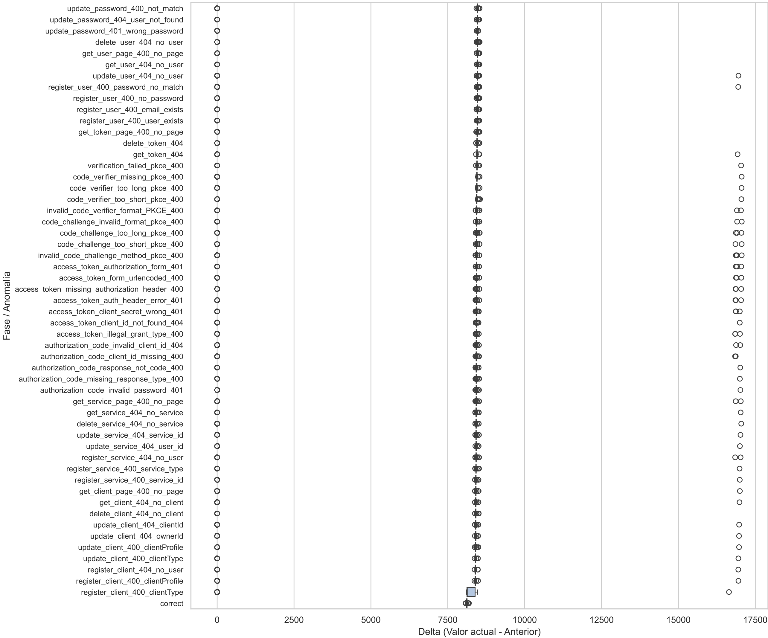
Boxplot Horizontal(prometheus_http_response_size_bytes_sum_diff)
