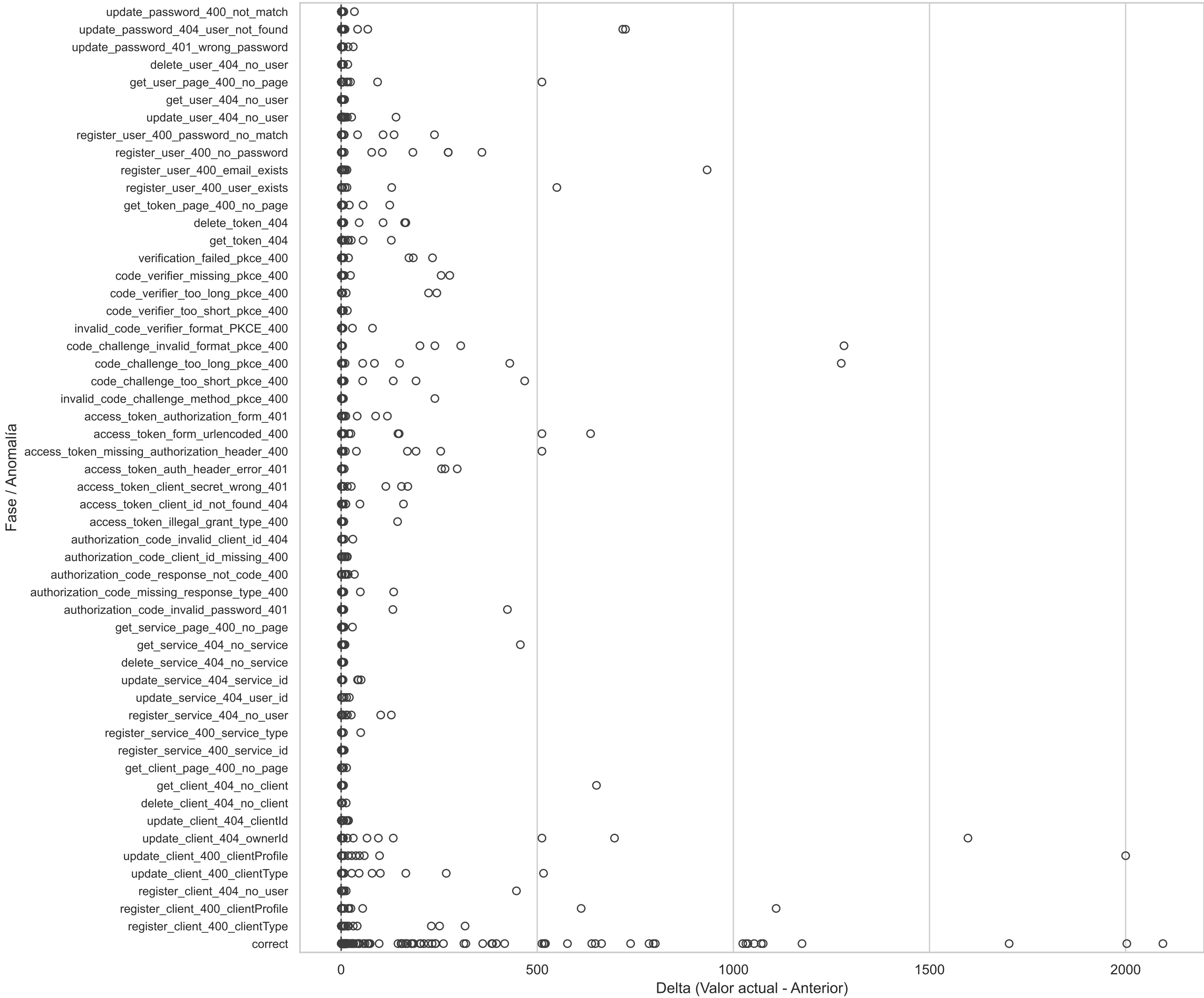
Boxplot Horizontal(node_vmstat_pswpin_diff)
