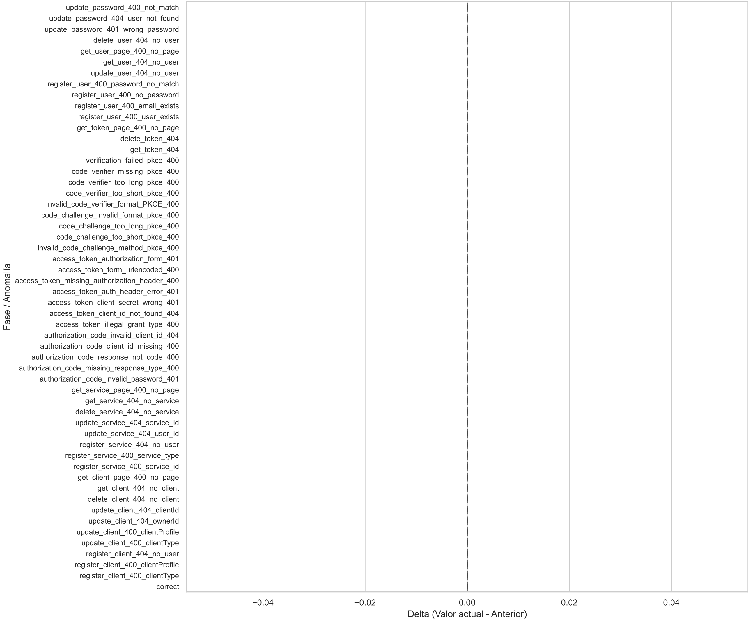
Boxplot Horizontal(node_os_version_diff)
