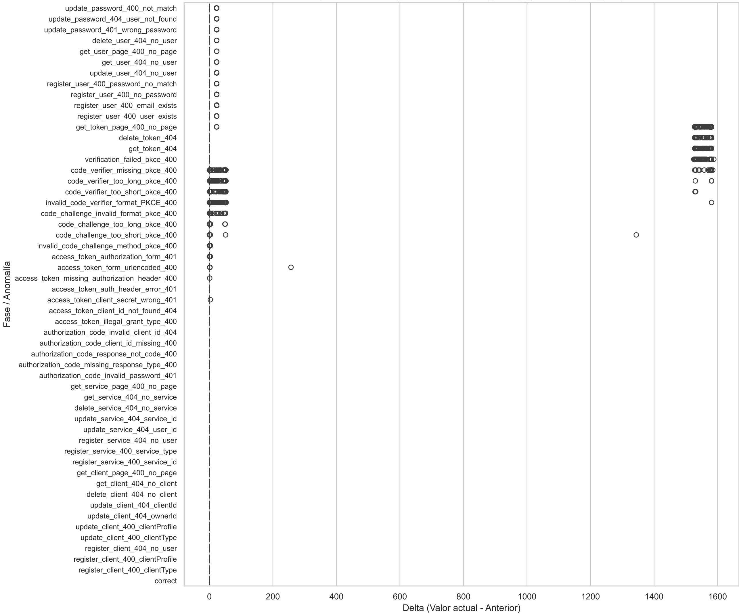
Boxplot Horizontal(prometheus_tsdb_mmap_chunks_total_diff)
