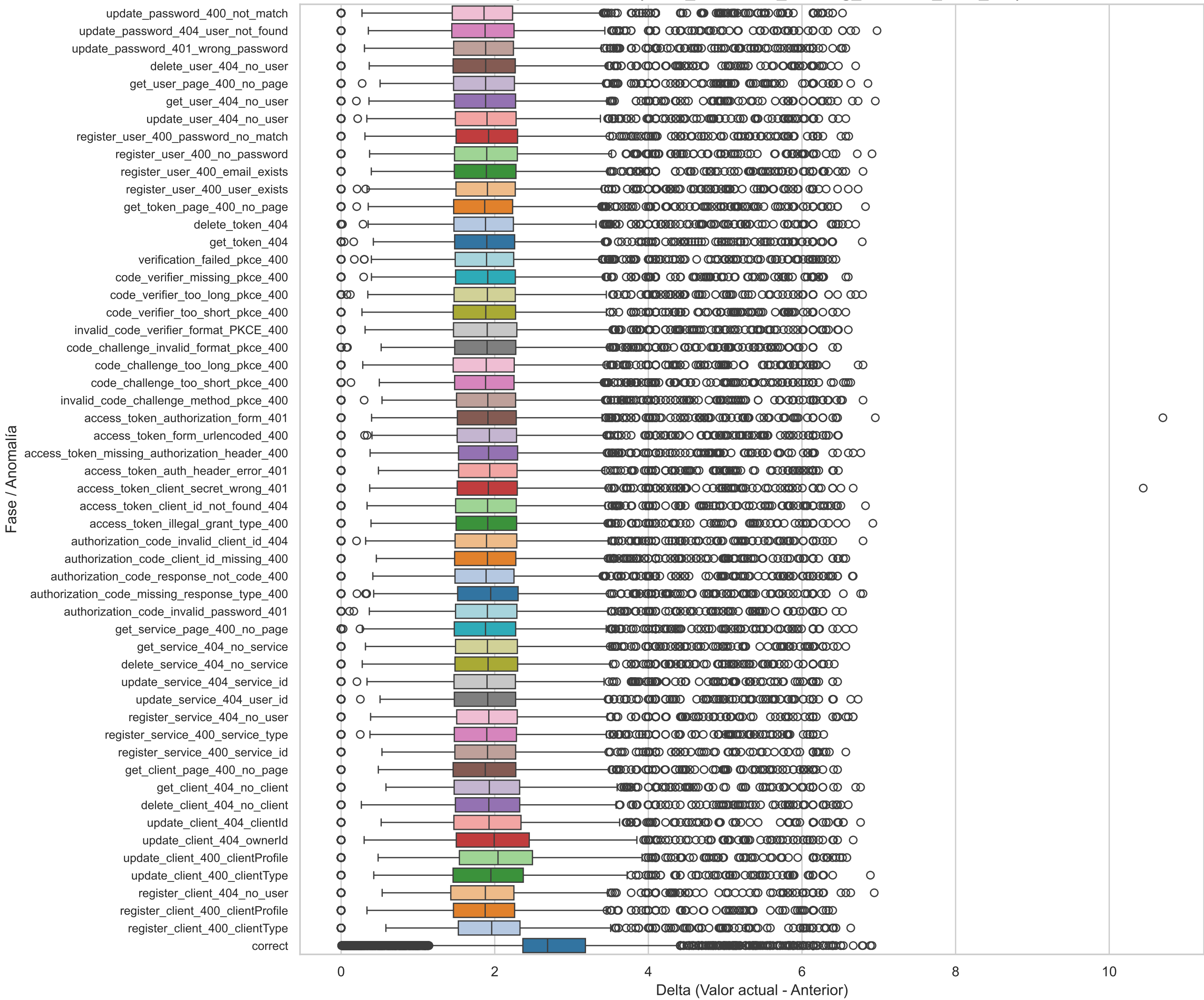
Boxplot Horizontal(node_schedstat_running_seconds_total_diff)
