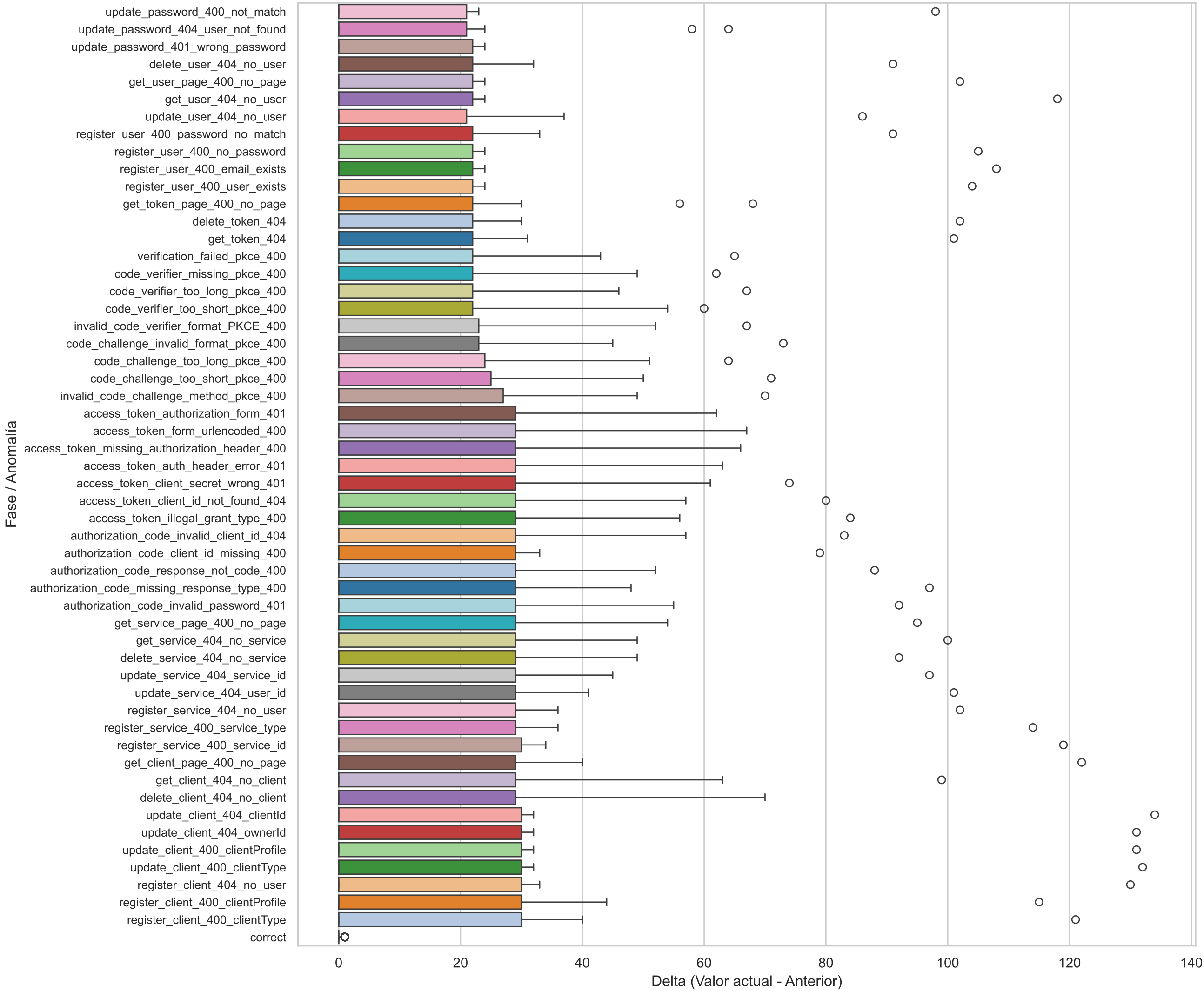
Boxplot Horizontal(go_gc_duration_seconds_count_diff)
