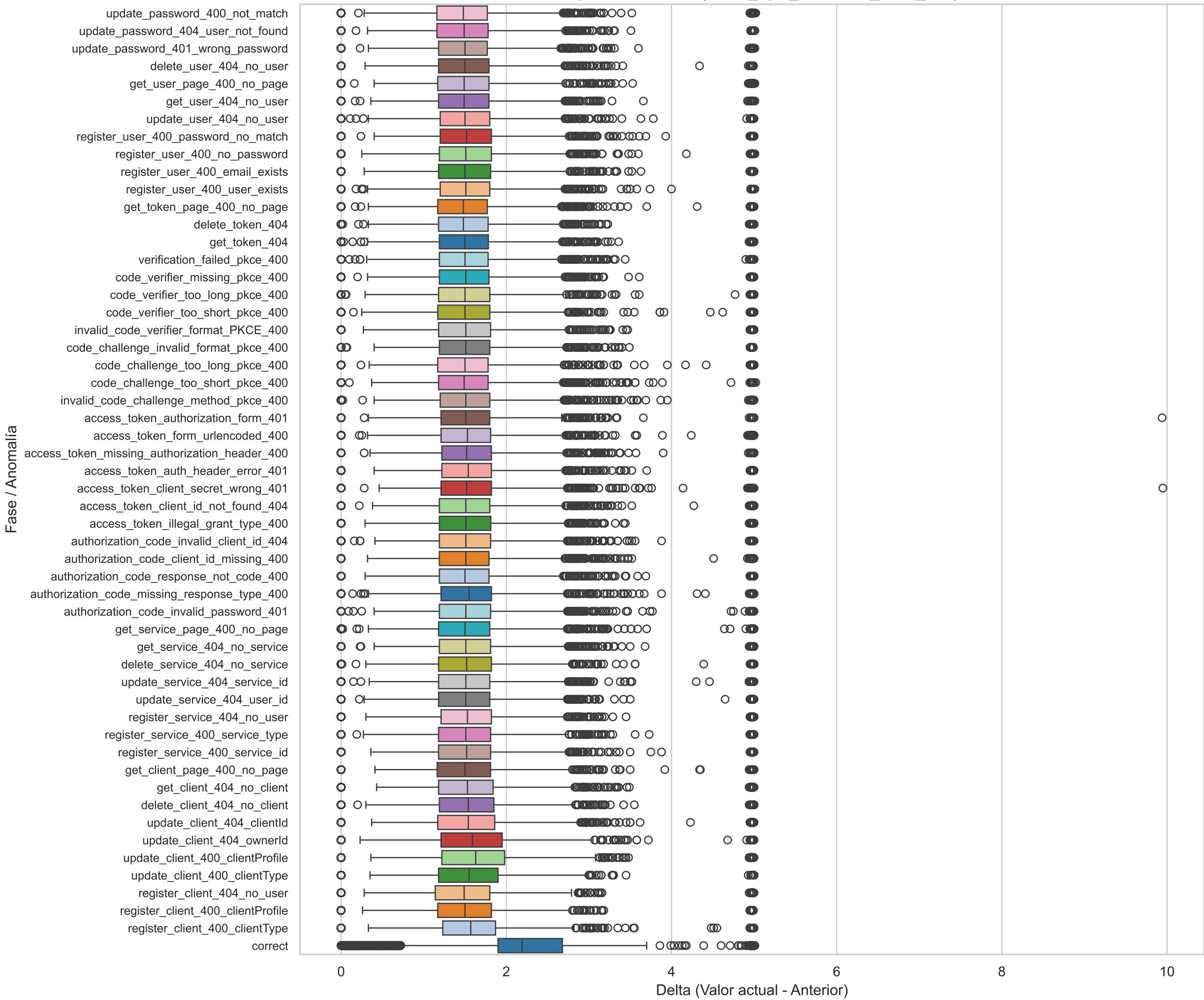
Boxplot Horizontal(node_cpu_seconds_total_diff)
