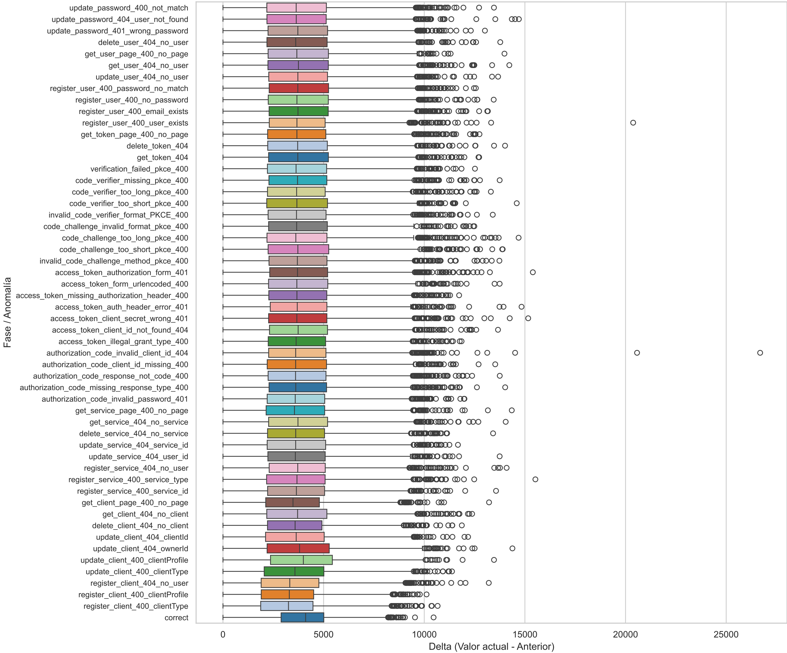
Boxplot Horizontal(node_softnet_processed_total_diff)
