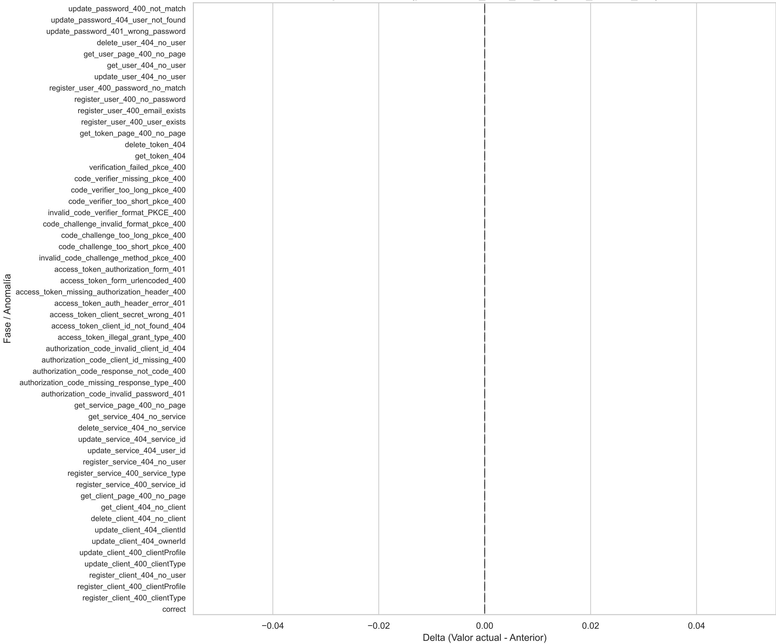
Boxplot Horizontal(prometheus_tsdb_wal_segment_current_diff)
