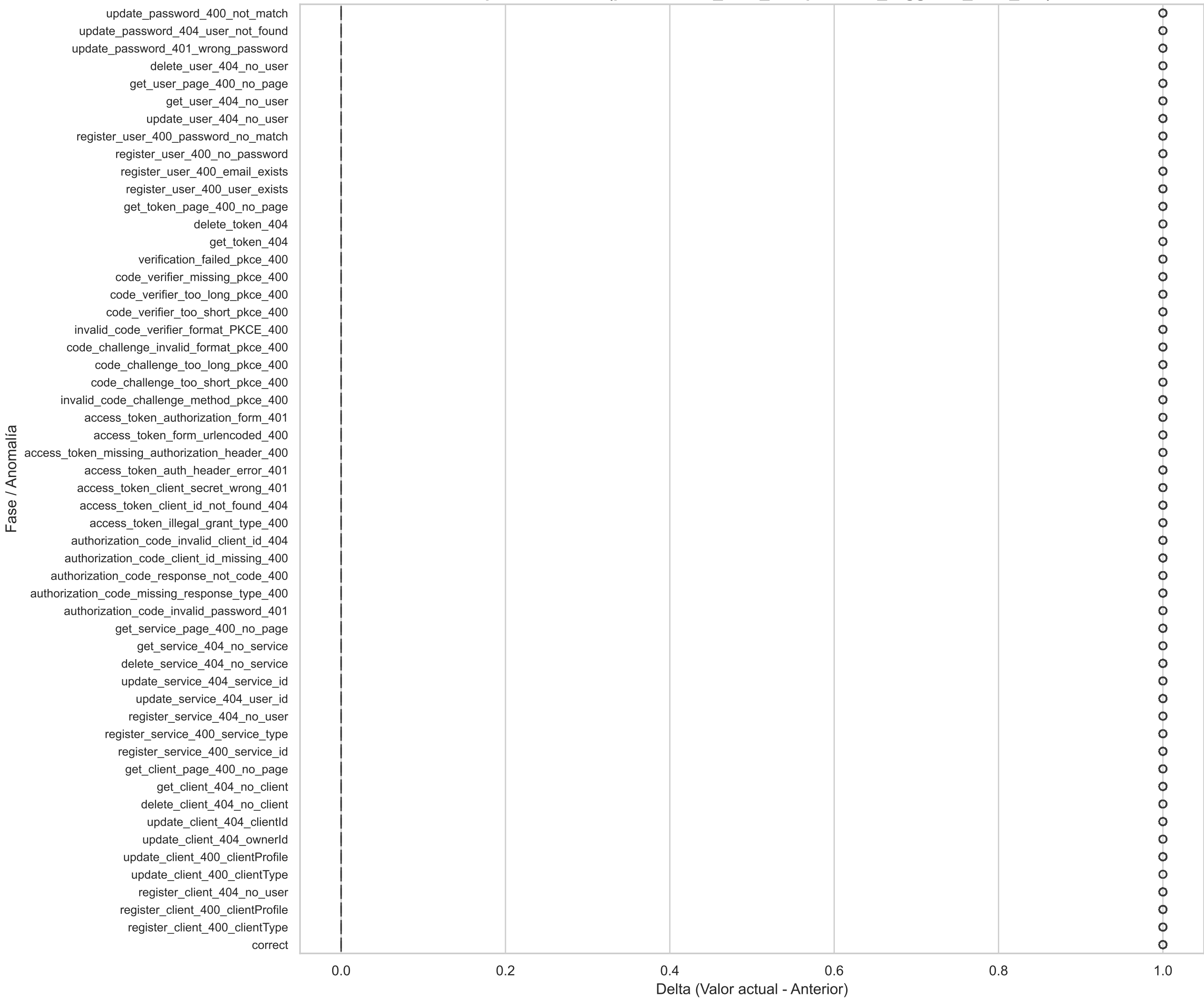
Boxplot Horizontal(prometheus_tsdb_compactions_triggered_total_diff)
