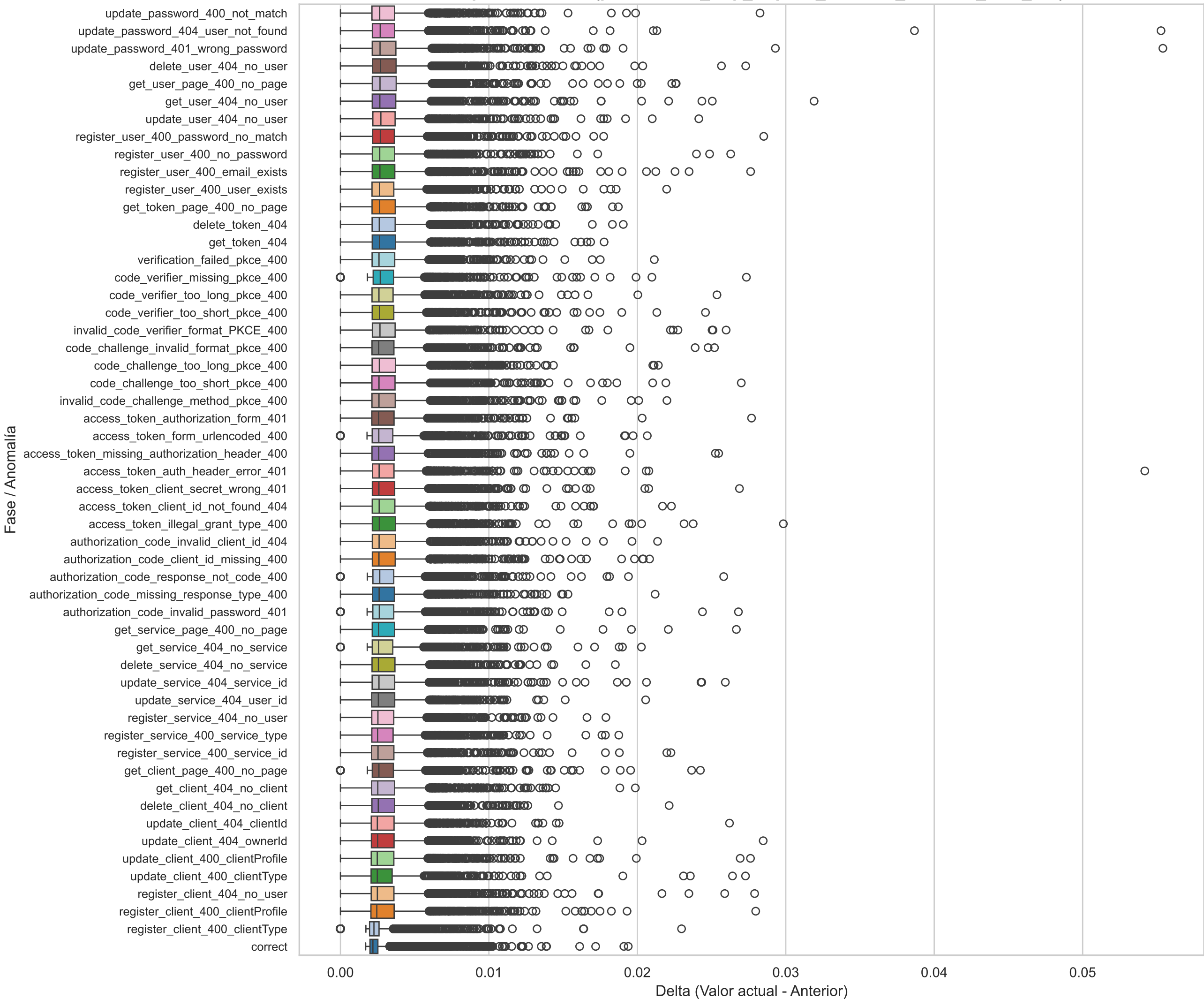
Boxplot Horizontal(prometheus_http_request_duration_seconds_sum_diff)
