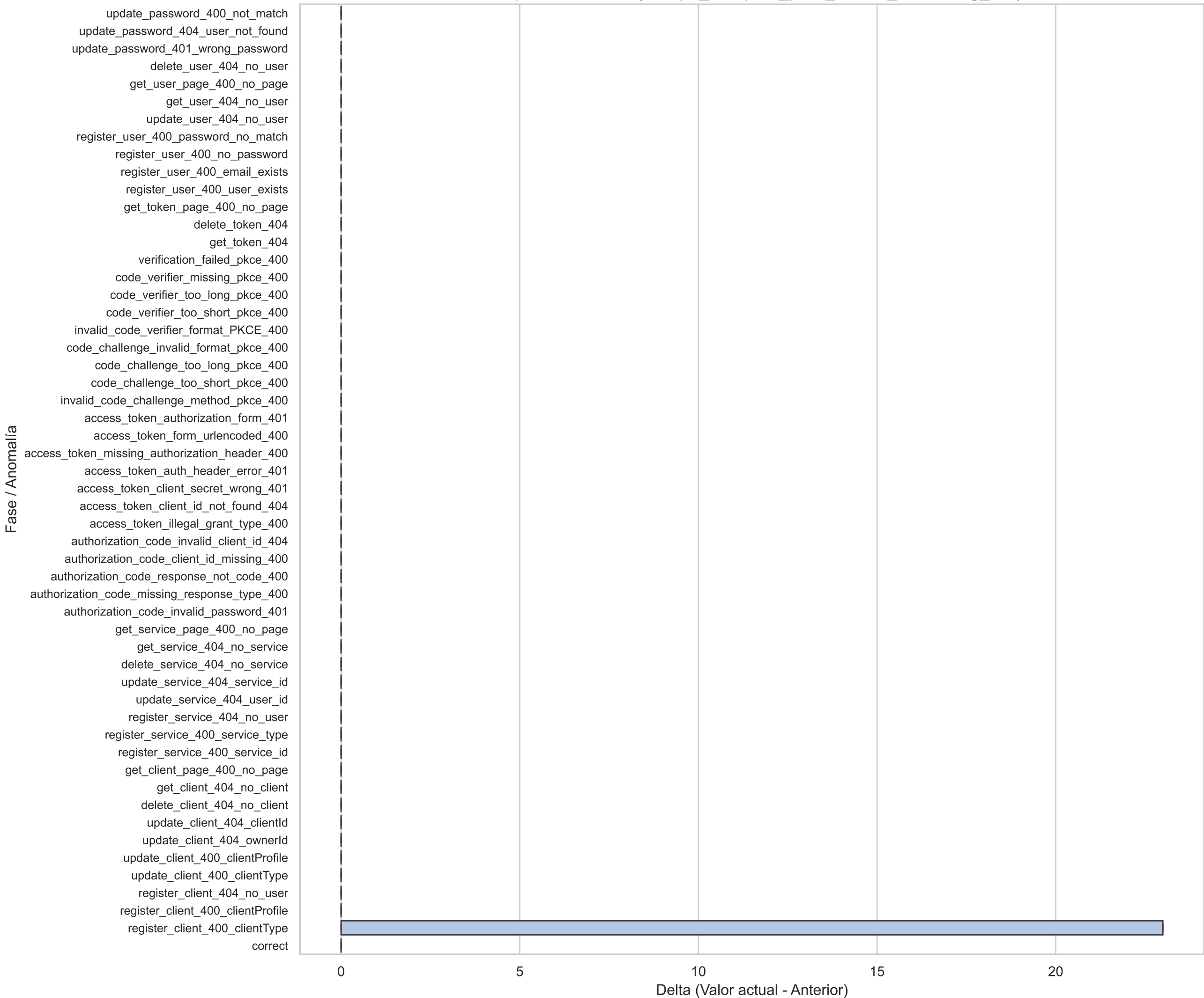
Boxplot Horizontal(scrape_samples_post_metric_relabeling_diff)
