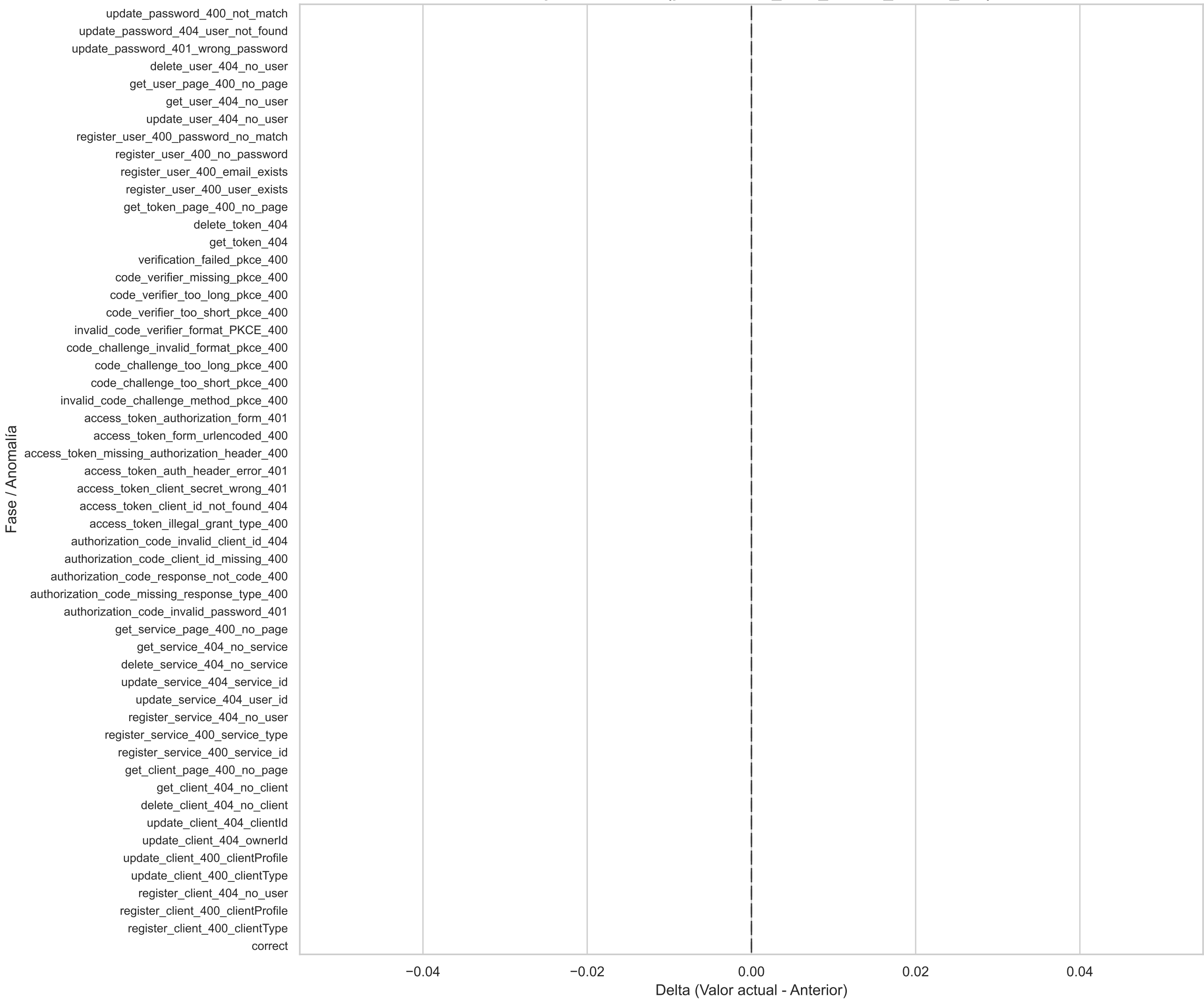
Boxplot Horizontal(prometheus_tsdb_blocks_loaded_diff)
