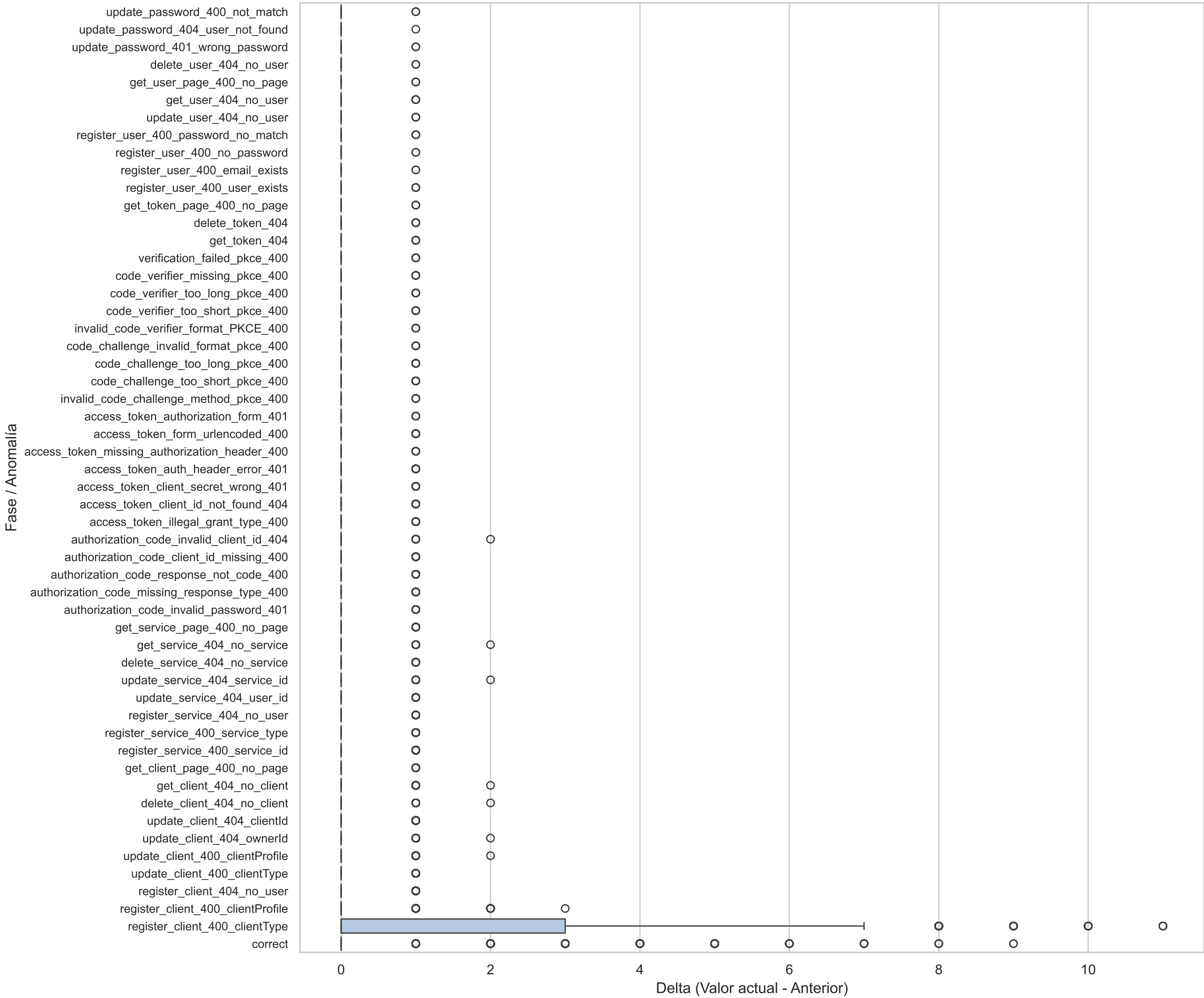
Boxplot Horizontal(go_threads_diff)
