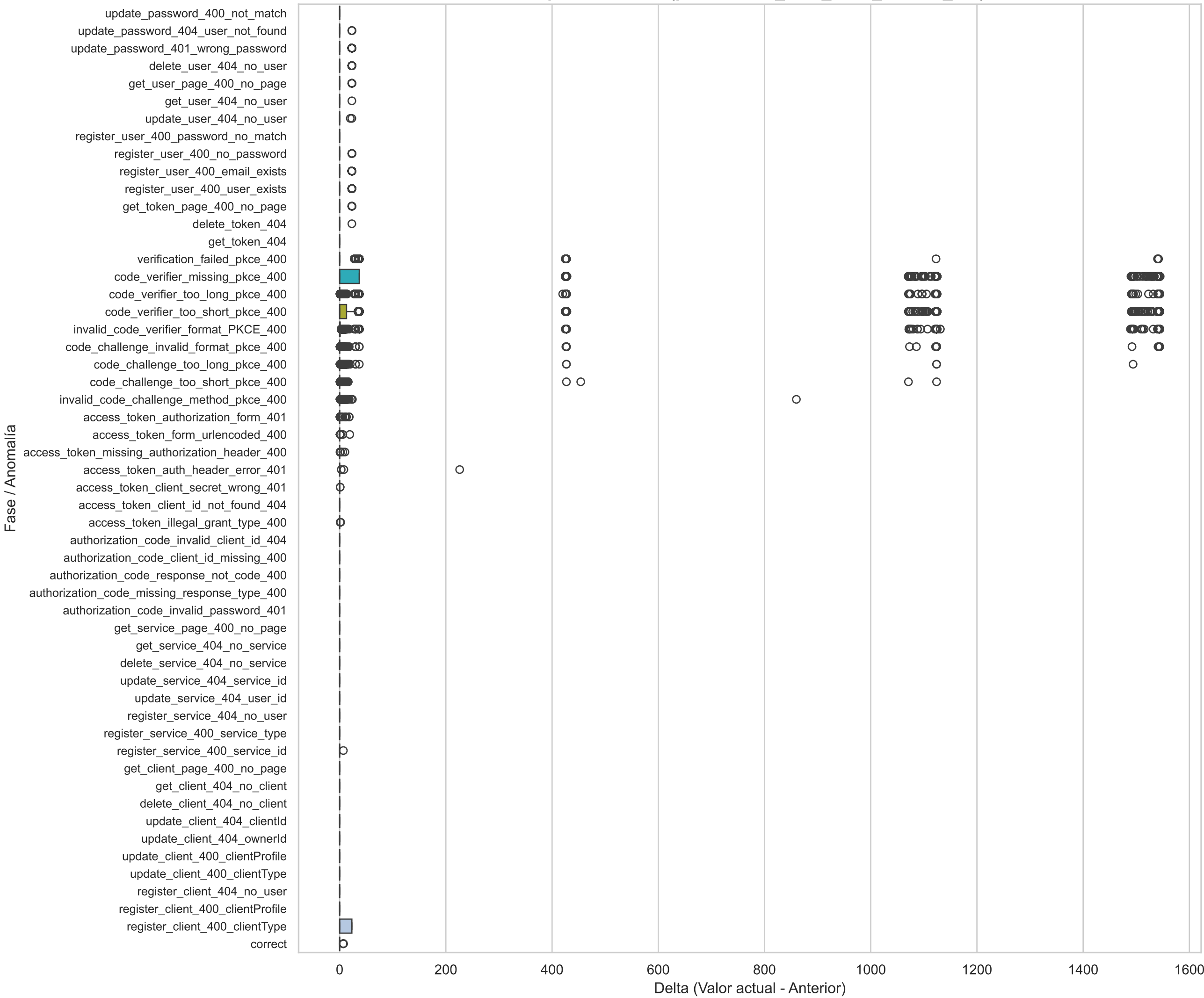
Boxplot Horizontal(prometheus_tsdb_head_chunks_diff)
