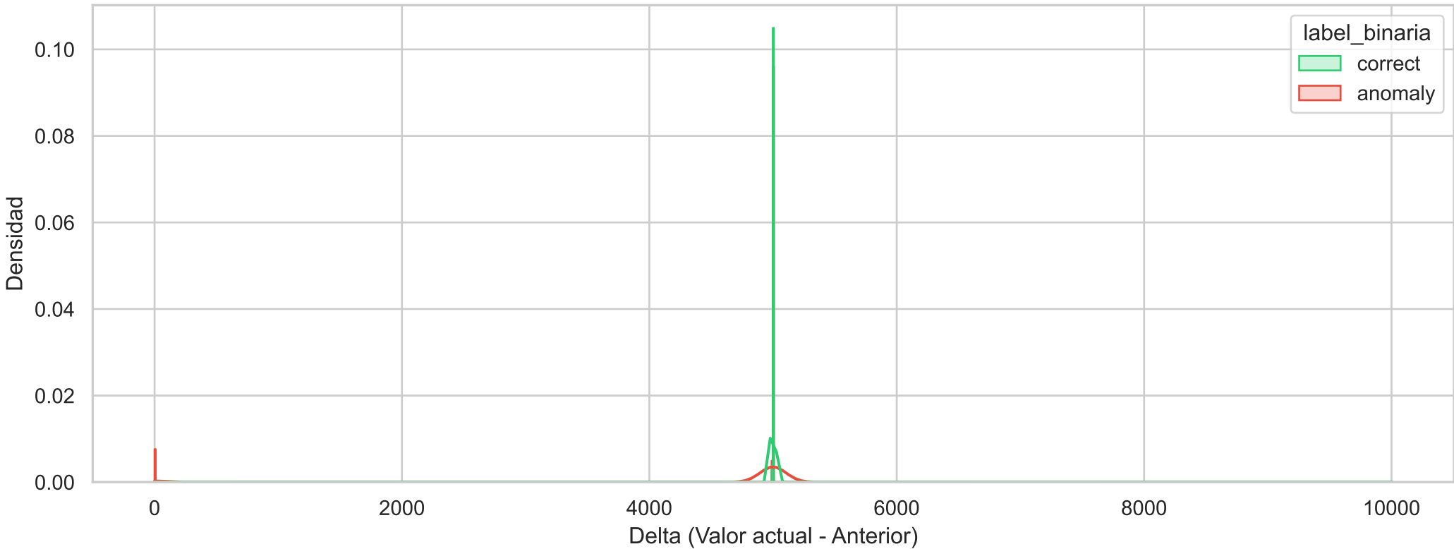
Histograma de Densidad Binario (prometheus_tsdb_head_max_time_diff)
