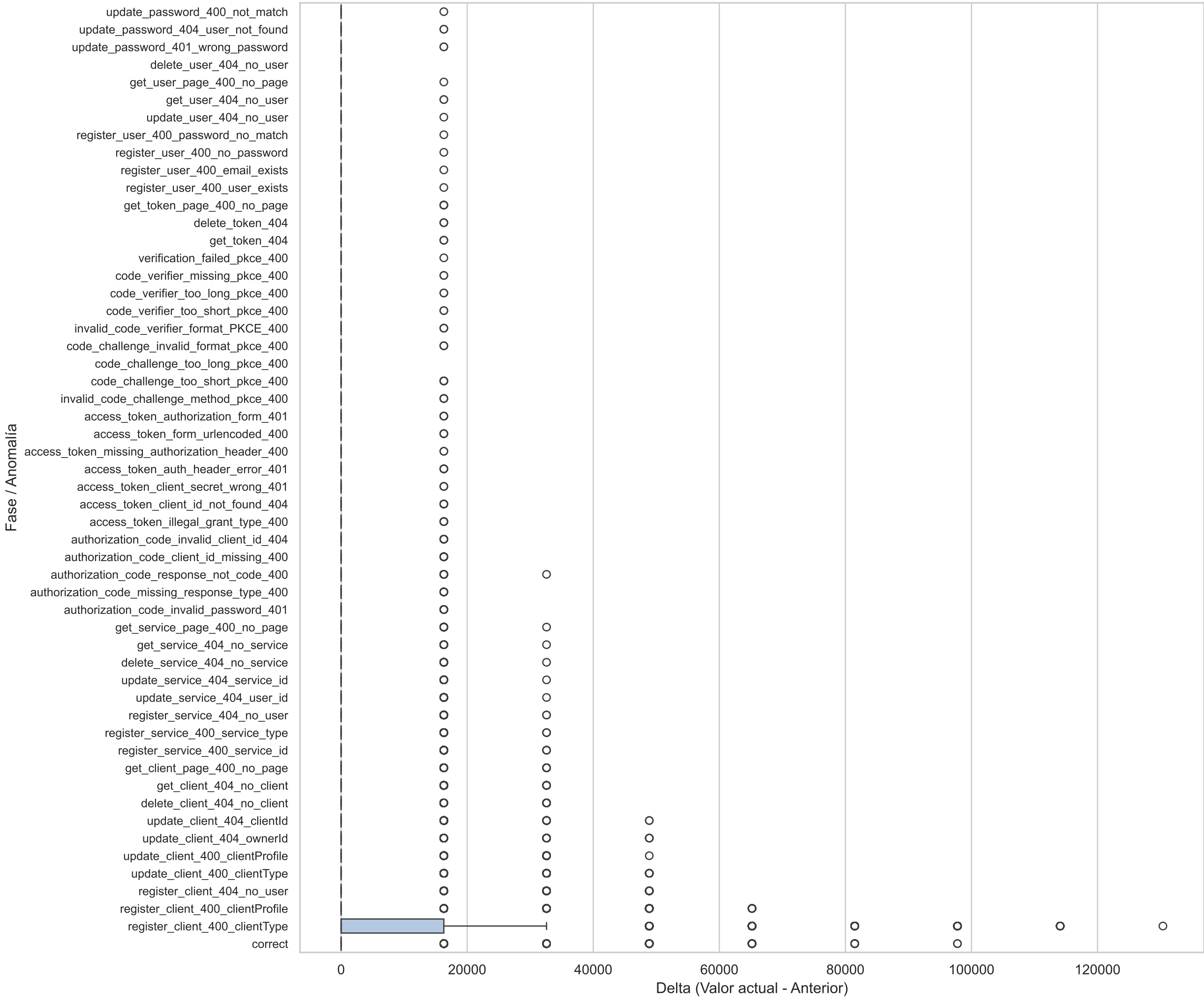
Boxplot Horizontal(go_memstats_mspan_sys_bytes_diff)
