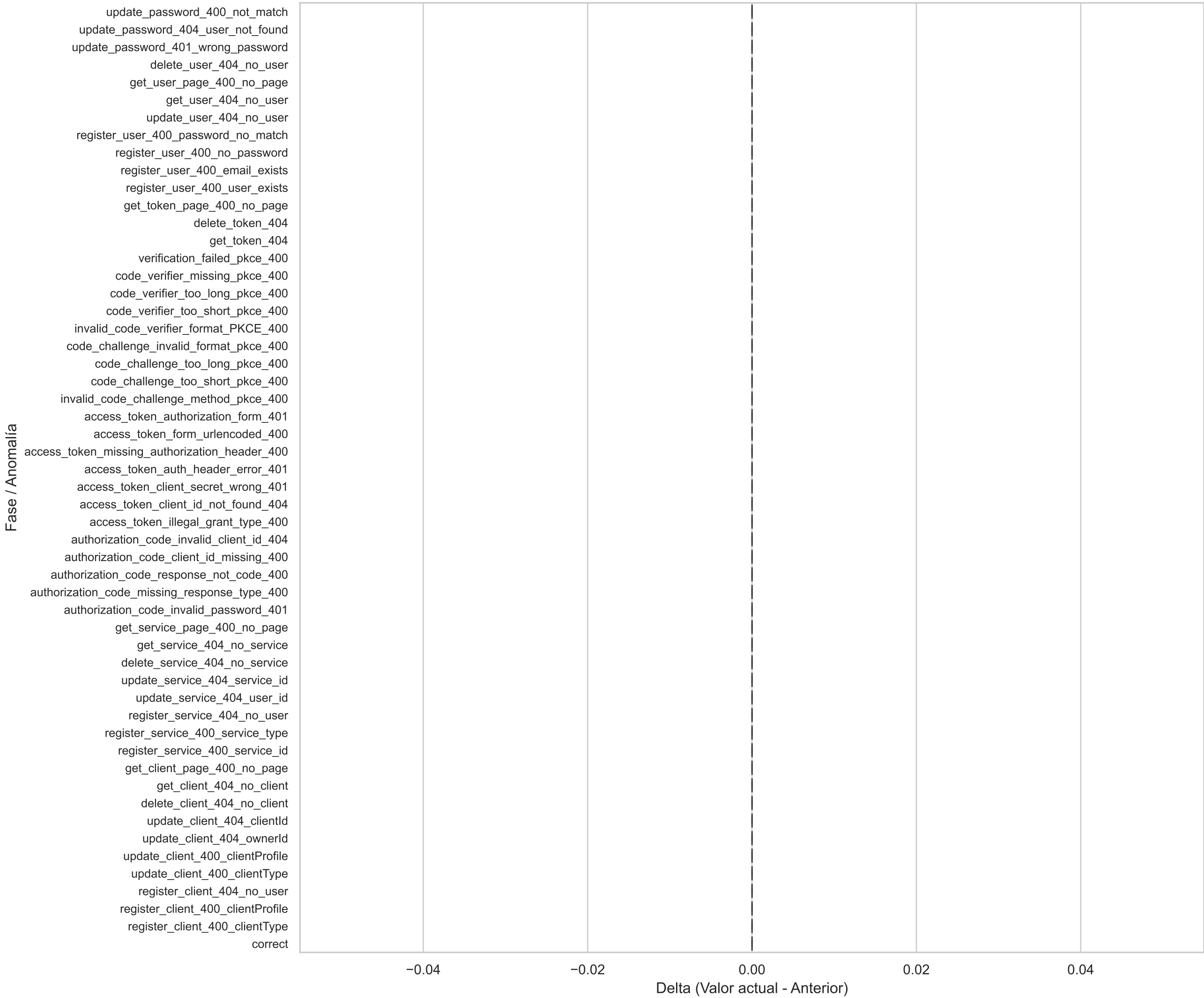
Boxplot Horizontal(prometheus_tsdb_symbol_table_size_bytes_diff)
