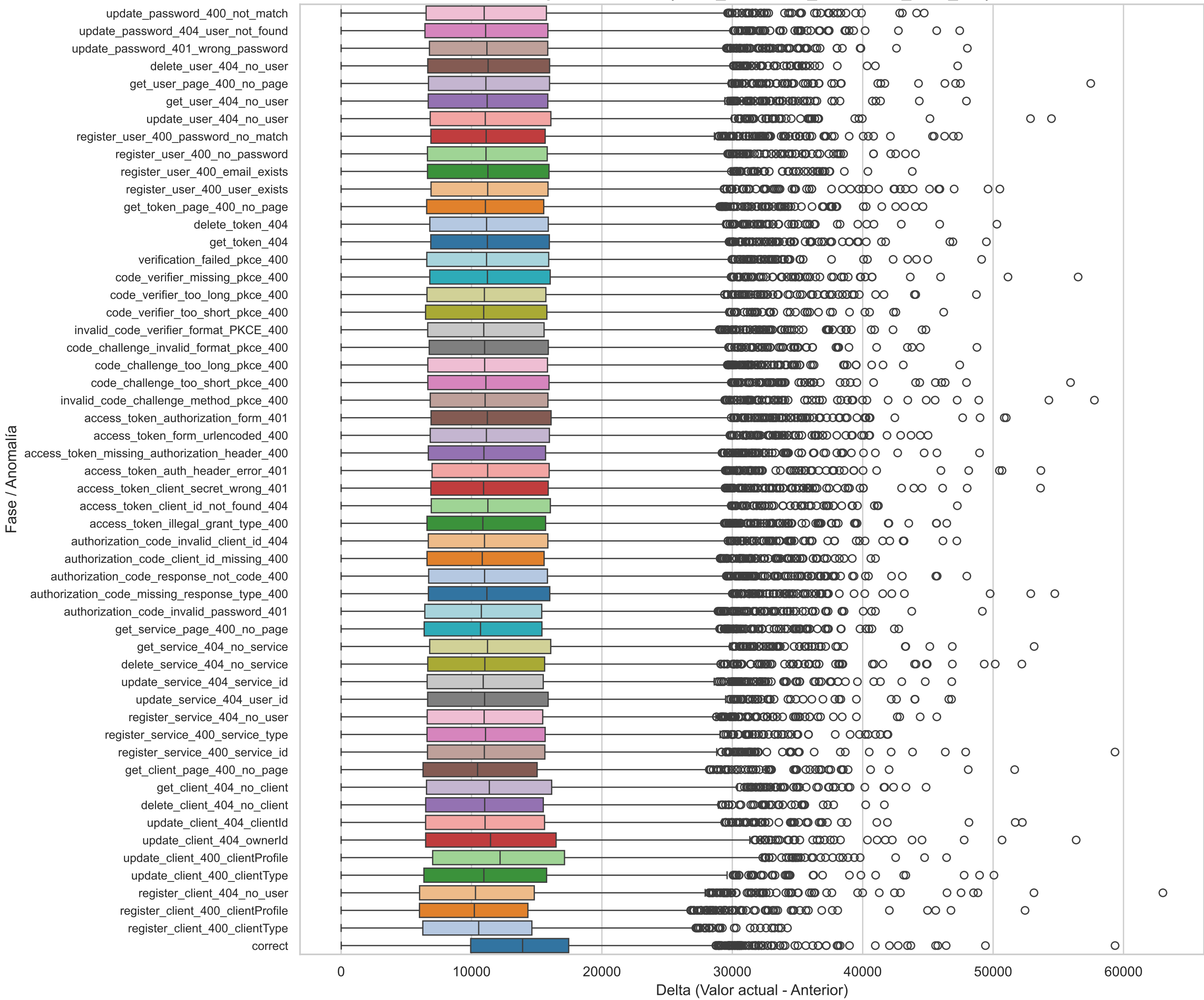
Boxplot Horizontal(node_schedstat_timeslices_total_diff)
