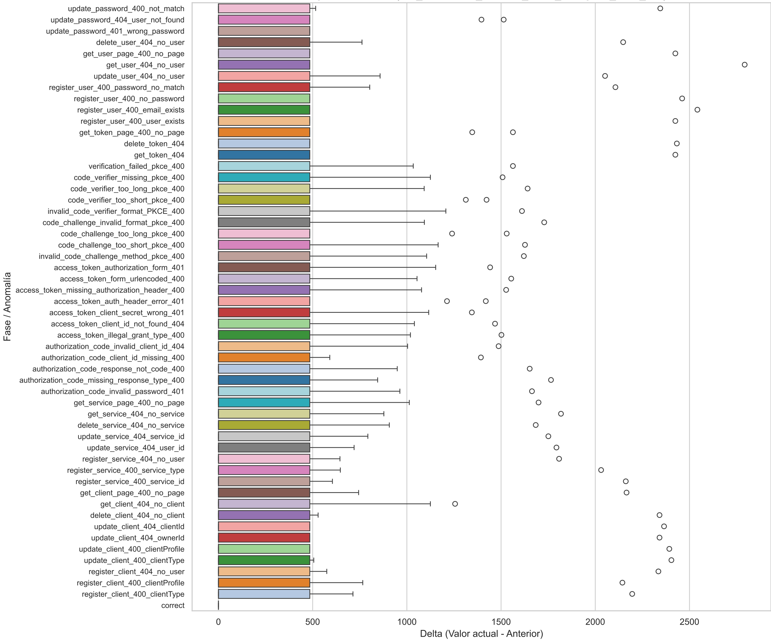
Boxplot Horizontal(net_contrack_listener_conn_accepted_total_diff)
