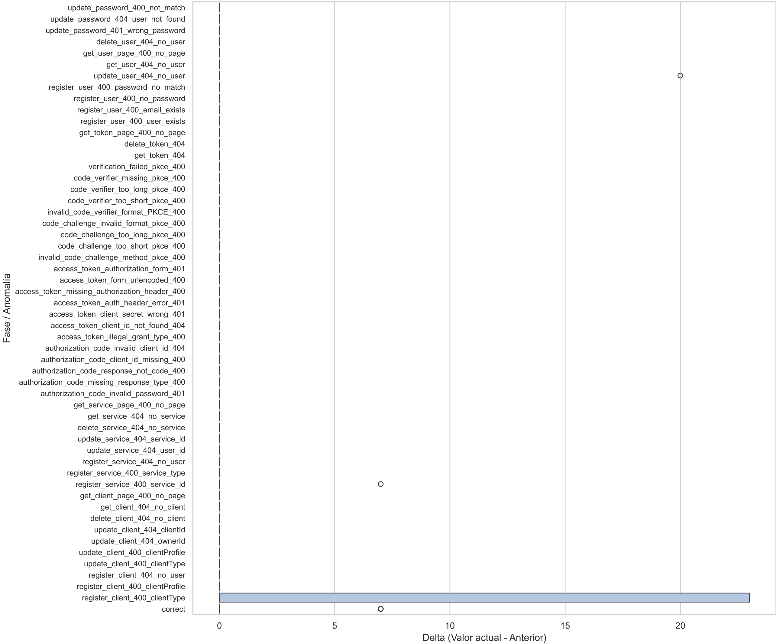
Boxplot Horizontal(prometheus_tsdb_head_series_created_total_diff)
