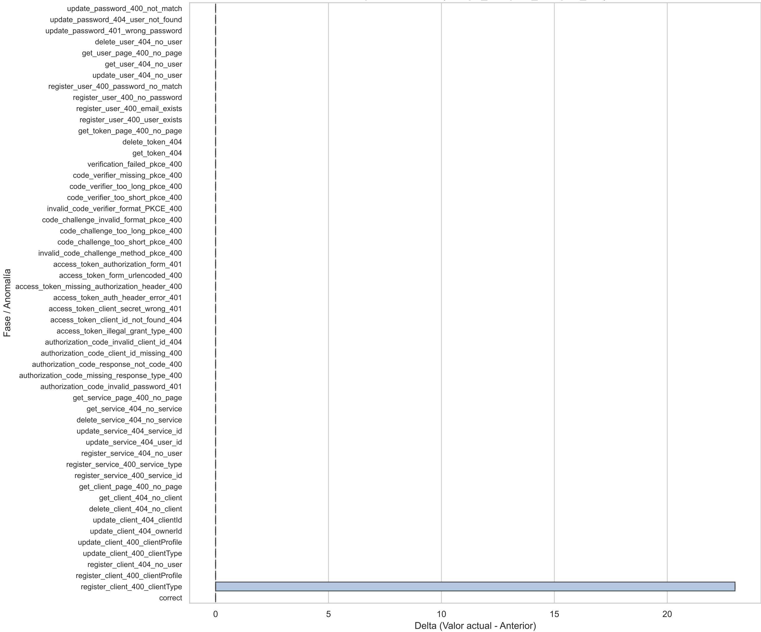
Boxplot Horizontal(scrape_samples_scraped_diff)
