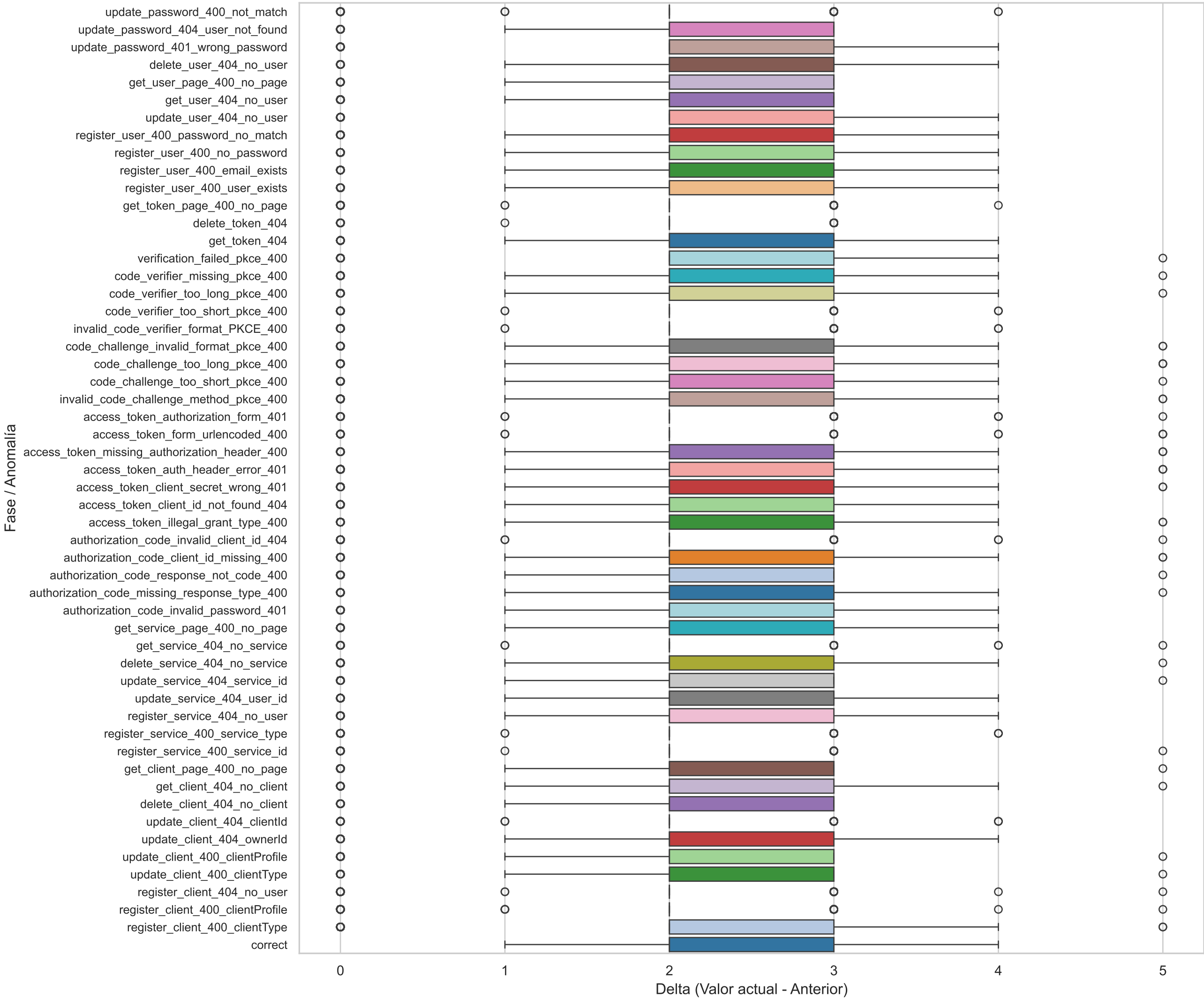
Boxplot Horizontal(prometheus_tsdb_wal_page_flushes_total_diff)
