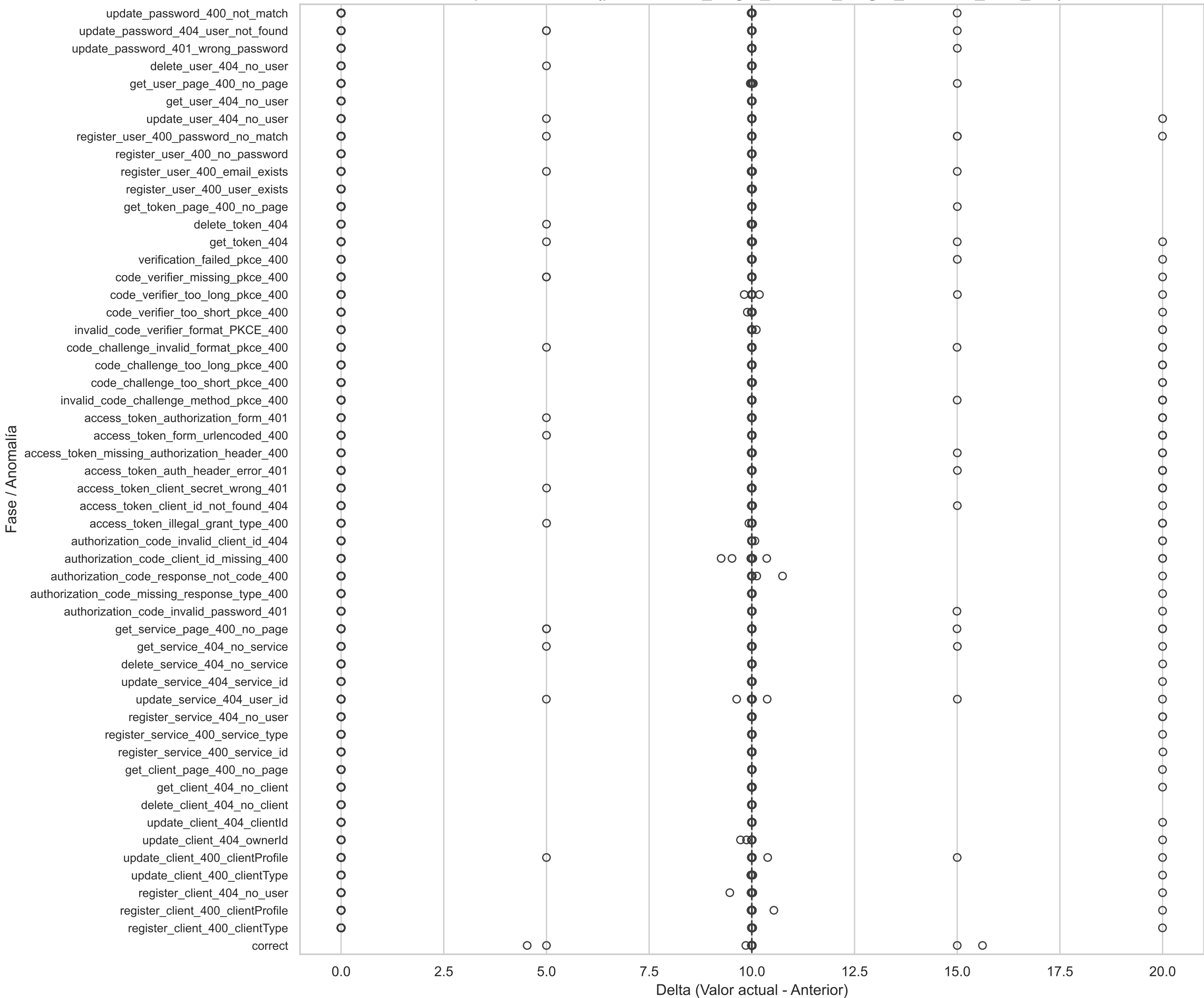
Boxplot Horizontal(prometheus_target_interval_length_seconds_sum_diff)
