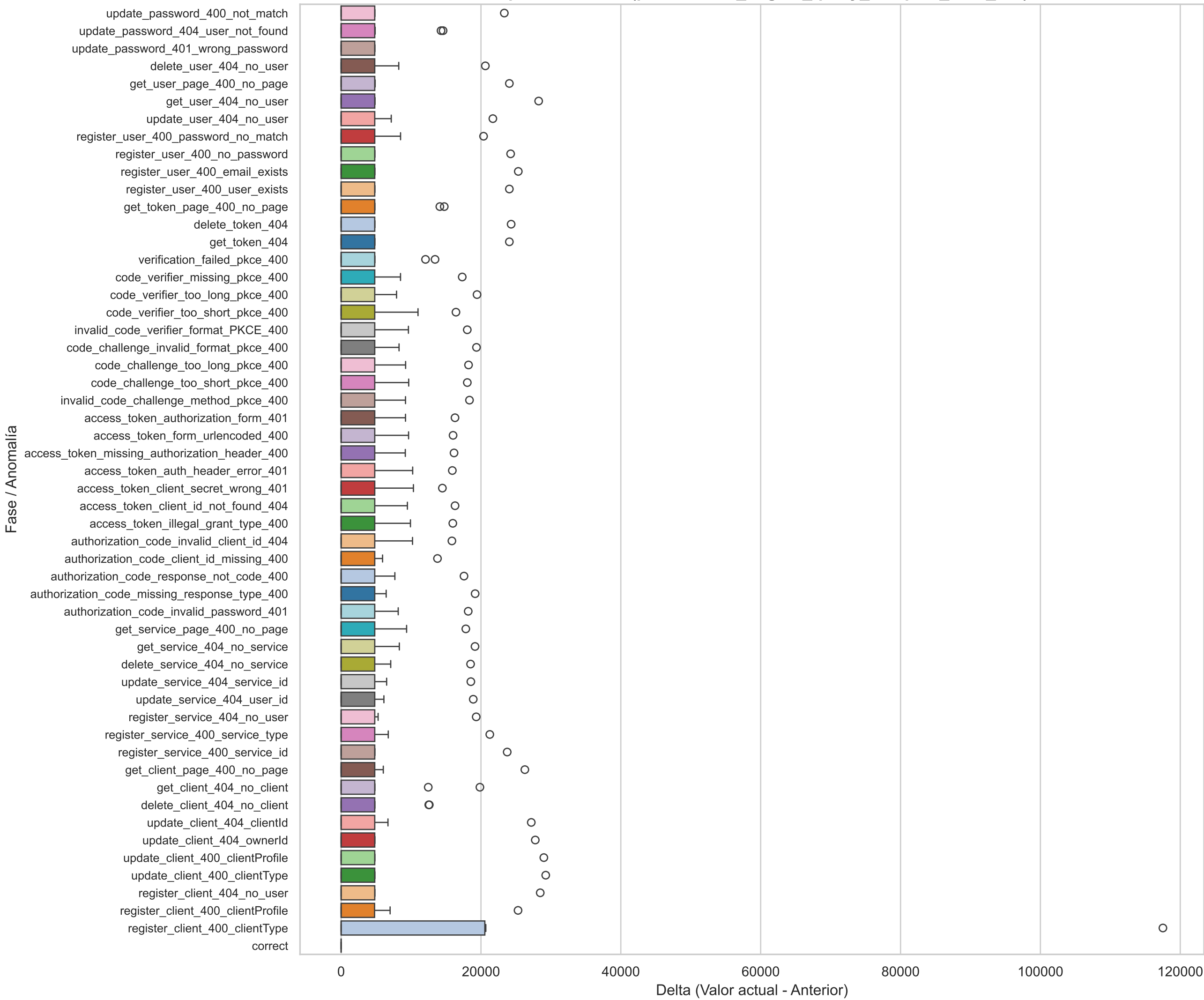
Boxplot Horizontal(prometheus_engine_query_samples_total_diff)
