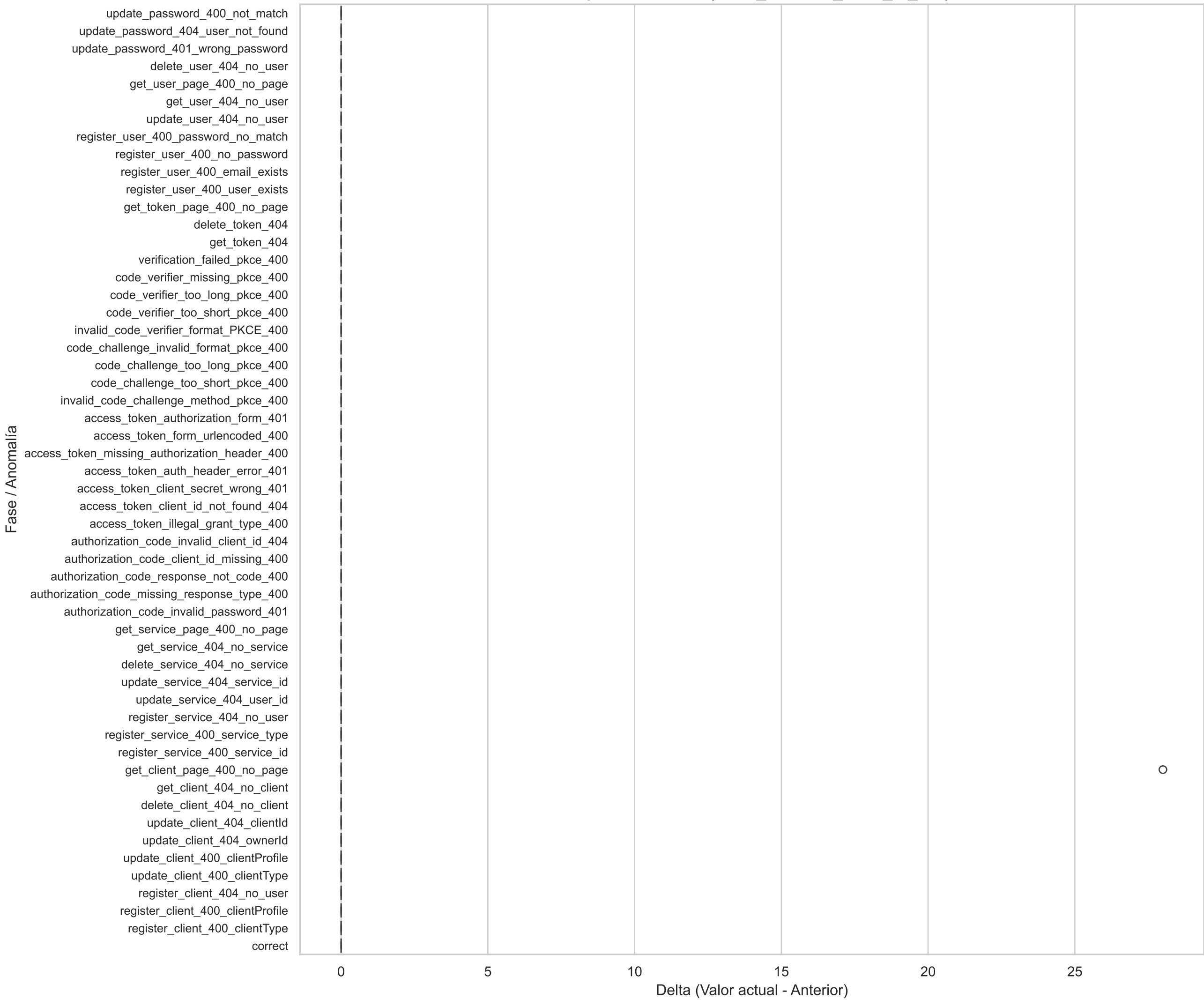
Boxplot Horizontal(node_network_iface_id_diff)
