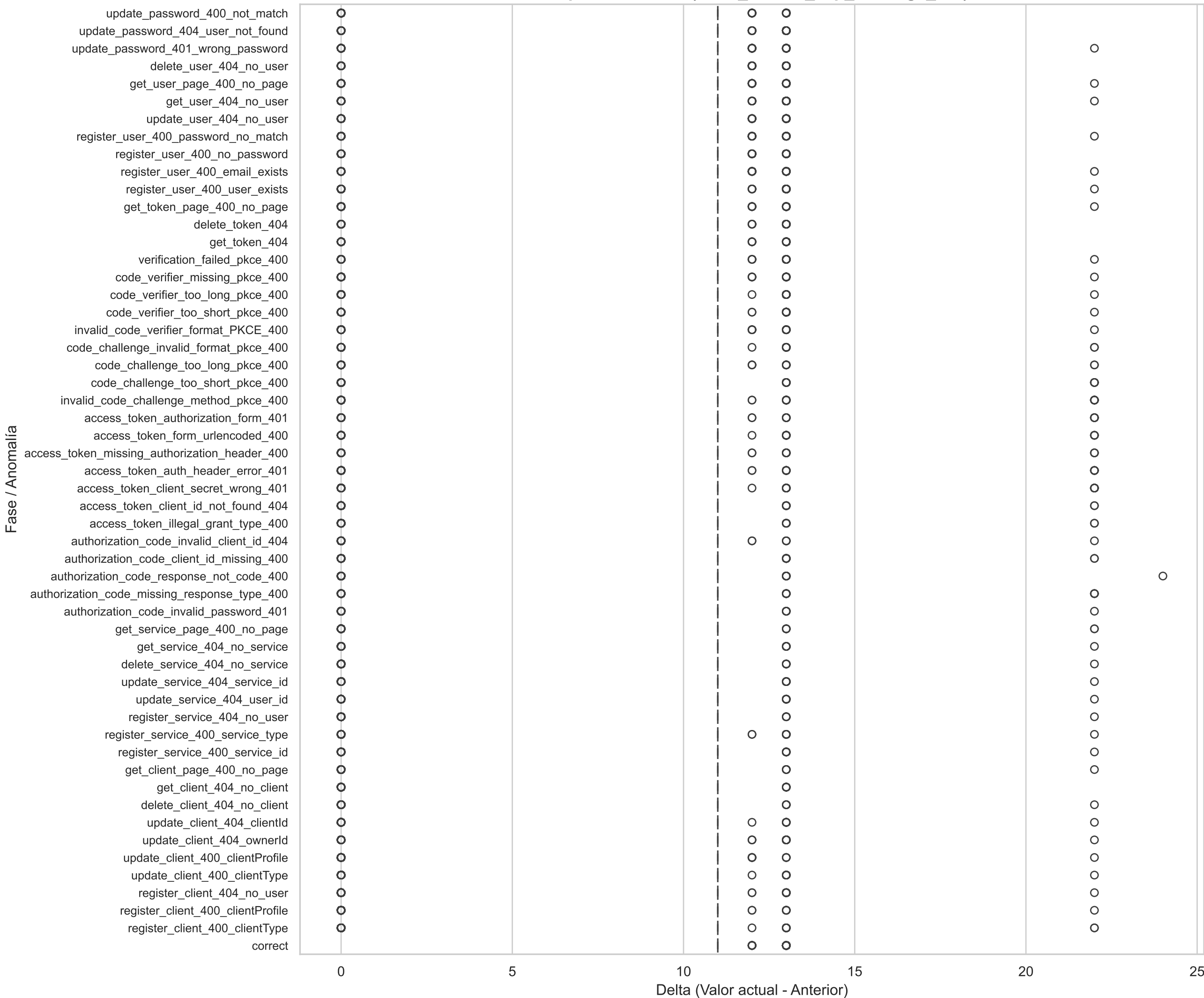
Boxplot Horizontal(node_netstat_Tcp_OutSegs_diff)
