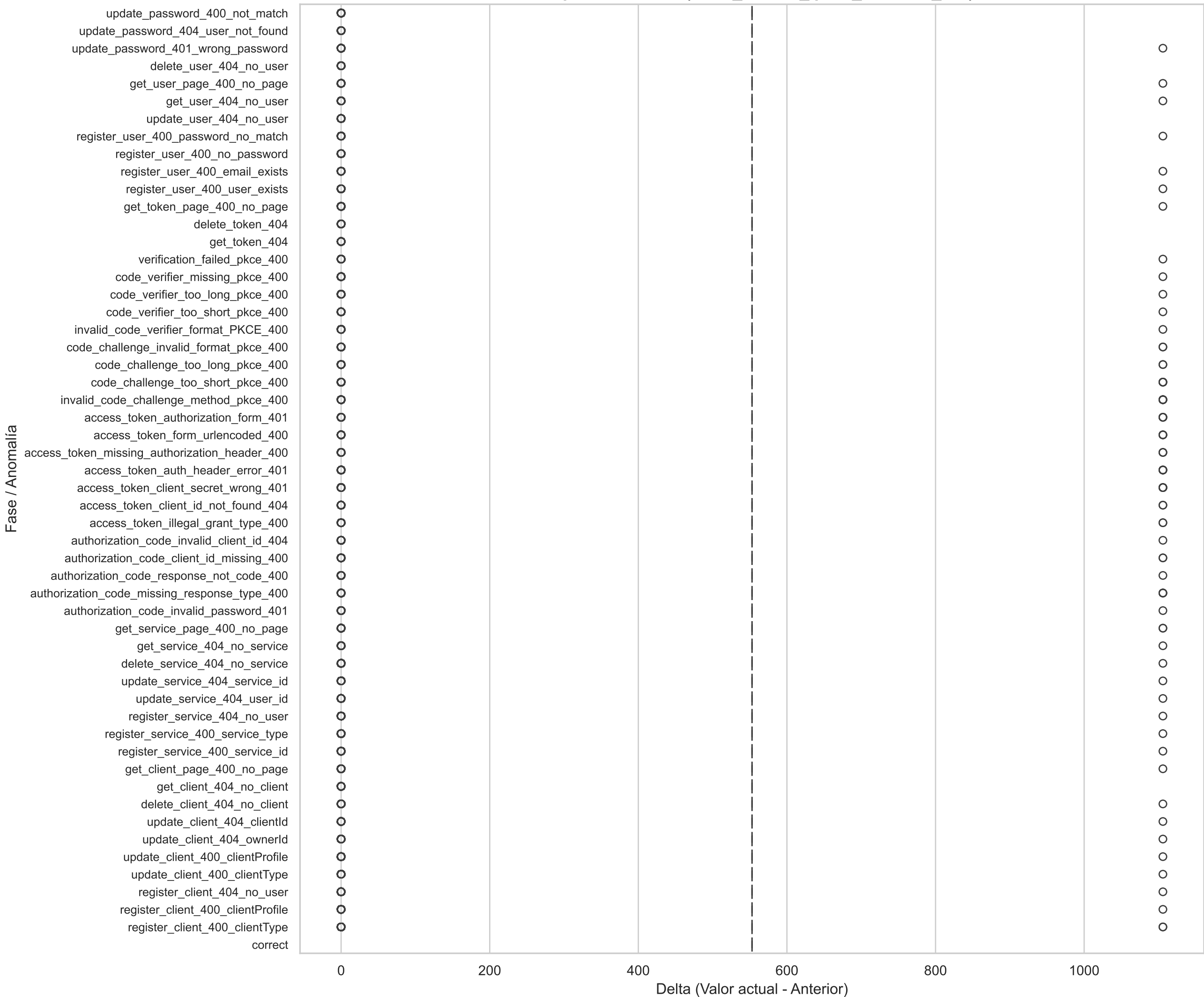
Boxplot Horizontal(node_netstat_IpExt_InOctets_diff)
