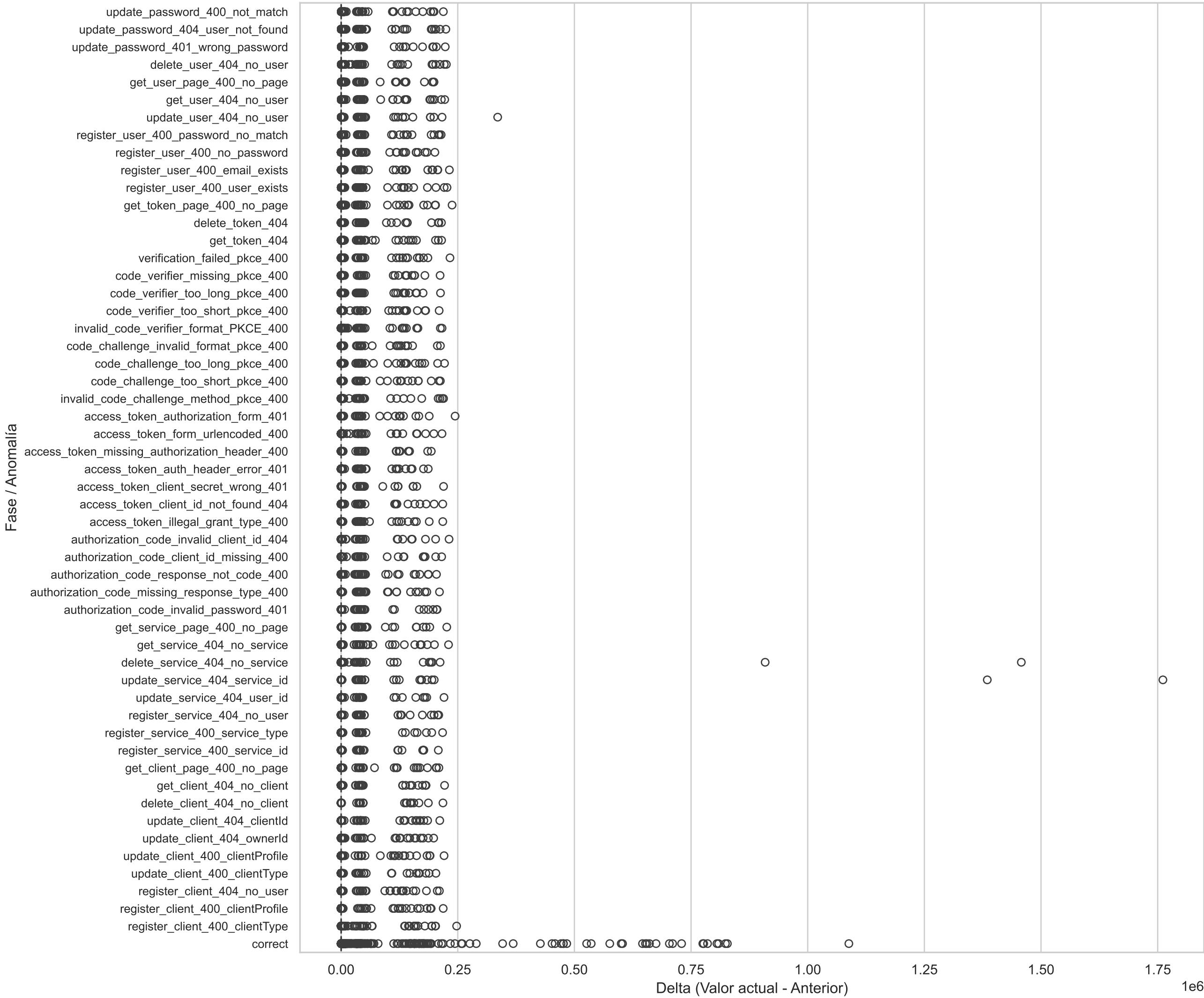
Boxplot Horizontal(node_vmstat_pgpgin_diff)
