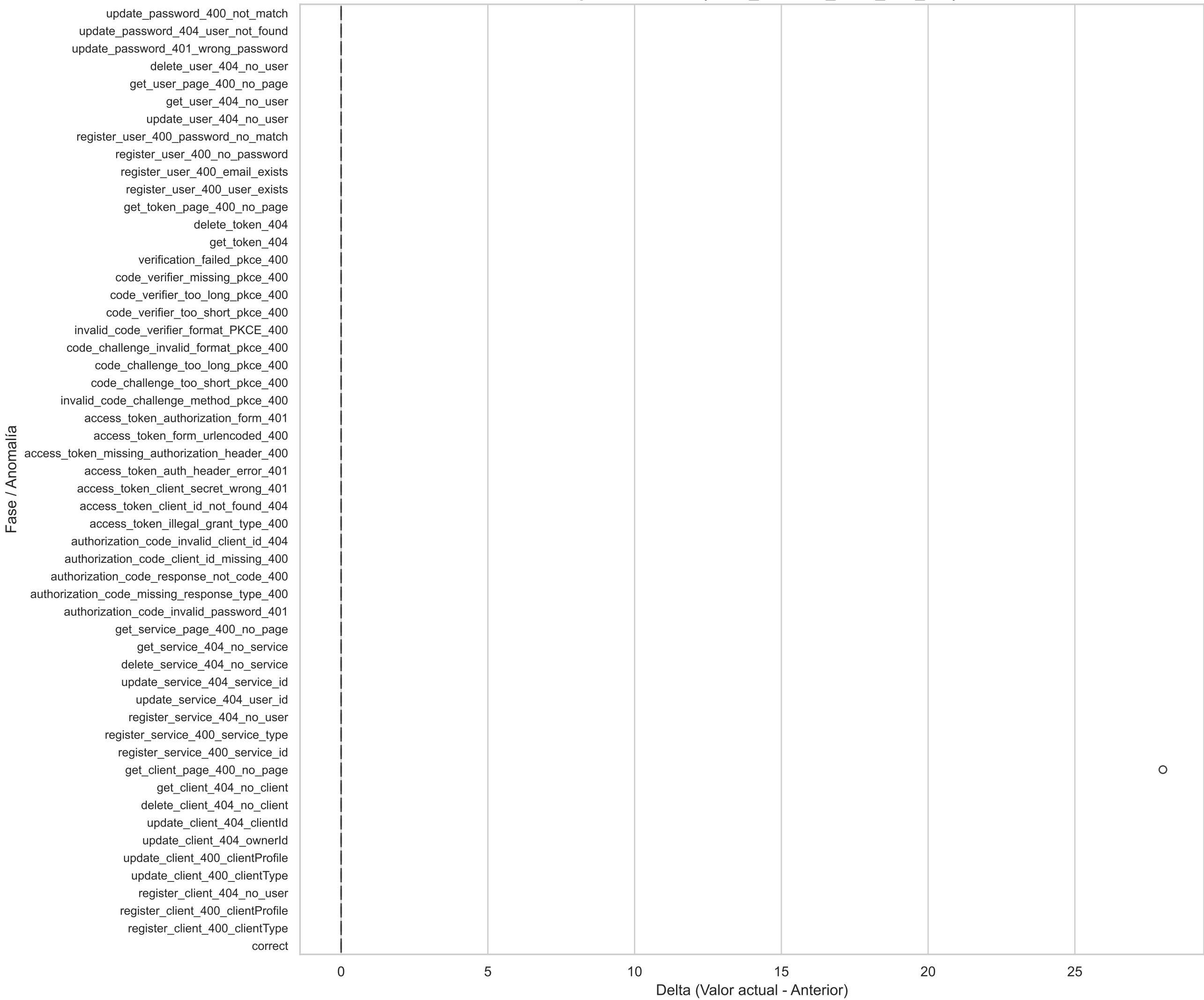
Boxplot Horizontal(node_network_iface_link_diff)
