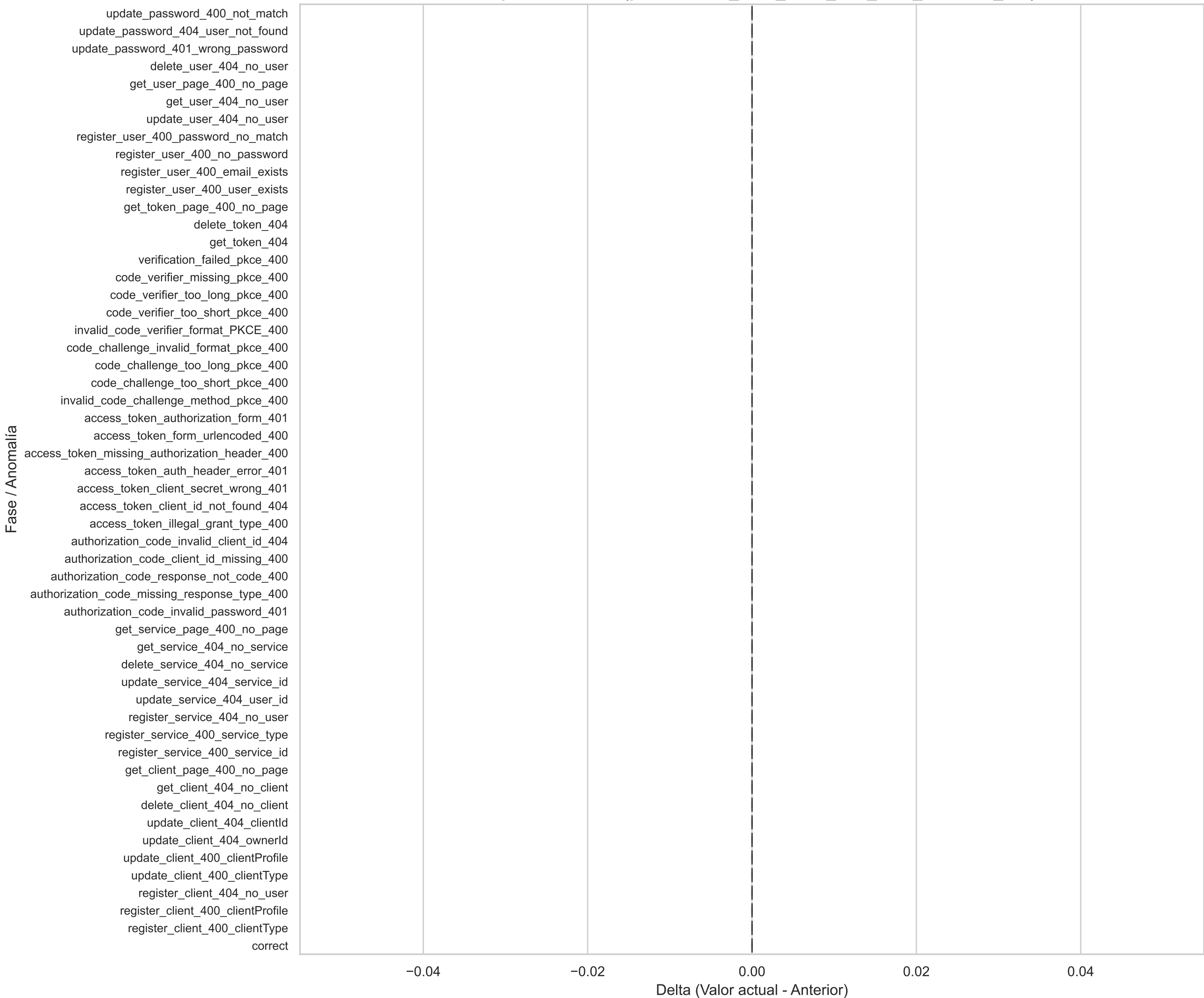
Boxplot Horizontal(prometheus_tsdb_head_min_time_seconds_diff)
