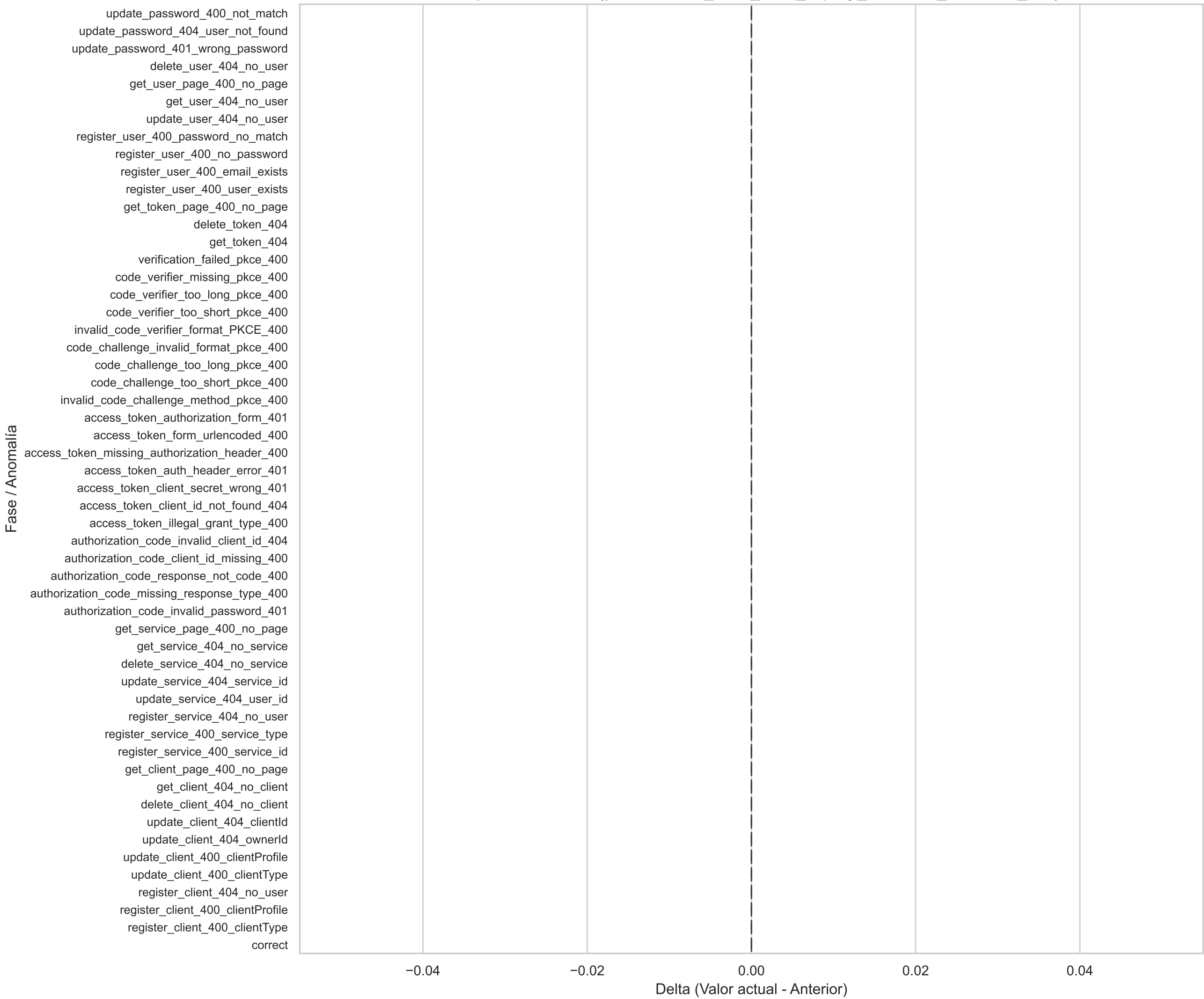
Boxplot Horizontal(prometheus_tsdb_data_replay_duration_seconds_diff)
