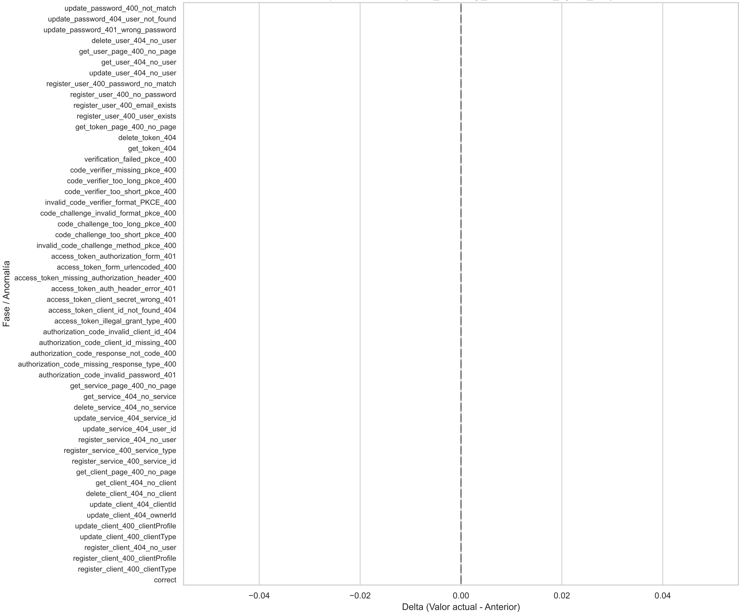
Boxplot Horizontal(node_memory_VmallocTotal_bytes_diff)
