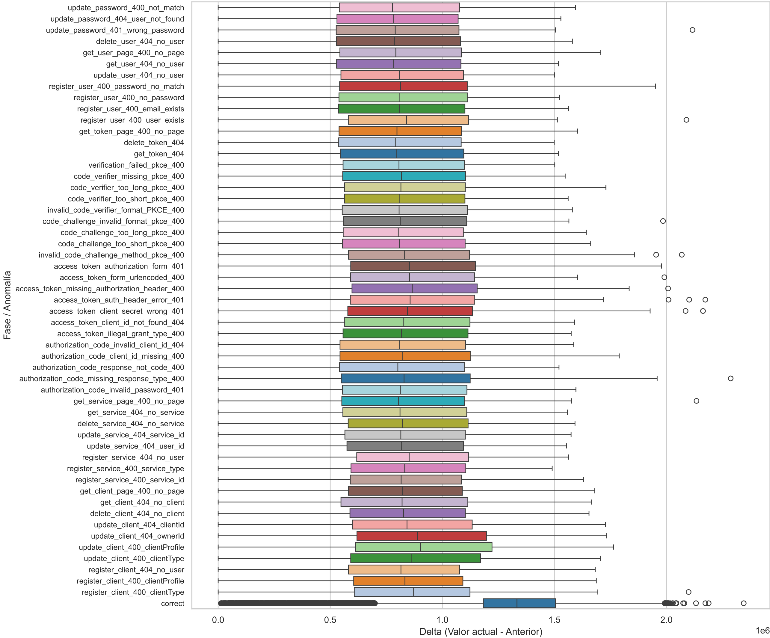
Boxplot Horizontal(node_vmstat_pgfault_diff)
