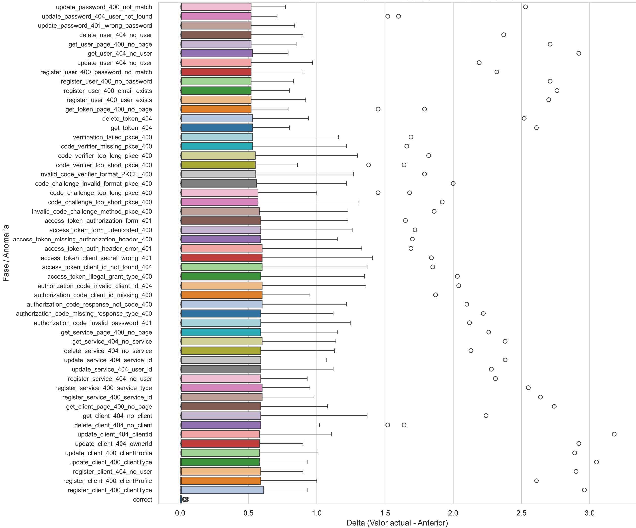
Boxplot Horizontal(process_cpu_seconds_total_diff)
