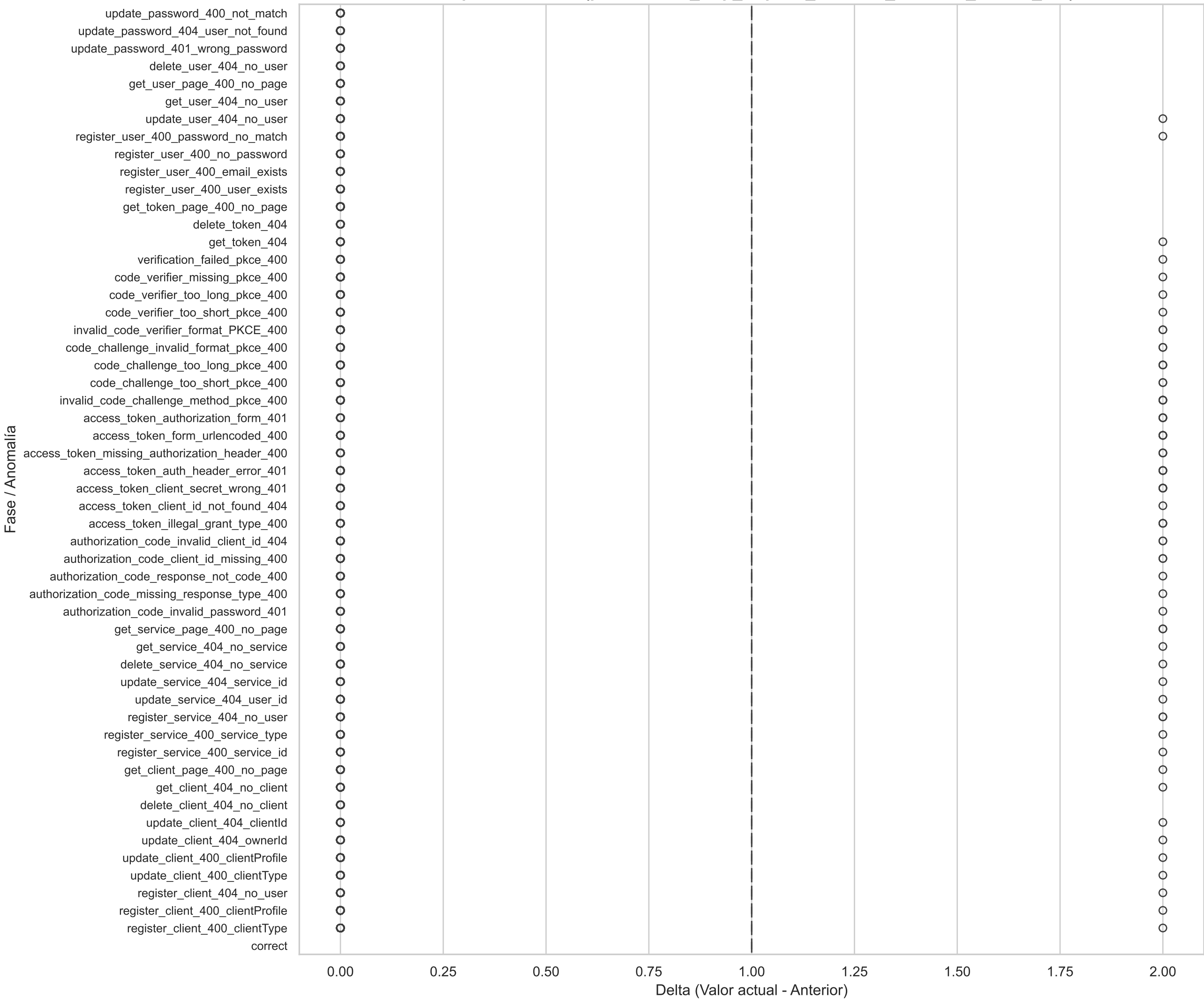
Boxplot Horizontal(prometheus_http_request_duration_seconds_bucket_diff)
