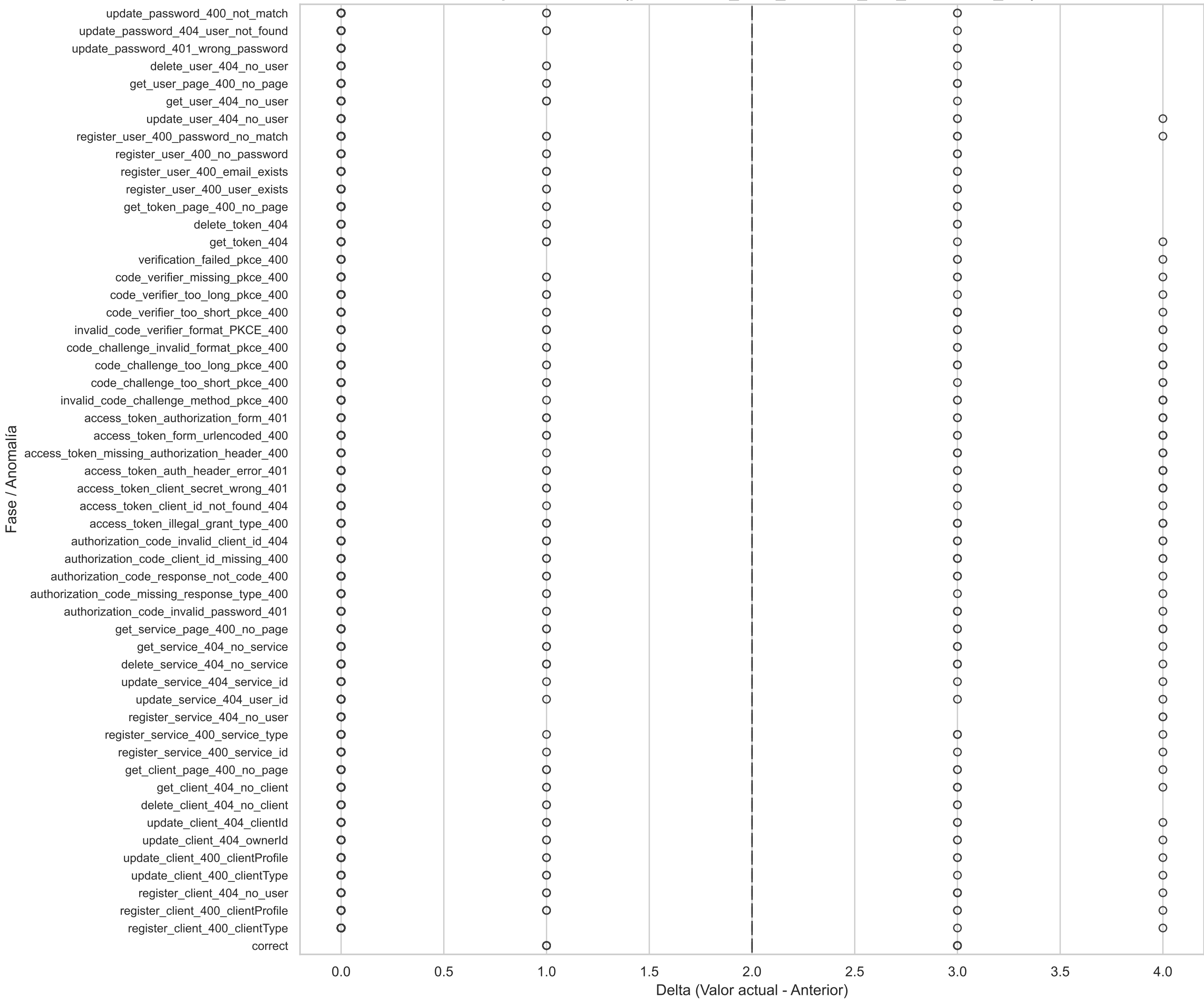
Boxplot Horizontal(prometheus_tsdb_isolation_low_watermark_diff)
