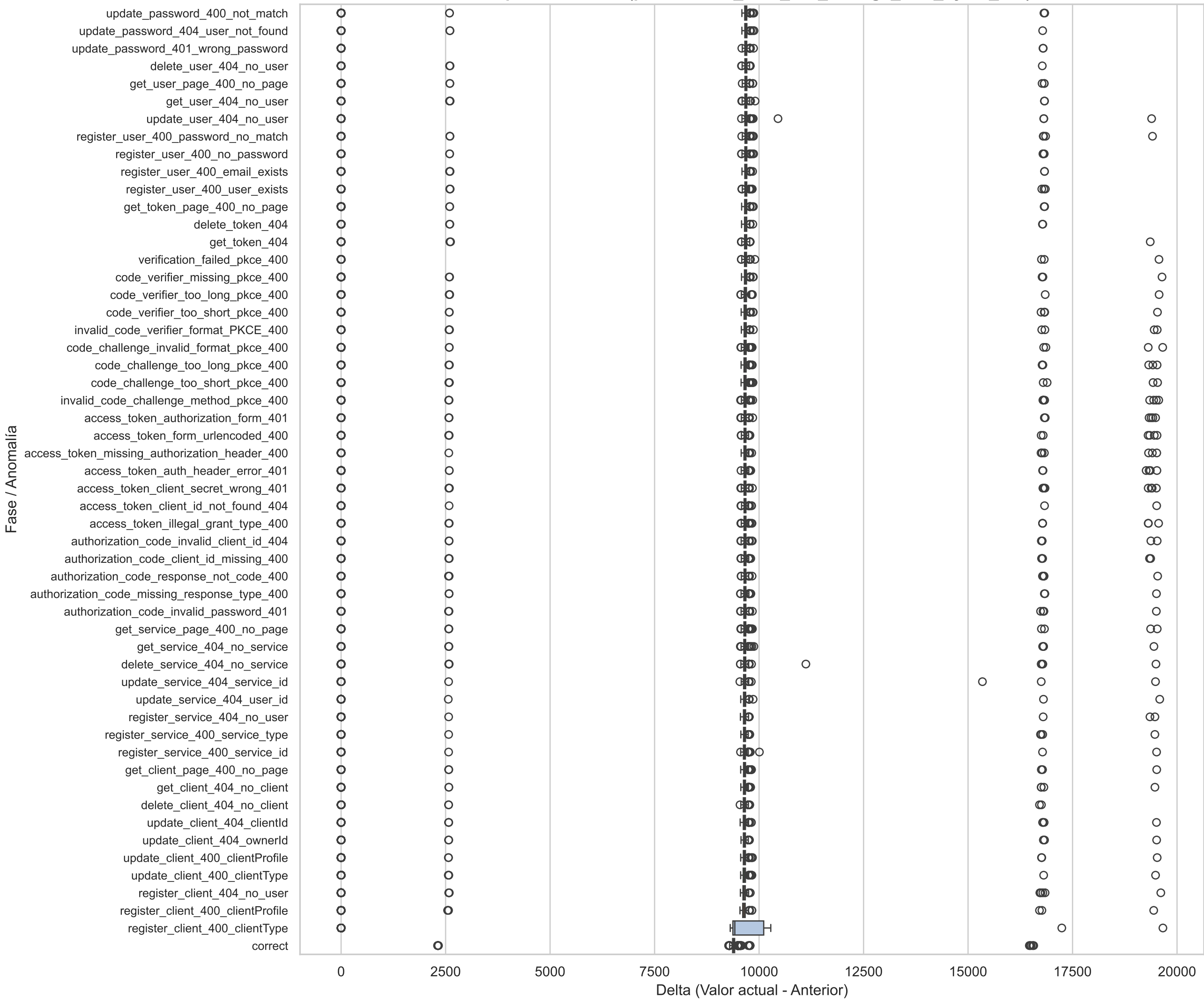
Boxplot Horizontal(prometheus_tsdb_wal_storage_size_bytes_diff)
