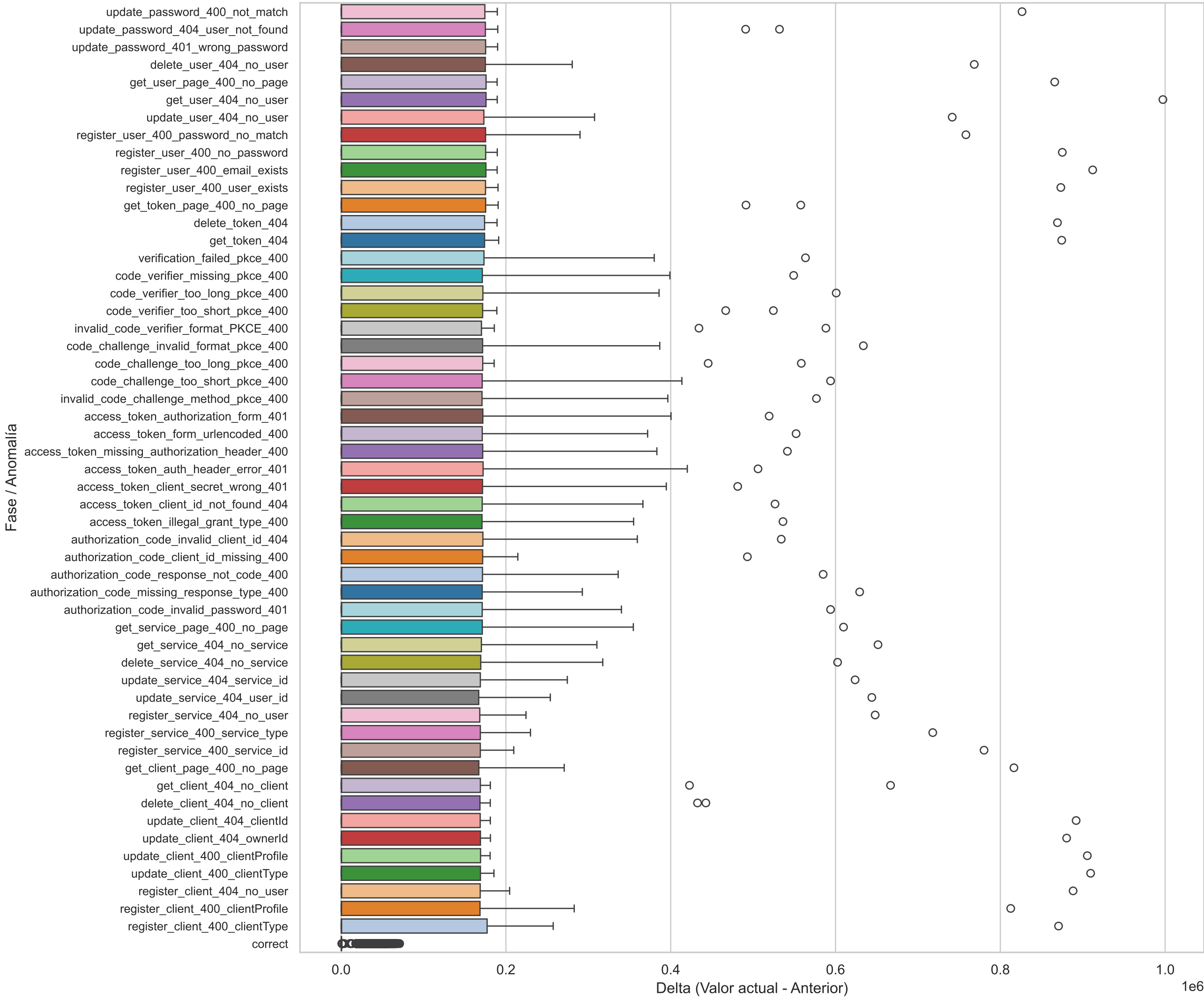
Boxplot Horizontal(go_memstats_frees_total_diff)
