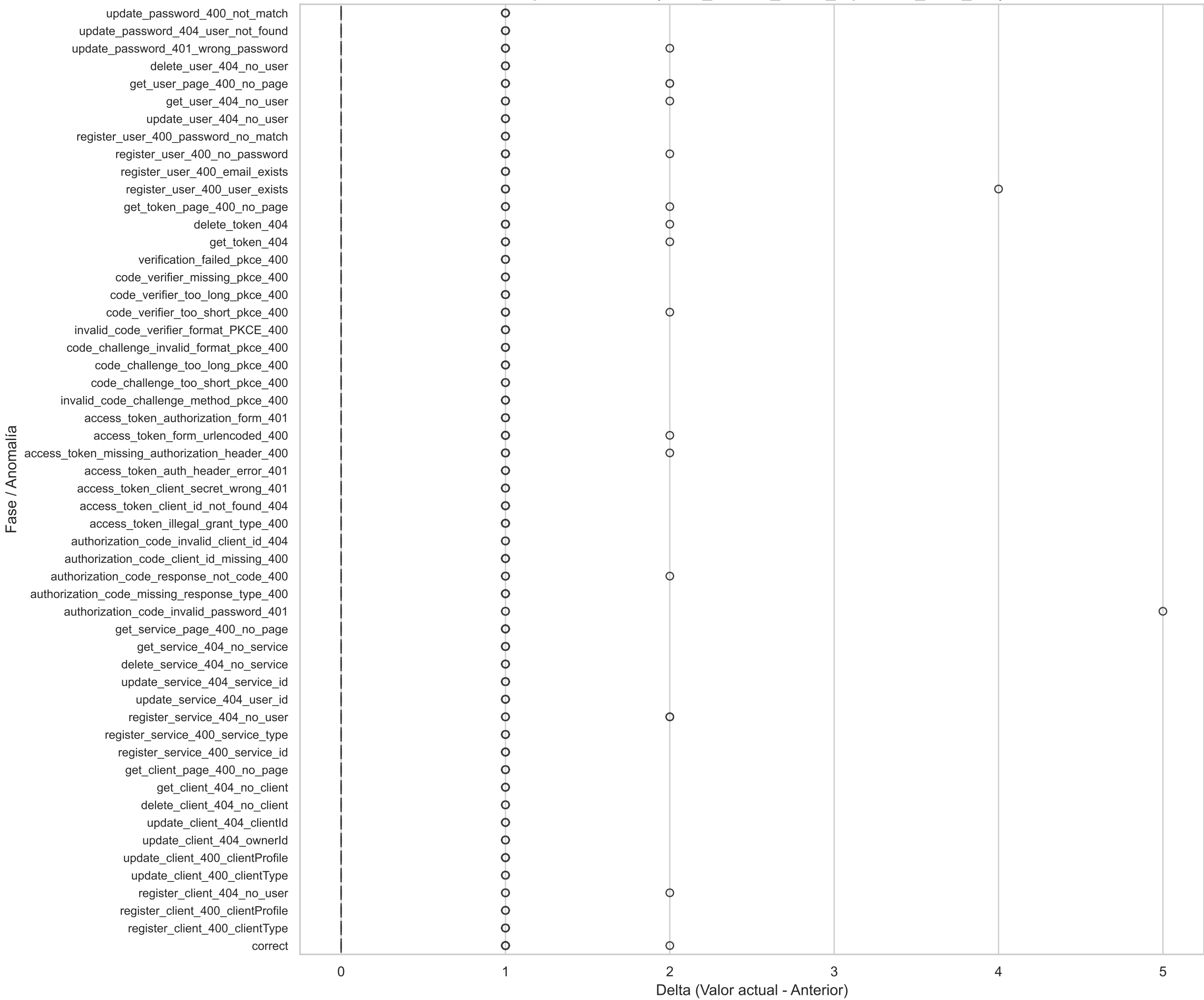
Boxplot Horizontal(node_softnet_times_squeezed_total_diff)
