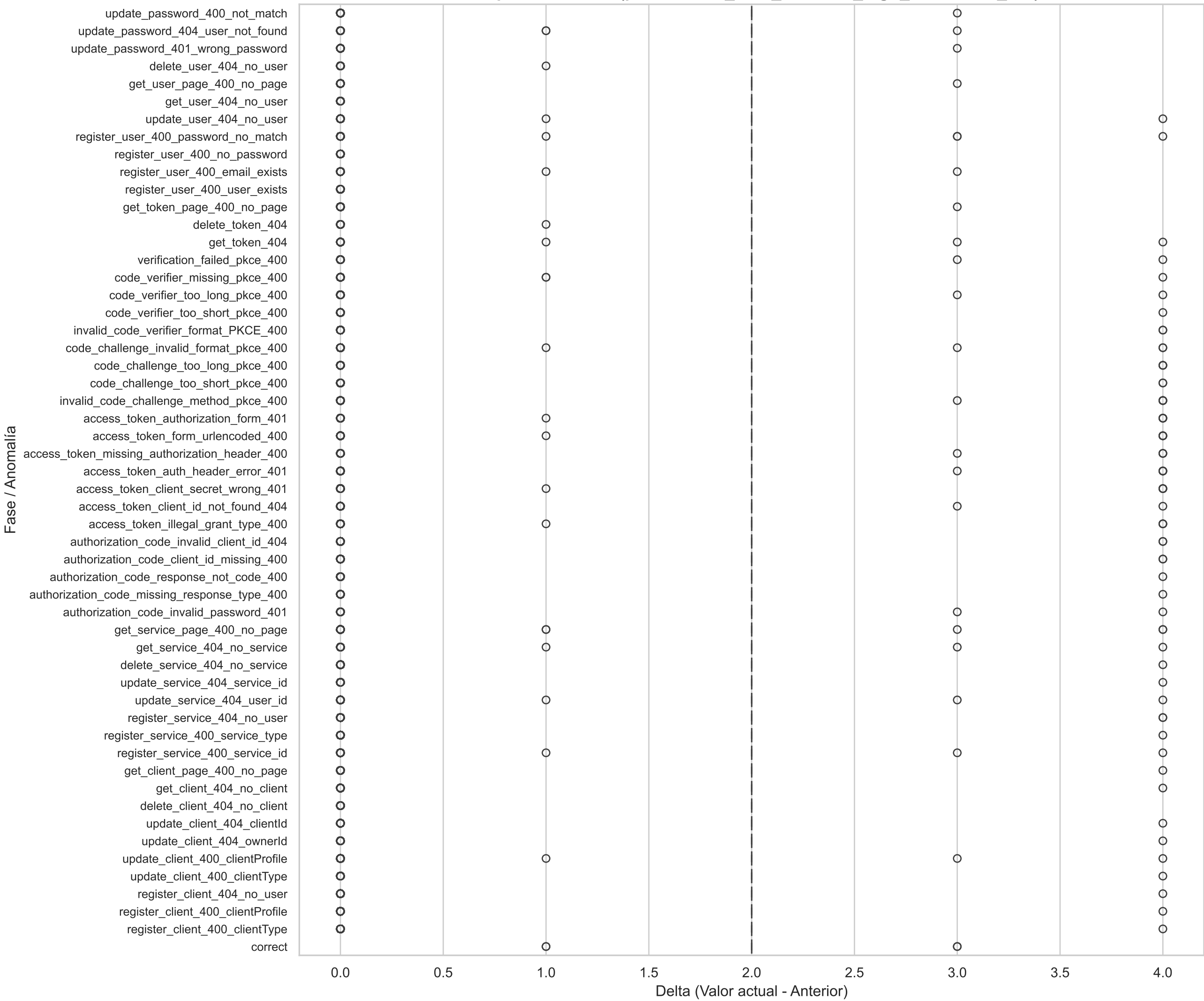
Boxplot Horizontal(prometheus_tsdb_isolation_high_watermark_diff)
