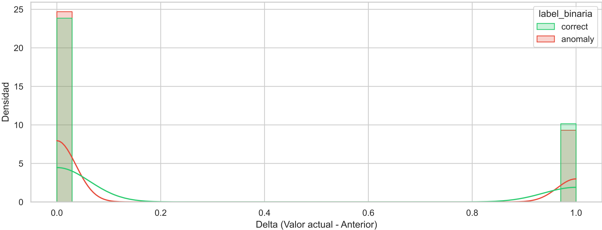
Histograma de Densidad Binario (prometheus_tsdb_wal_completed_pages_total_diff)
