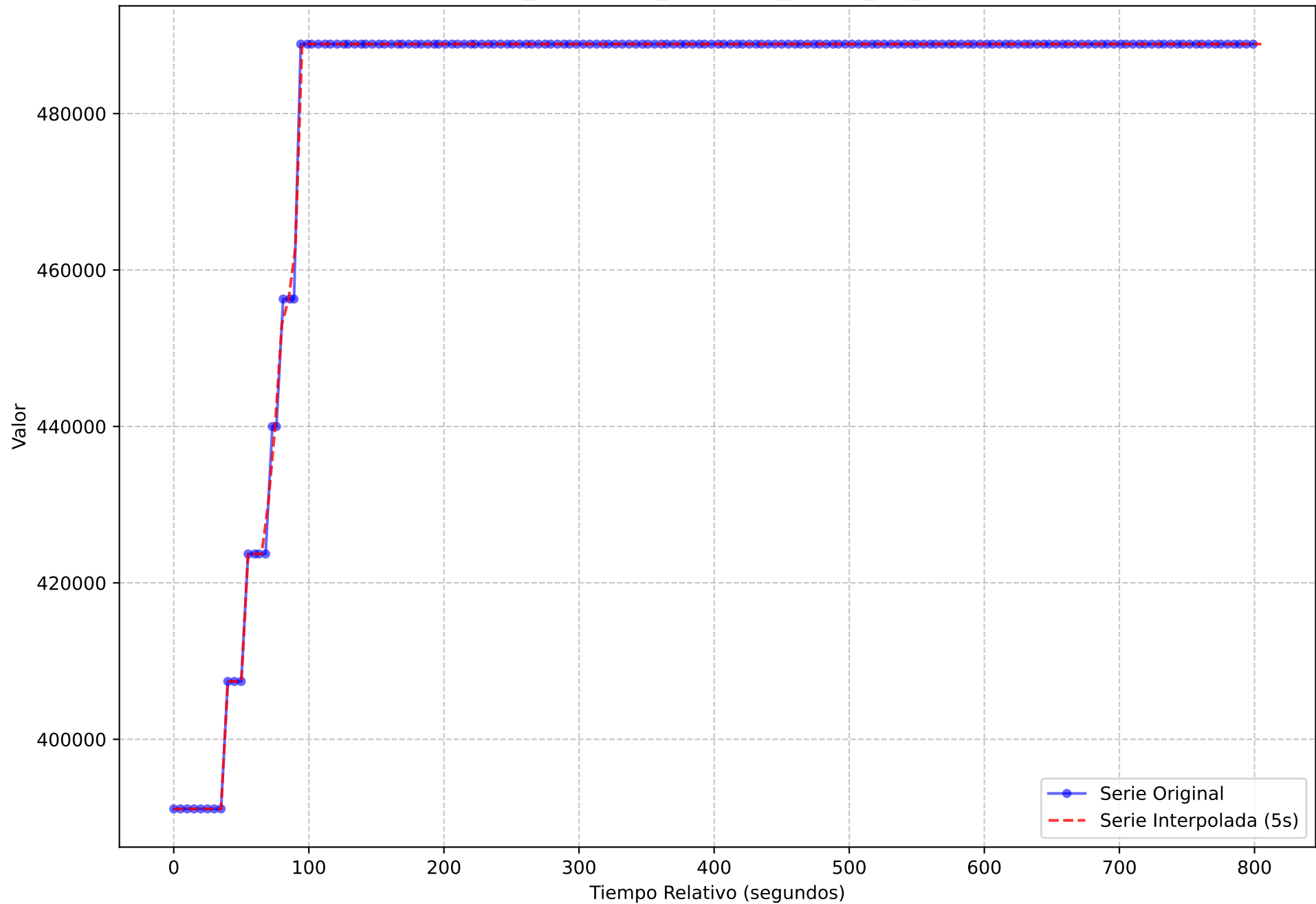
Serie Temporal Original vs. Interpolada (Muestreo 5s) execution_name = light-oauth2-data-1720167247.tar metric_name = go_memstats_mspan_sys_bytes
