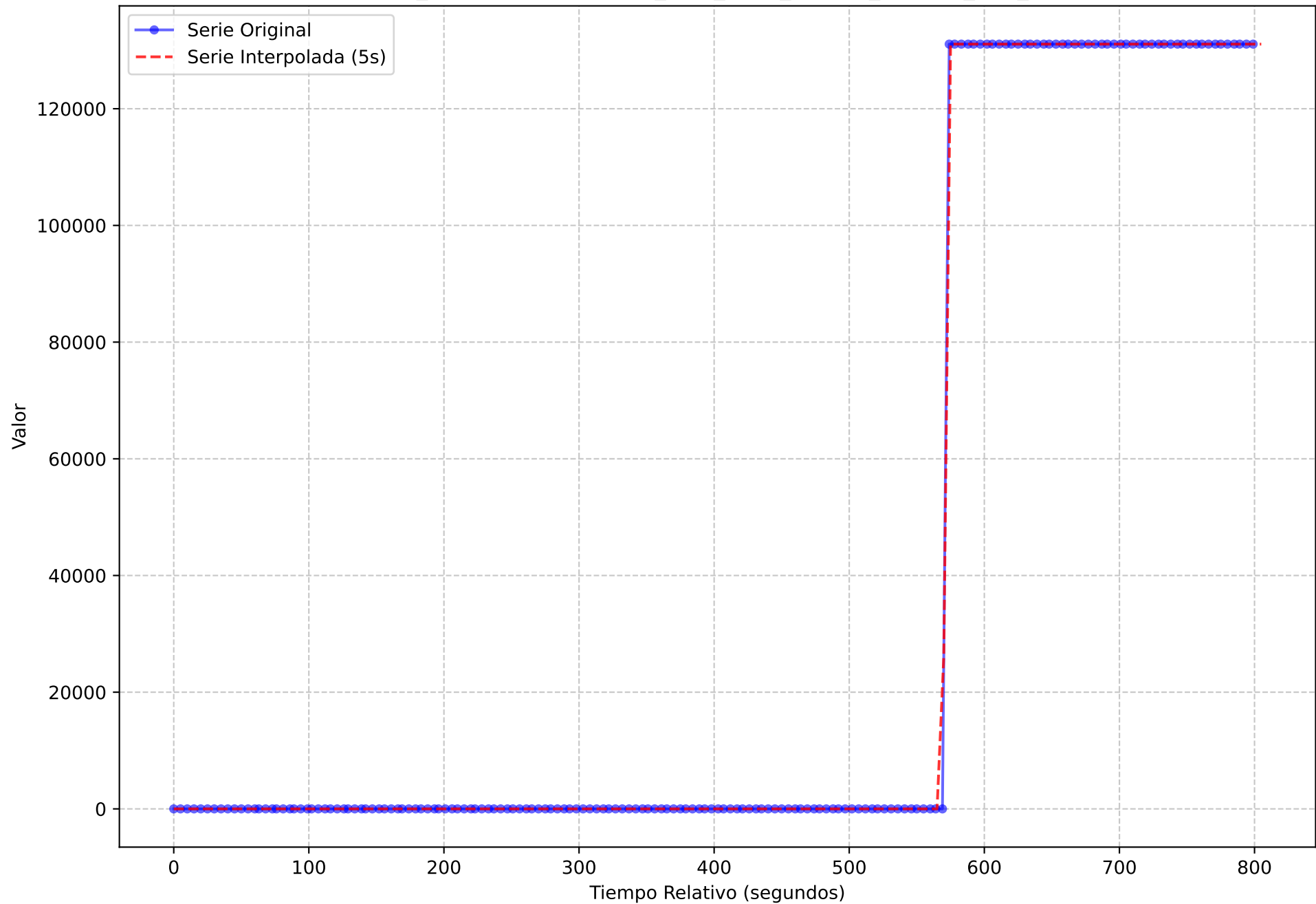
Serie Temporal Original vs. Interpolada (Muestreo 5s) execution_name = light-oauth2-data-1720167247.tar metric_name = prometheus_tsdb_head_chunks_storage_size_bytes
