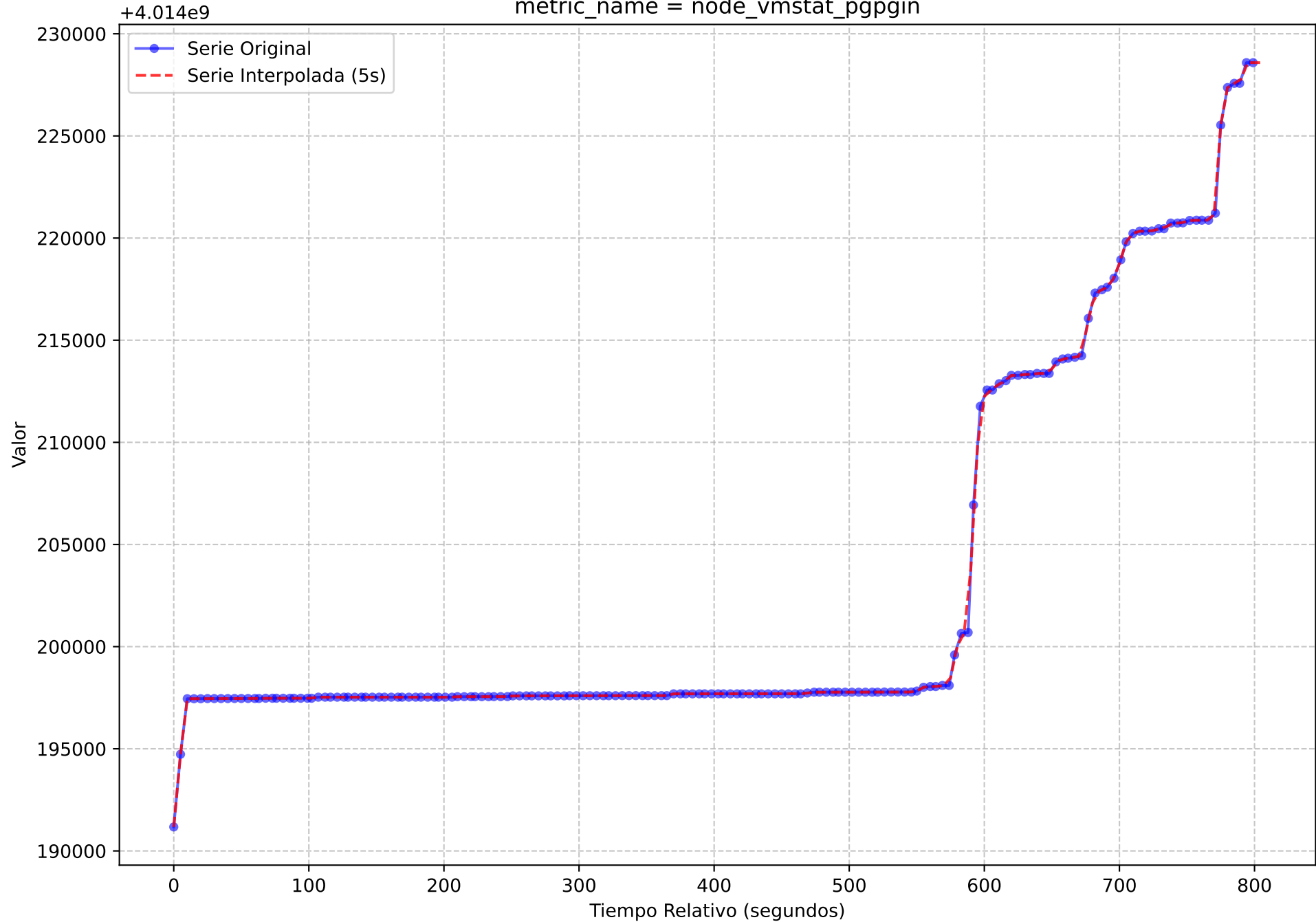
Serie Temporal Original vs. Interpolada (Muestreo 5s) execution_name = light-oauth2-data-1720167247.tar metric_name = node_vmstat_pgpgin
