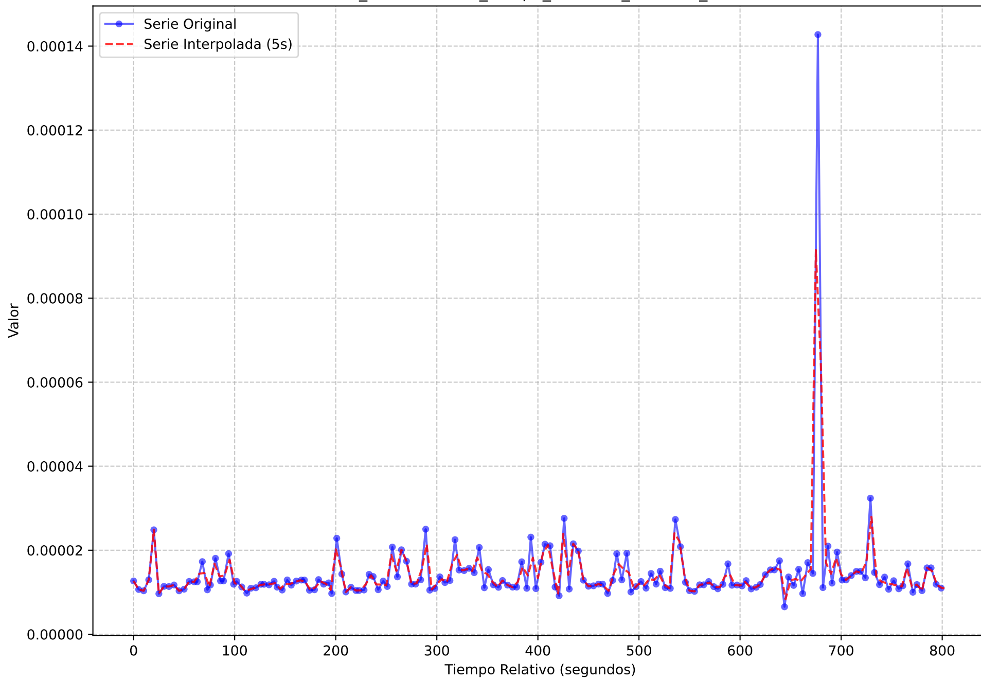
Serie Temporal Original vs. Interpolada (Muestreo 5s) execution_name = light-oauth2-data-1720167247.tar metric_name = node_scrape_collector_duration_seconds
