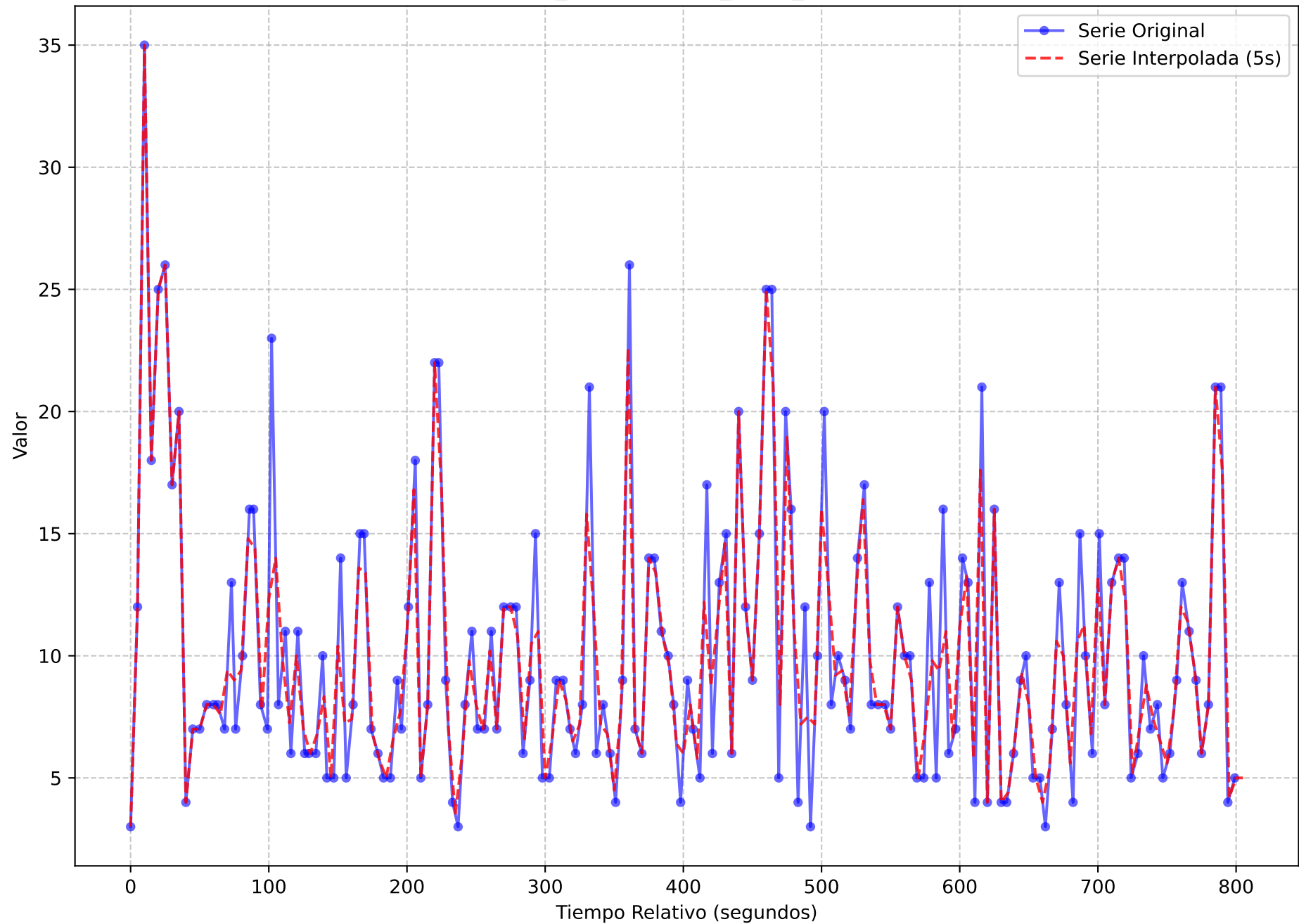
Serie Temporal Original vs. Interpolada (Muestreo 5s) execution_name = light-oauth2-data-1720167247.tar metric_name = node_procs_running
