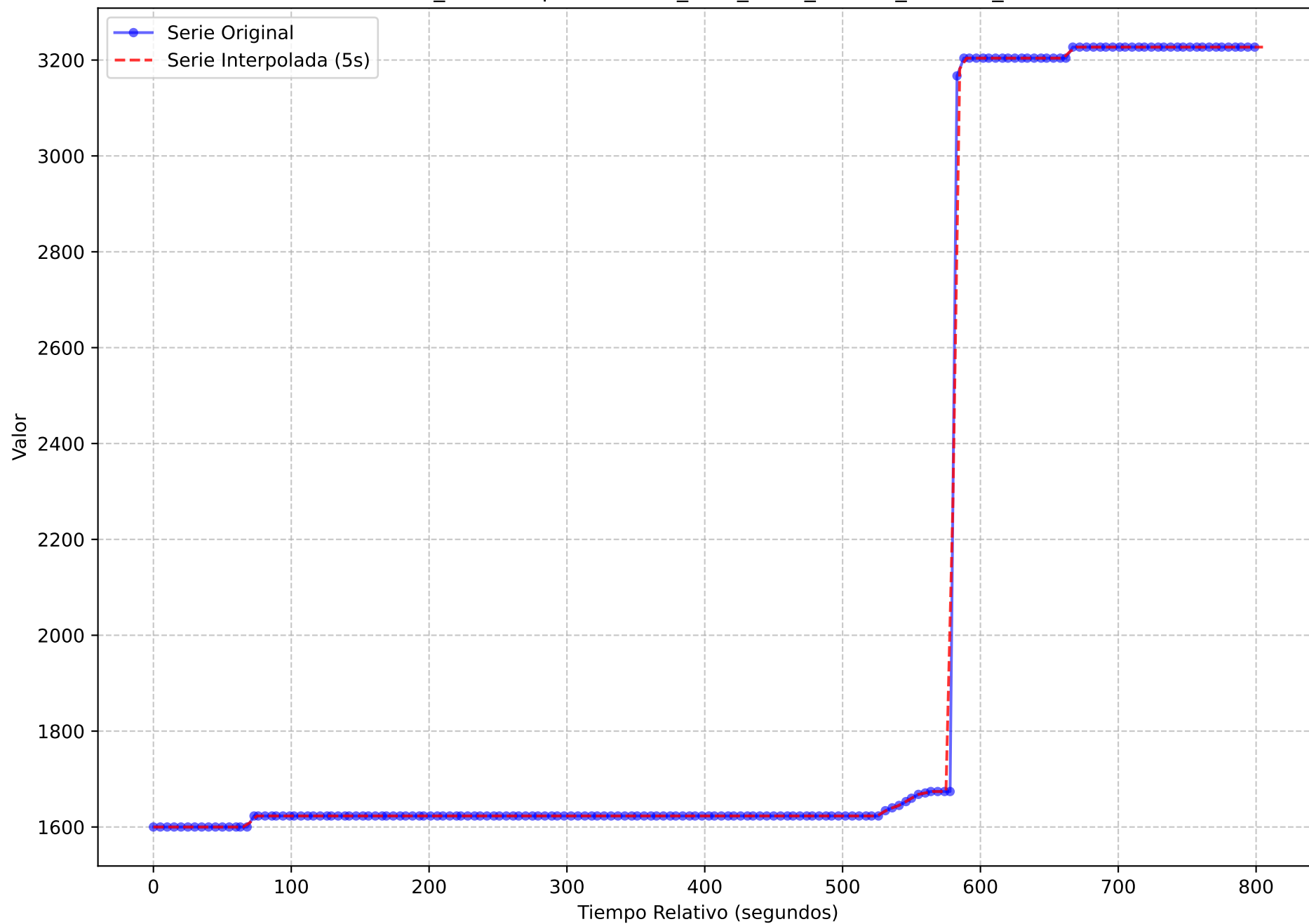
Serie Temporal Original vs. Interpolada (Muestreo 5s) execution_name = light-oauth2-data-1720167247.tar metric_name = prometheus_tsdb_head_chunks_created_total
