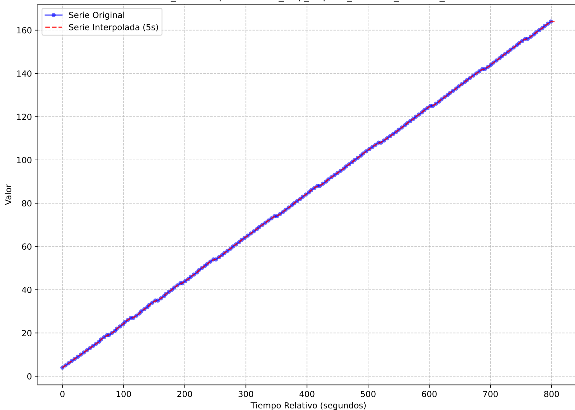
Serie Temporal Original vs. Interpolada (Muestreo 5s) execution_name = light-oauth2-data-1720167247.tar metric_name = prometheus_http_request_duration_seconds_bucket
