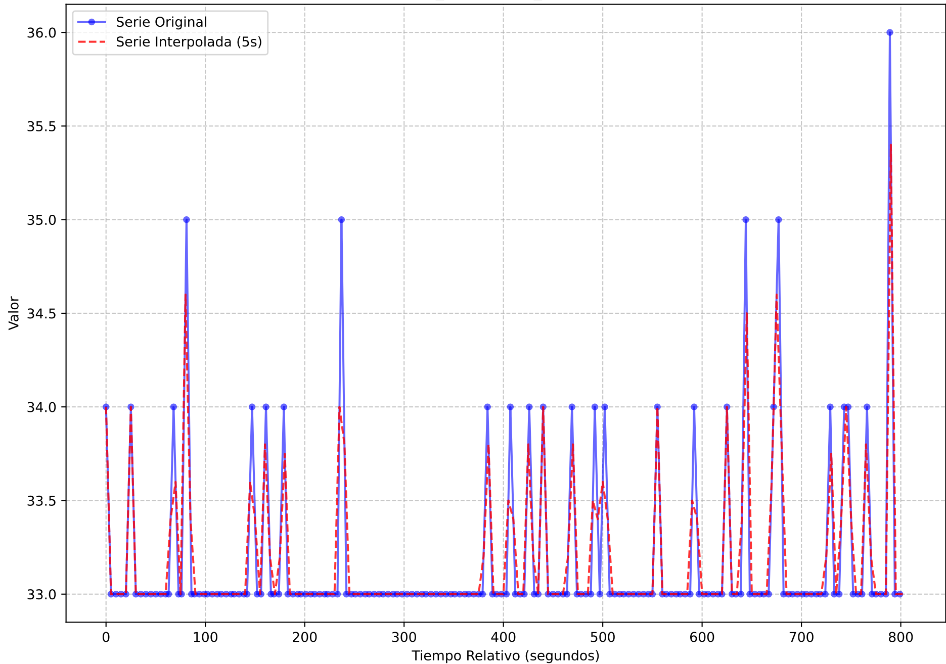
Serie Temporal Original vs. Interpolada (Muestreo 5s) execution_name = light-oauth2-data-1720167247.tar metric_name = go_goroutines
