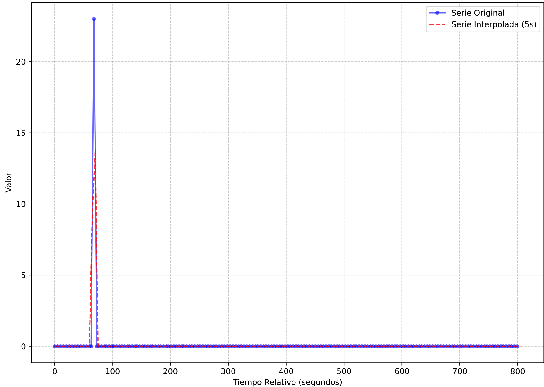
Serie Temporal Original vs. Interpolada (Muestreo 5s) execution_name = light-oauth2-data-1720167247.tar metric_name = scrape_series_added
