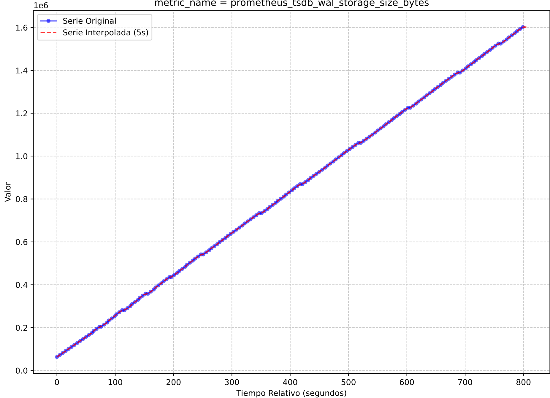
Serie Temporal Original vs. Interpolada (Muestreo 5s) execution_name = light-oauth2-data-1720167247.tar metric_name = prometheus_tsdb_wal_storage_size_bytes
