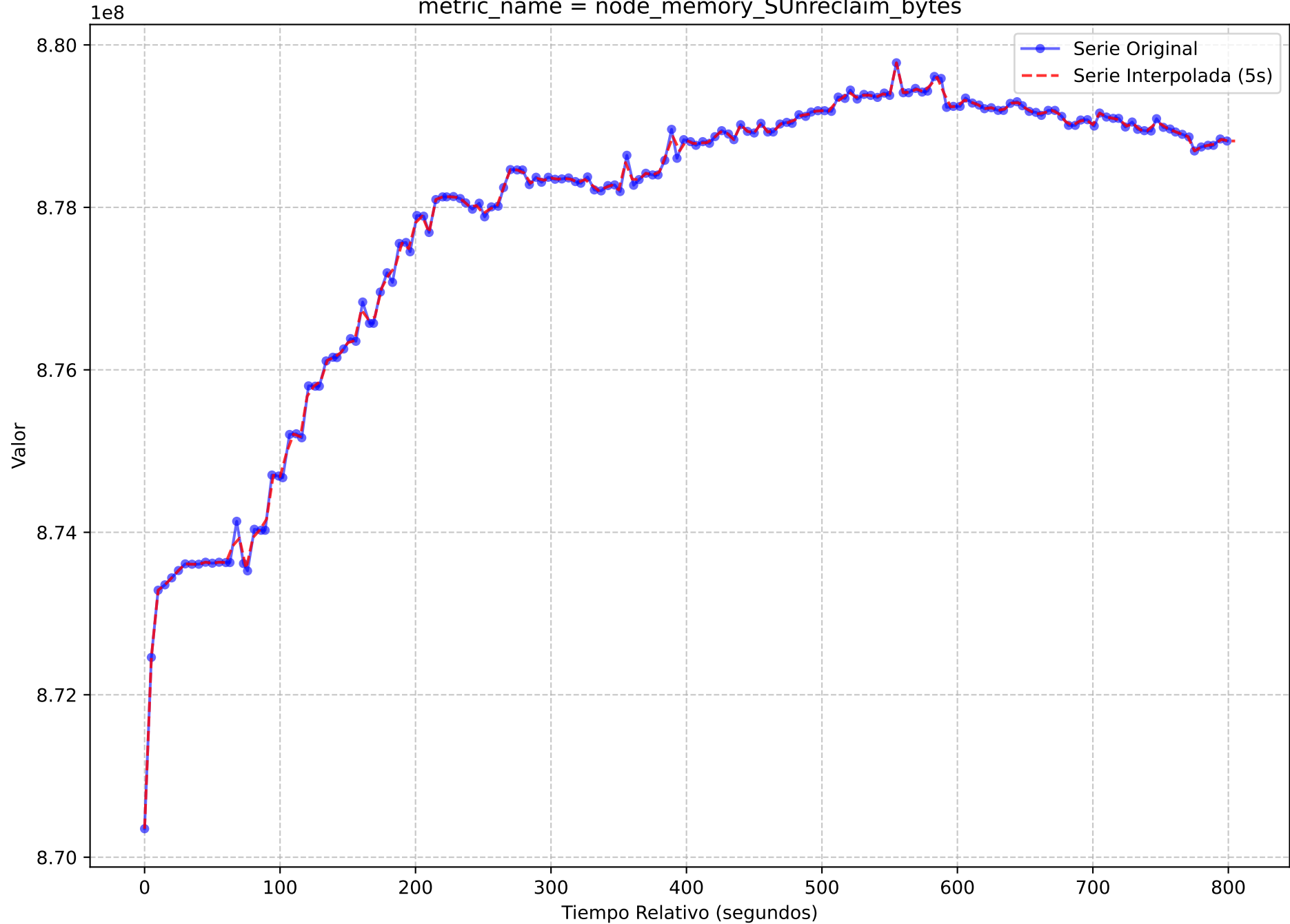
Serie Temporal Original vs. Interpolada (Muestreo 5s) execution_name = light-oauth2-data-1720167247.tar metric_name = node_memory_SUnreclaim_bytes
