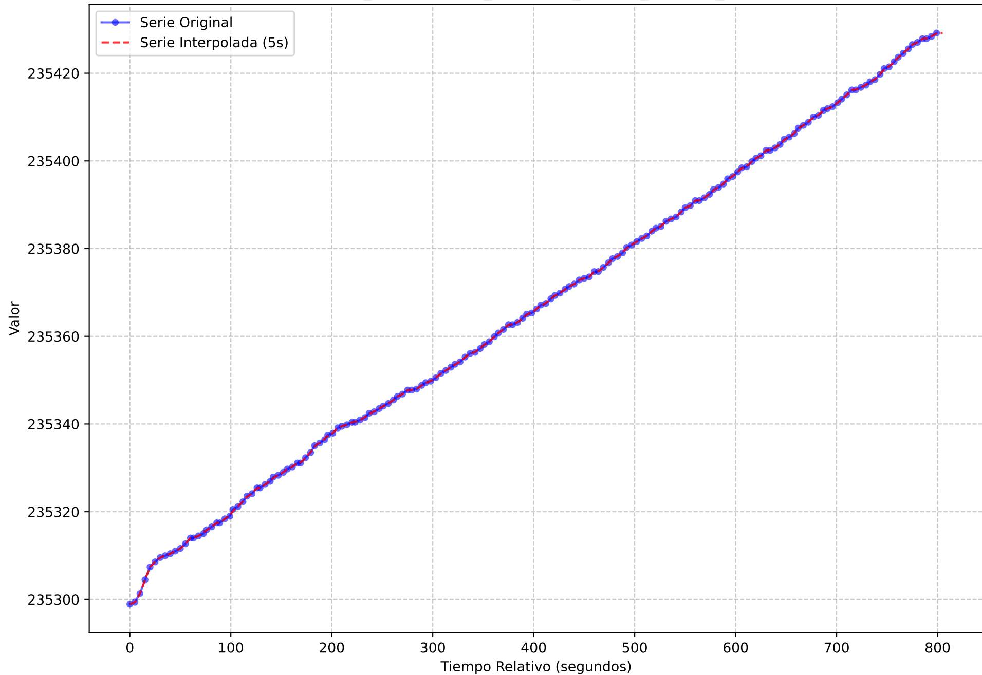
Serie Temporal Original vs. Interpolada (Muestreo 5s) execution_name = light-oauth2-data-1720167247.tar metric_name = node_schedstat_waiting_seconds_total
