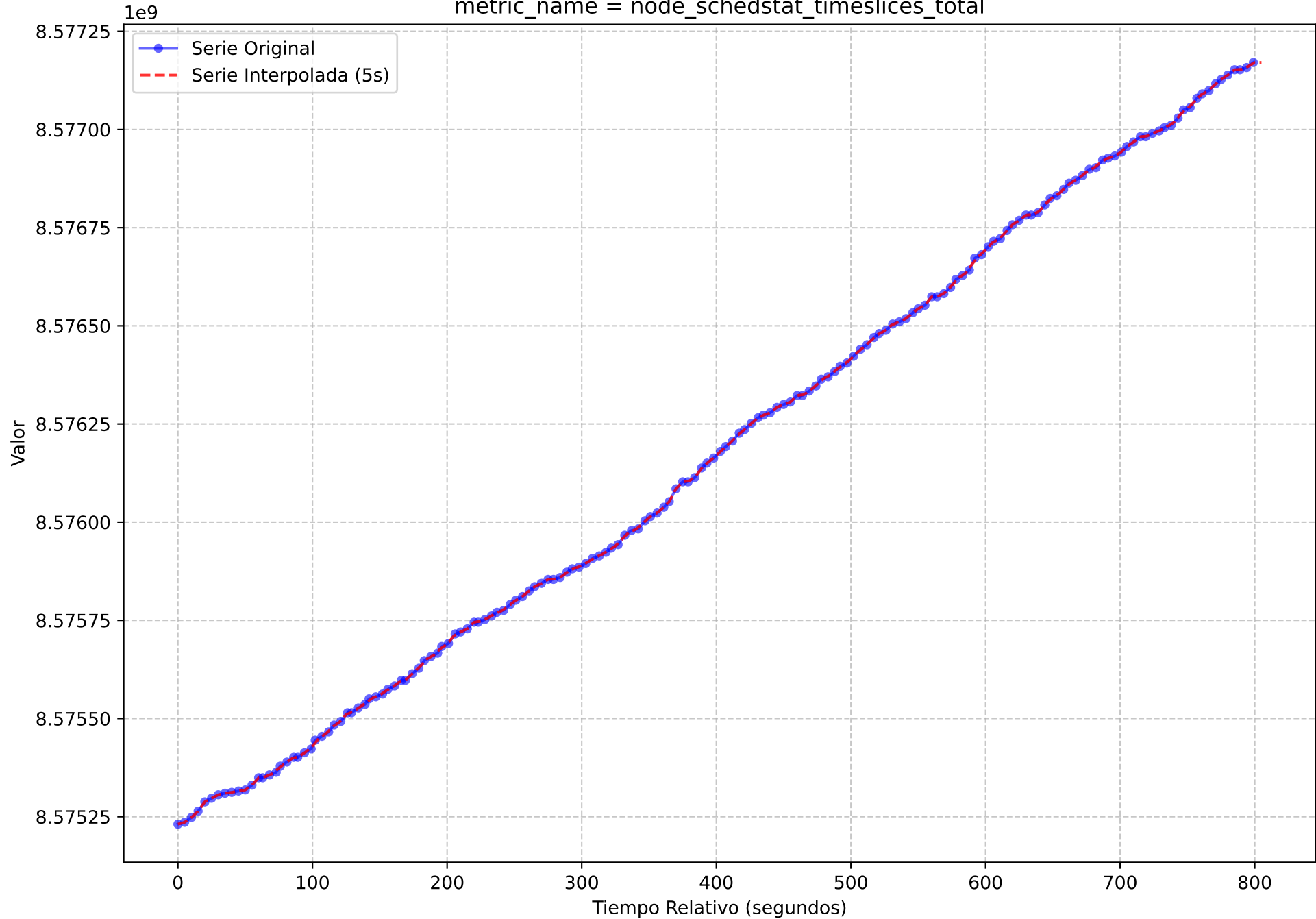
Serie Temporal Original vs. Interpolada (Muestreo 5s) execution_name = light-oauth2-data-1720167247.tar metric_name = node_schedstat_timeslices_total
