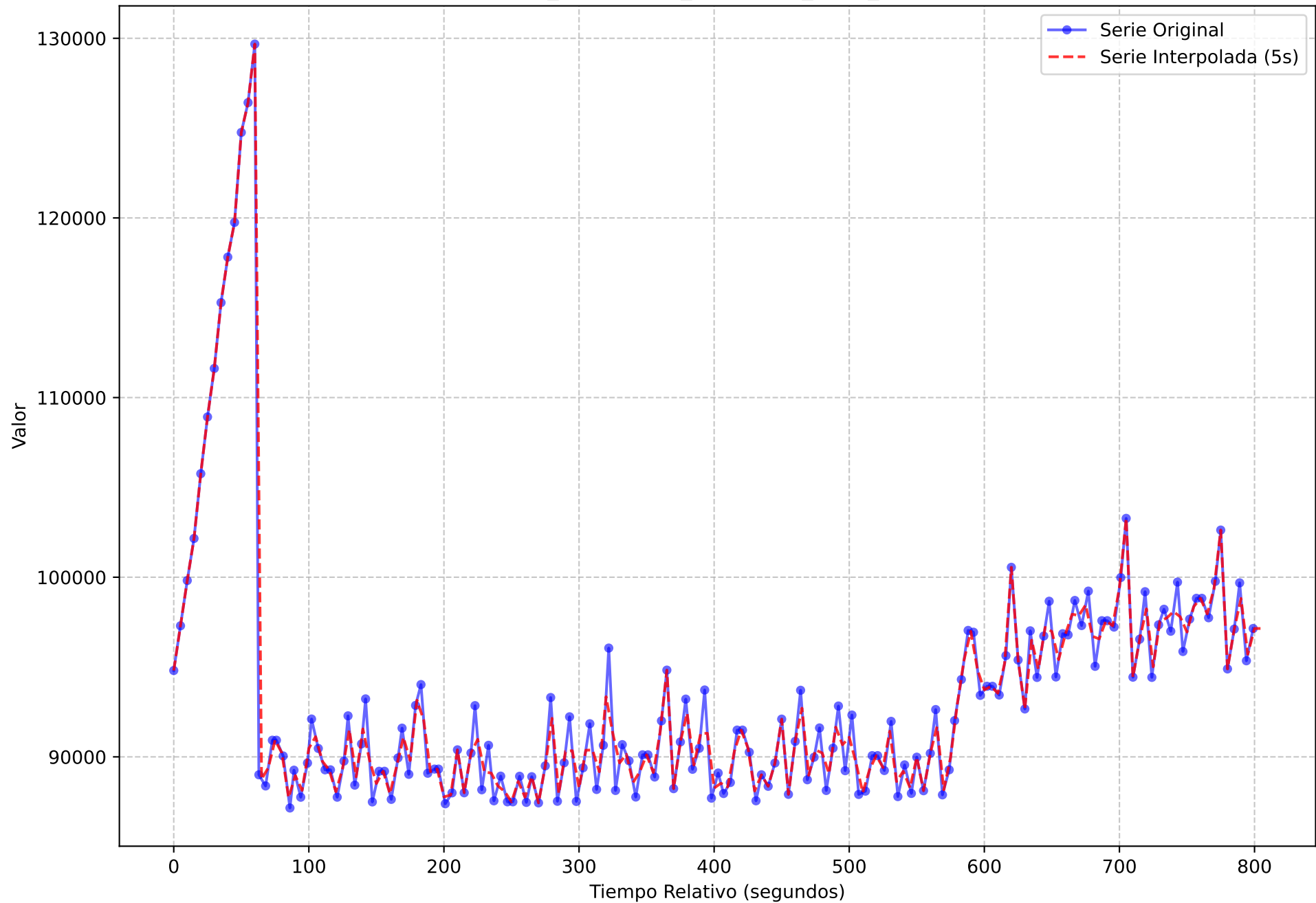
Serie Temporal Original vs. Interpolada (Muestreo 5s) execution_name = light-oauth2-data-1720167247.tar metric_name = go_memstats_heap_objects
