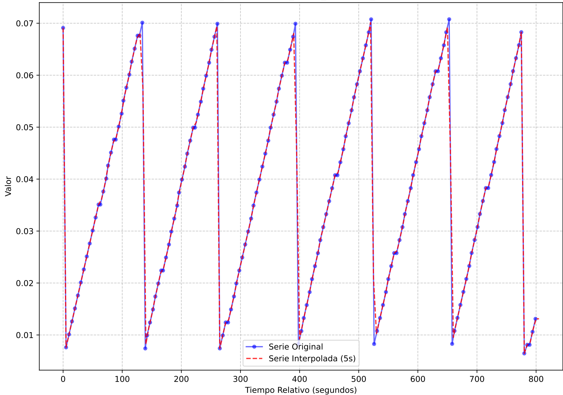
Serie Temporal Original vs. Interpolada (Muestreo 5s) execution_name = light-oauth2-data-1720167247.tar metric_name = node_timex_maxerror_seconds
