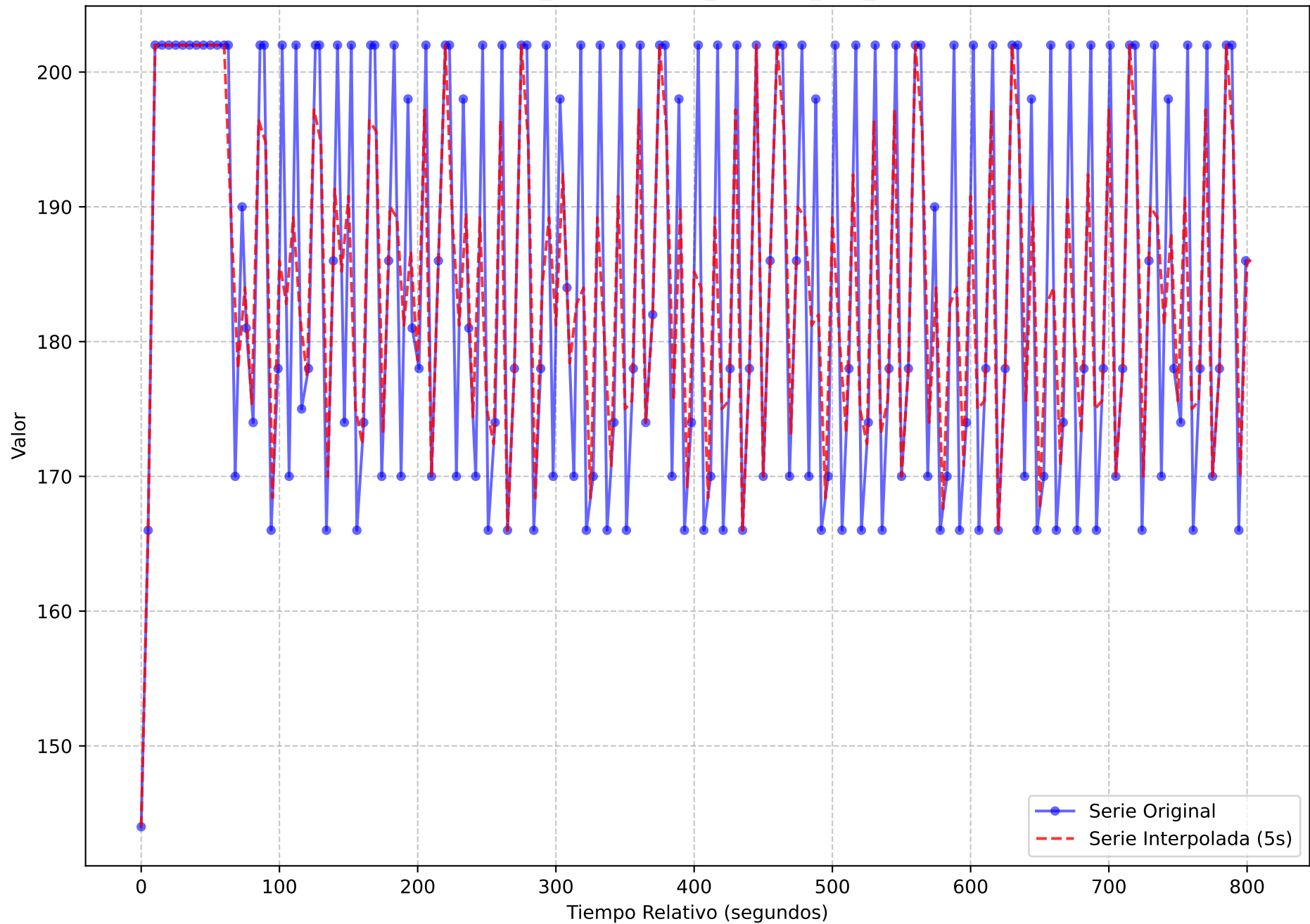
Serie Temporal Original vs. Interpolada (Muestreo 5s) execution_name = light-oauth2-data-1720167247.tar metric_name = node_sockstat_TCP_alloc
