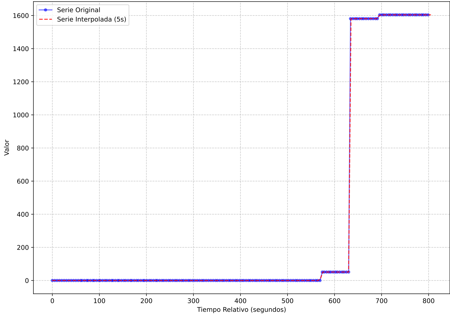
Serie Temporal Original vs. Interpolada (Muestreo 5s) execution_name = light-oauth2-data-1720167247.tar metric_name = prometheus_tsdb_mmap_chunks_total
