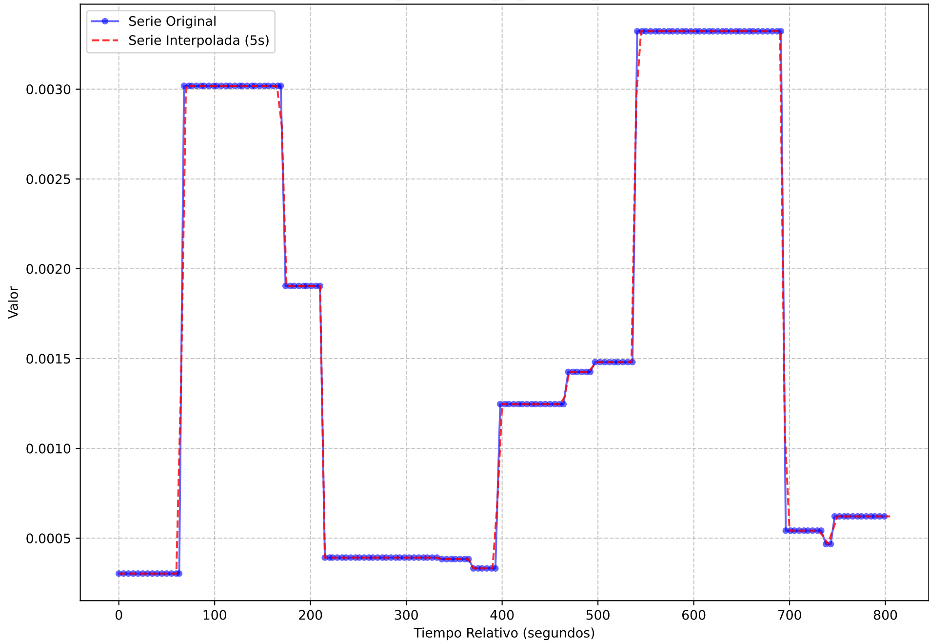
Serie Temporal Original vs. Interpolada (Muestreo 5s) execution_name = light-oauth2-data-1720167247.tar metric_name = go_gc_duration_seconds
