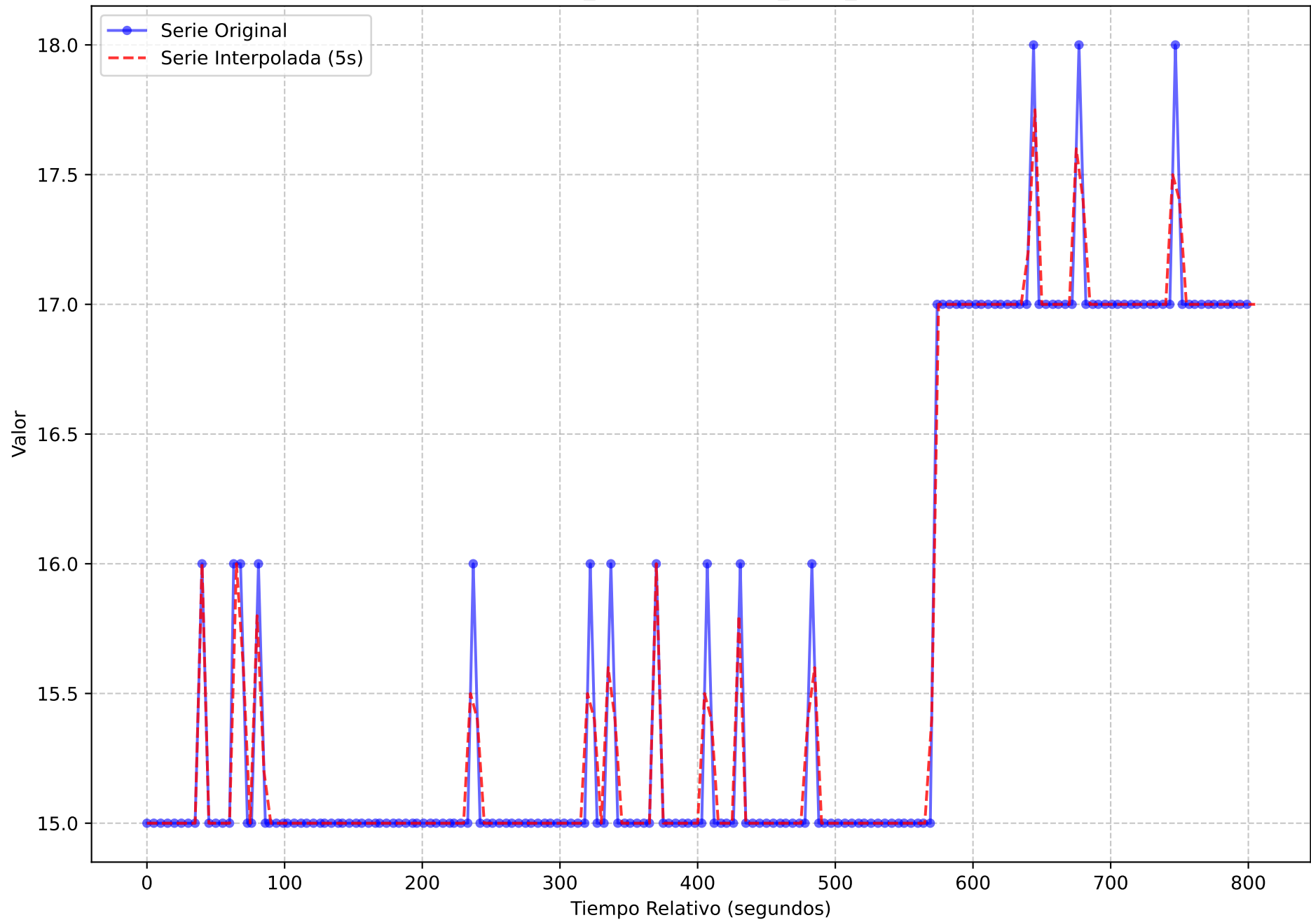
Serie Temporal Original vs. Interpolada (Muestreo 5s) execution_name = light-oauth2-data-1720167247.tar metric_name = process_open_fds
