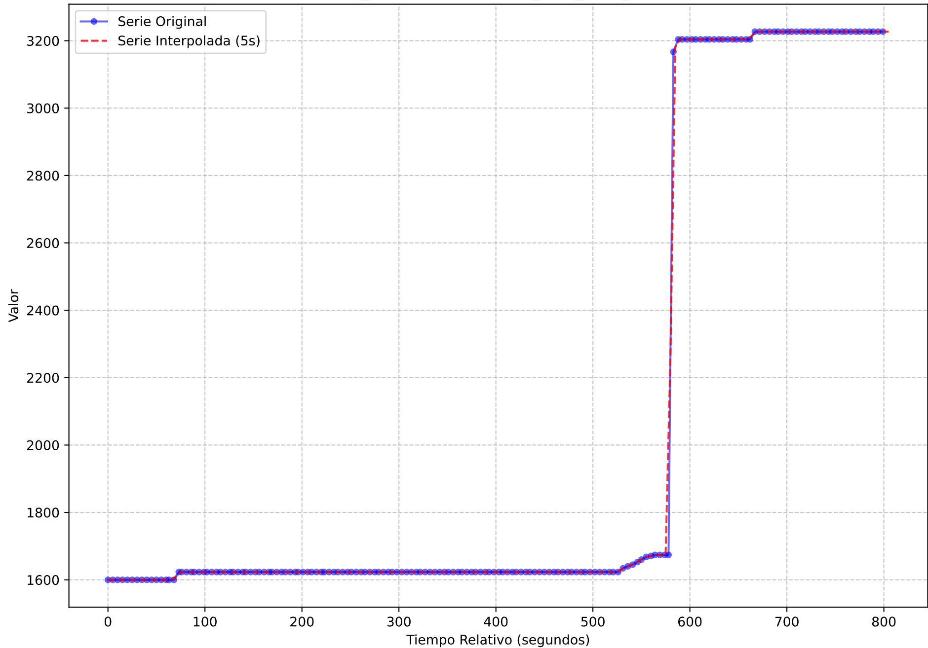
Serie Temporal Original vs. Interpolada (Muestreo 5s) execution_name = light-oauth2-data-1720167247.tar metric_name = prometheus_tsdb_head_chunks
