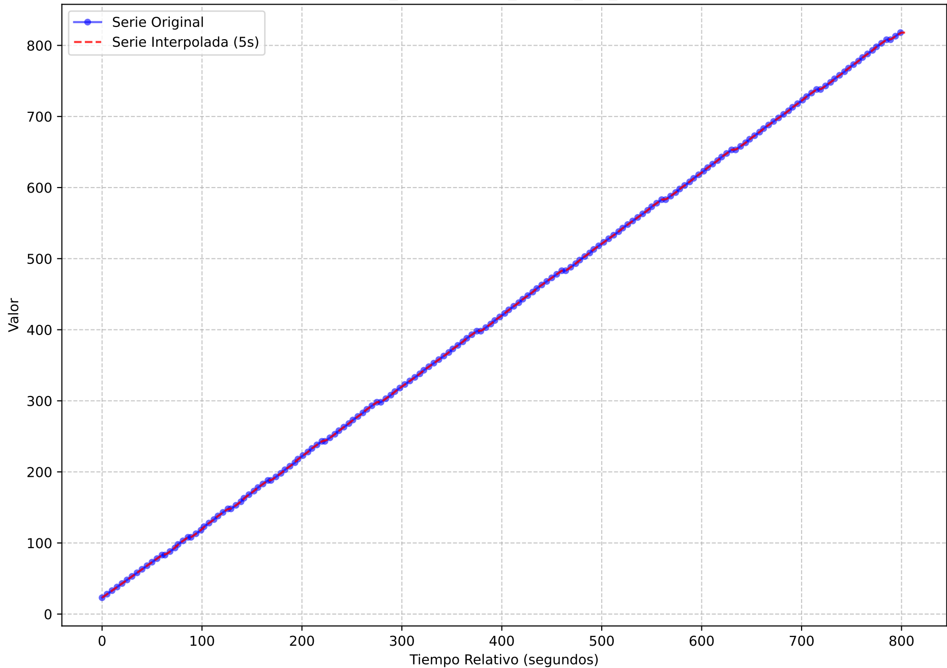
Serie Temporal Original vs. Interpolada (Muestreo 5s) execution_name = light-oauth2-data-1720167247.tar metric_name = node_netstat_Tcp_InSegs
