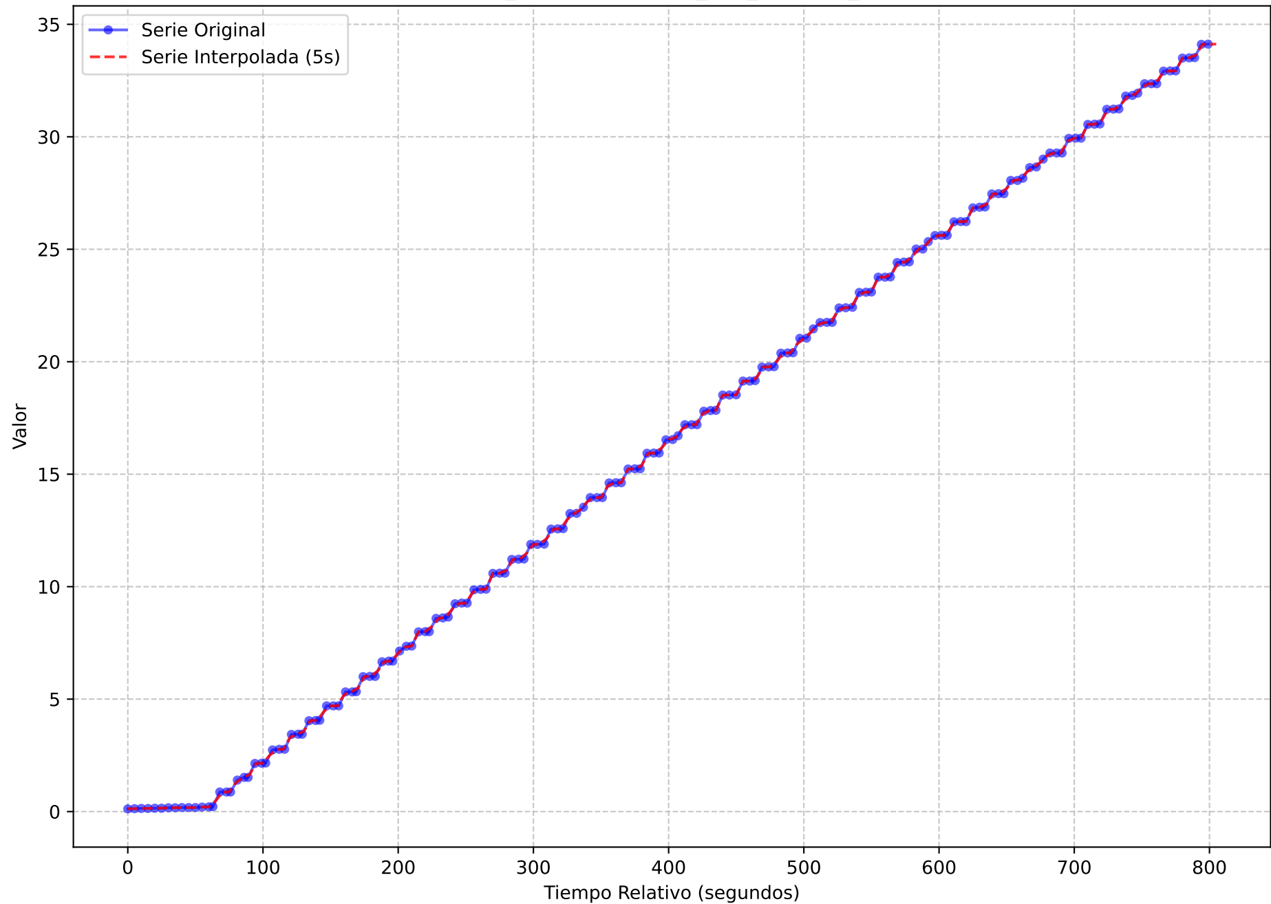
Serie Temporal Original vs. Interpolada (Muestreo 5s) execution_name = light-oauth2-data-1720167247.tar metric_name = process_cpu_seconds_total
