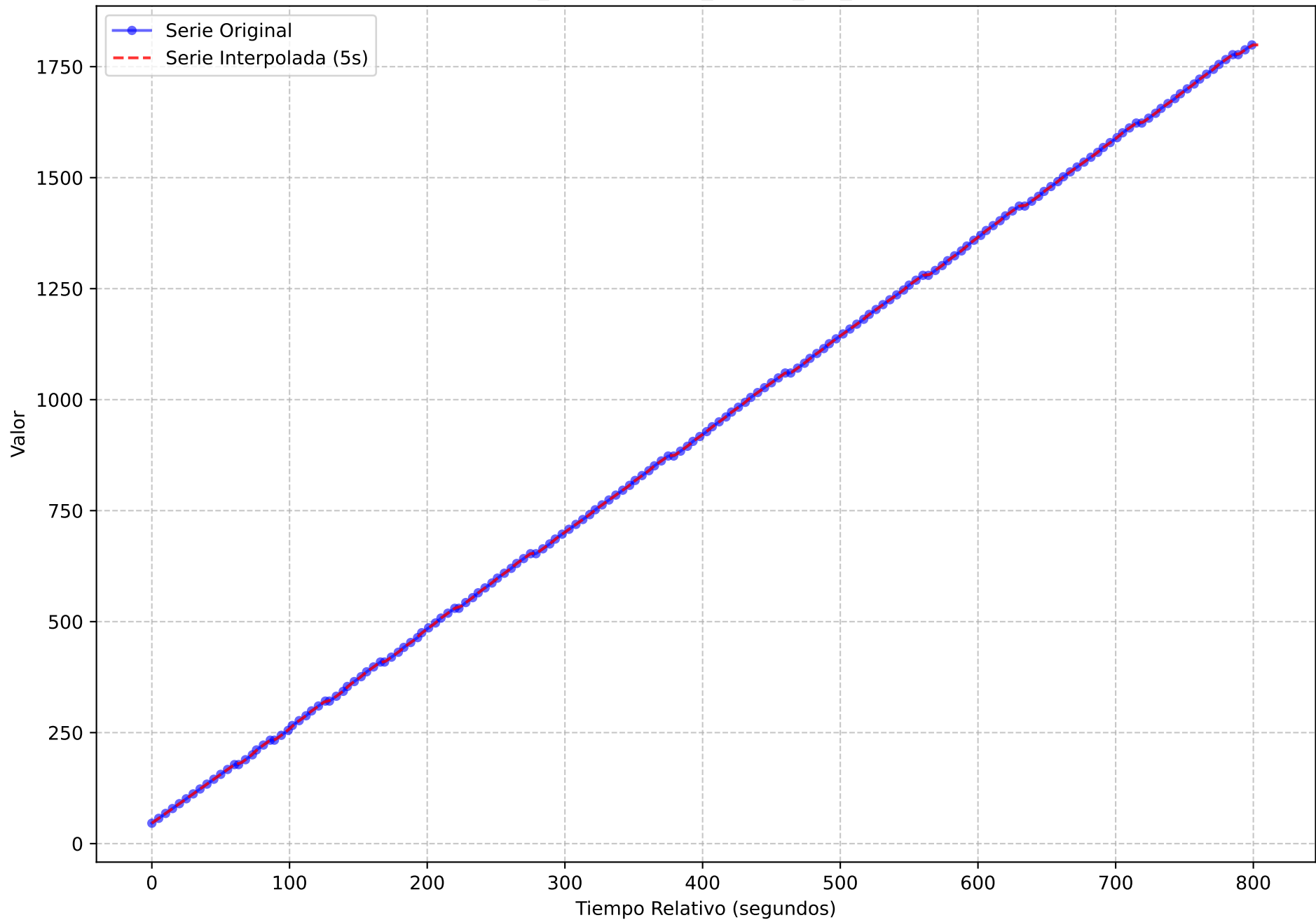
Serie Temporal Original vs. Interpolada (Muestreo 5s) execution_name = light-oauth2-data-1720167247.tar metric_name = node_netstat_Tcp_OutSegs
