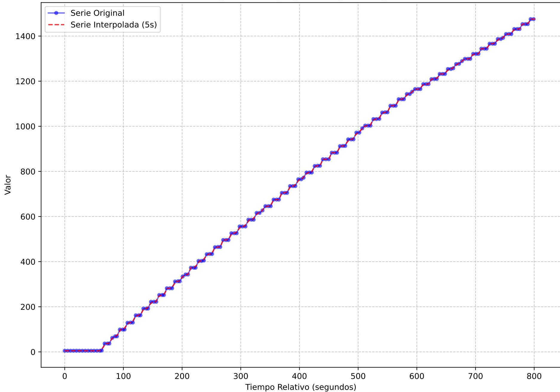
Serie Temporal Original vs. Interpolada (Muestreo 5s) execution_name = light-oauth2-data-1720167247.tar metric_name = go_gc_duration_seconds_count
