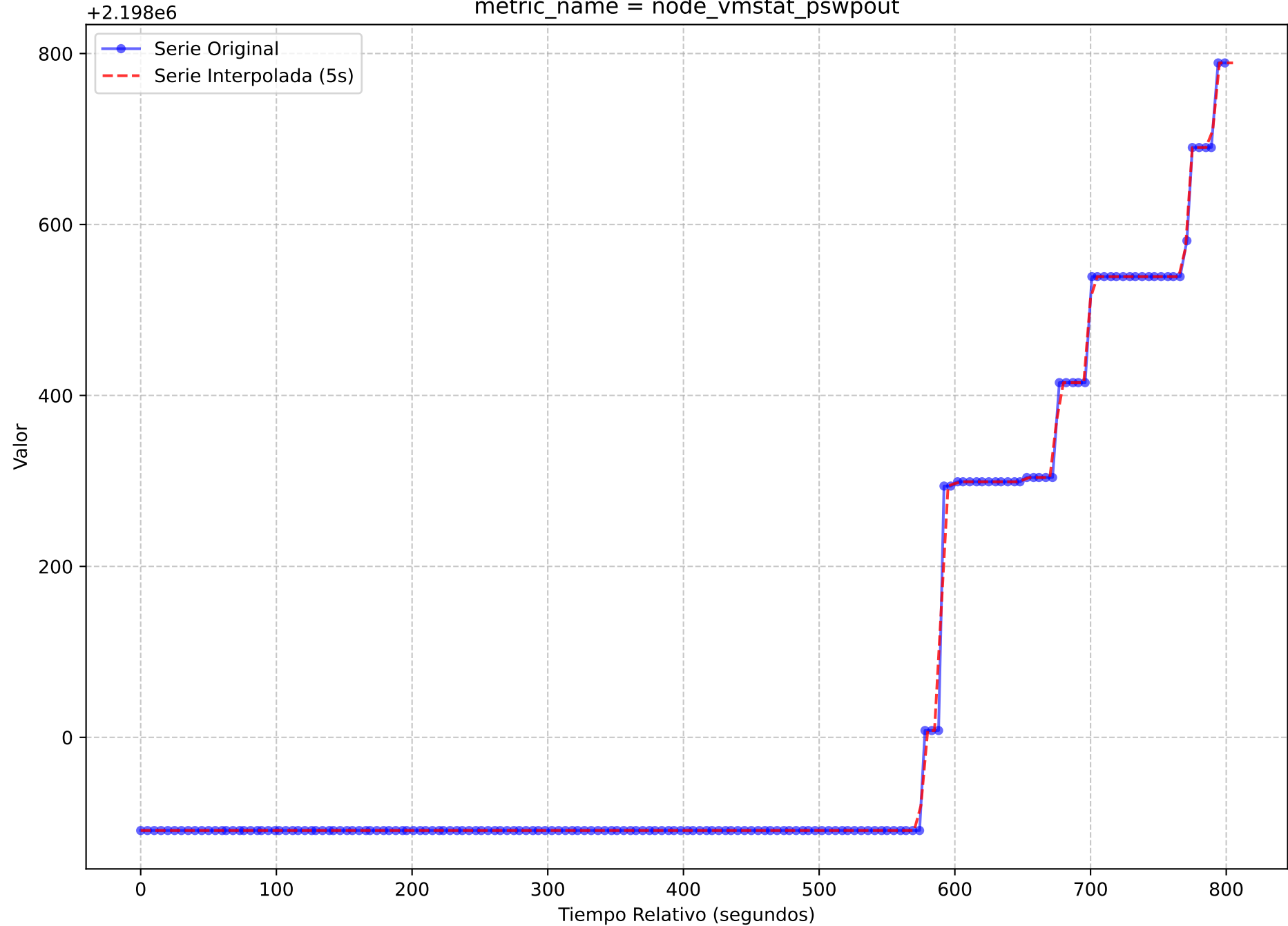
Serie Temporal Original vs. Interpolada (Muestreo 5s) execution_name = light-oauth2-data-1720167247.tar metric_name = node_vmstat_pswpout
