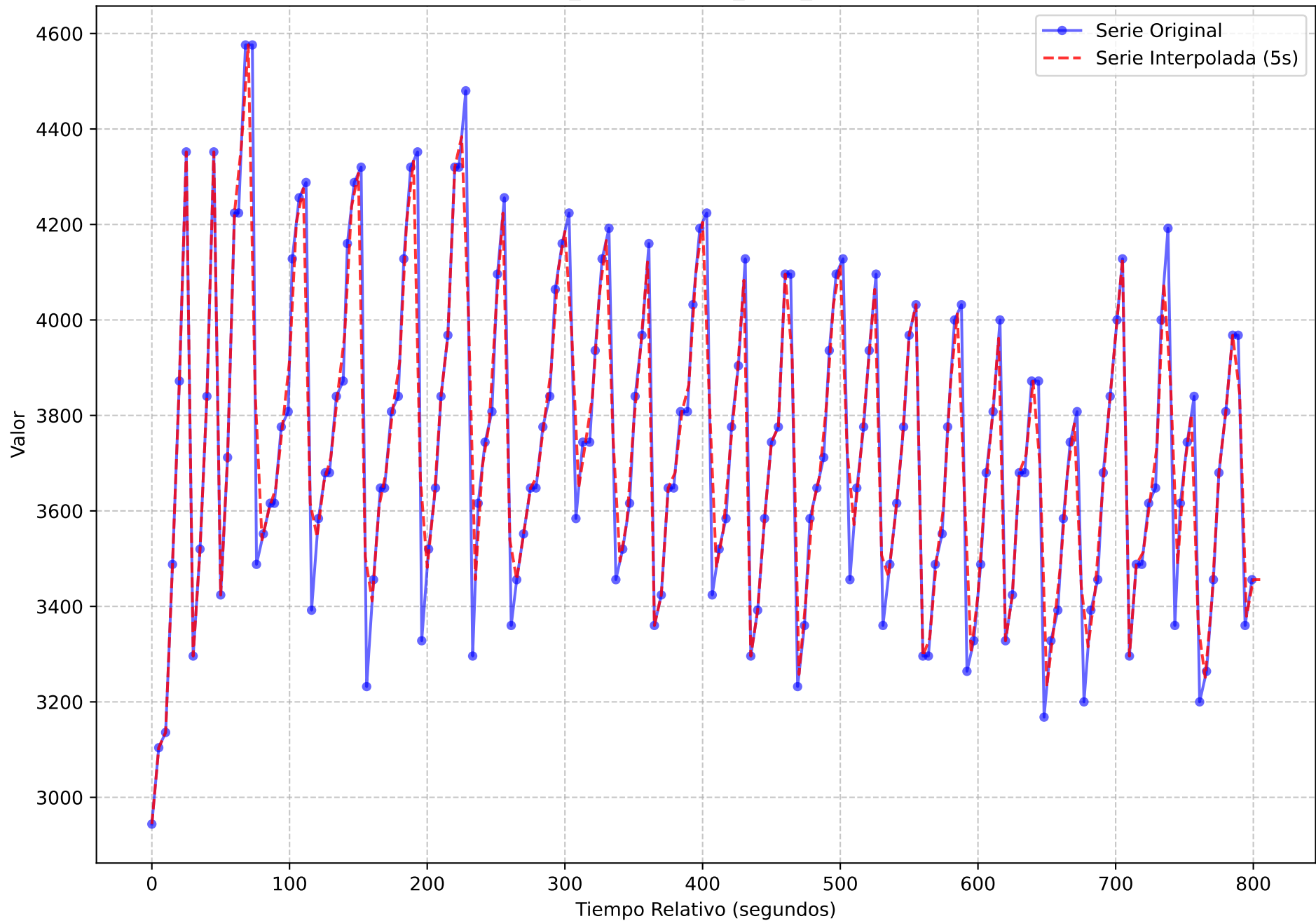
Serie Temporal Original vs. Interpolada (Muestreo 5s) execution_name = light-oauth2-data-1720167247.tar metric_name = node_filefd_allocated
