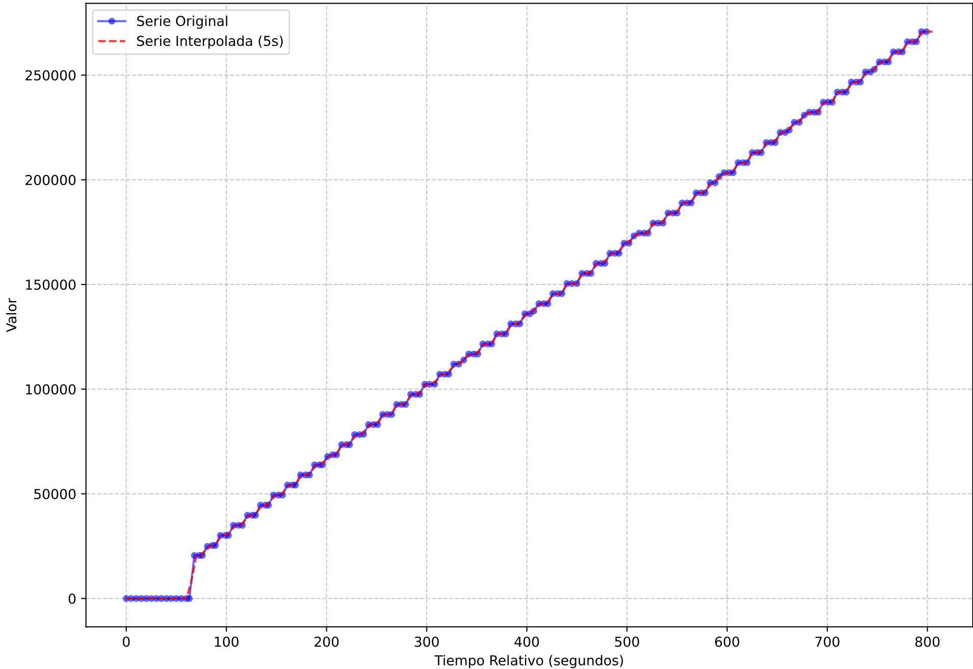
Serie Temporal Original vs. Interpolada (Muestreo 5s) execution_name = light-oauth2-data-1720167247.tar metric_name = prometheus_engine_query_samples_total
