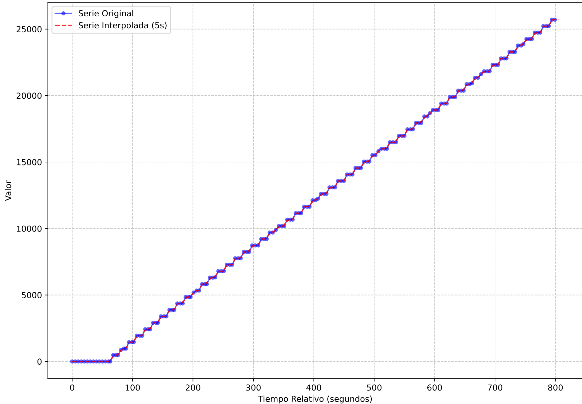
Serie Temporal Original vs. Interpolada (Muestreo 5s) execution_name = light-oauth2-data-1720167247.tar metric_name = prometheus_engine_query_duration_seconds_count
