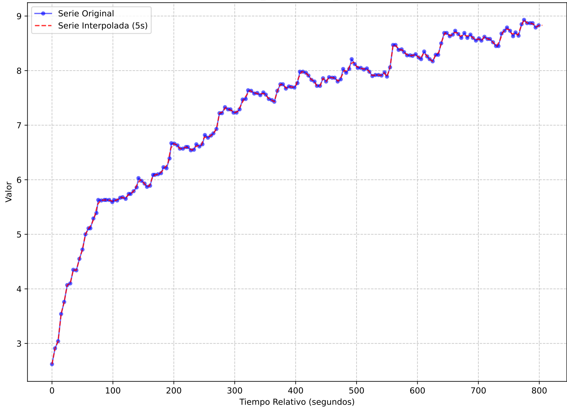
Serie Temporal Original vs. Interpolada (Muestreo 5s) execution_name = light-oauth2-data-1720167247.tar metric_name = node_load5
