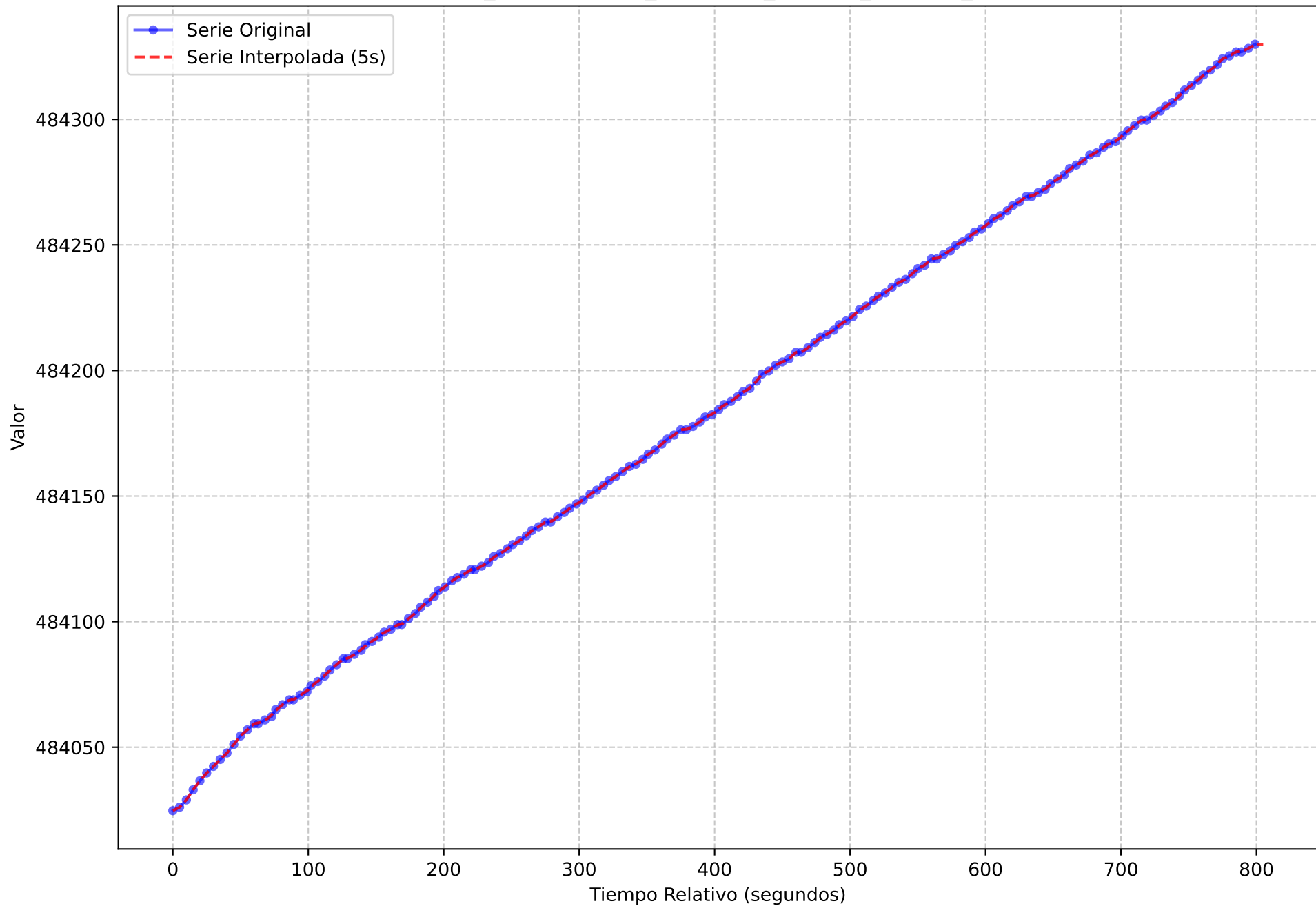
Serie Temporal Original vs. Interpolada (Muestreo 5s) execution_name = light-oauth2-data-1720167247.tar metric_name = node_schedstat_running_seconds_total
