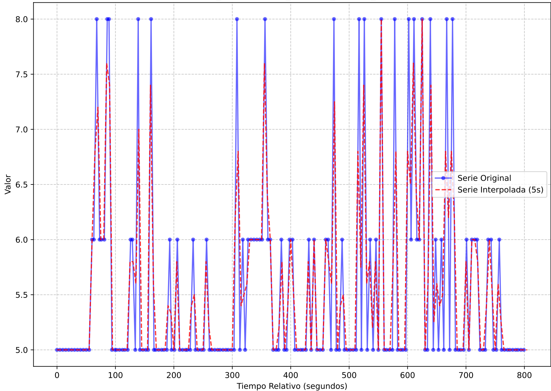
Serie Temporal Original vs. Interpolada (Muestreo 5s) execution_name = light-oauth2-data-1720167247.tar metric_name = node_sockstat_sockets_used
