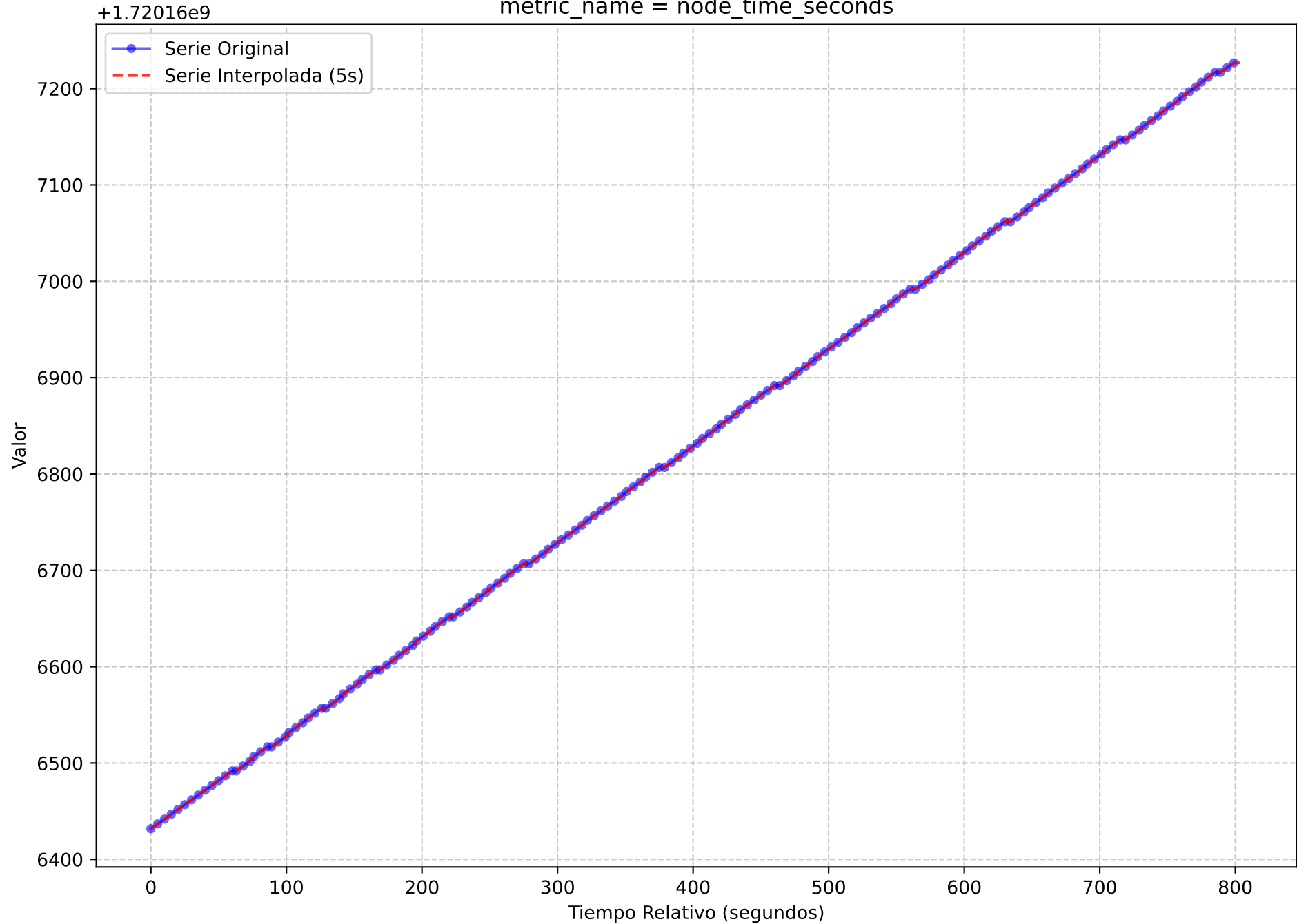
Serie Temporal Original vs. Interpolada (Muestreo 5s) execution_name = light-oauth2-data-1720167247.tar metric_name = node_time_seconds
