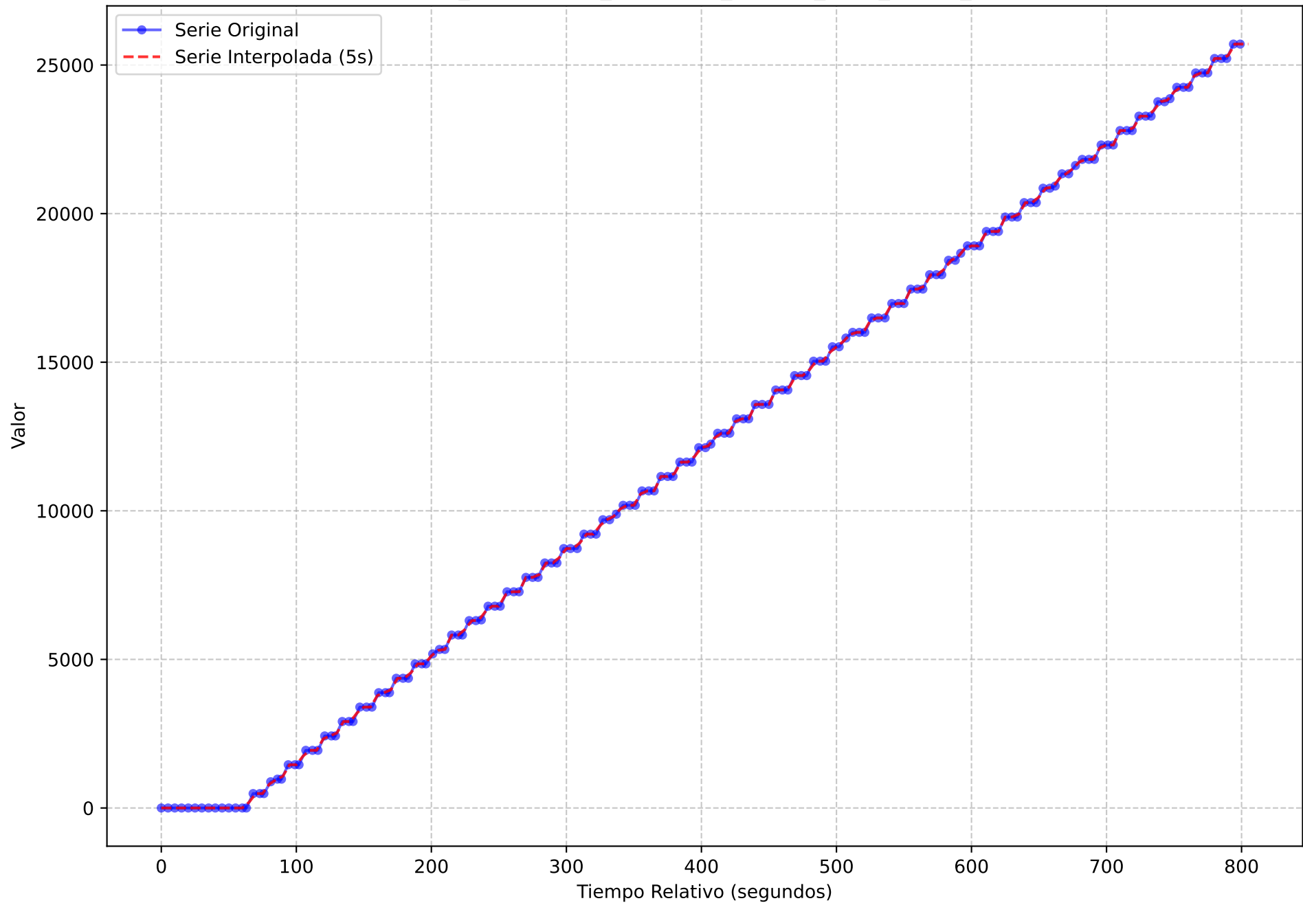
Serie Temporal Original vs. Interpolada (Muestreo 5s) execution_name = light-oauth2-data-1720167247.tar metric_name = net_contrack_listener_conn_closed_total
