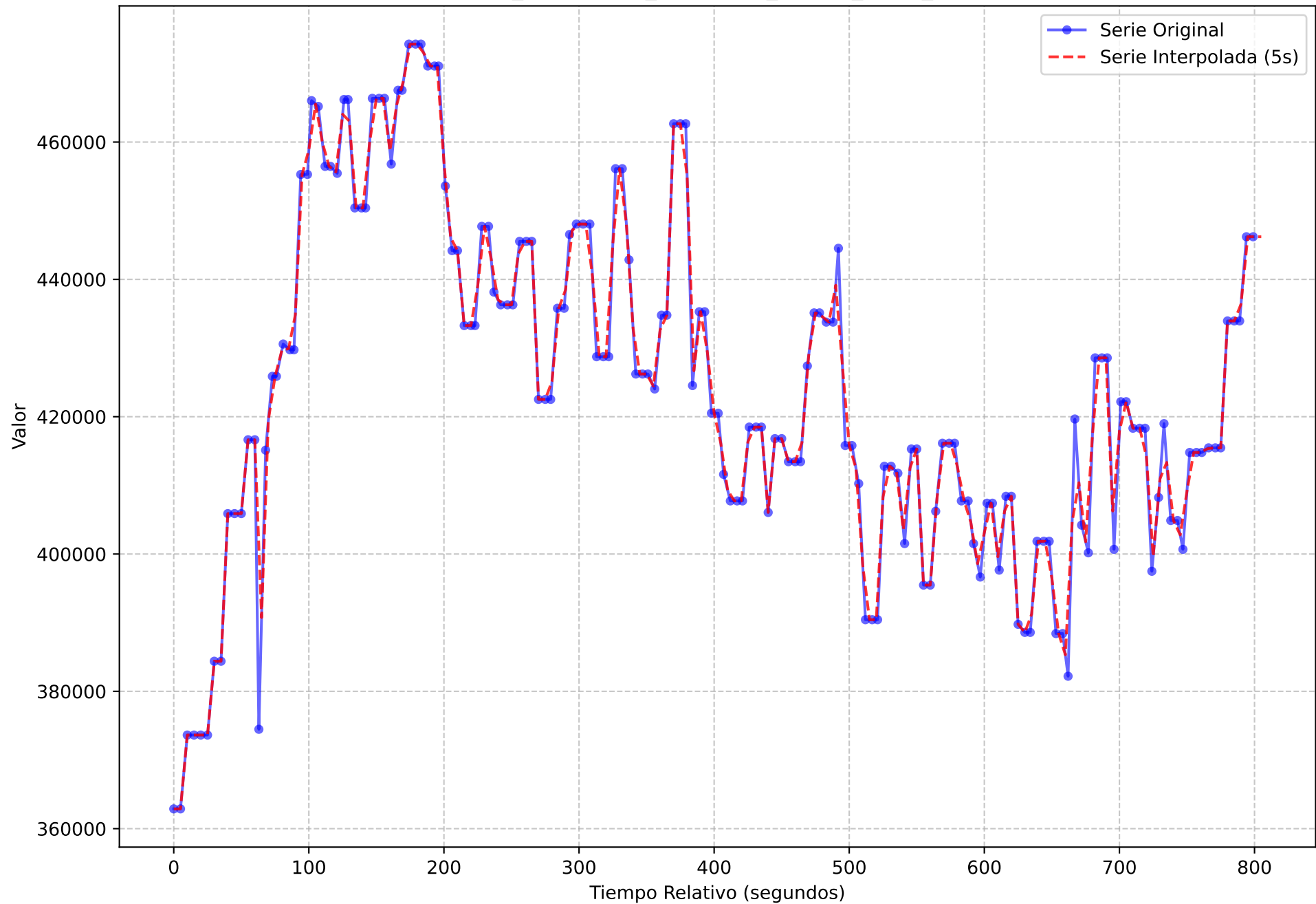
Serie Temporal Original vs. Interpolada (Muestreo 5s) execution_name = light-oauth2-data-1720167247.tar metric_name = go_memstats_mspan_inuse_bytes
