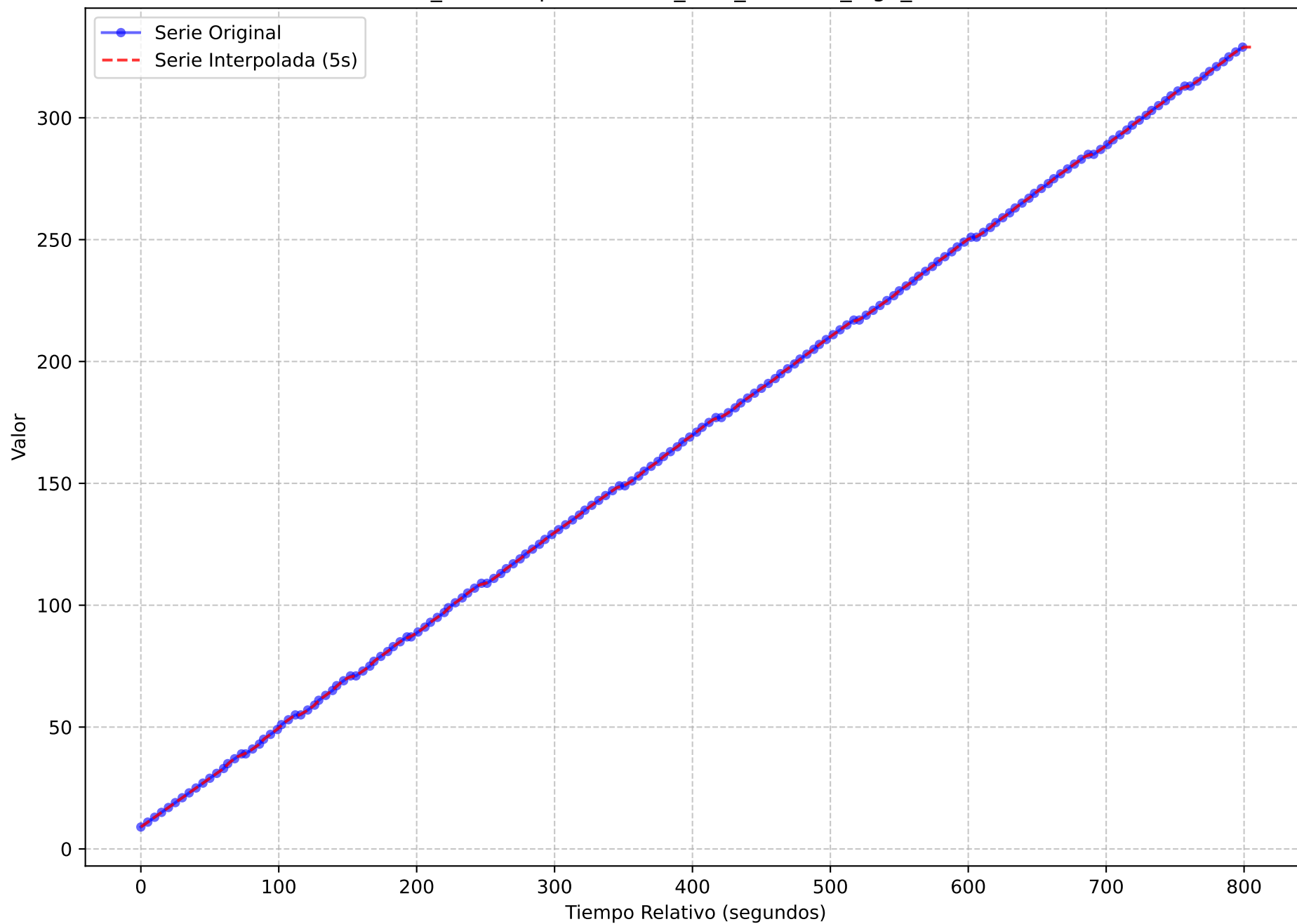
Serie Temporal Original vs. Interpolada (Muestreo 5s) execution_name = light-oauth2-data-1720167247.tar metric_name = prometheus_tsdb_isolation_high_watermark
