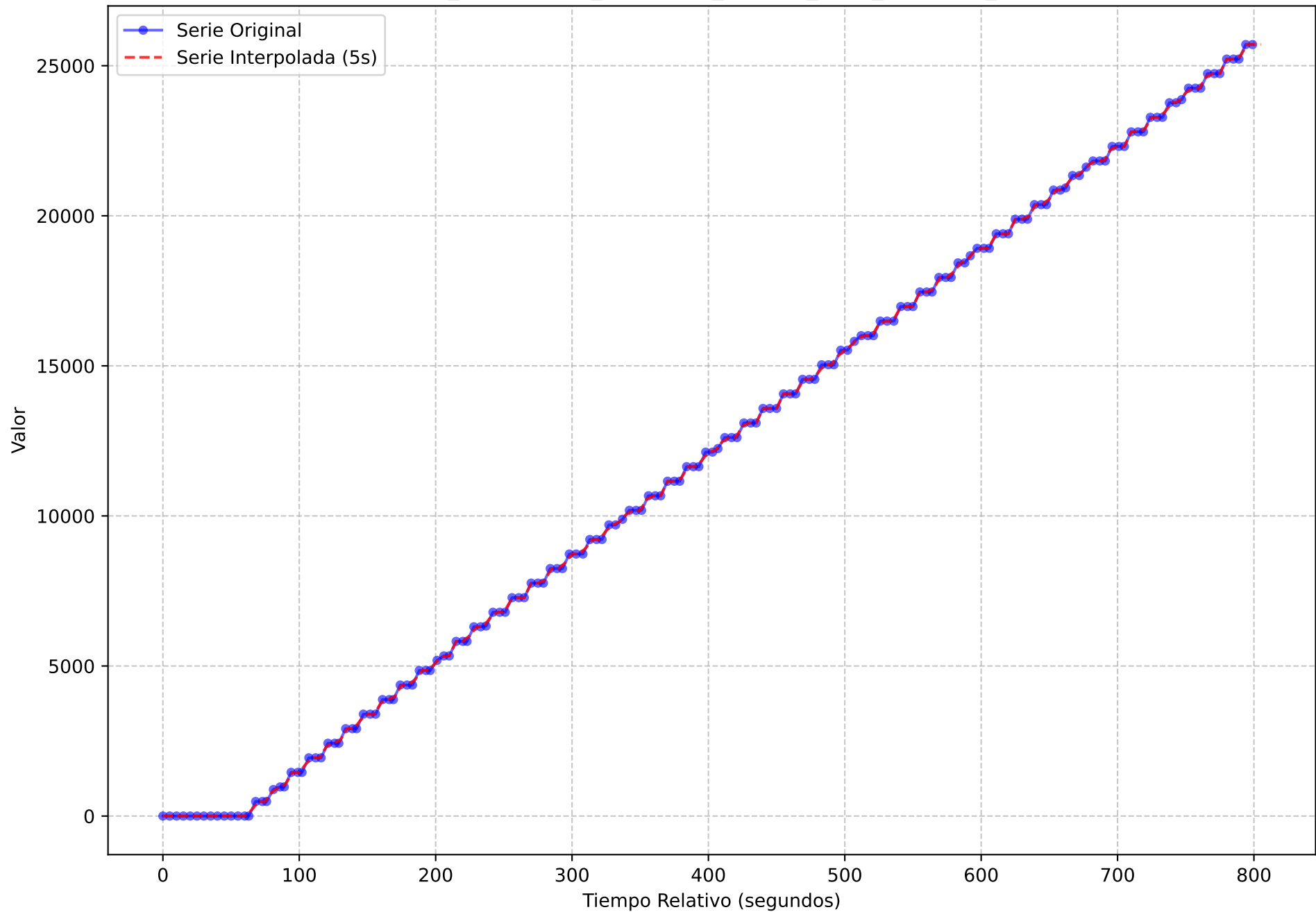
Serie Temporal Original vs. Interpolada (Muestreo 5s) execution_name = light-oauth2-data-1720167247.tar metric_name = net_contrack_listener_conn_accepted_total
