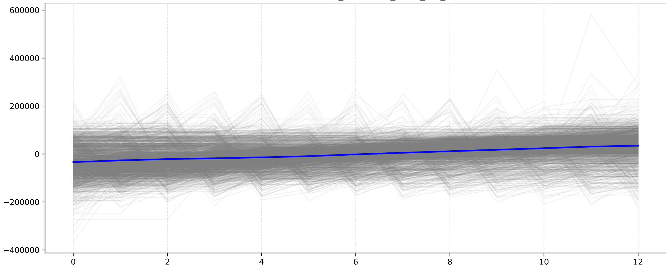
Series Centradas: go_memstats_stack_sys_bytes
