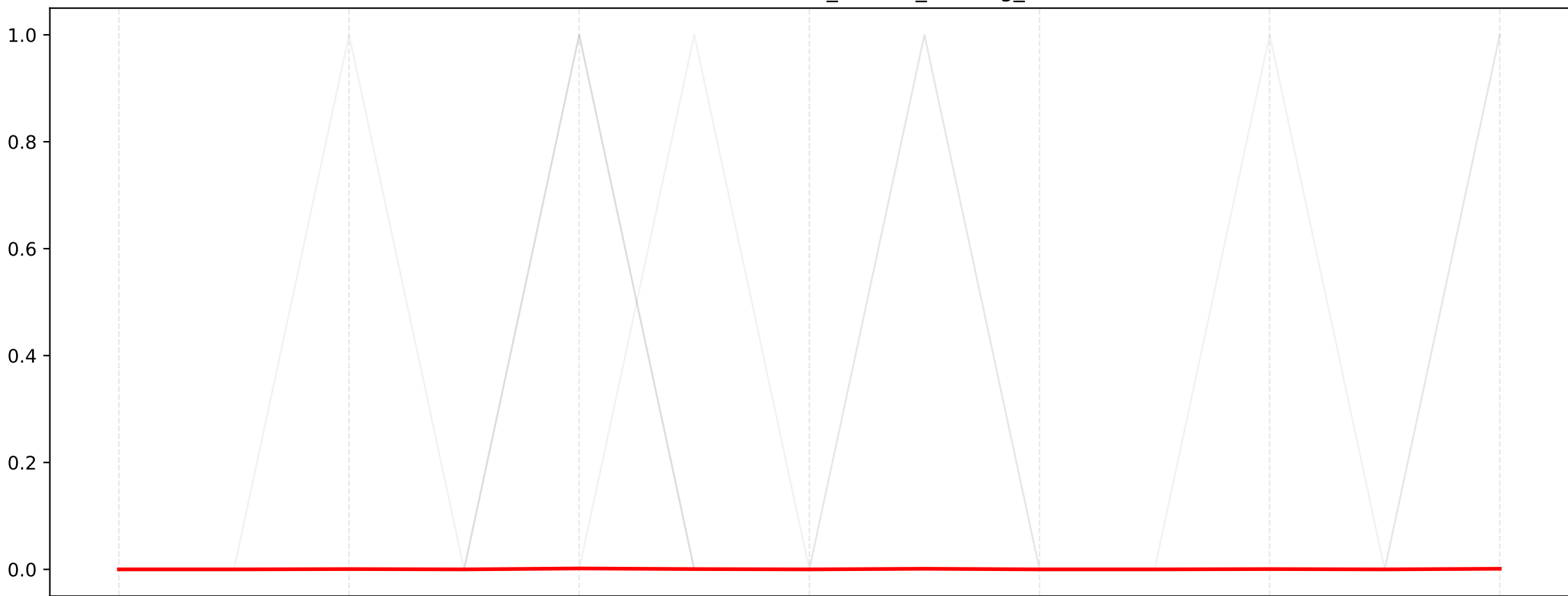
Series Centradas: node_softnet_backlog_len
