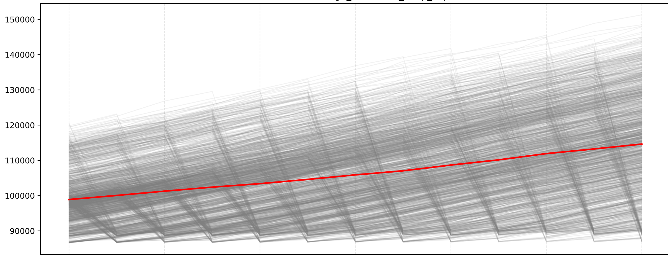
Series Centradas: go_memstats_heap_objects
