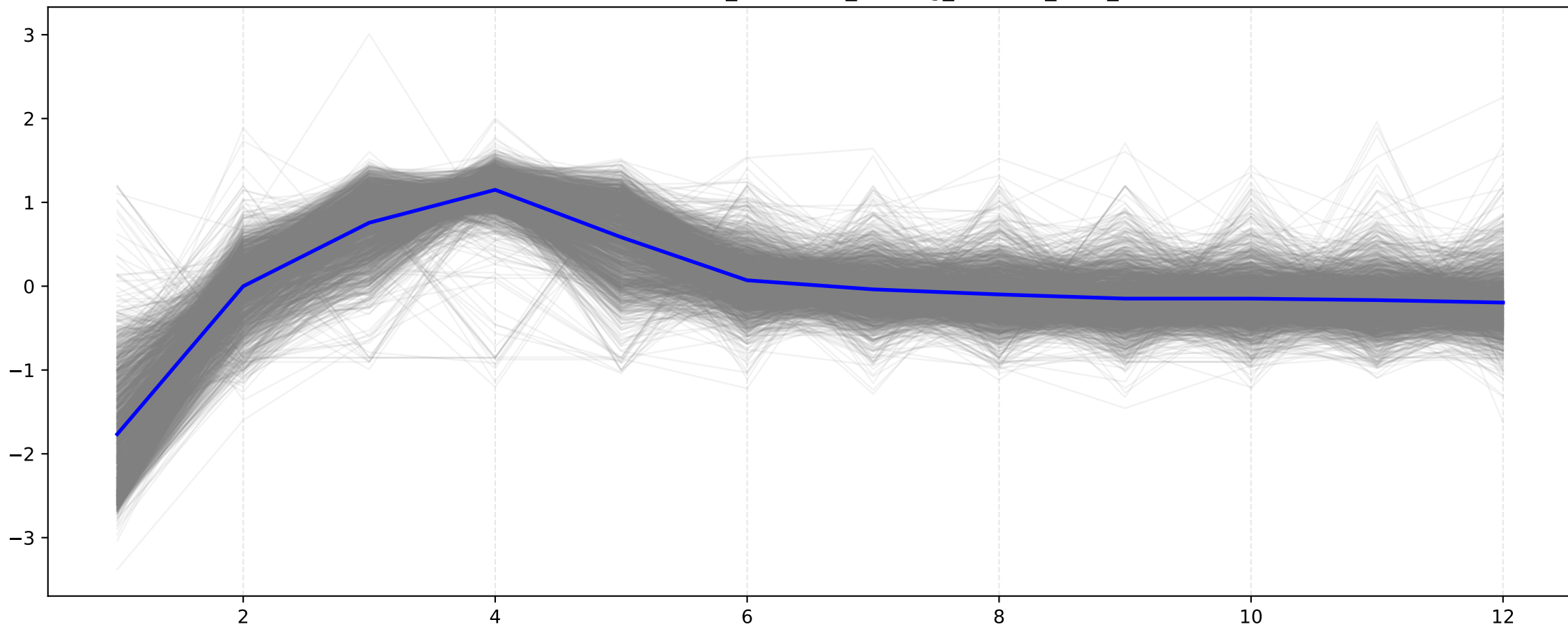
Series Centradas: node_schedstat_running_seconds_total_diff
