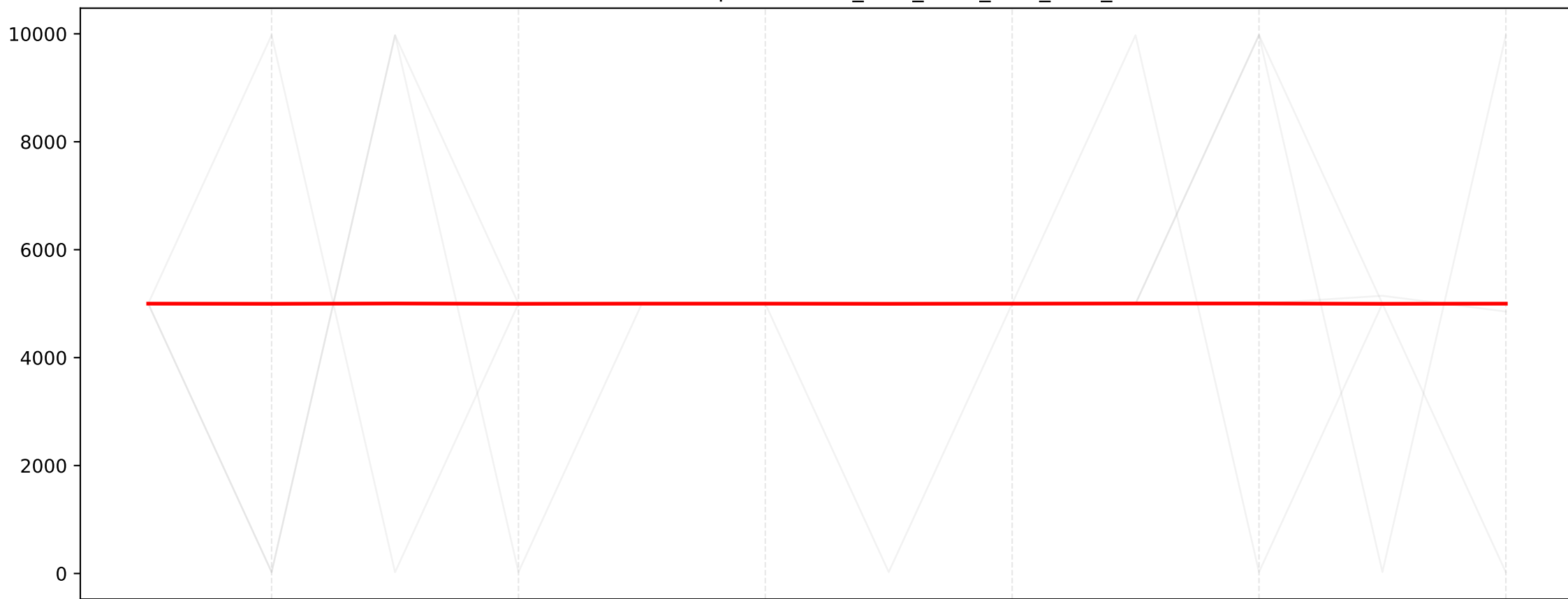
Series Centradas: prometheus_tsdb_head_max_time_diff
