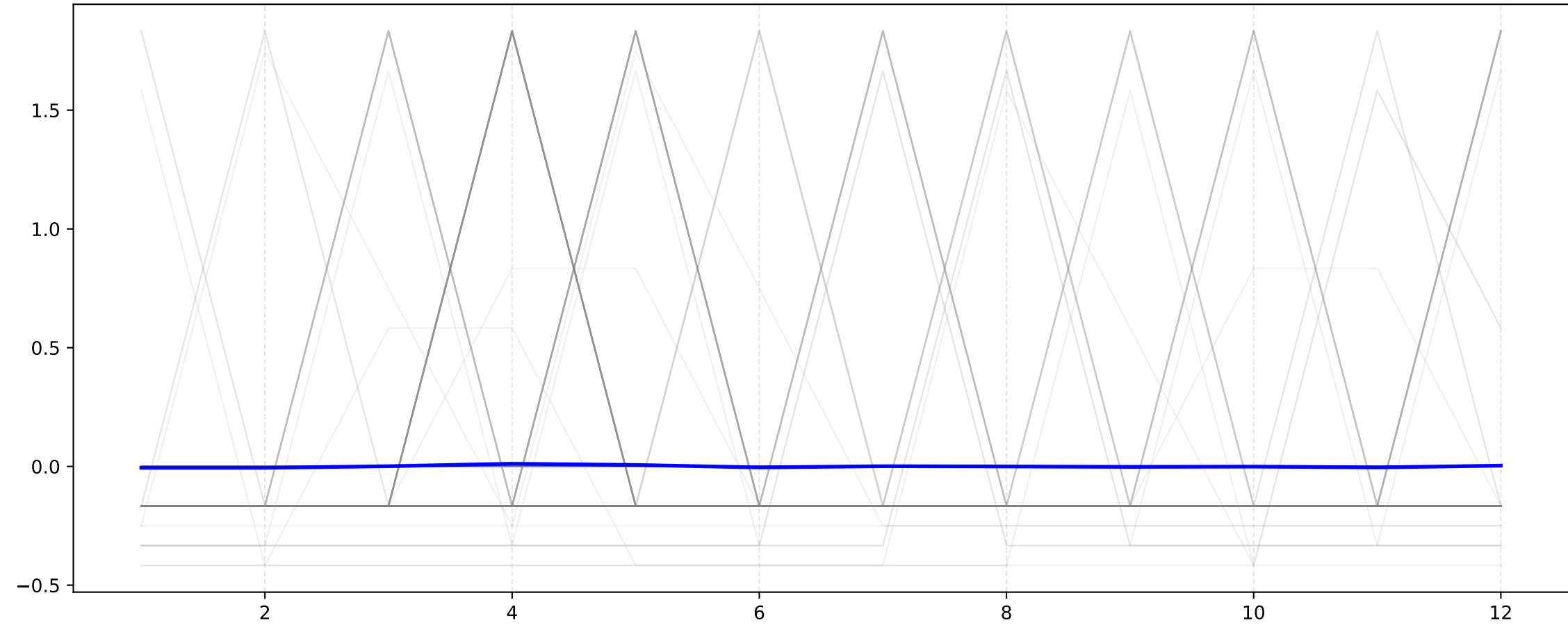
Series Centradas: node_netstat_Tcp_OutSegs_diff
