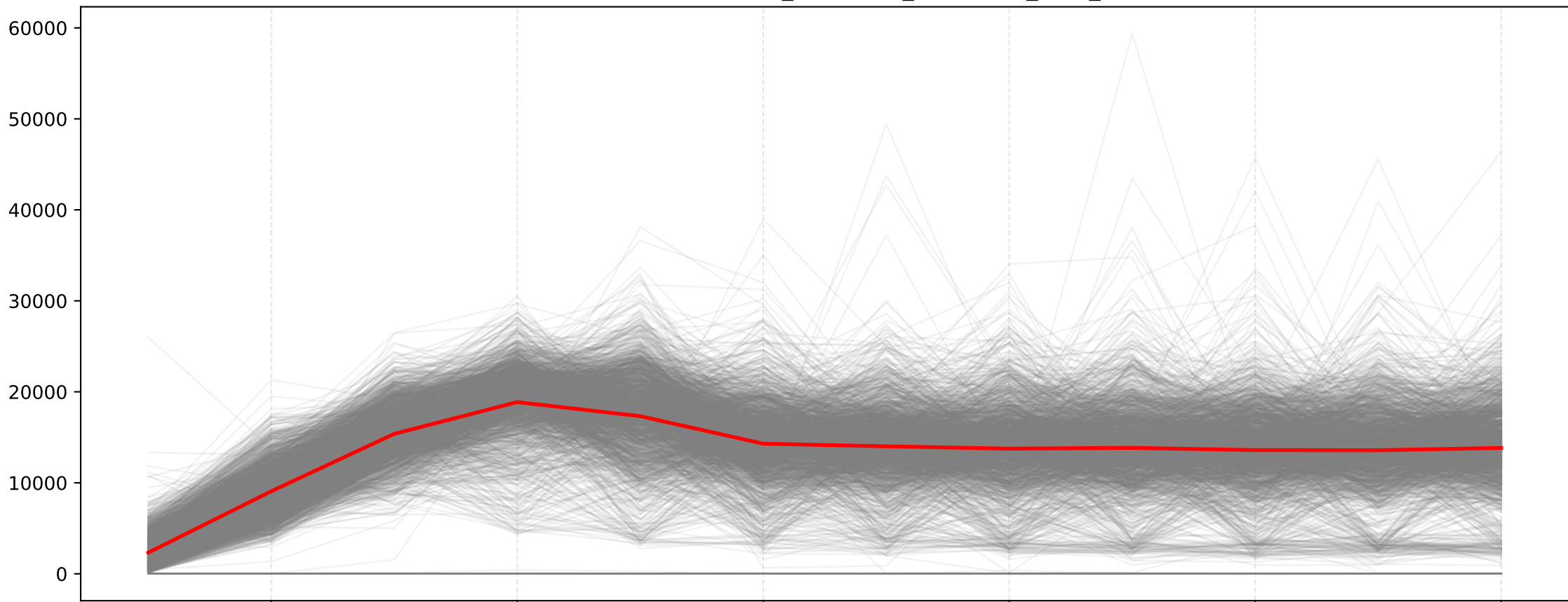
Series Centradas: node_schedstat_timeslices_total_diff
