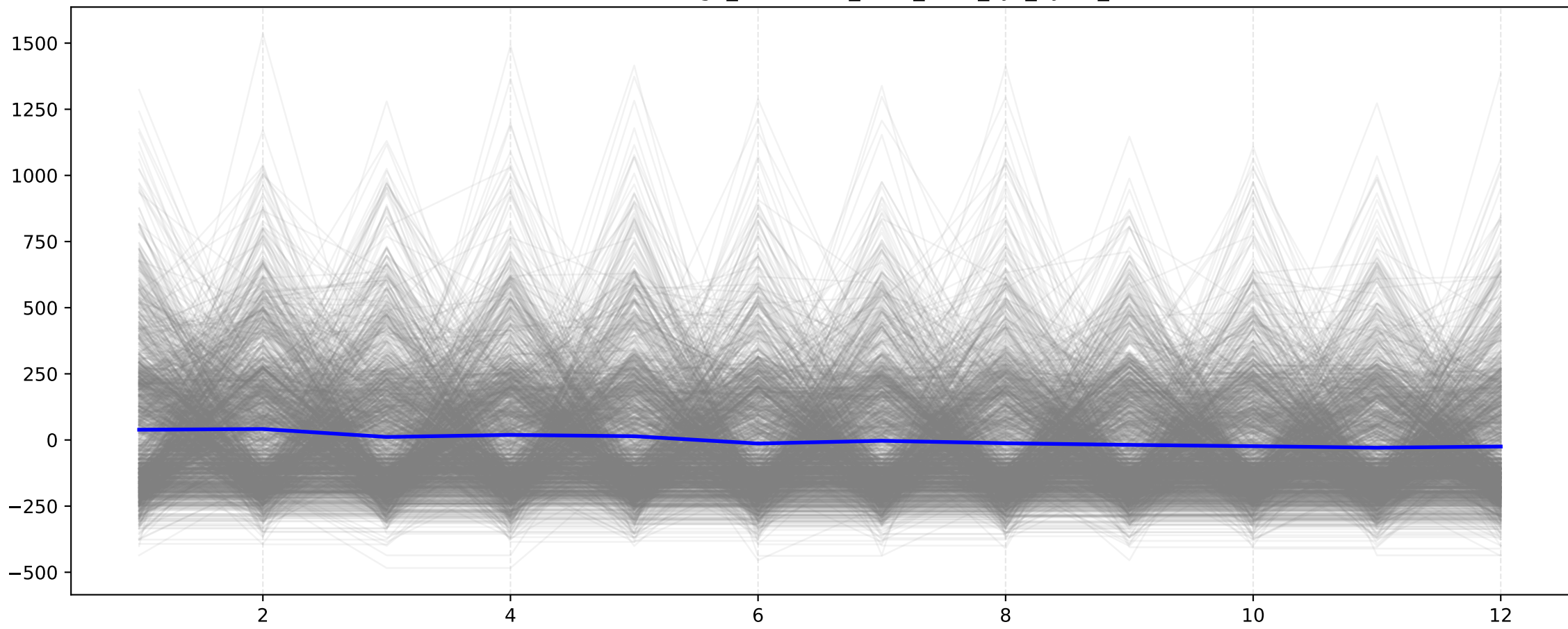
Series Centradas: go_memstats_buck_hash_sys_bytes_diff
