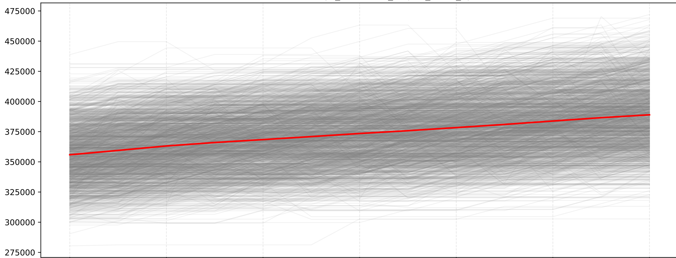
Series Centradas: go_memstats_mspan_inuse_bytes
