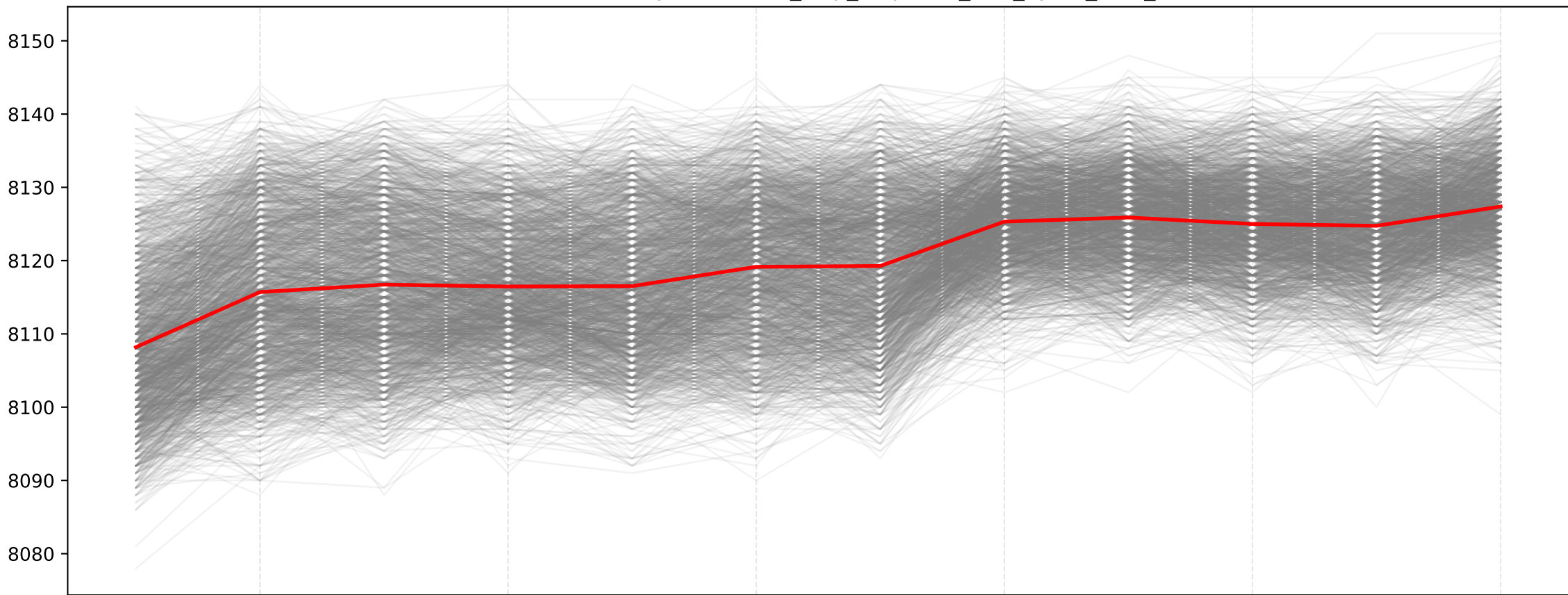
Series Centradas: prometheus_http_response_size_bytes_sum_diff
