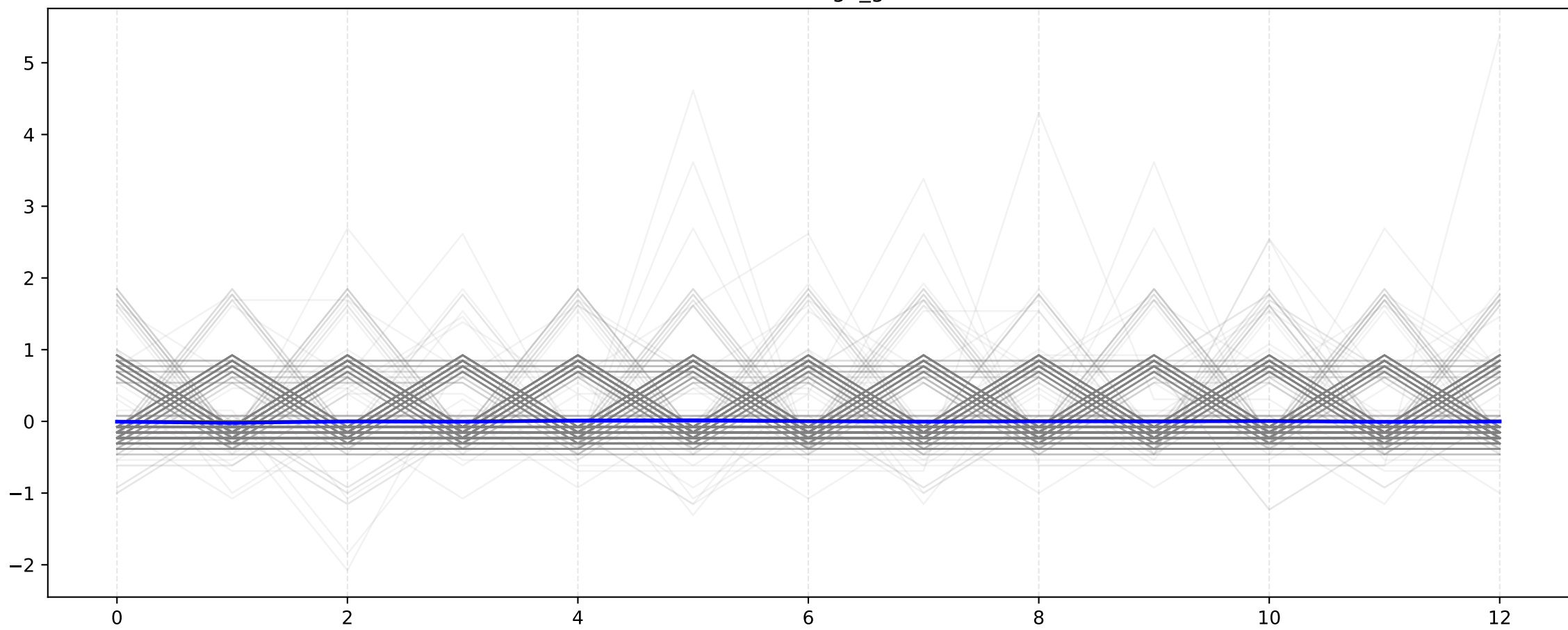
Series Centradas: go_goroutines
