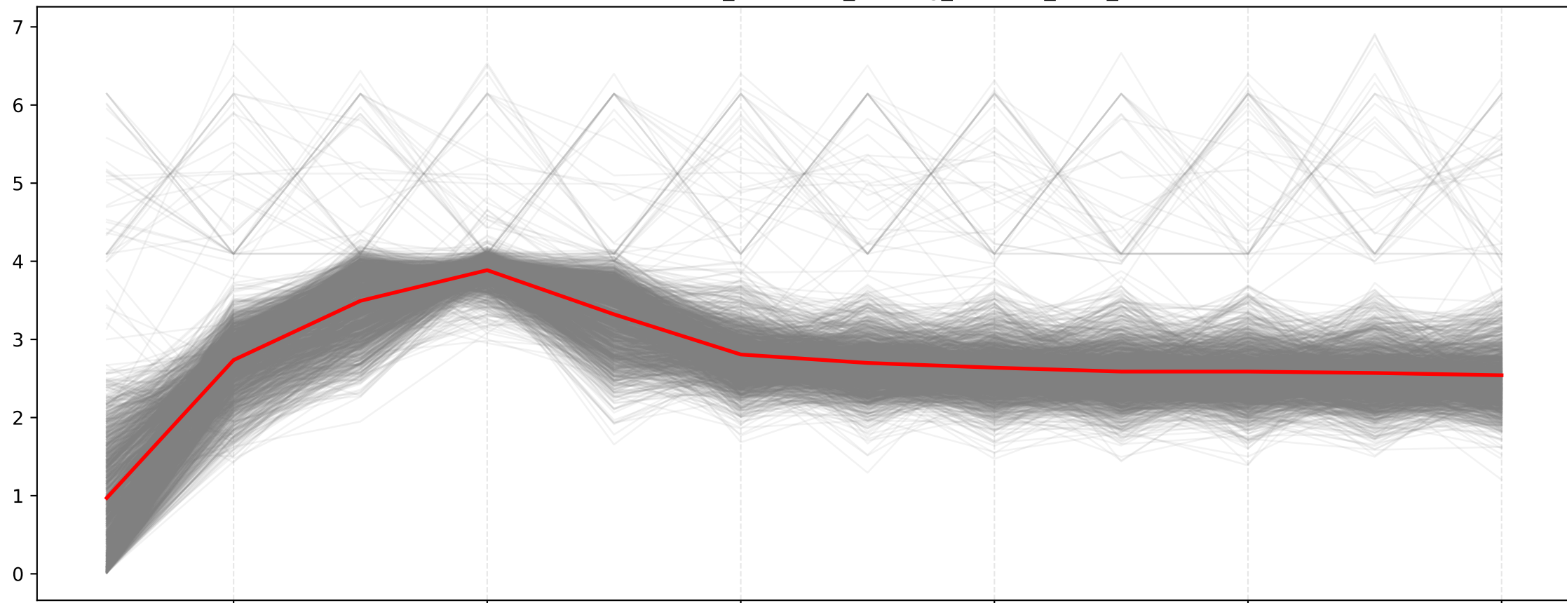
Series Centradas: node_schedstat_running_seconds_total_diff
