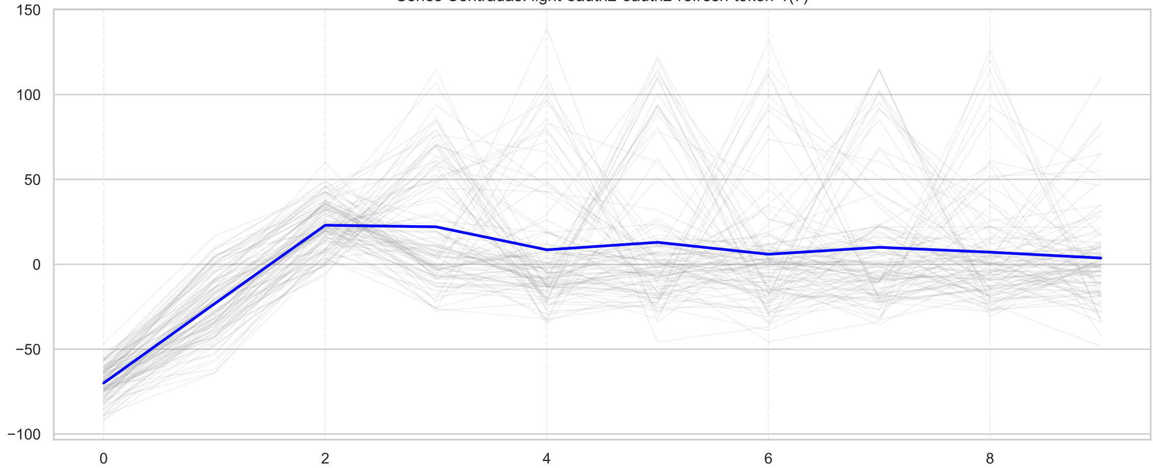
Series Centradas: light-oauth2-oauth2-refresh-token-1(7)
