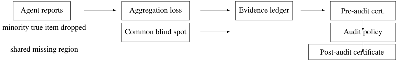
Figure 1: False convergence mechanisms and the decoupled completion workflow. Holdout gain is not a pre-audit signal; it updates the ledger only after audit.
