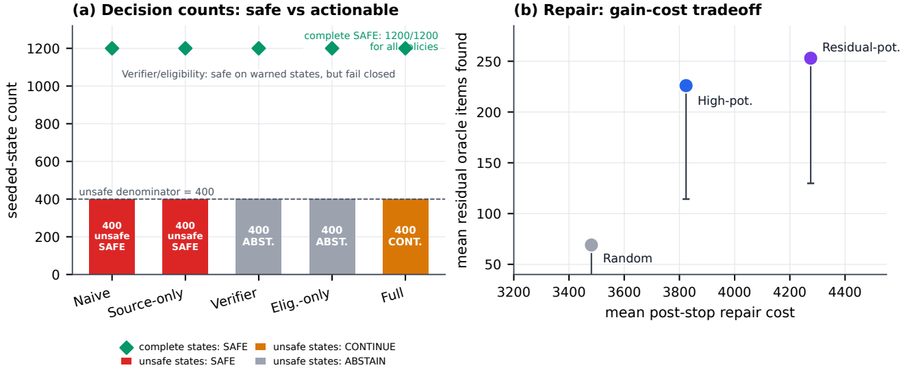
Figure 4: Controller evaluation dashboard for safe, actionable, and cost-aware stopping on seeded residual-warning states and seeded complete-state perturbations. The decision panel compares safety and usefulness: verifier-gate is safe on this denominator but fail-closed, while the full controller is safe and actionable on unsafe states with runtime residual candidates. The repair panel compares target rules and budget choices, showing residual-potential as a high-yield but non-optimal repair heuristic.
