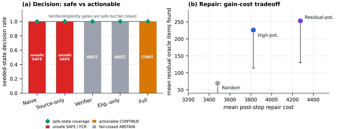
Figure 4: Controller evaluation dashboard for safe, actionable, and cost-aware stopping on seeded residual-warning states and seeded complete-state perturbations. The decision panel compares safety and usefulness: verifier-gate is safe on this denominator but fail-closed, while the full controller is safe and actionable on unsafe states with runtime residual candidates. The repair panel compares target rules and budget choices, showing residual-potential as a high-yield but non-optimal repair heuristic.
