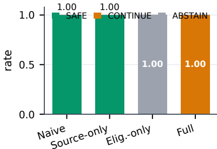
Unsafe states: decision mix
