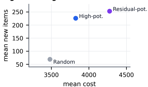
Repair target variants: mean gain vs. cost
