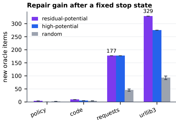
Figure 5: Repair gain for residual-potential, high-potential, and random probes with 95% confidence intervals. Sensitivity details are reported in the supplementary material.
