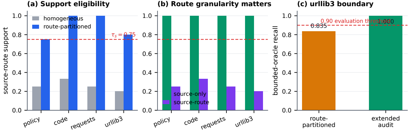
Figure 3: Main diagnostic and ablation. Left: homogeneous base states have low source-route support; broader audits increase support. Middle: source-only support is full in homogeneous runs, but source-route support remains localized, exposing the route-level certificate mismatch. Right: urllib3 is the boundary case: route-partitioned audit is broad but incomplete, while the extended audit reaches completion. Dashed lines mark the operational support and recall thresholds used for evaluation.
