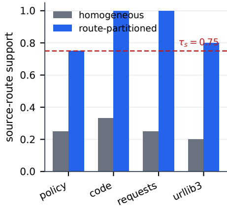
(a) Support eligibility
