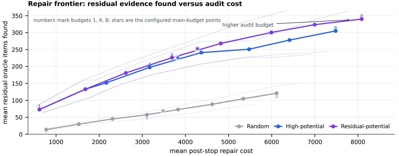
Figure 4: Repair cost frontier. Each curve averages the same seeded unsafe repair states over the two external repositories; faint traces show per-repository frontiers. Numbers mark budgets 1, 4, and 8, and stars mark the configured main-budget points used in Table 4. The plot is a cost-side complement to the decision table: residual-potential repair exposes more residual evidence than random repair, but it spends more audit budget.
