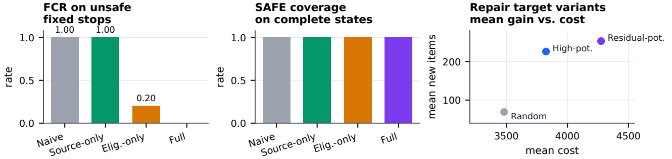
Figure 1: Controller variant comparison. Naive stop acceptance and source-only control accept unsafe observed stop states. Source-route eligibility reduces false SAFE decisions but remains insufficient on the broad-but-productive urllib3 boundary. Repair-enabled variants preserve safe-state coverage; residual-potential is the method instance used by the full controller.
