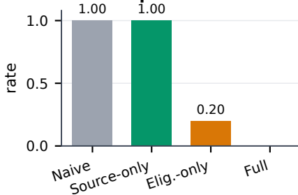
FCR on unsafe fixed stops
