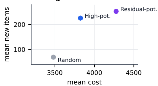
Repair target variants mean gain vs. cost
