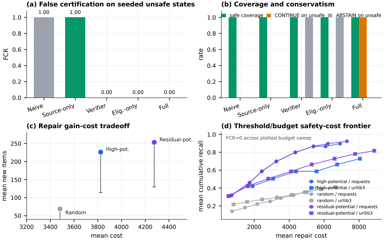
Figure 1: Controller variant comparison. Naive stop acceptance and source-only control accept seeded unsafe states. The full controller and repair-enabled variants avoid SAFE on seeded unsafe repair states while preserving SAFE coverage on seeded complete states. Source-route eligibility alone is evaluated separately on the broad-but-productive urllib3 fixed boundary in the main text.
