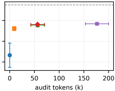
Click
