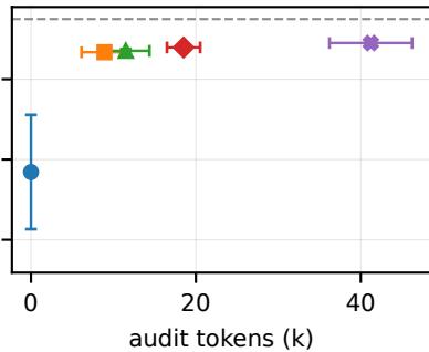
itsdangerous
