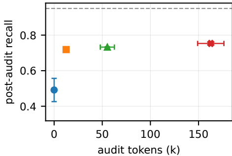
Requests
