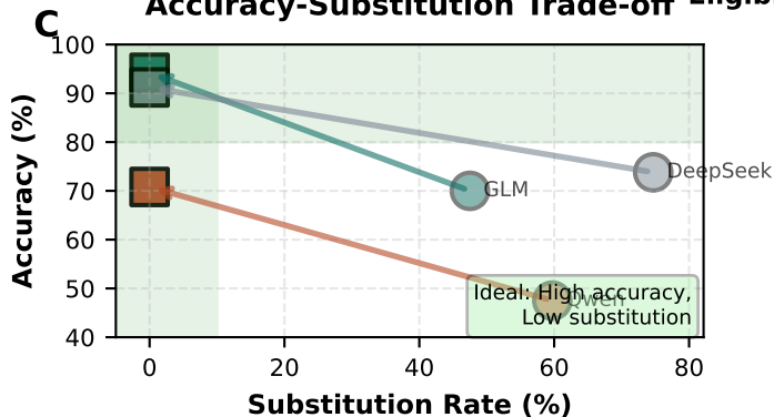
Accuracy-Substitution Trade-off
