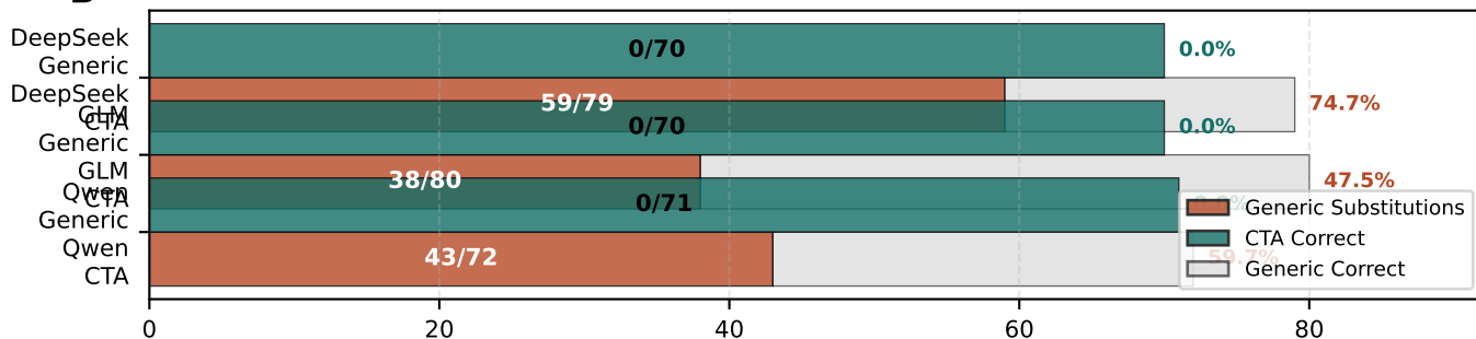
Accuracy-Substitution Trade-off
