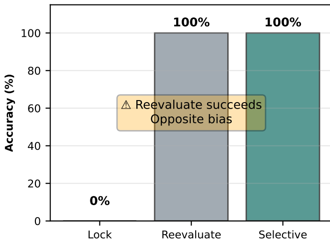
C Reevaluate-Only: Favors Reevaluate
