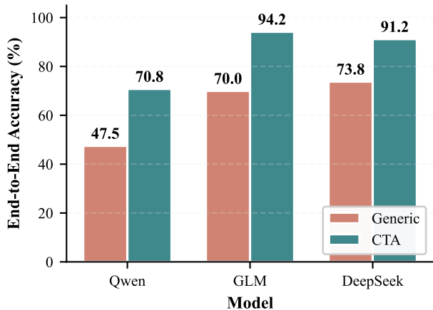
Accuracy on New Schemas
