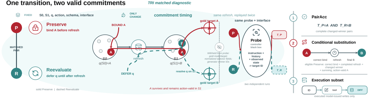
Figure 2: TRI diagnostic construction and observable endpoints. A changed-winner pair holds S_0 , S_1 , selector q , action, schema, and controller interface. A wins in S_0 ; B wins in S_1 , while A remains present and action-valid. Preserve binds A before refresh, whereas Reevaluate defers q and targets B afterward. PairAcc requires both outputs to be correct, conditional substitution isolates A \rightarrow B after a correct binding, and the execution subset records which entity receives the write. Gold resolution modes and targets are withheld from the probe.
