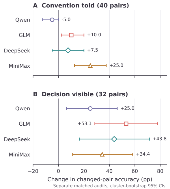
Figure 6: Post-primary equal-call contrasts. A: natural-language convention only (40 changed pairs). B: complete decision block visible to the actor (32 actionable changed pairs). Bars are cluster-bootstrap 95% CIs; inventories are separate and unpooled.
