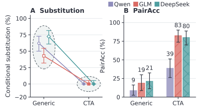
Figure 4: Ten-schema outcomes after correct initial binding. A: Generic versus CTA substitution on rows eligible under both controllers (Wilson 95% CIs; zero CTA estimates lie at the lower bound); ellipses group controller endpoints and lines link models. B: changed-winner PairAcc over 80 pairs (cluster-bootstrap 95% CIs); labels are rounded percentages. Counts (Qwen/GLM/DeepSeek) are Generic 7/15/17 of 80 and CTA 31/66/64 of 80. CTA makes no common-eligible substitutions; neither endpoint is a safety rate.
